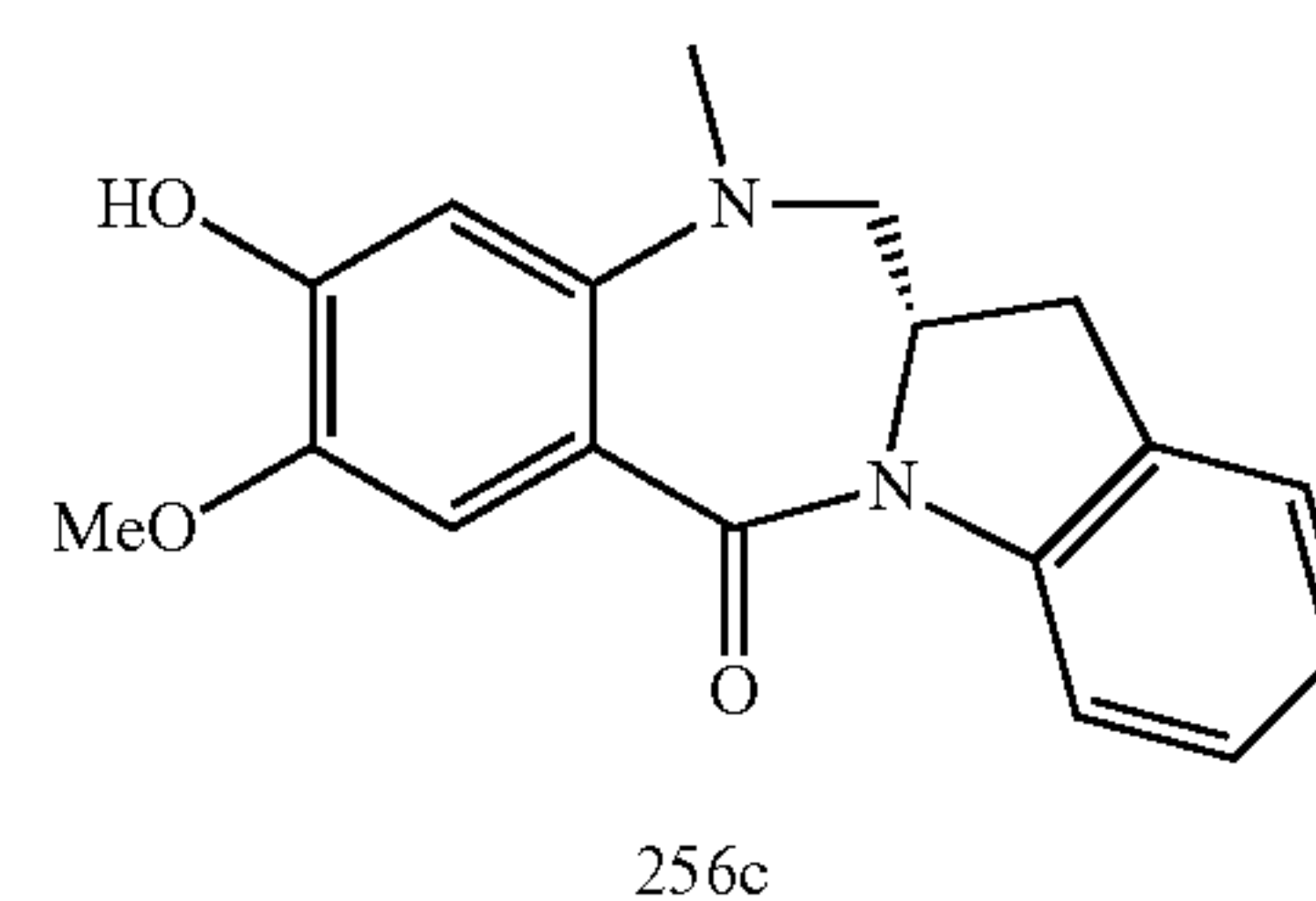
Compound 256c
