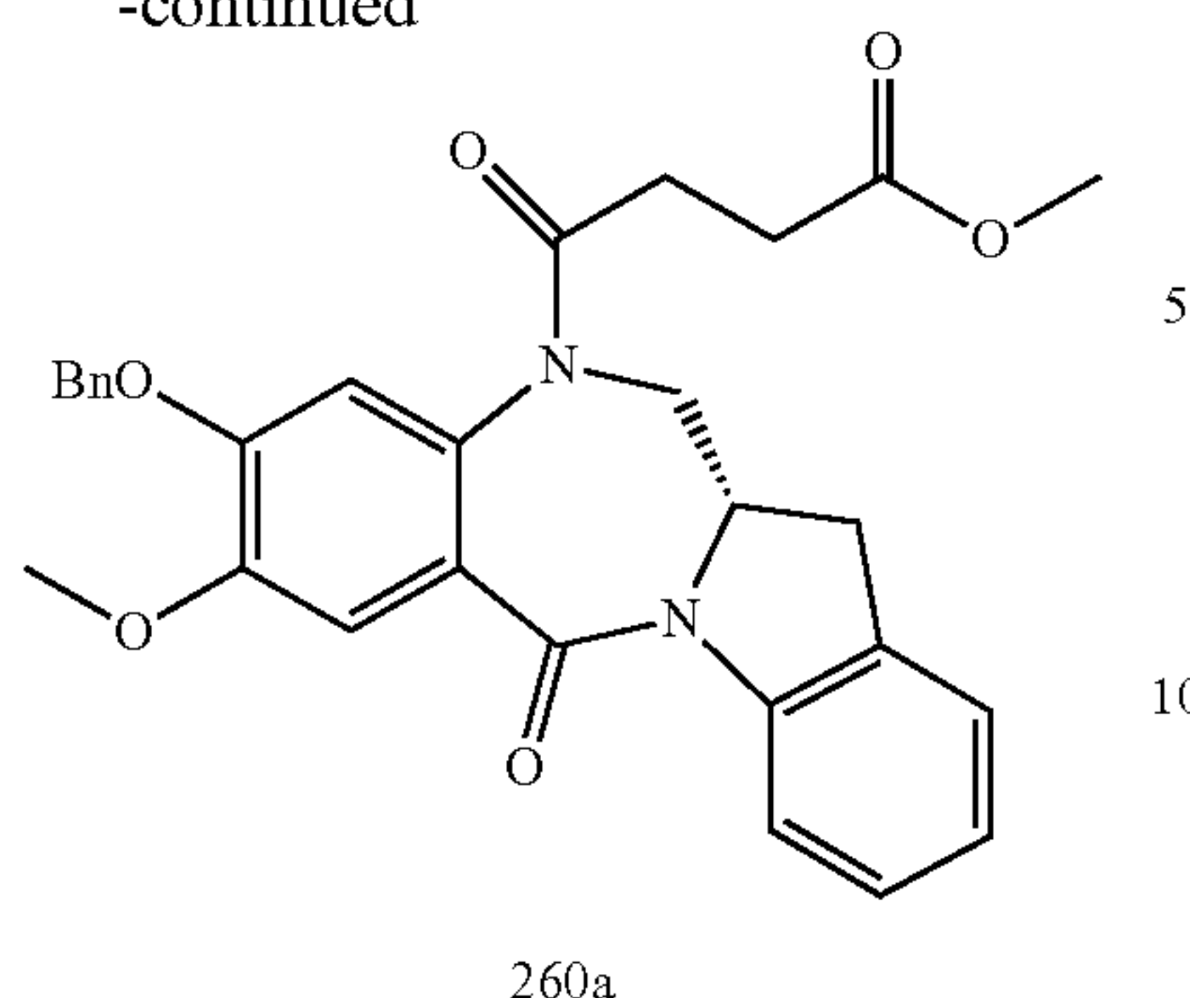
Compound 260a
