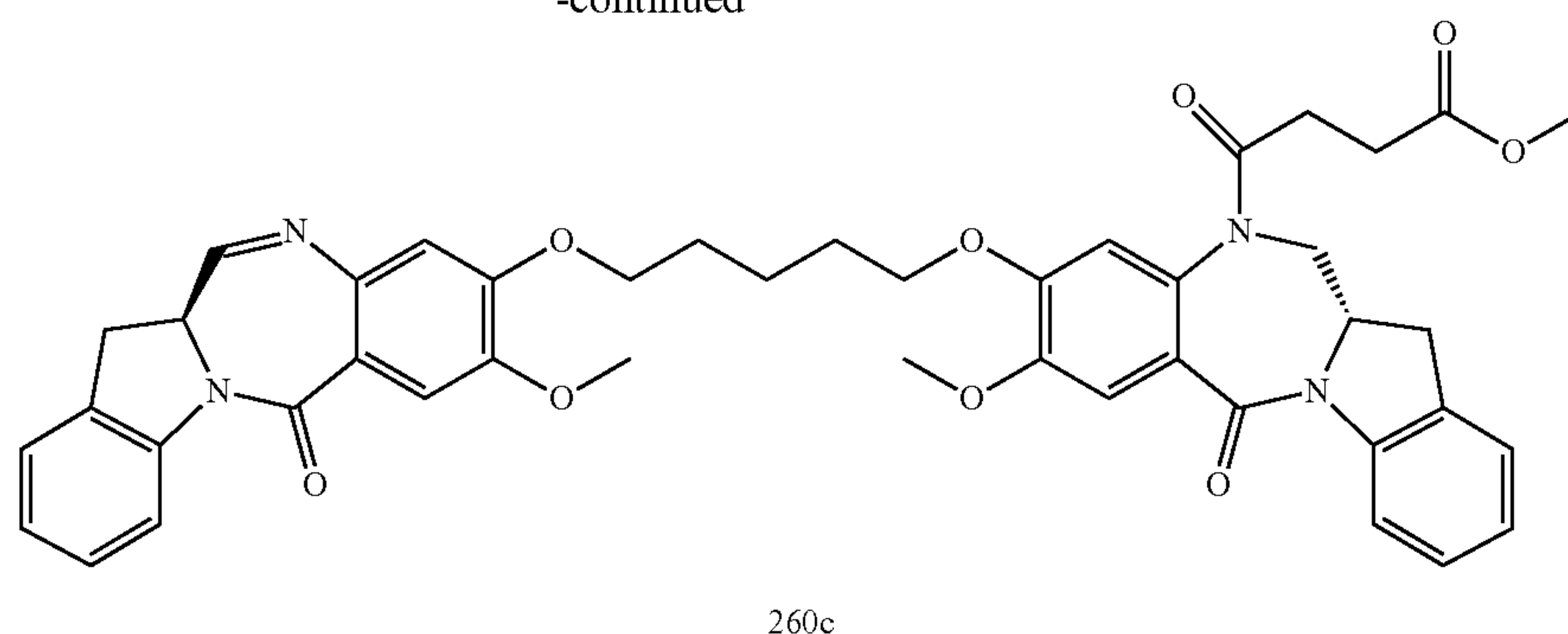
Compound 260c
