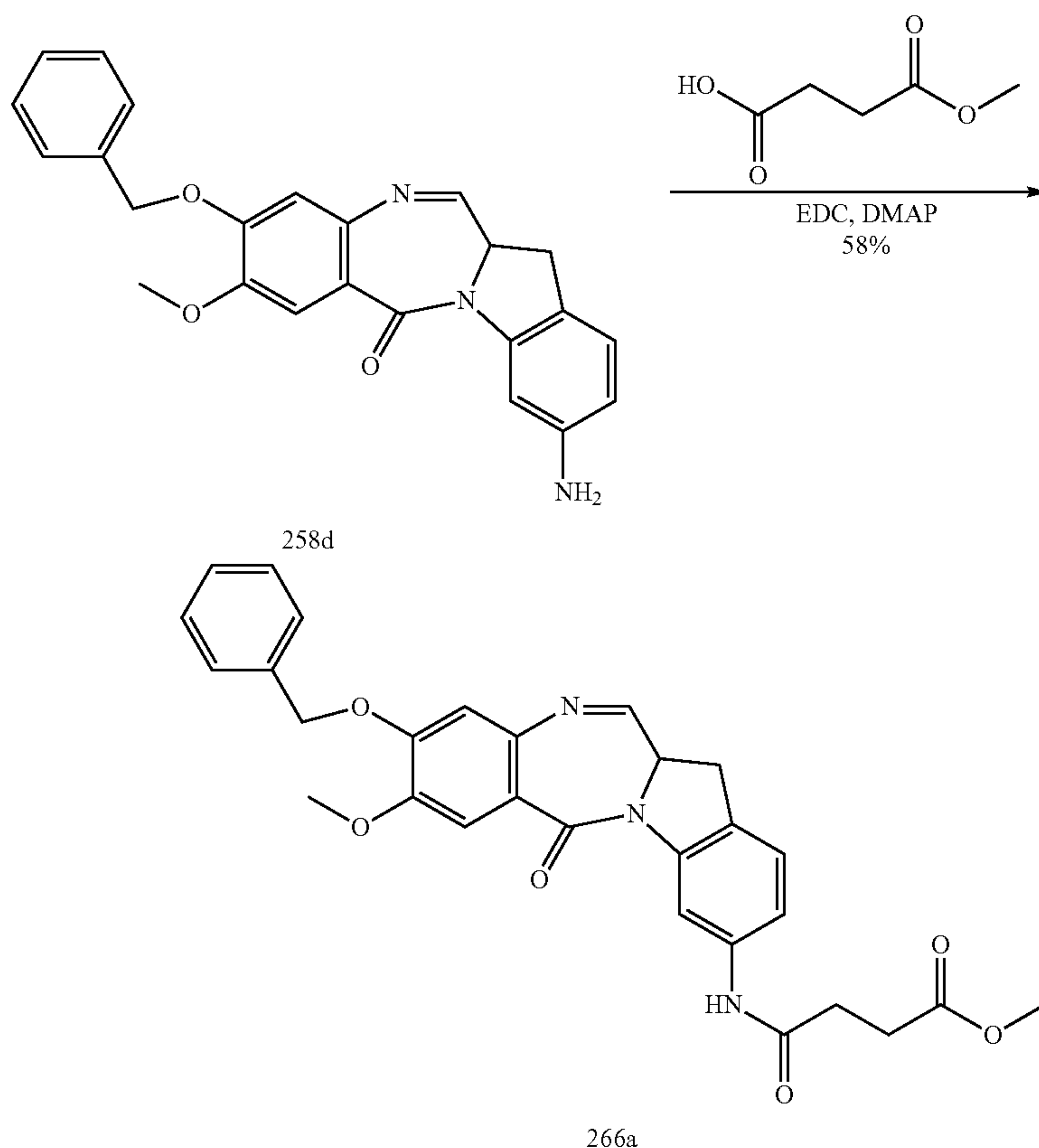
Compound 266a
