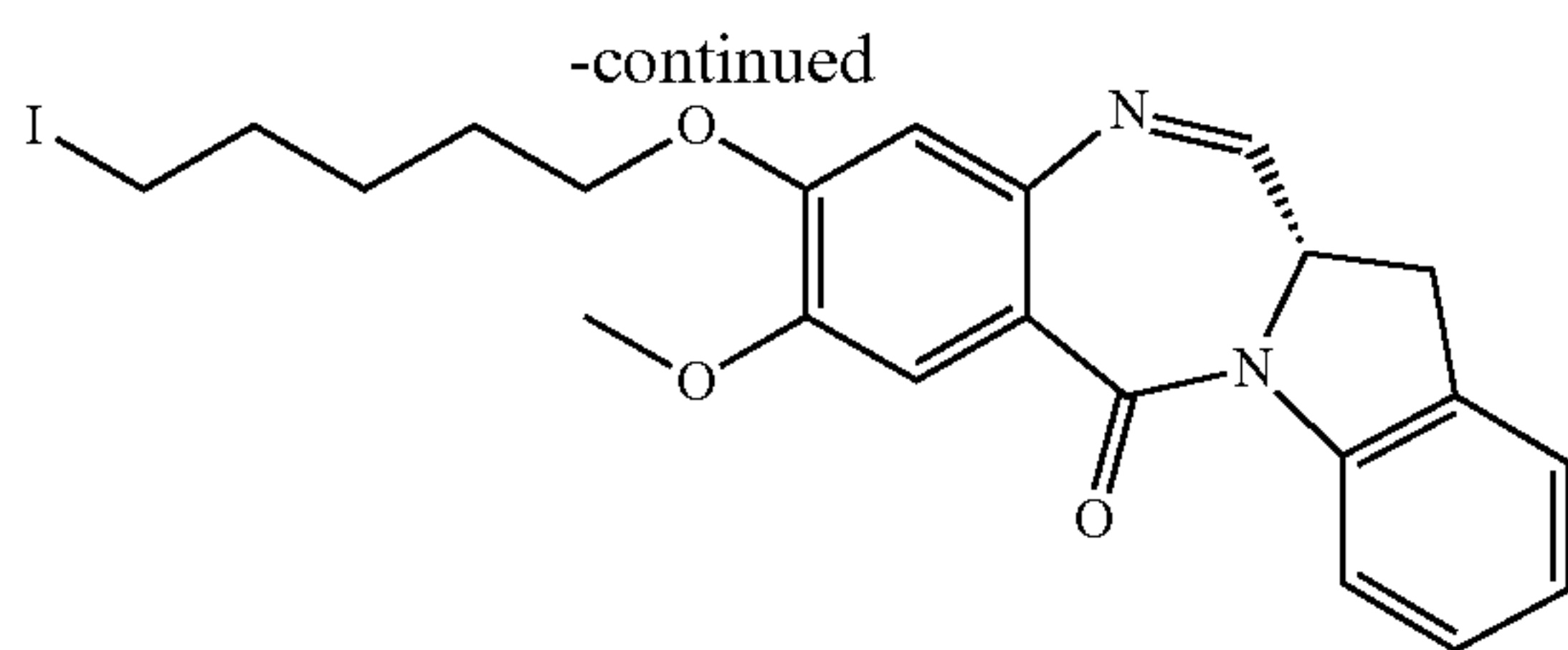
259a
