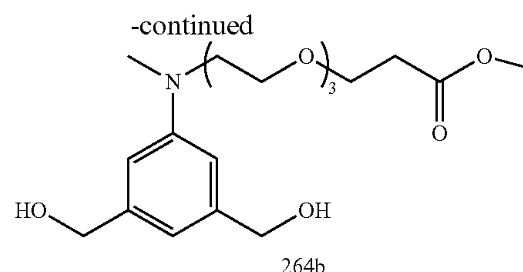
Compound 264b
