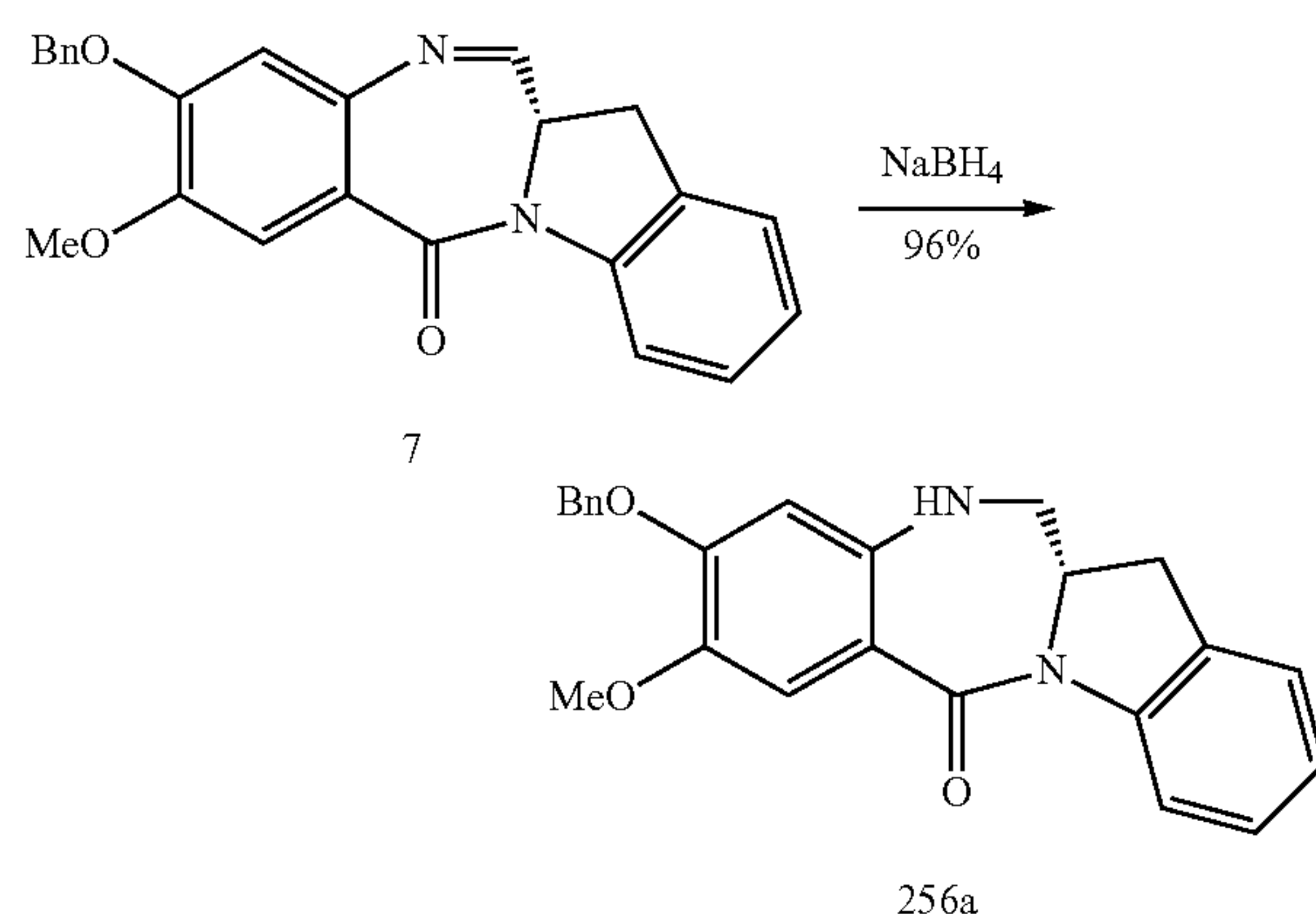
Compound 256a
