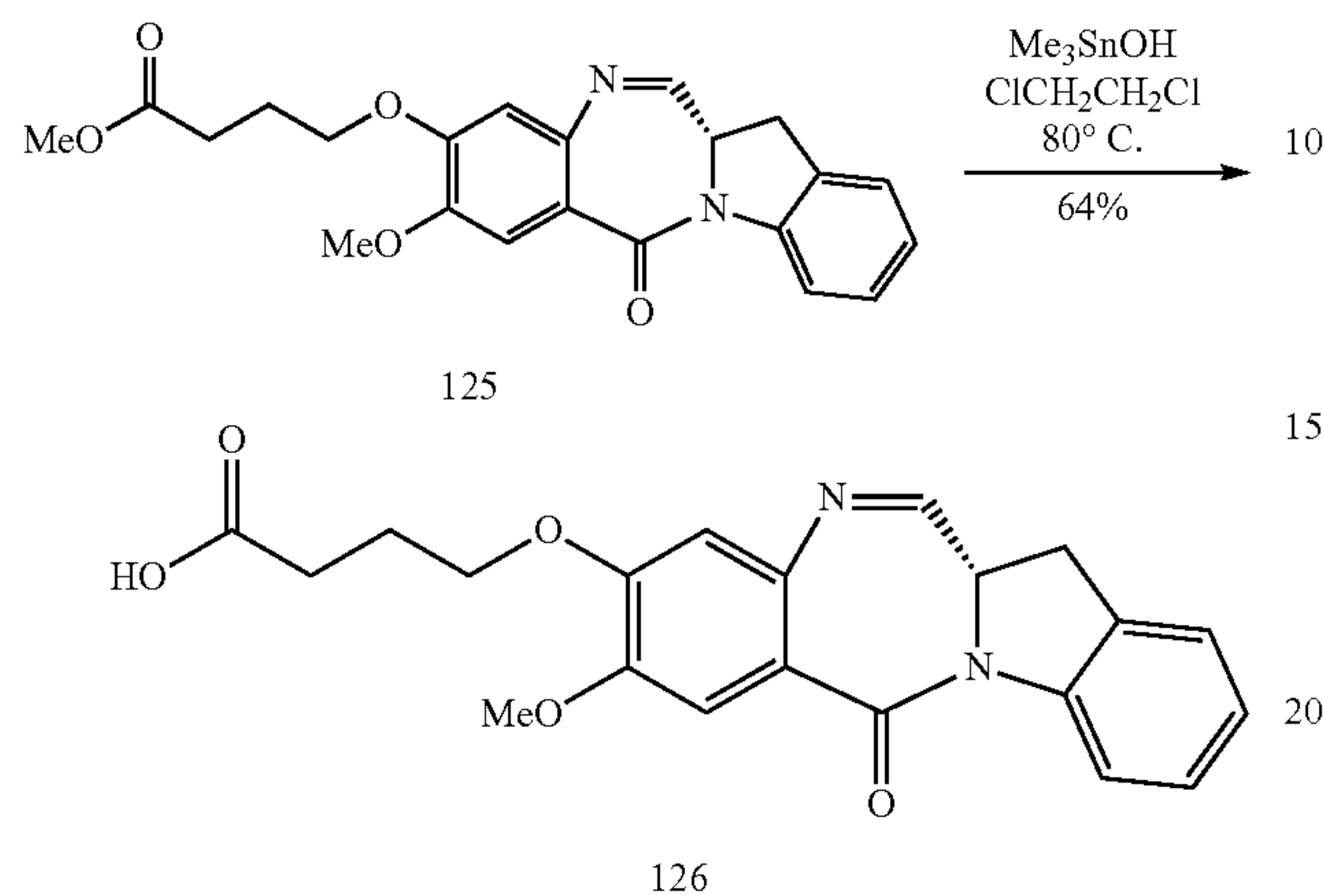
Compound 126
