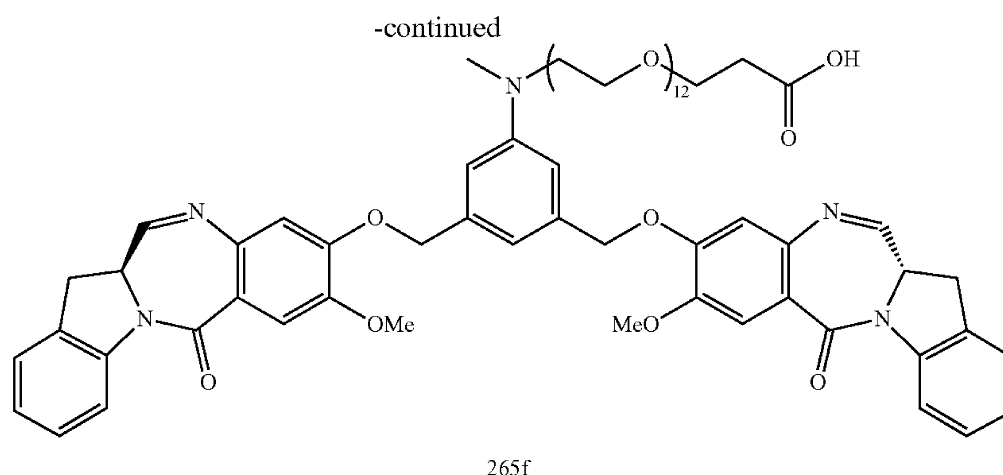
Compound 265f
