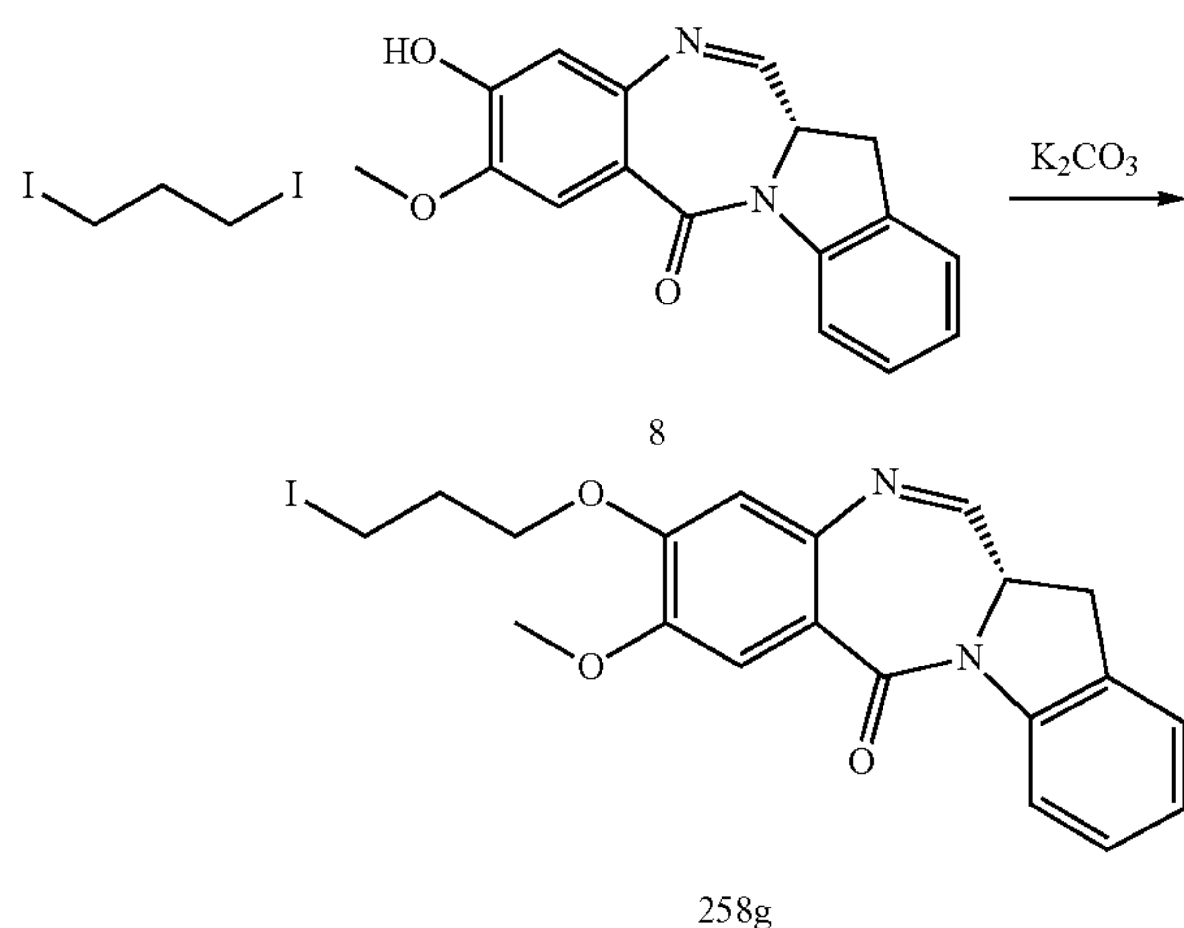
Compound 258g
