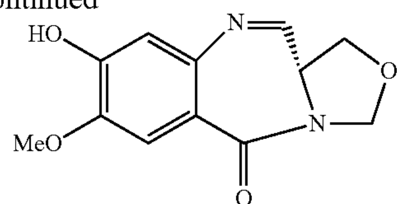
OBD monomer 14
