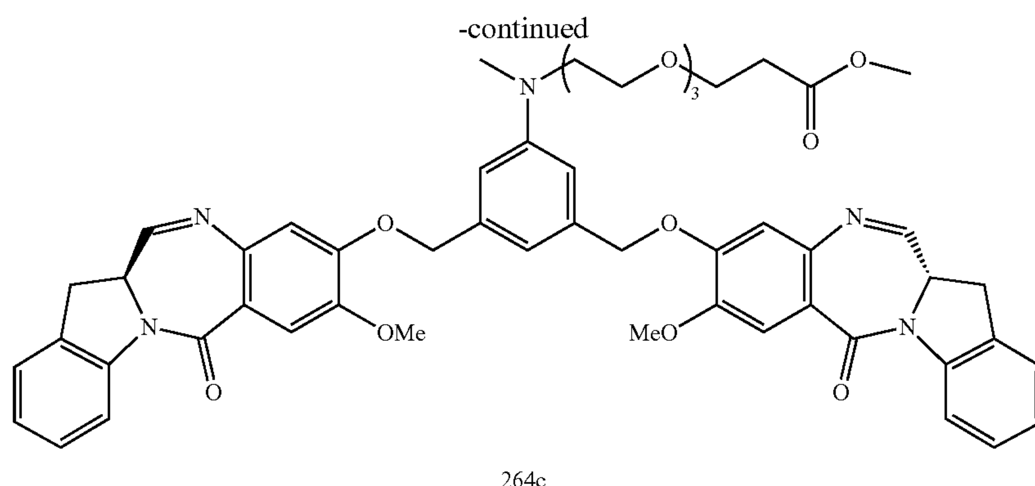
Compound 264c
