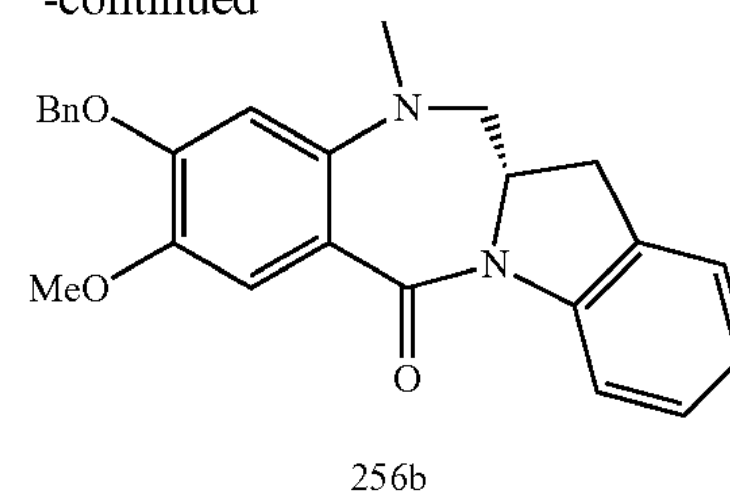
Compound 256b
