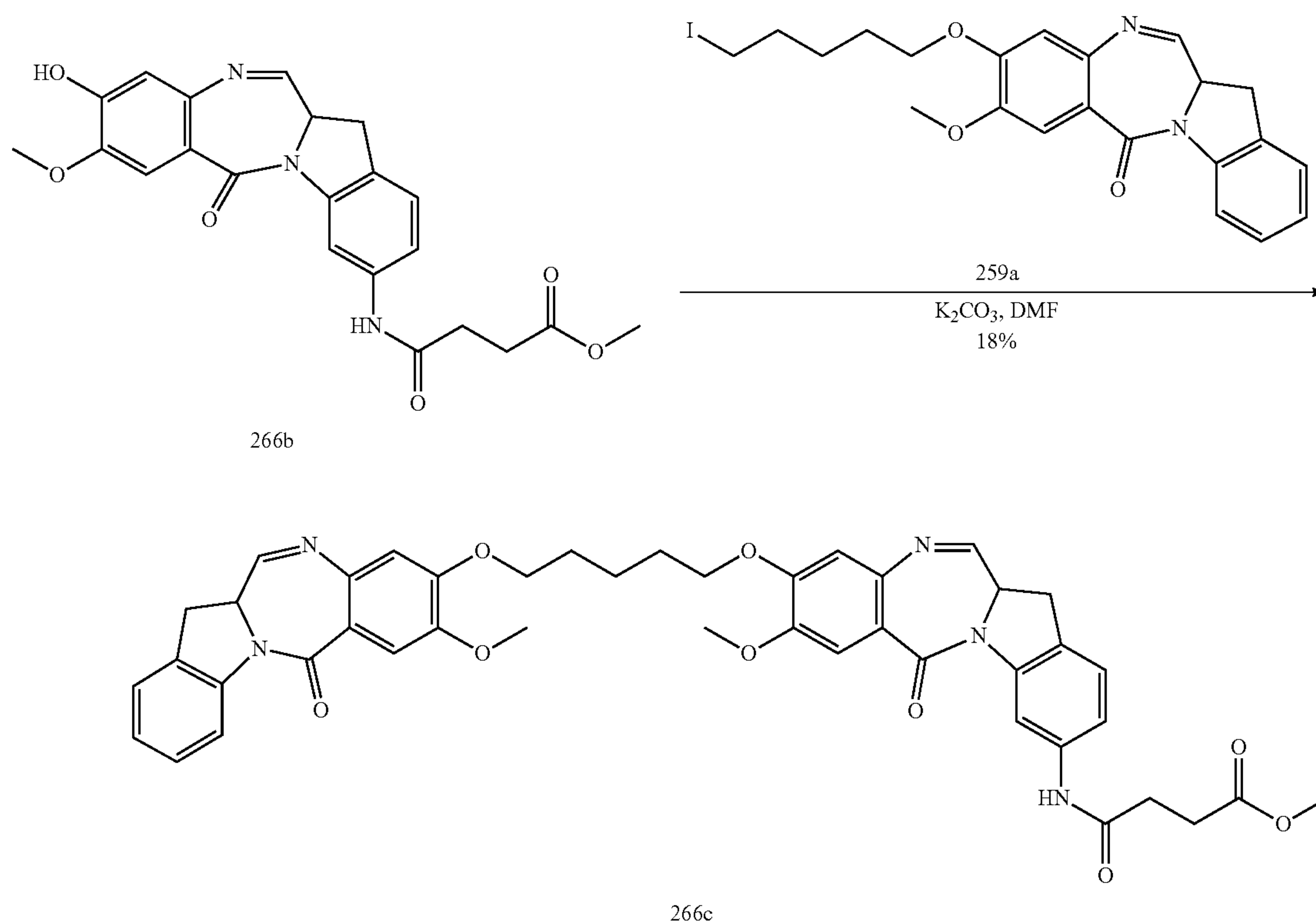
Compound 266c
