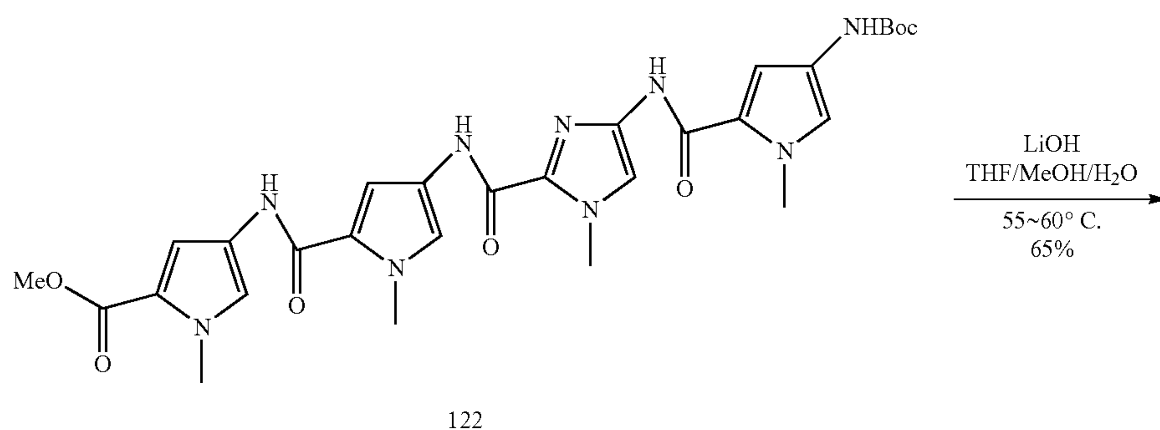
Compound 123
