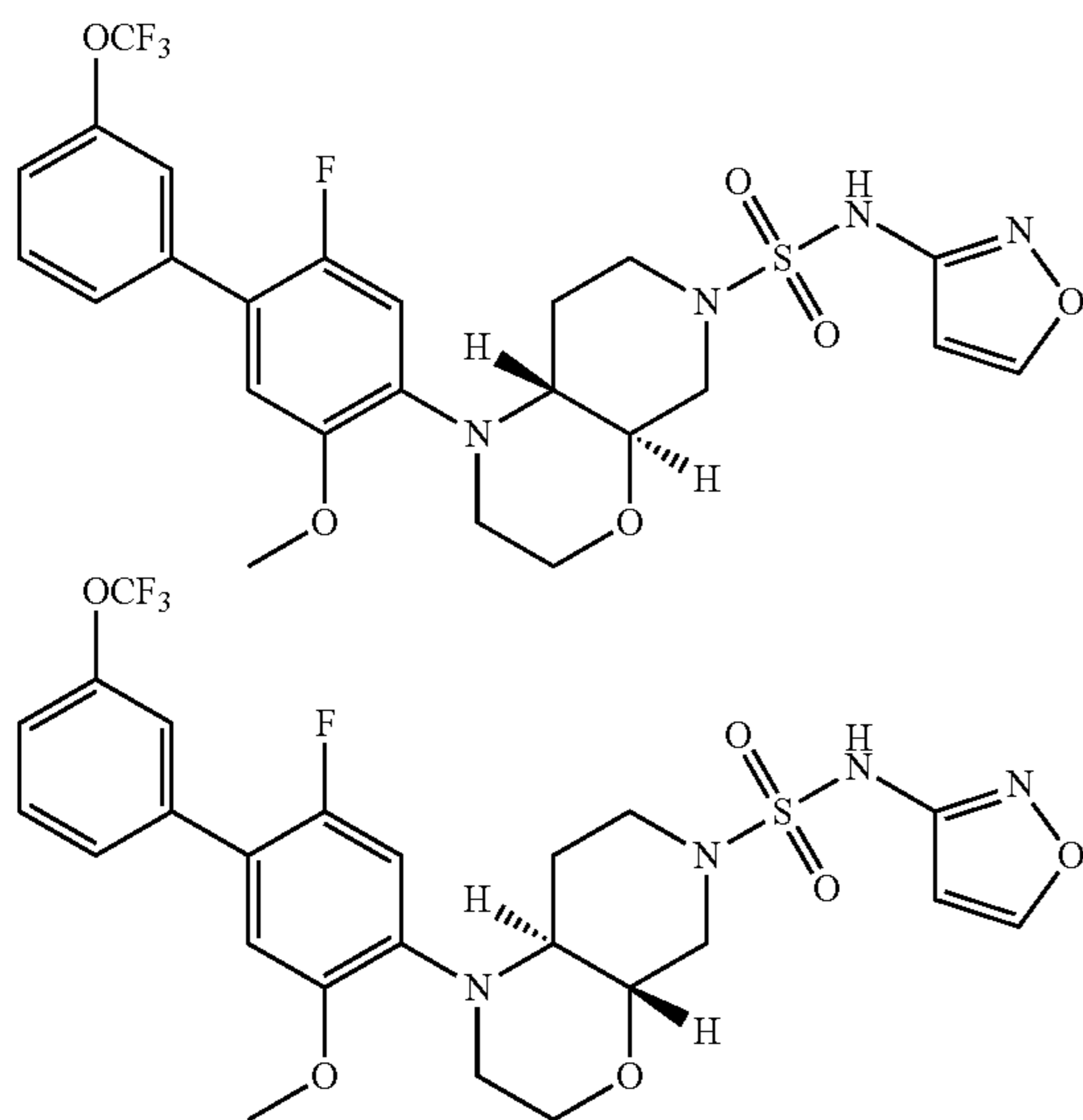
(4aR,8aR)-1-(2-fluoro-5-methoxy-3'-(trifluoromethoxy)-[1,1'-biphenyl]-4-yl)-N-(isoxazol-3-yl)hexahydro-H-pyrido[3,4-b][1,4]oxazine-6(7H)-sulfonamide & (4aS,8aS)-1-(2-fluoro-5-methoxy-3'-(trifluoromethoxy)-[1,1'-biphenyl]-4-yl)-N-(isoxazol-3-yl)hexahydro-1H-pyrido[3,4-b][1,4]oxazine-6(7H)-sulfonamide
