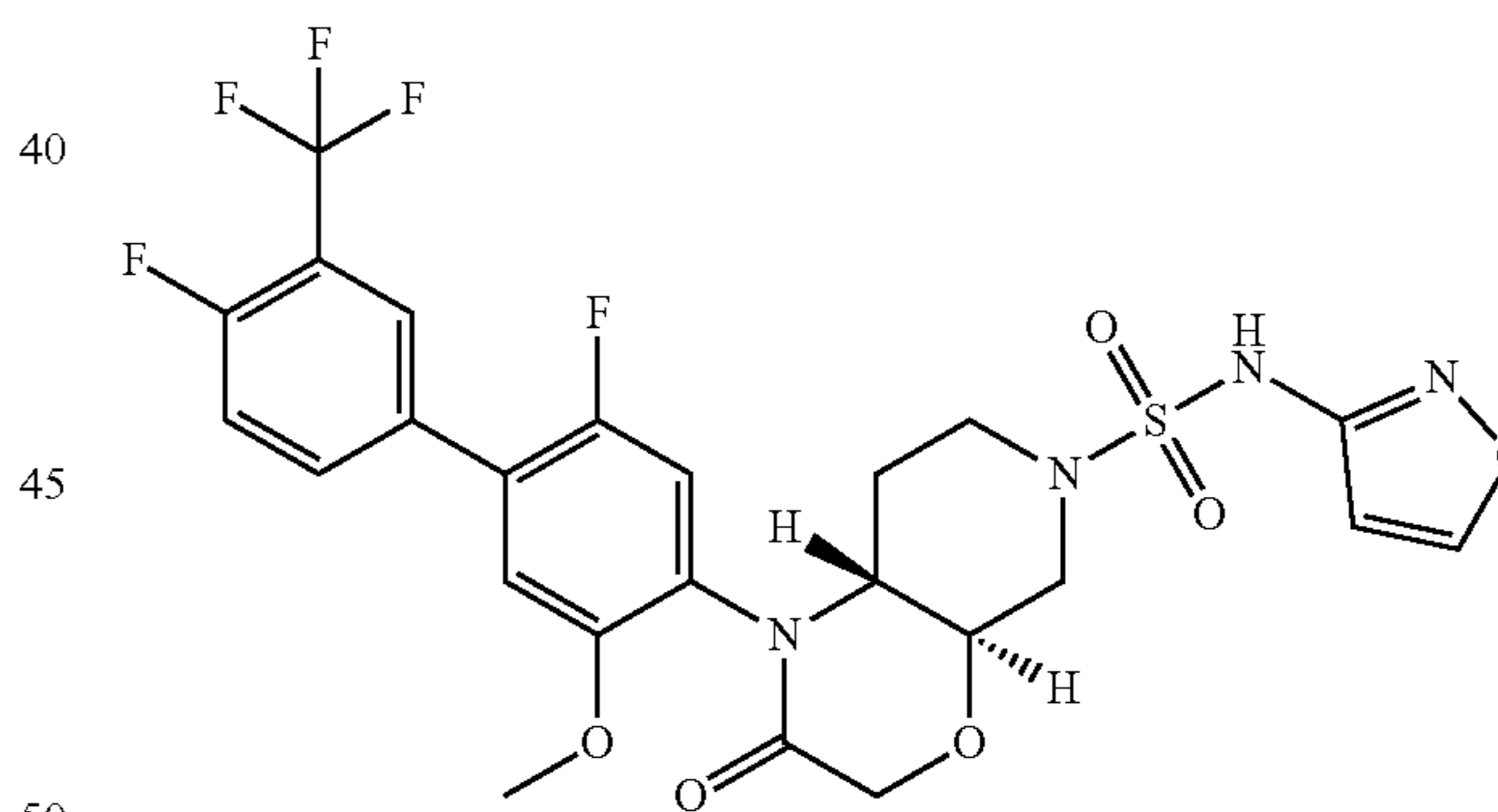
Rac-trans-1-(2,4'-difluoro-5-methoxy-3'-(trifluoromethyl)-[1,1'-biphenyl]-4-yl)-N-(isoxazol-3-yl)-2-oxohexahydro-1H-pyrido[3,4-b][1,4]oxazine-6(7H)-sulfonamide
