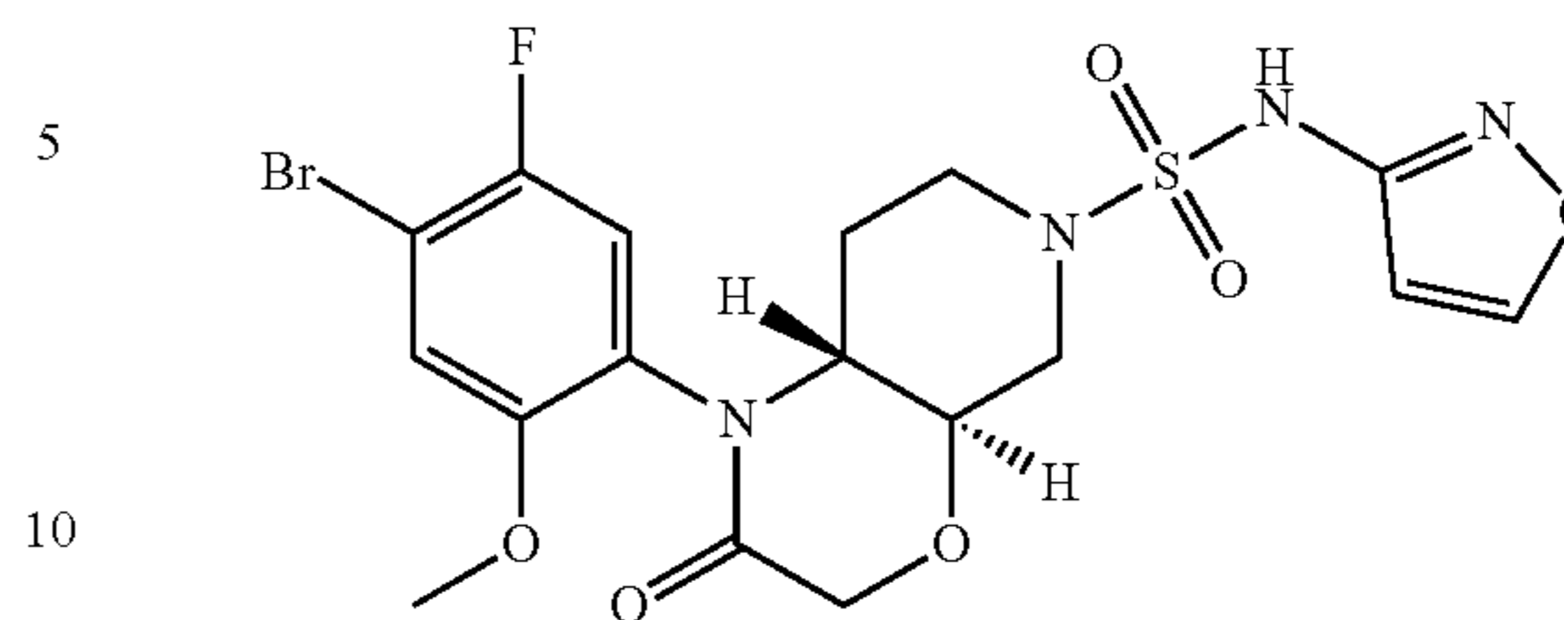
Rac-trans-1-(3'-bromo-2-fluoro-5-methoxy-[1,1'-biphenyl]-4-yl)-N-(isoxazol-3-yl)-2-oxohexahydro-1H-pyrido[3,4-b][1,4]oxazine-6(7H)-sulfonamide
