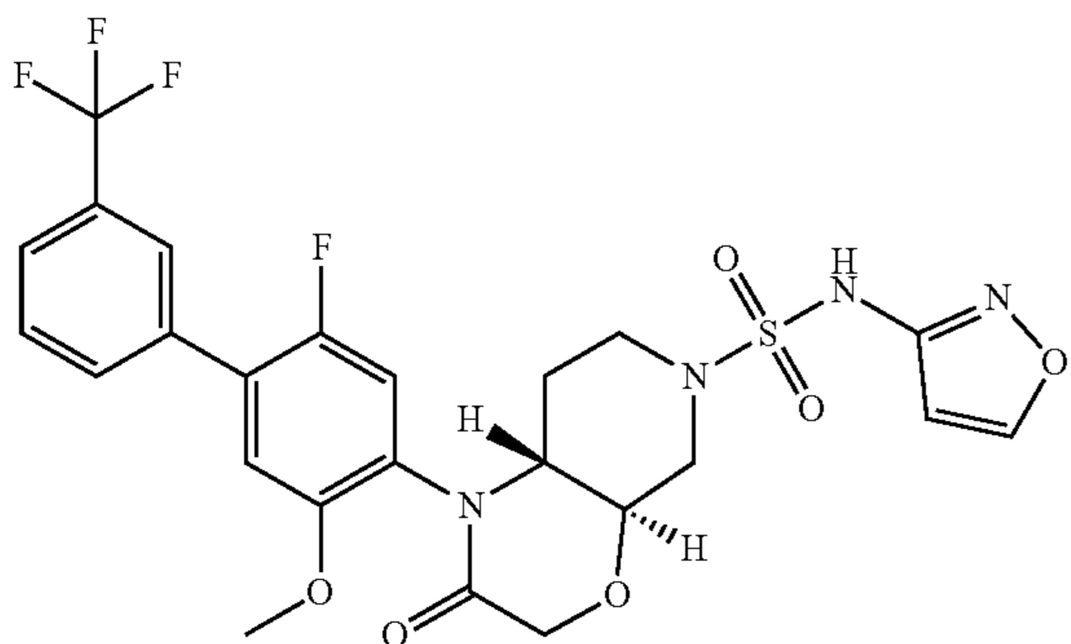
(4aR,8aR)-1-(2-fluoro-5-methoxy-3'-(trifluoromethyl)-[1,1'-biphenyl]-4-yl)-N-(isoxazol-3-yl)-2-oxohexahydro-1H-pyrido[3,4-b][1,4]oxazine-6(7H)-sulfonamide & (4aS,8aS)-1-(2-fluoro-5-methoxy-3'-(trifluoromethyl)-[1,1'-biphenyl]-4-yl)-N-(isoxazol-3-yl)-2-oxohexahydro-1H-pyrido[3,4-b][1,4]oxazine-6(7H)-sulfonamide
