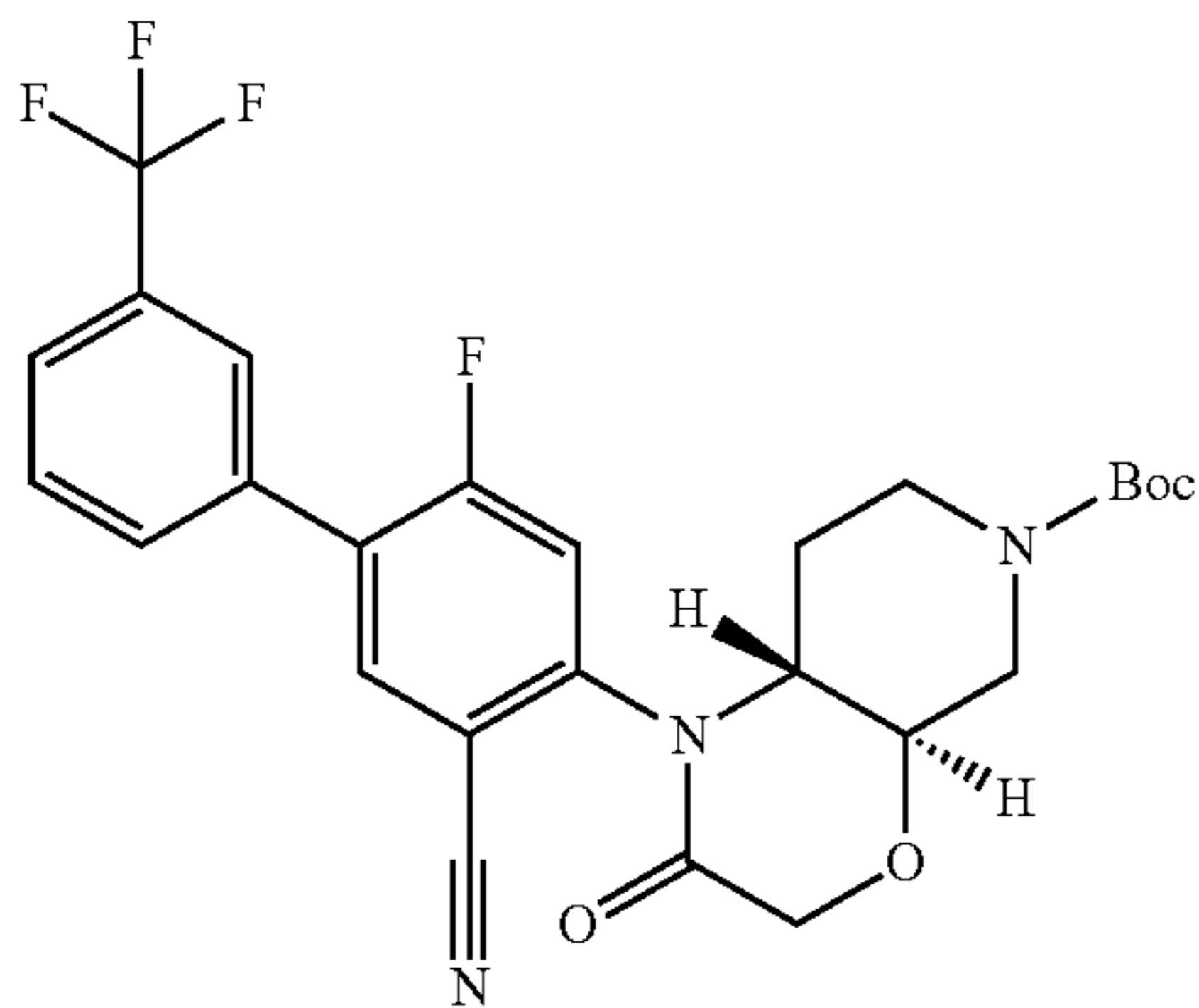
Rac-trans-tert-butyl 1-(5-cyano-2-fluoro-3'-(trifluoromethyl)-[1,1'-biphenyl]-4-yl)-2-oxohexahydro-1H-pyrido[3,4-b][1,4]oxazine-6(7H)-carboxylate
