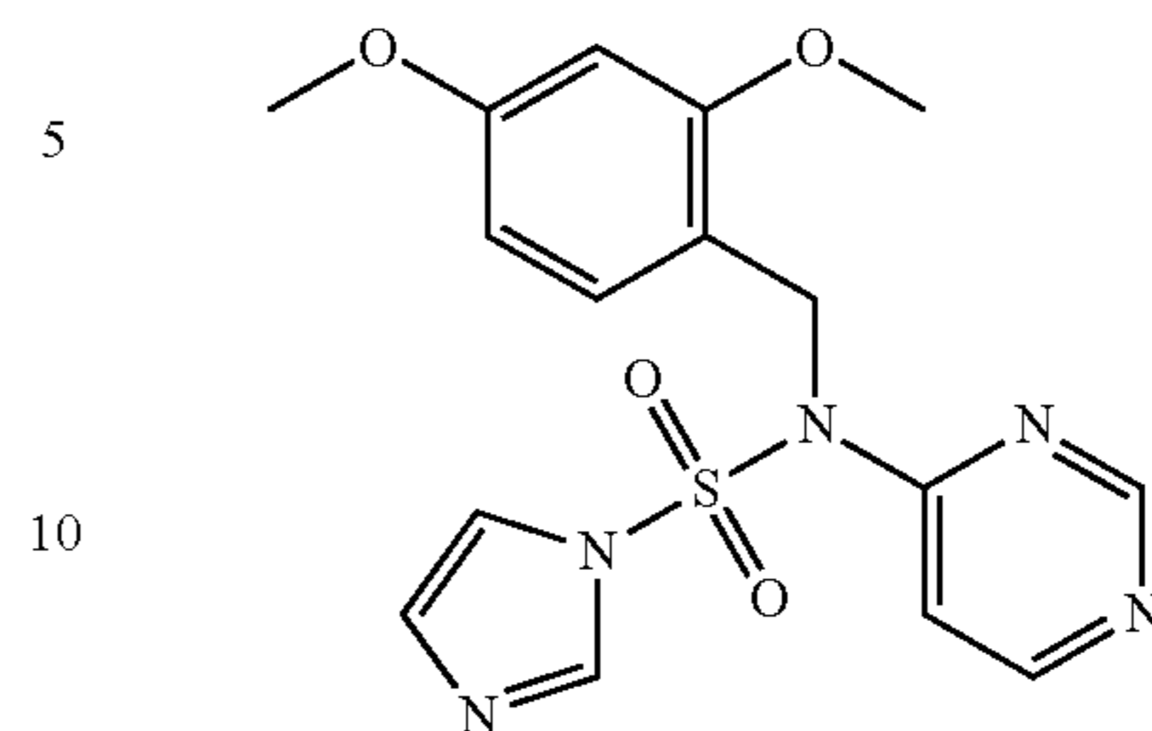
N-(2,4-dimethoxybenzyl)-N-(pyrimidin-4-yl)-1H-imidazole-1-sulfonamide
