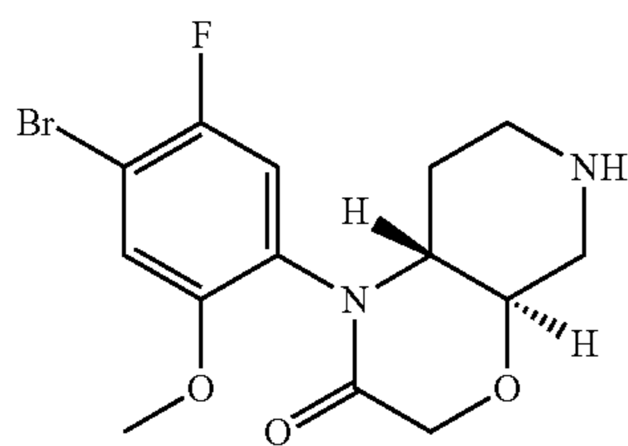
Rac-trans-1-(4-bromo-5-fluoro-2-methoxyphenyl)hexahydro-1H-pyrido[3,4-b][1,4]oxazin-2(3H)-one
