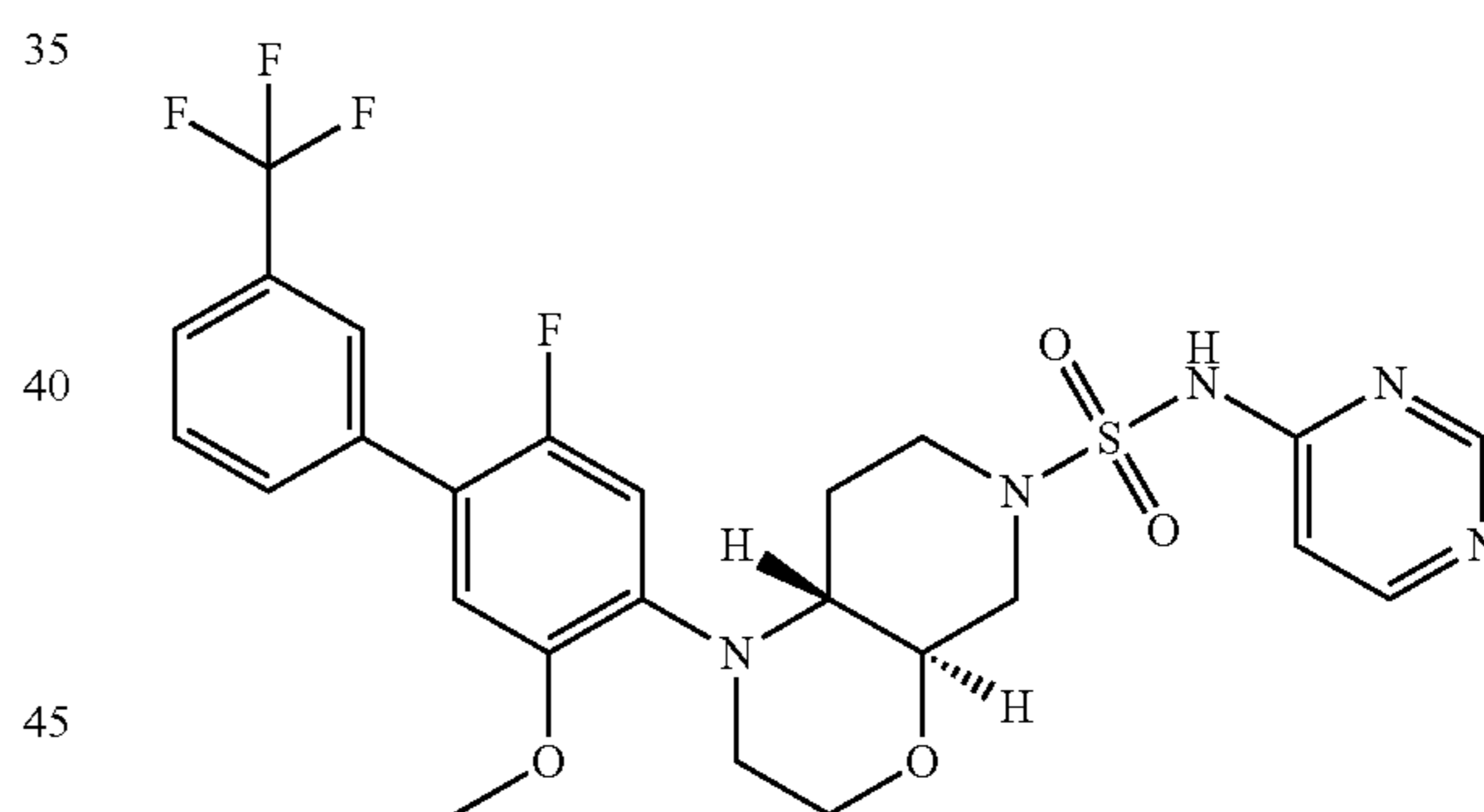
Rac-trans-1-(2-fluoro-5-methoxy-3'-(trifluoromethyl)-[1,1'-biphenyl]-4-yl)-N-(pyrimidin-4-yl)hexahydro-1H-pyrido[3,4-b][1,4]oxazine-6(7H)-sulfonamide
