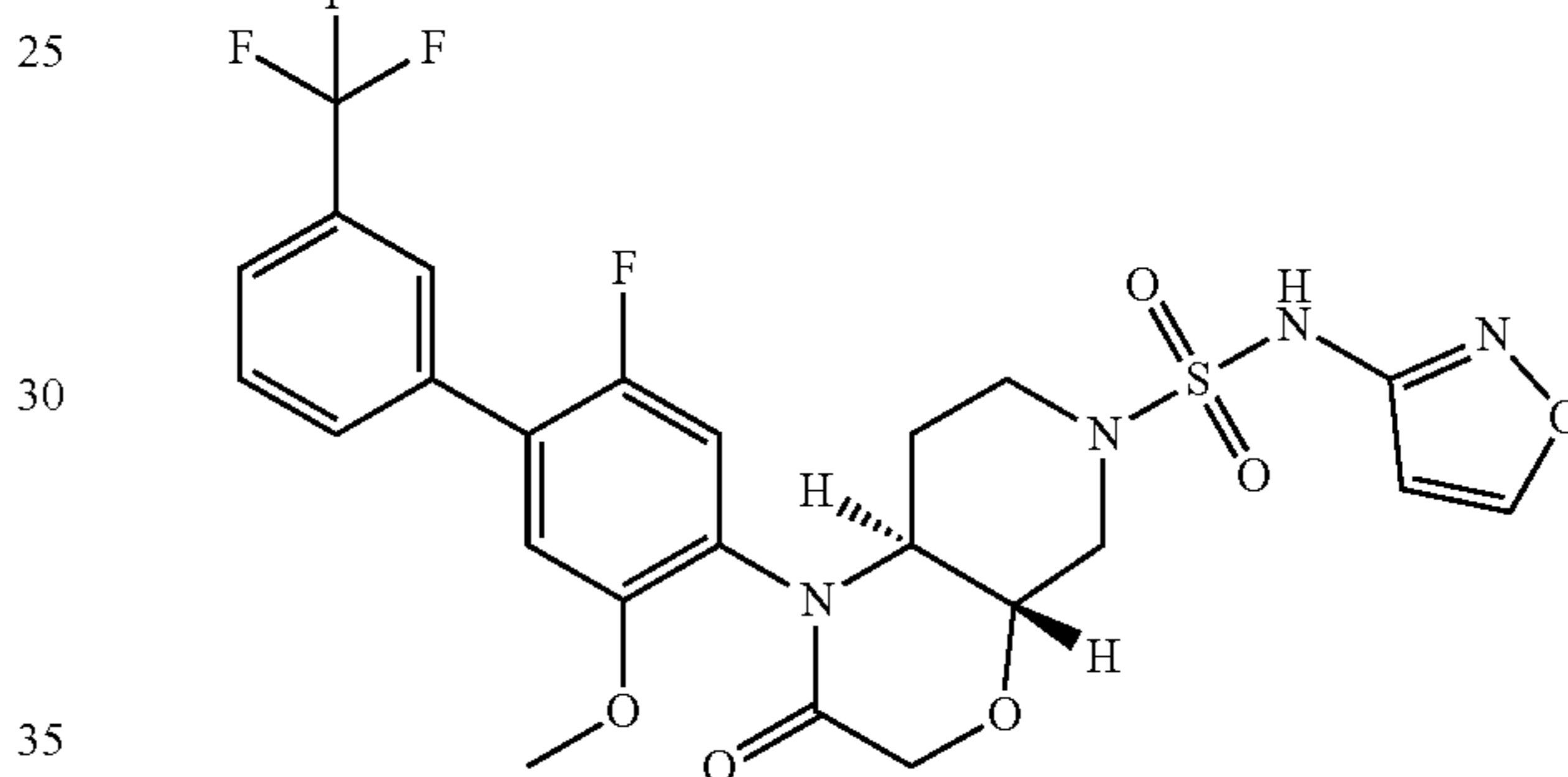
(4aR,8aR)-1-(2-fluoro-5-methoxy-3'-(trifluoromethyl)-[1,1'-biphenyl]-4-yl)-N-(isoxazol-3-yl)-2-oxohexahydro-1H-pyrido[3,4-b][1,4]oxazine-6(7H)-sulfonamide & (4aS,8aS)-1-(2-fluoro-5-methoxy-3'-(trifluoromethyl)-[1,1'-biphenyl]-4-yl)-N-(isoxazol-3-yl)-2-oxohexahydro-1H-pyrido[3,4-b][1,4]oxazine-6(7H)-sulfonamide
