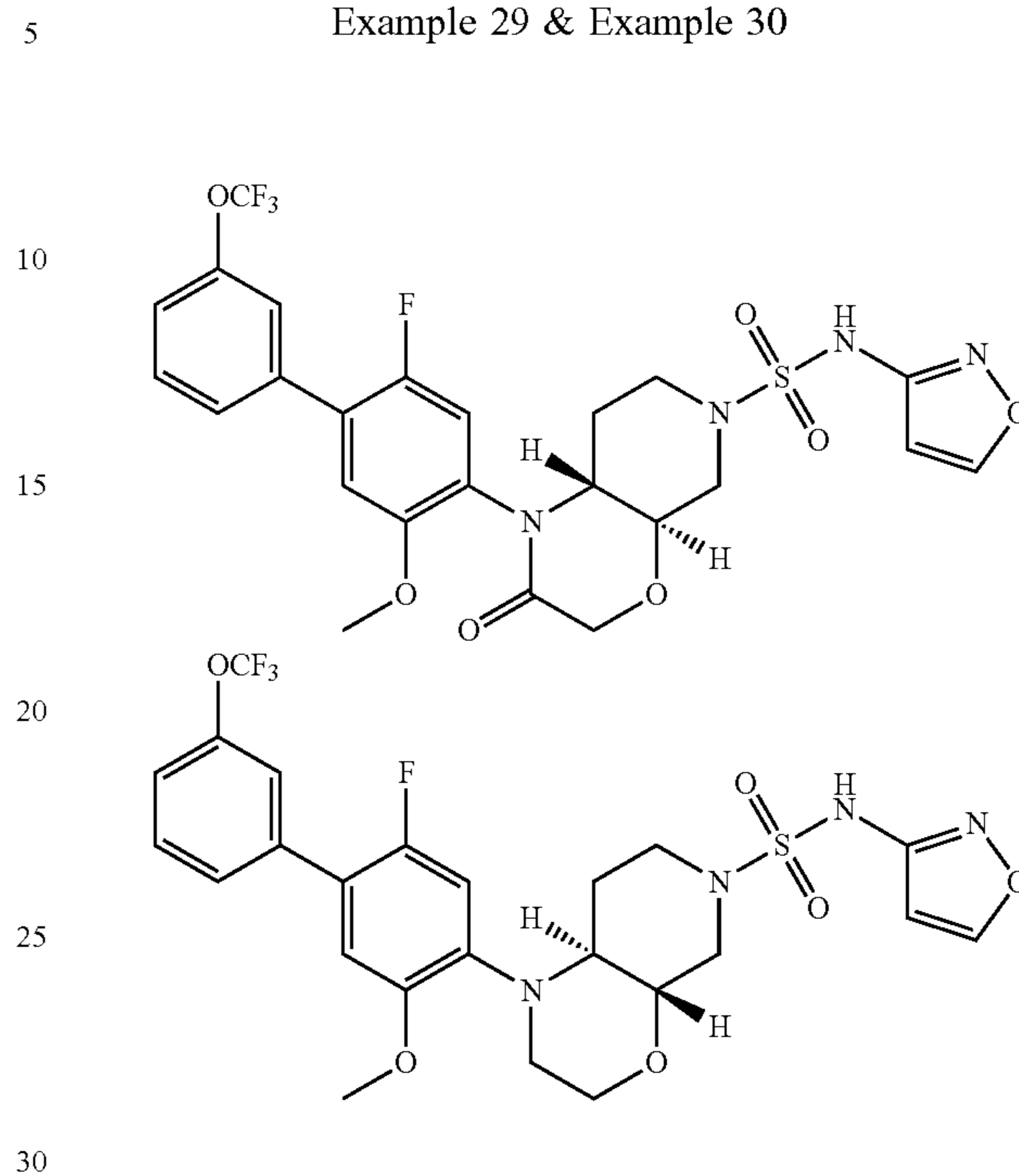
(4aR,8aR)-1-(2-fluoro-5-methoxy-3'-(trifluoromethoxy)-[1,1'-biphenyl]-4-yl)-N-(isoxazol-3-yl)-2-oxohexahydro-1H-pyrido[3,4-b][1,4]oxazine-6(7H)-sulfonamide & (4aS,8aS)-1-(2-fluoro-5-methoxy-3'-(trifluoromethoxy)-[1,1'-biphenyl]-4-yl)-N-(isoxazol-3-yl)-2-oxohexahydro-1H-pyrido[3,4-b][1,4]oxazine-6(7H)-sulfonamide
