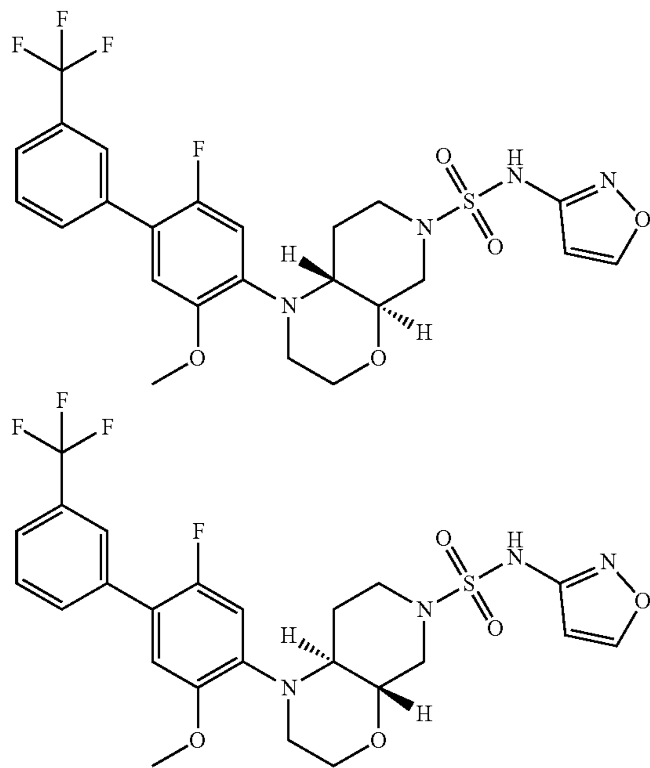
(4aR,8aR)-1-(2-fluoro-5-methoxy-3'-(trifluoromethyl)-[1,1'-biphenyl]-4-yl)-N-(isoxazol-3-yl)hexahydro-1H-pyrido[3,4-b][1,4]oxazine-6(7H)-sulfonamide & (4aS,8aS)-1-(2-fluoro-5-methoxy-3'-(trifluoromethyl)-[1,1'-biphenyl]-4-yl)-N-(isoxazol-3-yl)hexahydro-1H-pyrido[3,4-b][1,4]oxazine-6(7H)-sulfonamide
