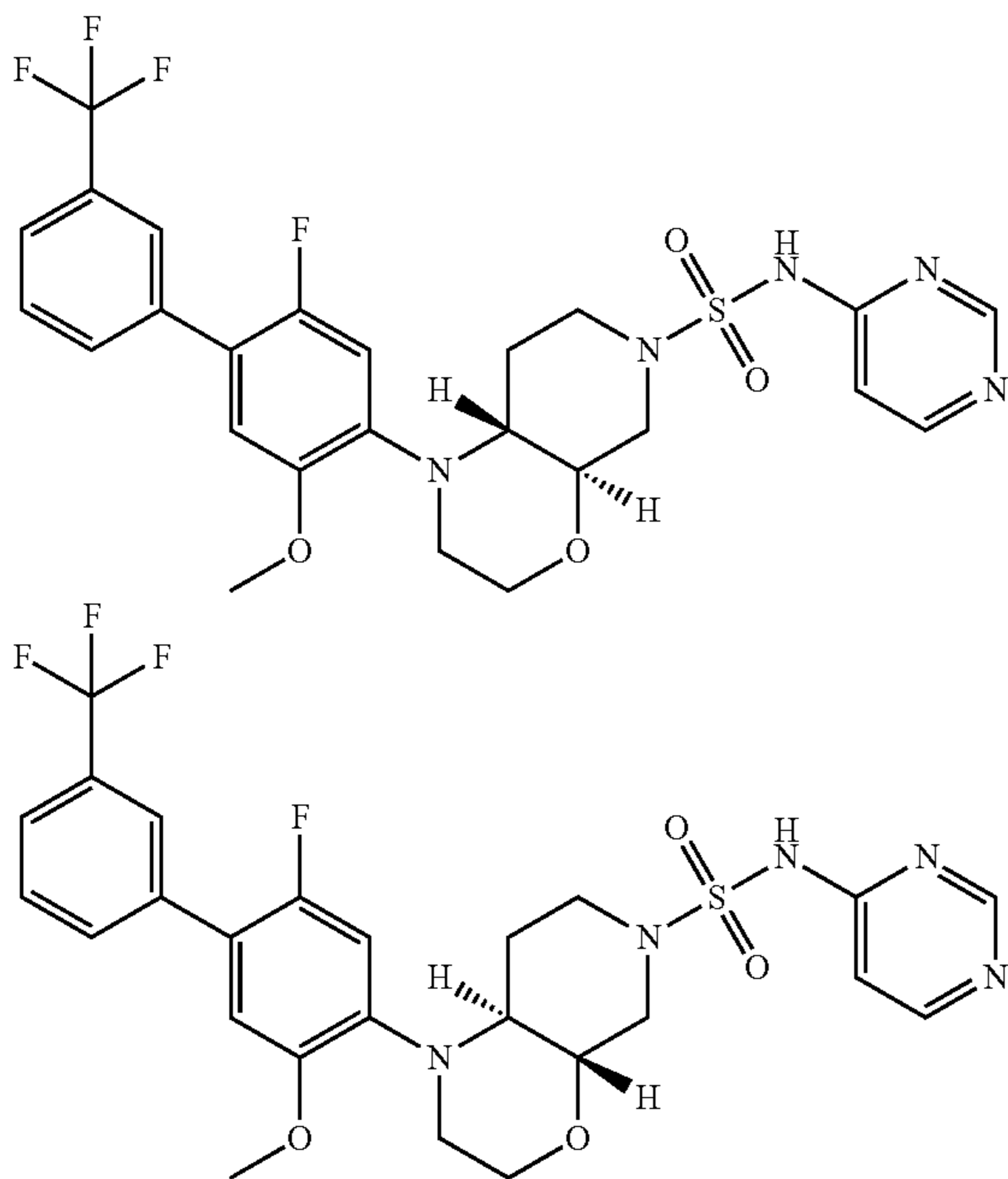
(4aR,8aR)-1-(2-fluoro-5-methoxy-3'-(trifluoromethyl)-[1,1'-biphenyl]-4-yl)-N-(pyrimidin-4-yl)hexahydro-1H-pyrido[3,4-b][1,4]oxazine-6(7H)-sulfonamide & (4aS,8aS)-1-(2-fluoro-5-methoxy-3'-(trifluoromethyl)-[1,1'-biphenyl]-4-yl)-N-(pyrimidin-4-yl)hexahydro-1H-pyrido[3,4-b][1,4]oxazine-6(7H)-sulfonamide
