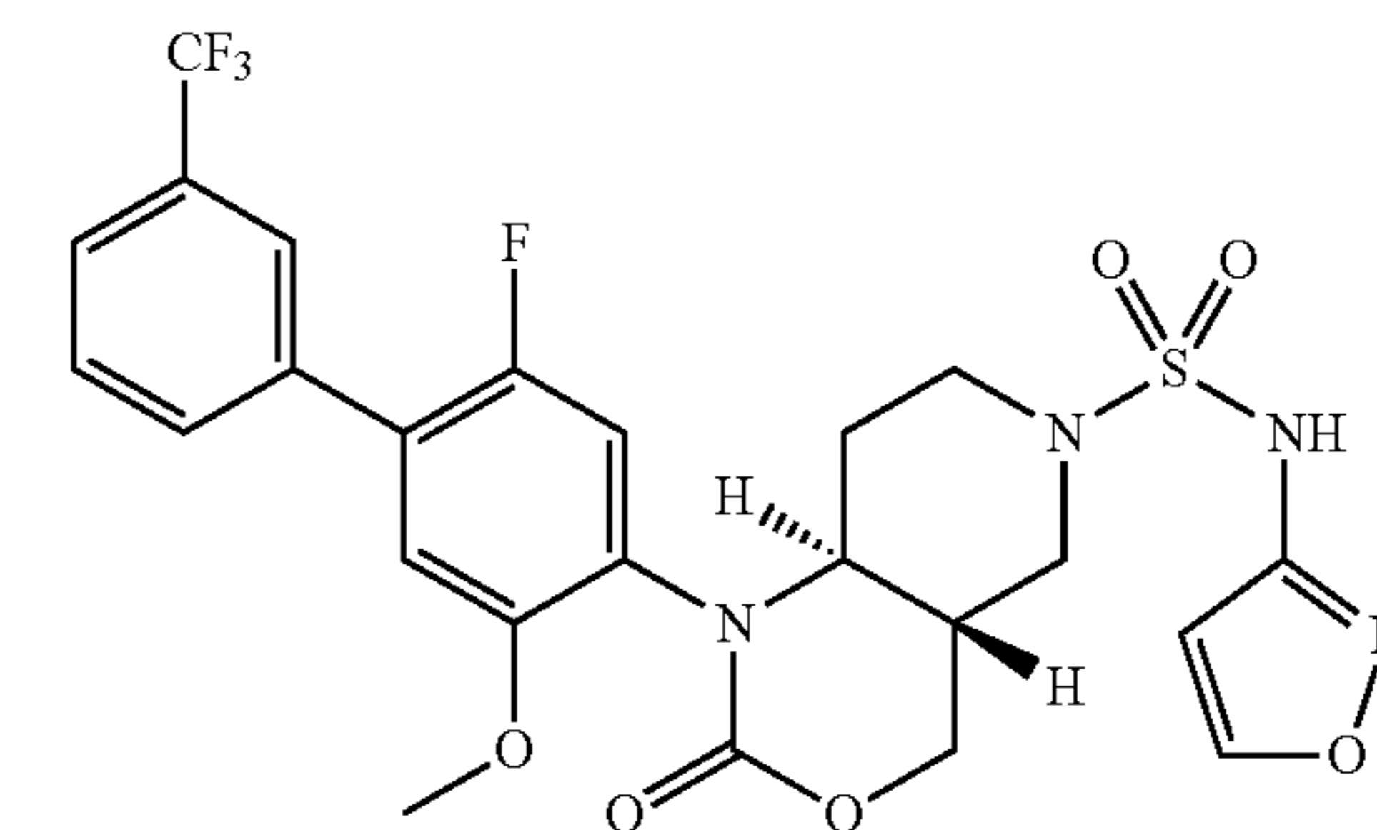
(4aR,8aR)-1-(2-fluoro-5-methoxy-3'-(trifluoromethyl)-[1,1'-biphenyl]-4-yl)-N-(isoxazol-3-yl)-2-oxohexahydro-2H-pyrido[4,3-d][1,3]oxazine-6(4H)-sulfonamide & (4aS,8aS)-1-(2-fluoro-5-methoxy-3'-(trifluoromethyl)-[1,1'-biphenyl]-4-yl)-N-(isoxazol-3-yl)-2-oxohexahydro-2H-pyrido[4,3-d][1,3]oxazine-6(4H)-sulfonamide
