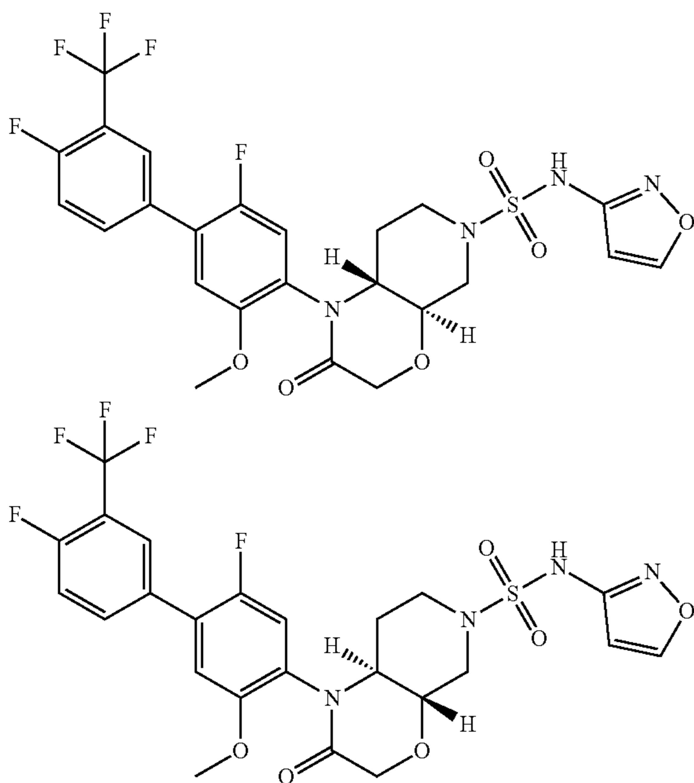
(4aR,8aR)-1-(2,4'-difluoro-5-methoxy-3'-(trifluoromethyl)-[1,1'-biphenyl]-4-yl)-N-(isoxazol-3-yl)-2-oxohexahydro-1H-pyrido[3,4-b][1,4]oxazine-6(7H)-sulfonamide & (4aS,8aS)-1-(2,4'-difluoro-5-methoxy-3'-(trifluoromethyl)-[1,1'-biphenyl]-4-yl)-N-(isoxazol-3-yl)-2-oxohexahydro-1H-pyrido[3,4-b][1,4]oxazine-6(7H)-sulfonamide
