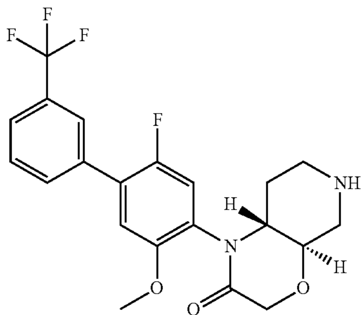
Rac-trans-1-(2-fluoro-5-methoxy-3'-(trifluoromethyl)-[1,1'-biphenyl]-4-yl)hexahydro-1H-pyrido[3,4-b][1,4]oxazin-2(3H)-one
