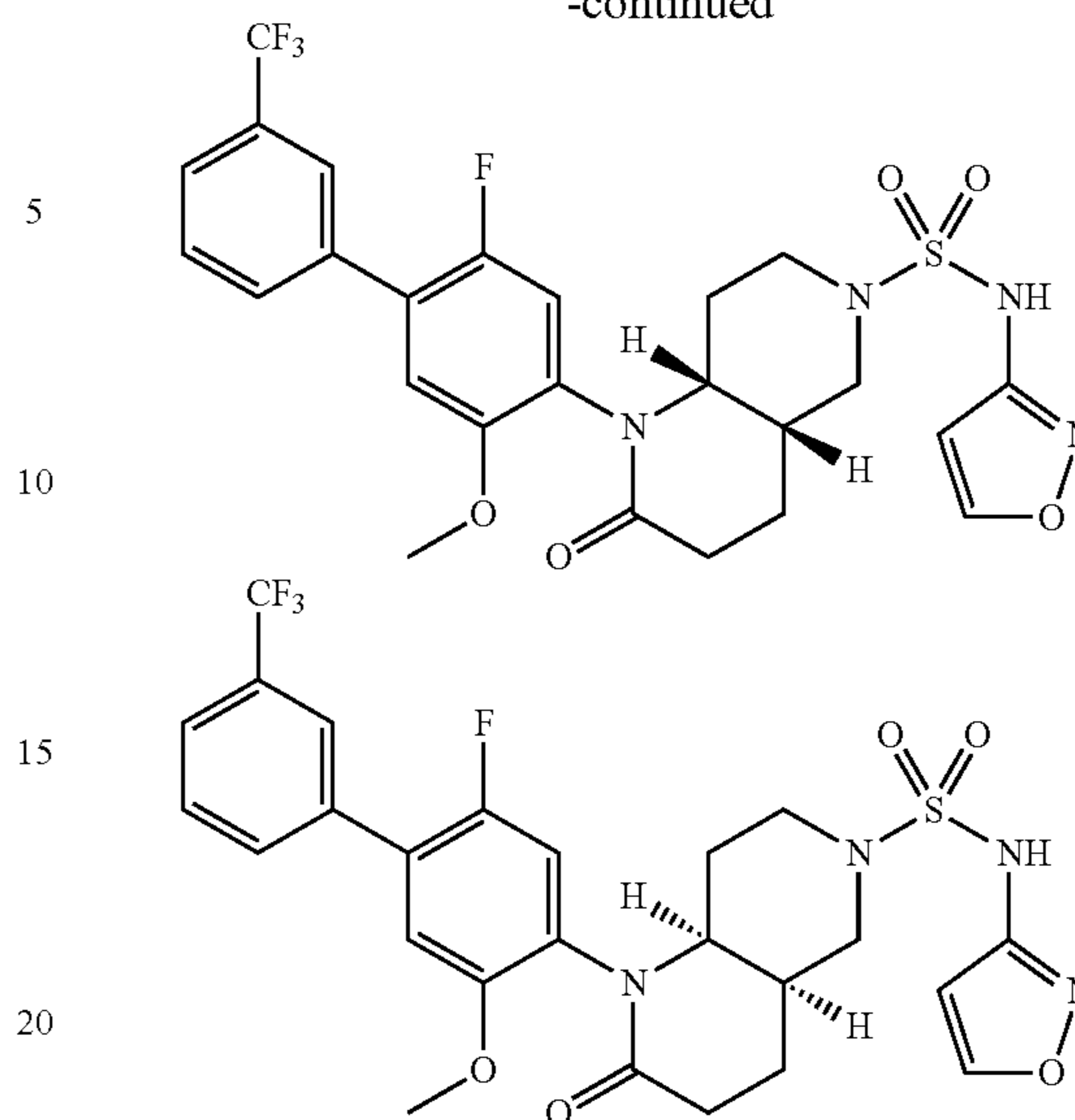
1-[5-fluoro-2-methoxy-4-[3-(trifluoromethyl)phenyl]phenyl]-N-isoxazol-3-yl-2-oxo-4,4a,5,7,8,8a-hexahydro-3H-1,6-naphthyridine-6-sulfonamide
