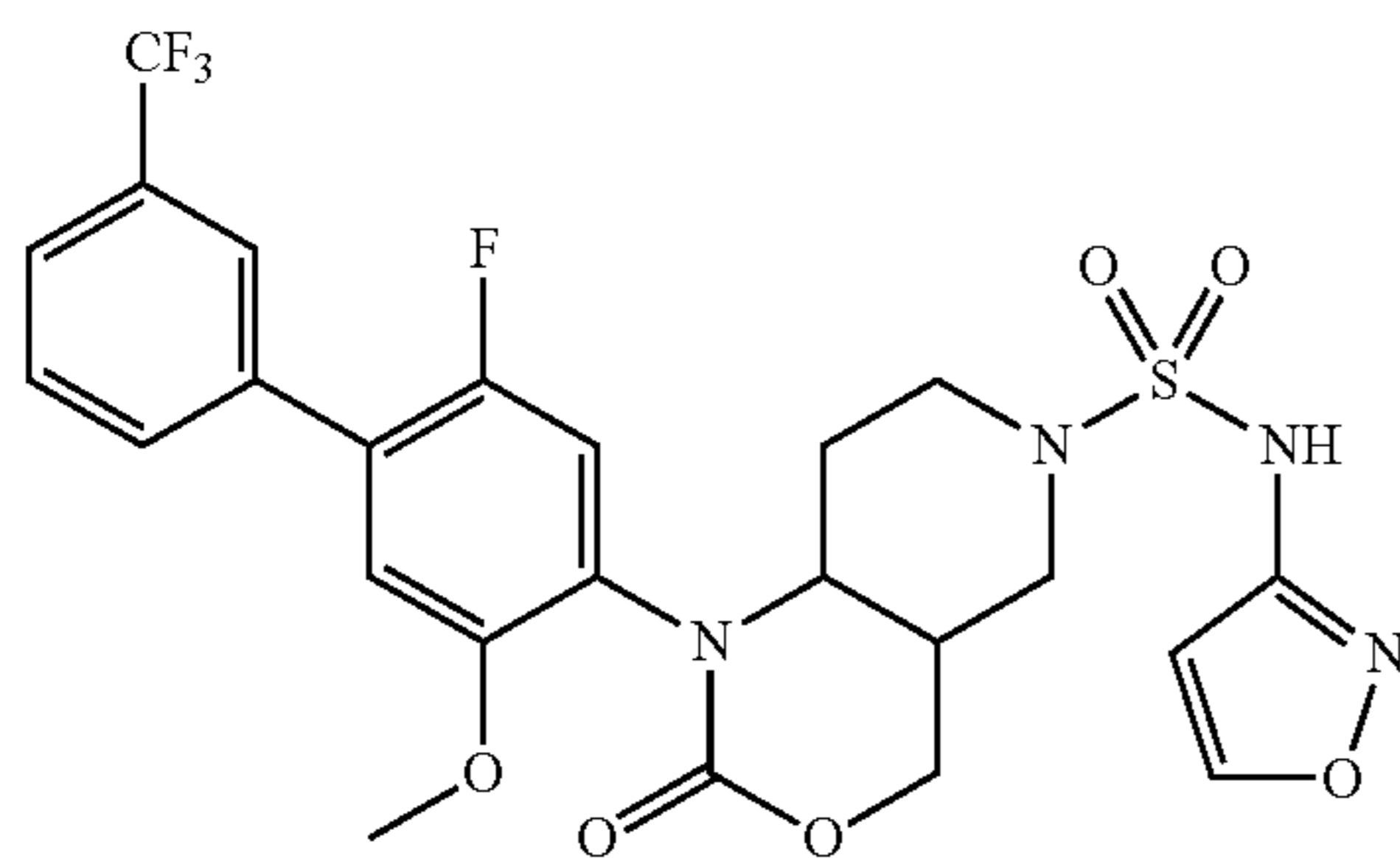
rac-trans-1-(2-fluoro-5-methoxy-3'-(trifluoromethyl)-[1,1'-biphenyl]-4-yl)-N-(isoxazol-3-yl)-2-oxohexahydro-2H-pyrido[4,3-d][1,3]oxazine-6(4H)-sulfonamide
