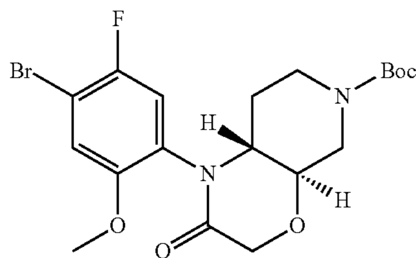
Rac-trans-tert-butyl 1-(4-bromo-5-fluoro-2-methoxyphenyl)-2-oxohexahydro-1H-pyrido[3,4-b][1,4]oxazine-6(7H)-carboxylate
