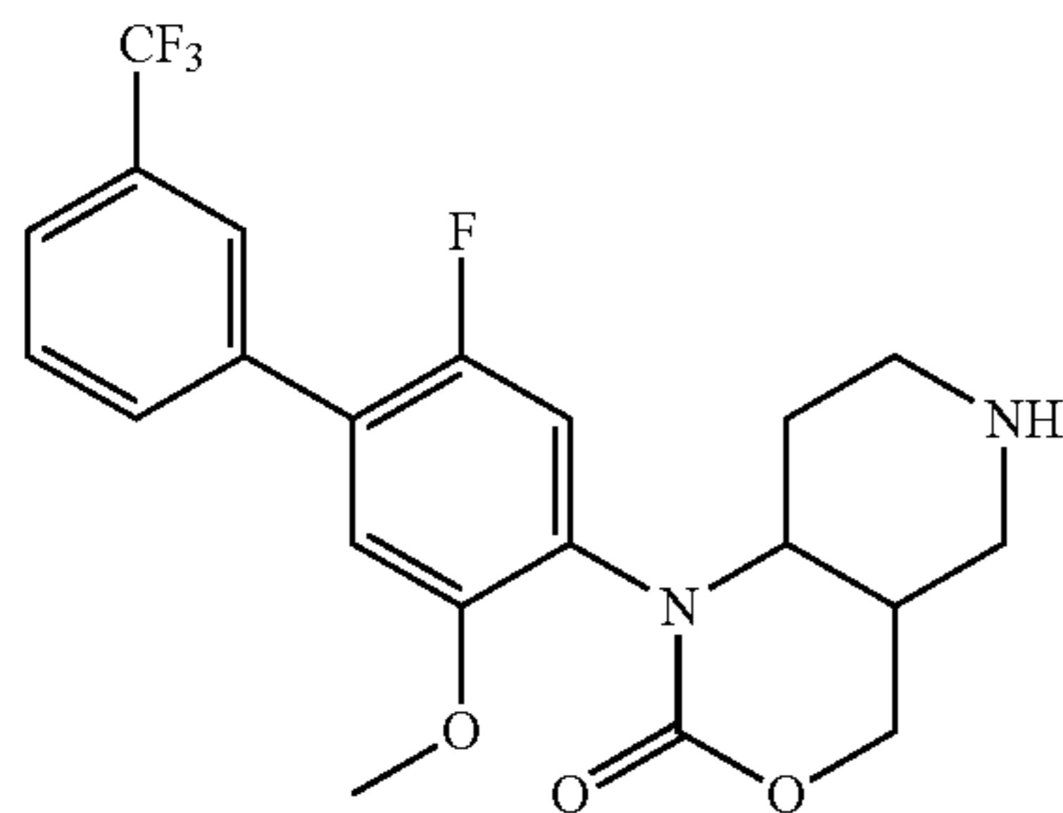
rac-trans-1-[5-fluoro-2-methoxy-4-[3-(trifluoromethyl)phenyl]phenyl]-4a,5,6,7,8,8a-hexahydro-4H-pyrido[4,3-d][1,3]oxazin-2-one
