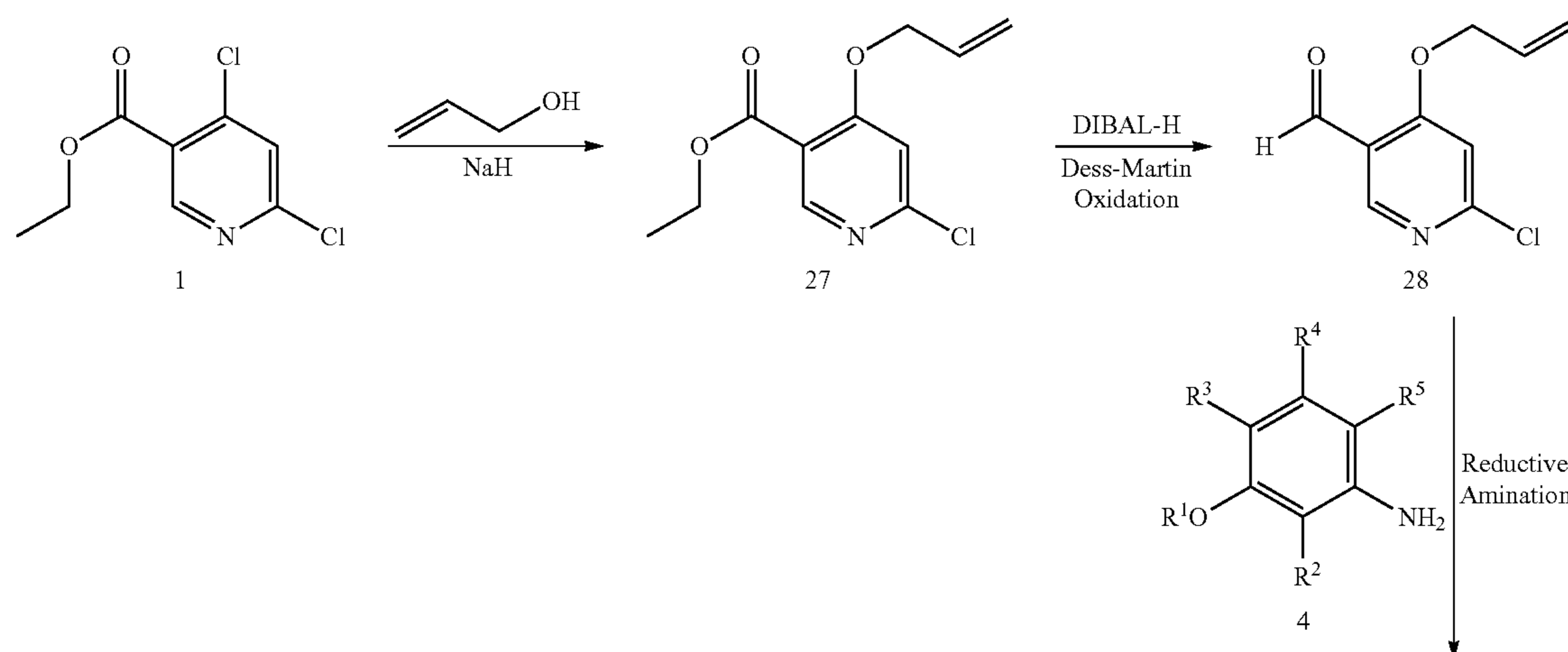
Scheme 6
