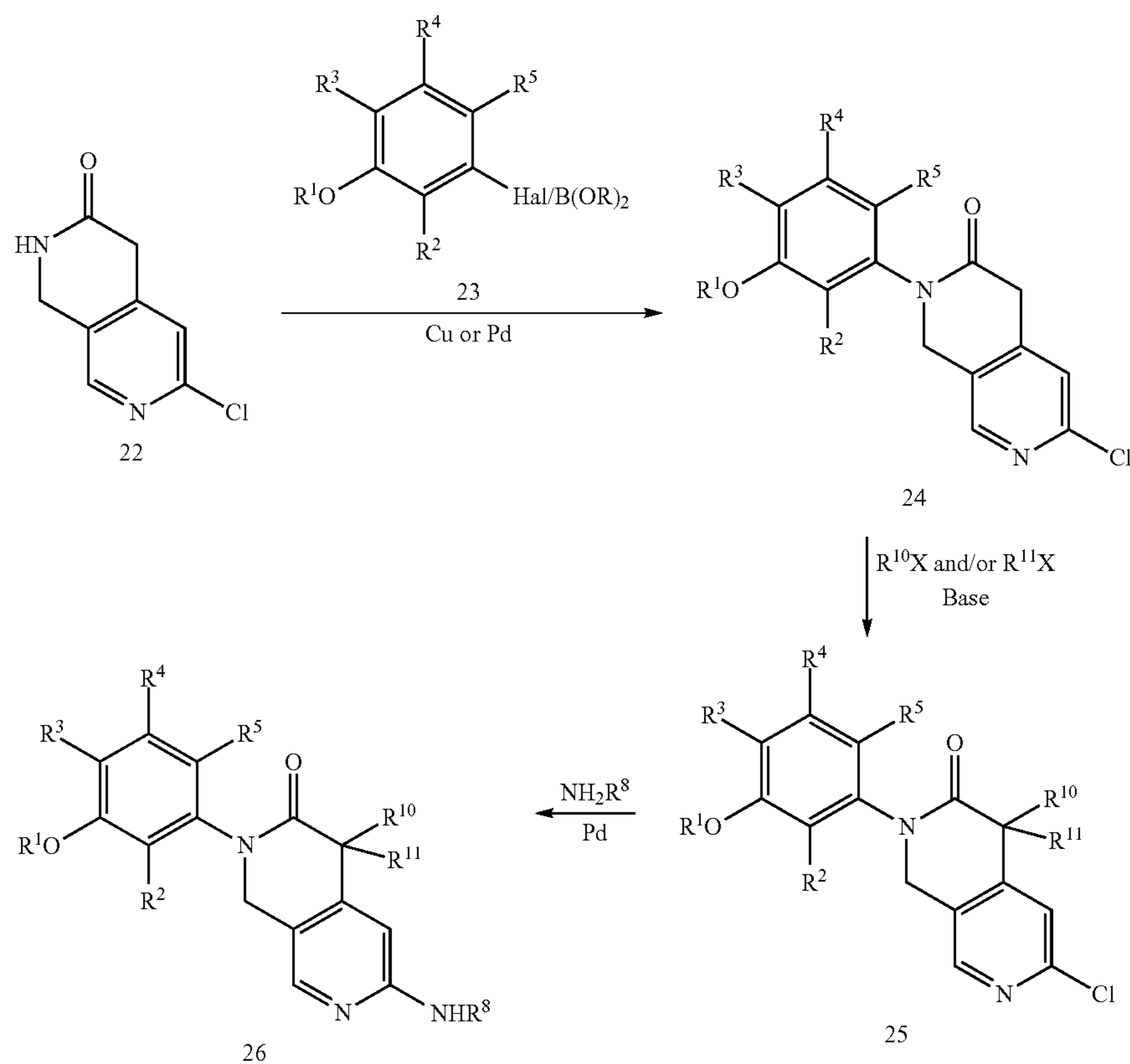
Scheme 5
