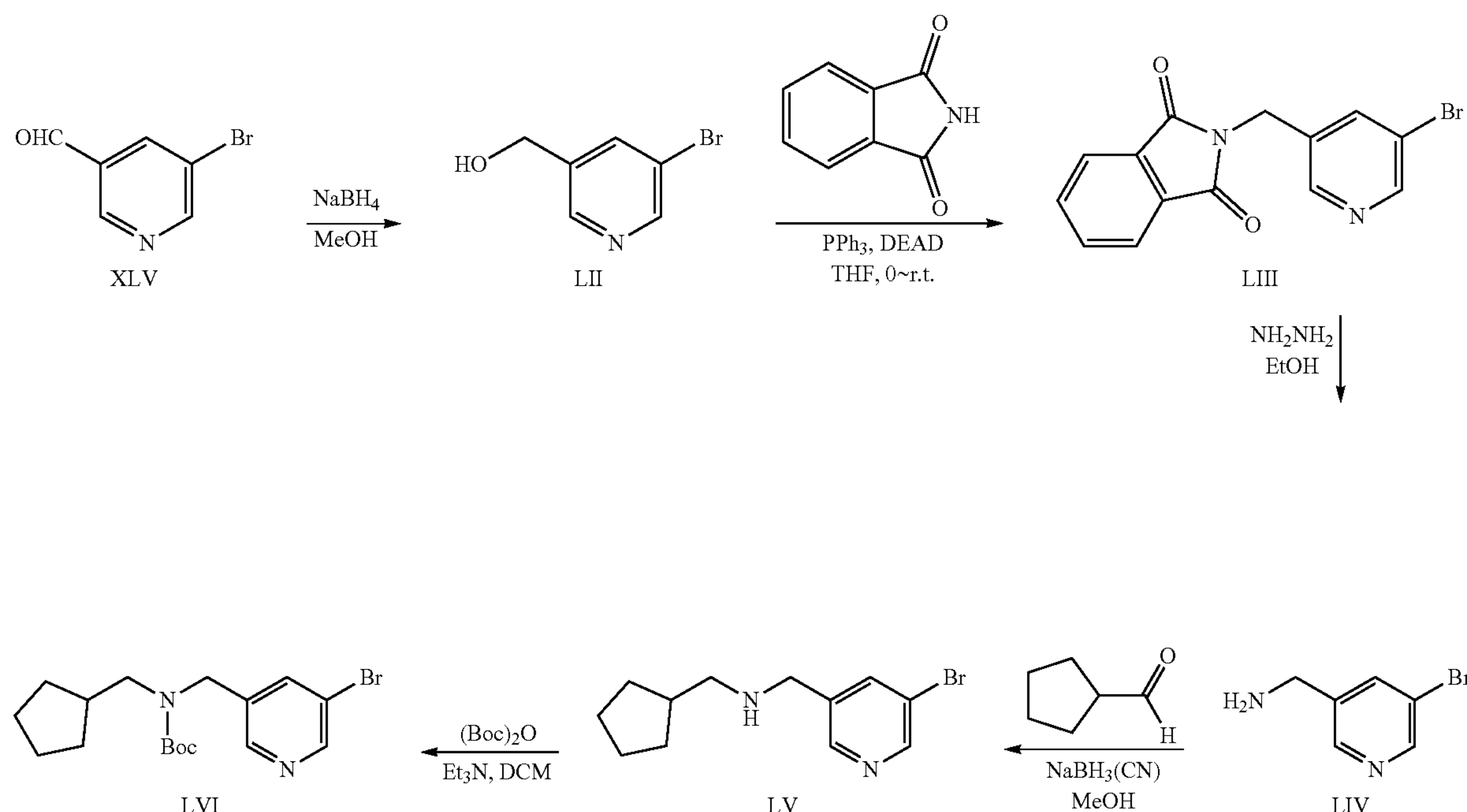
Scheme 11
