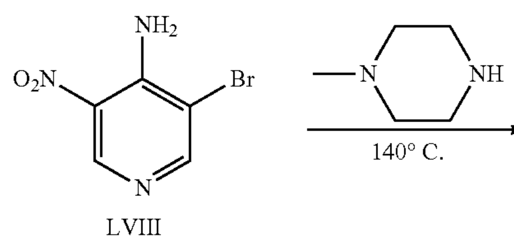
Scheme 13
