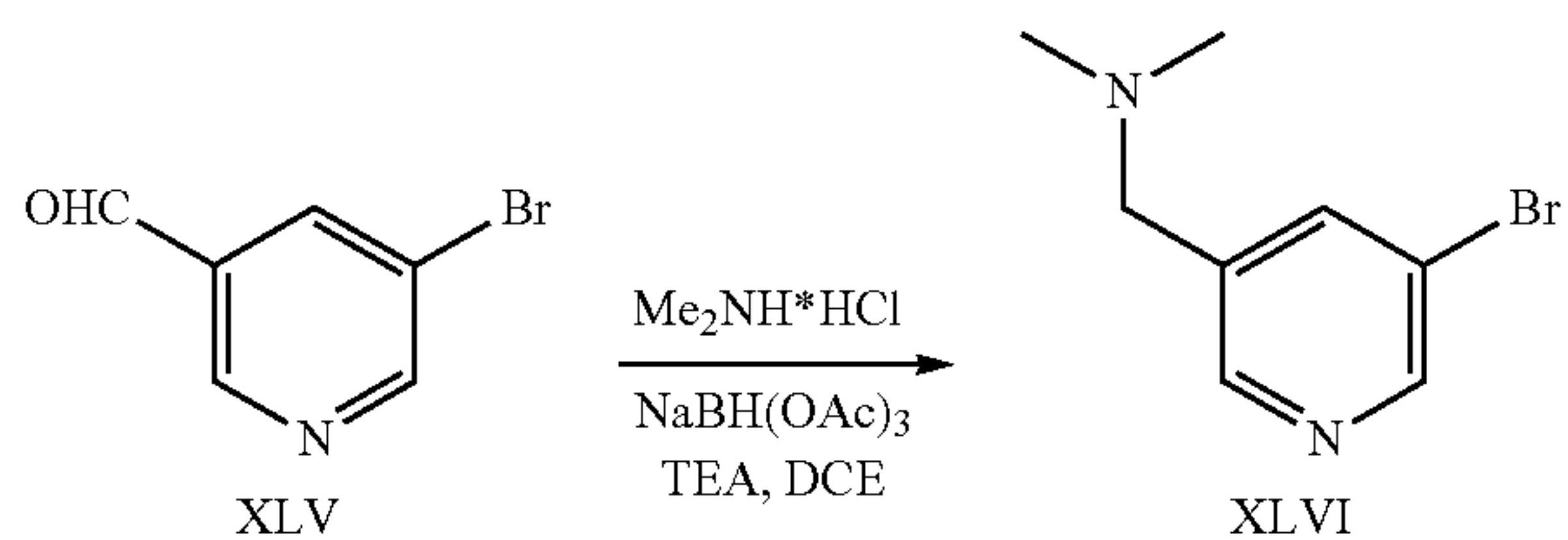
Scheme 10
