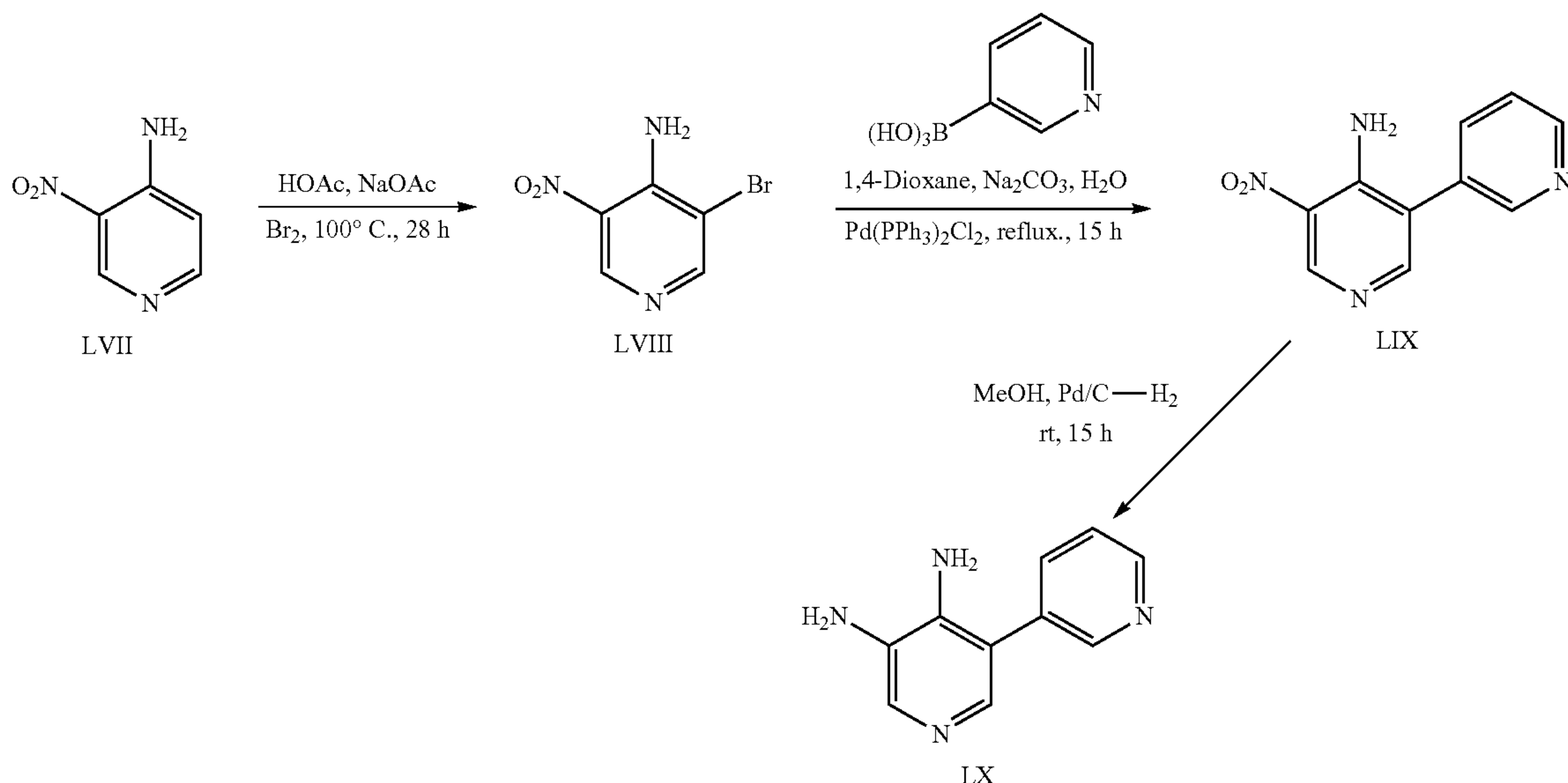
Scheme 12
