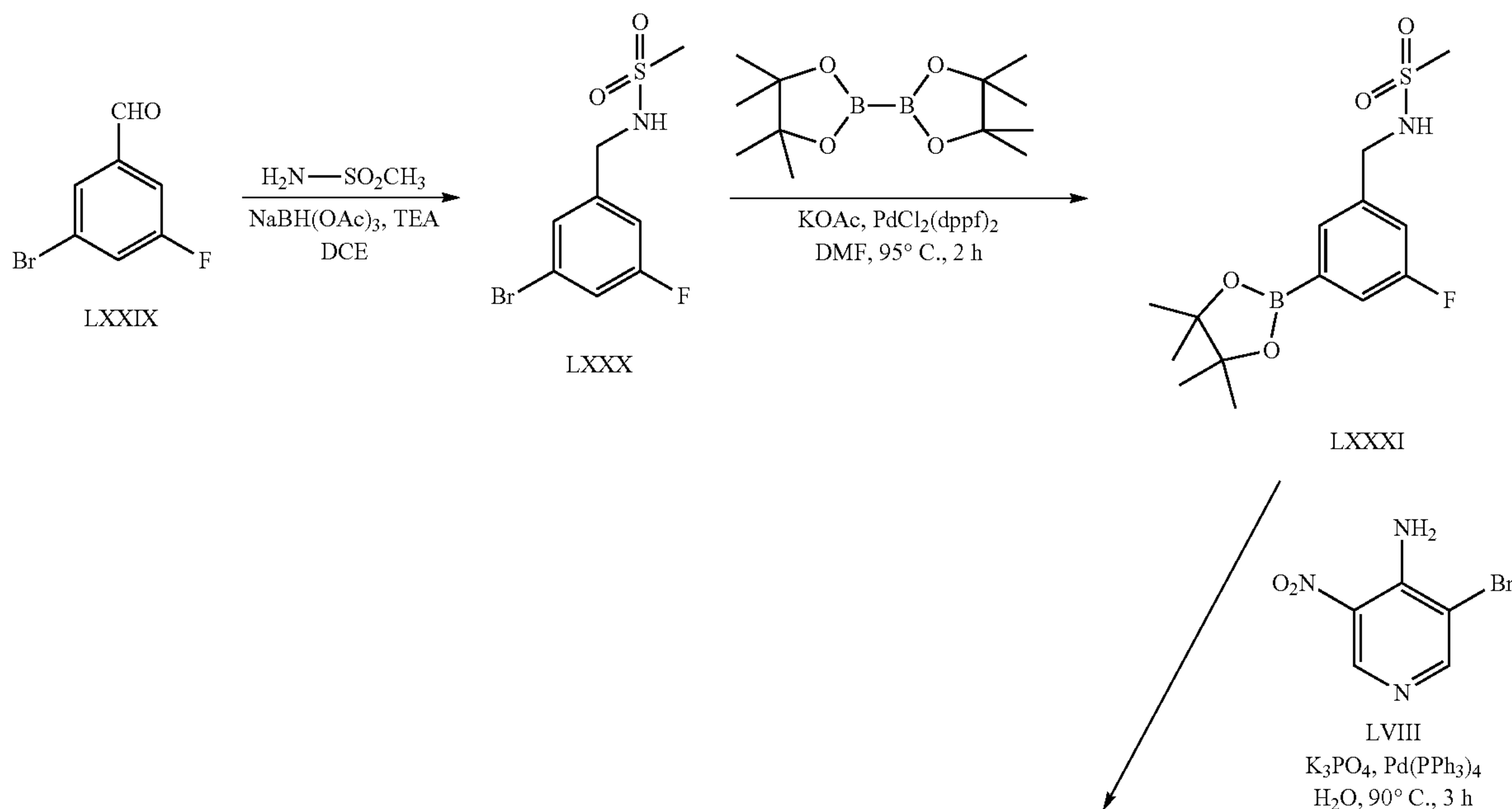
Scheme 15
