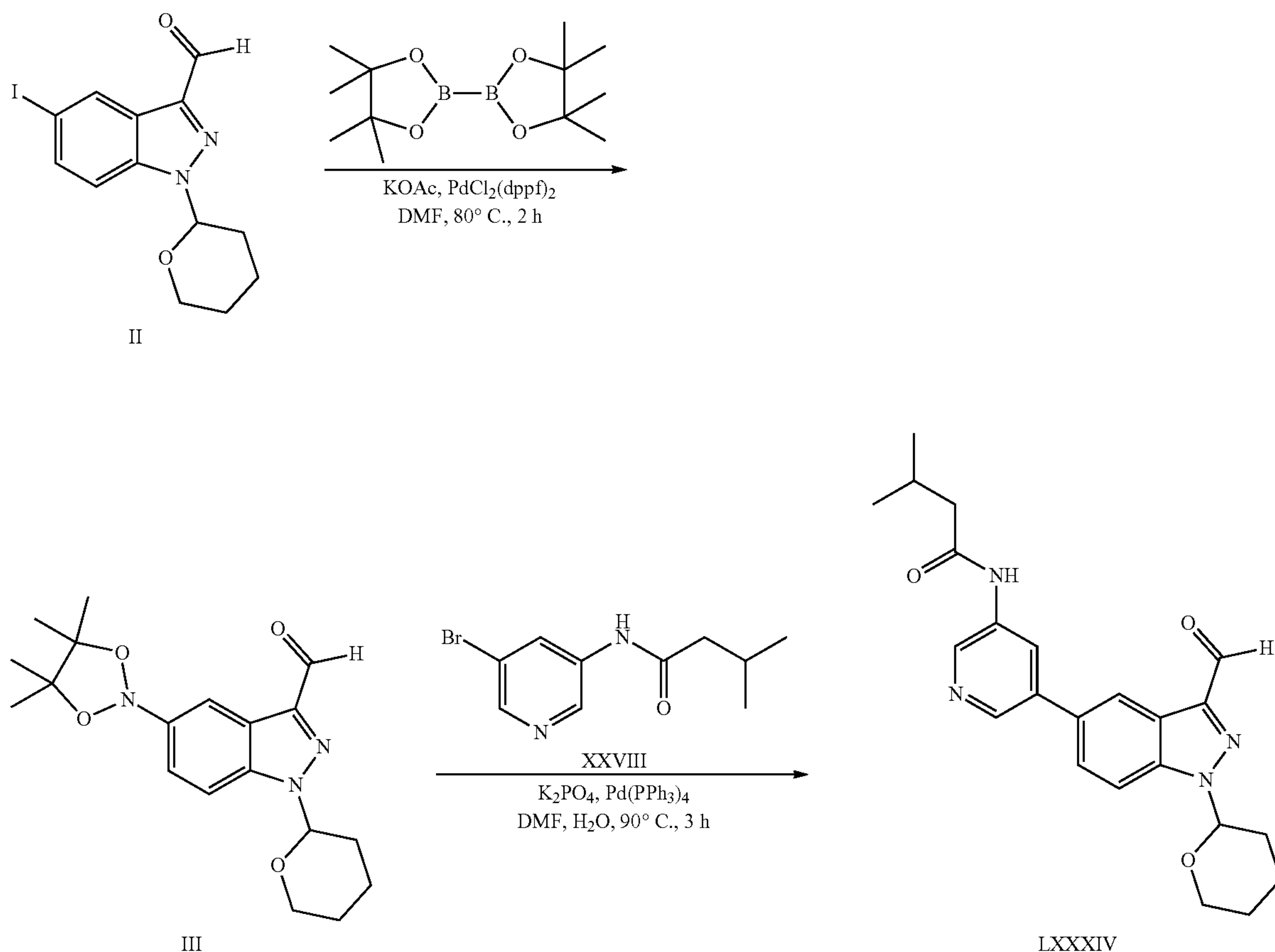
Scheme 16
