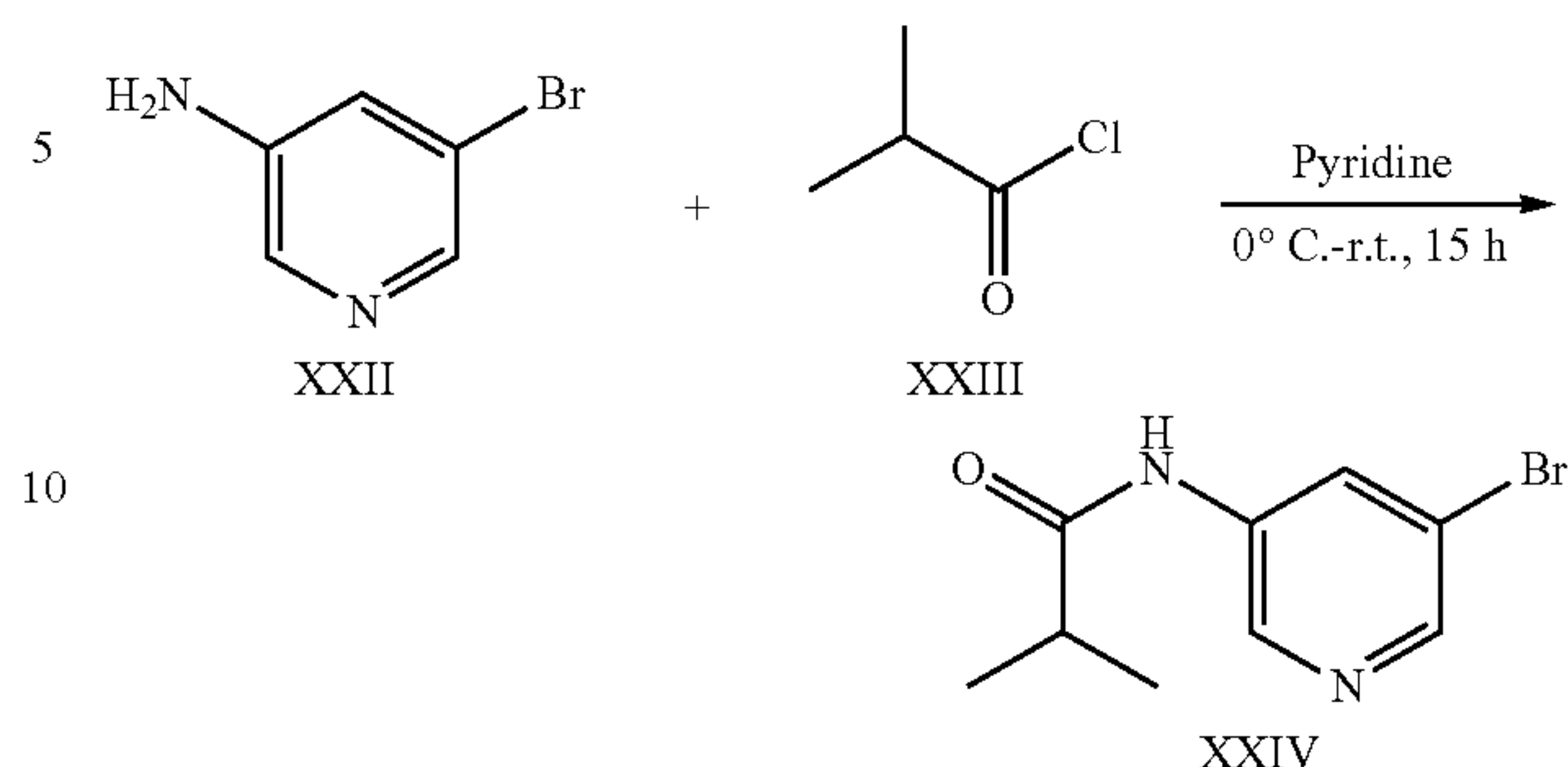
Scheme 6
