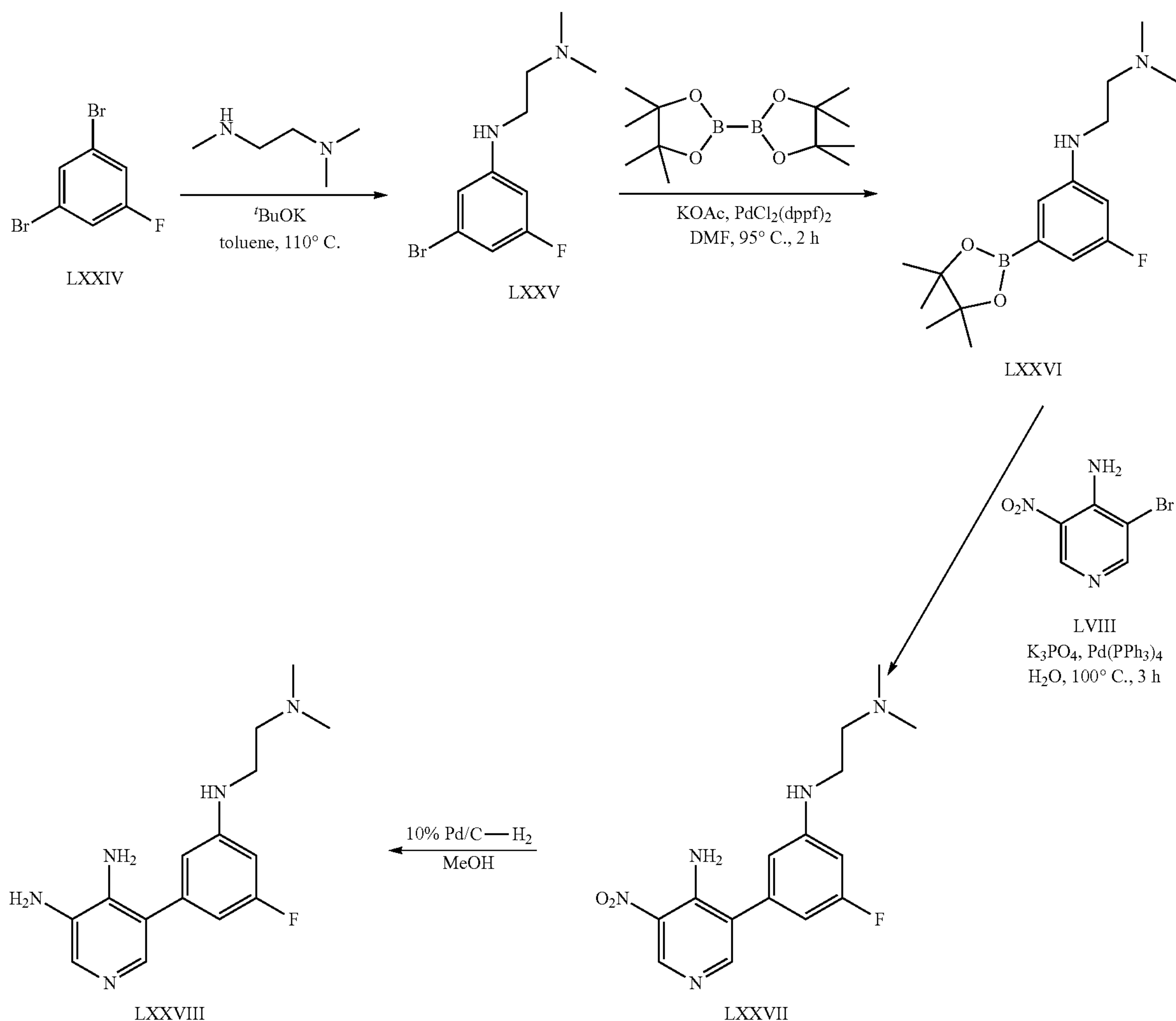
Scheme 14
