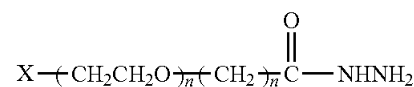
Hydrazide PEG
