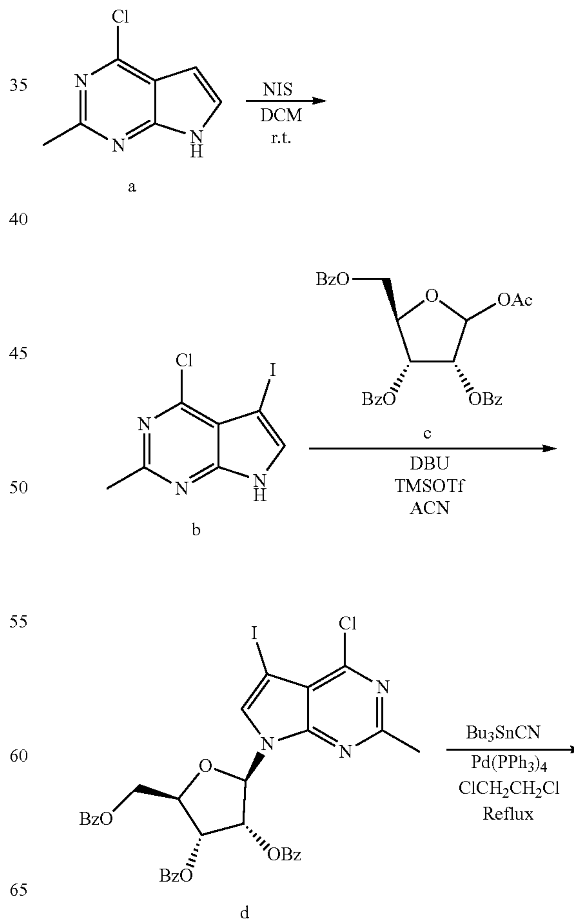
Scheme 1: General Synthesis of Compounds of the Invention
