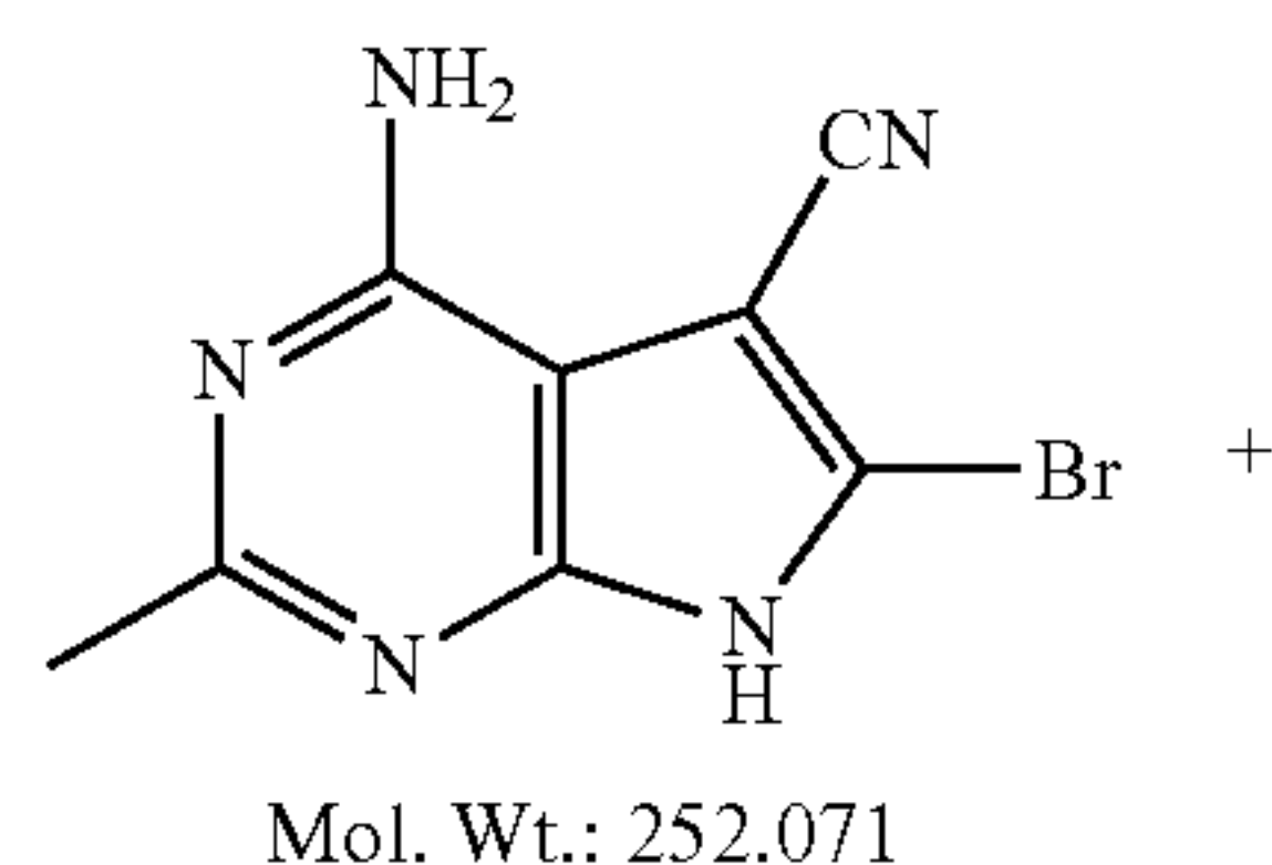
Scheme 2: General Synthesis of Compounds of the Invention
