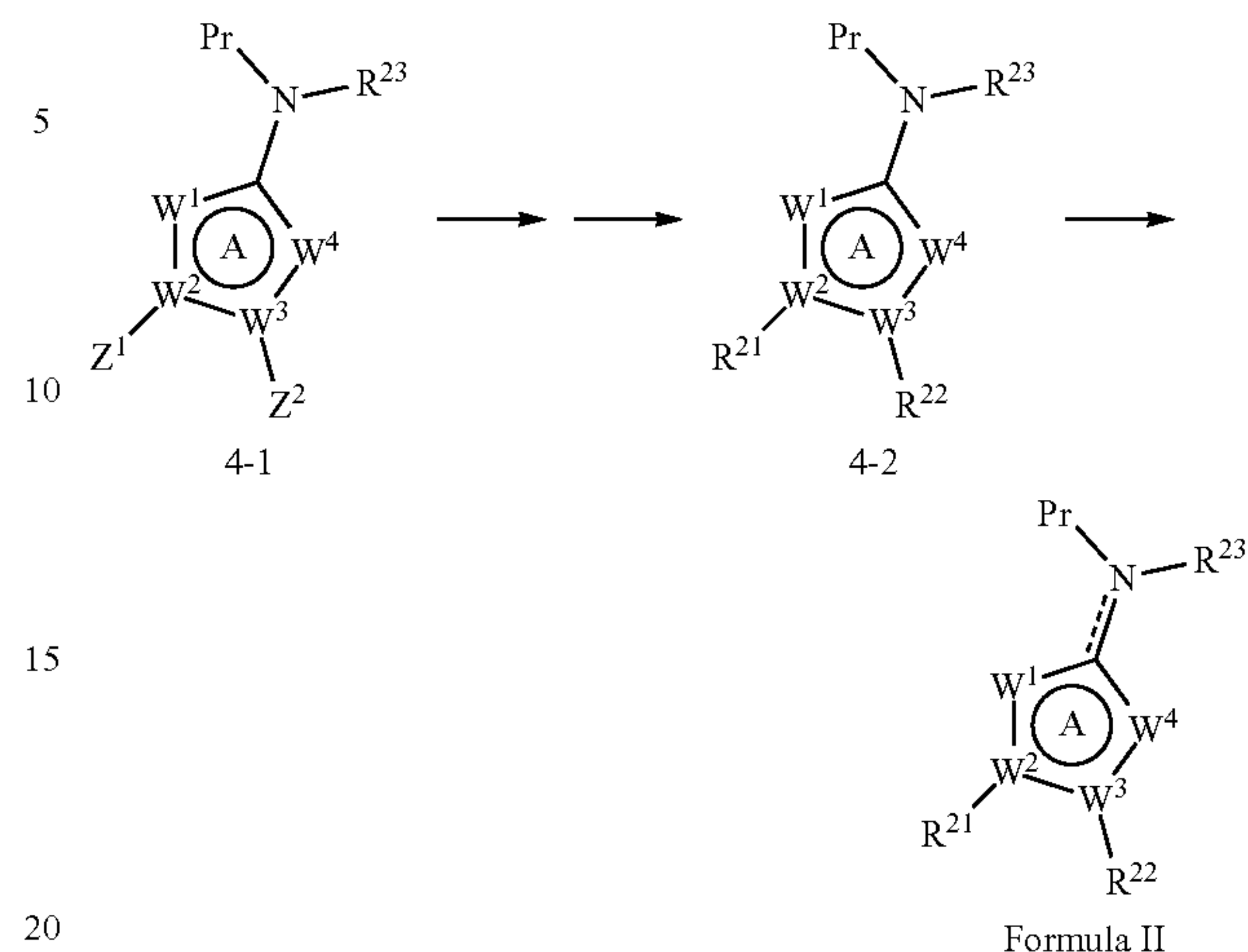
Scheme 4
