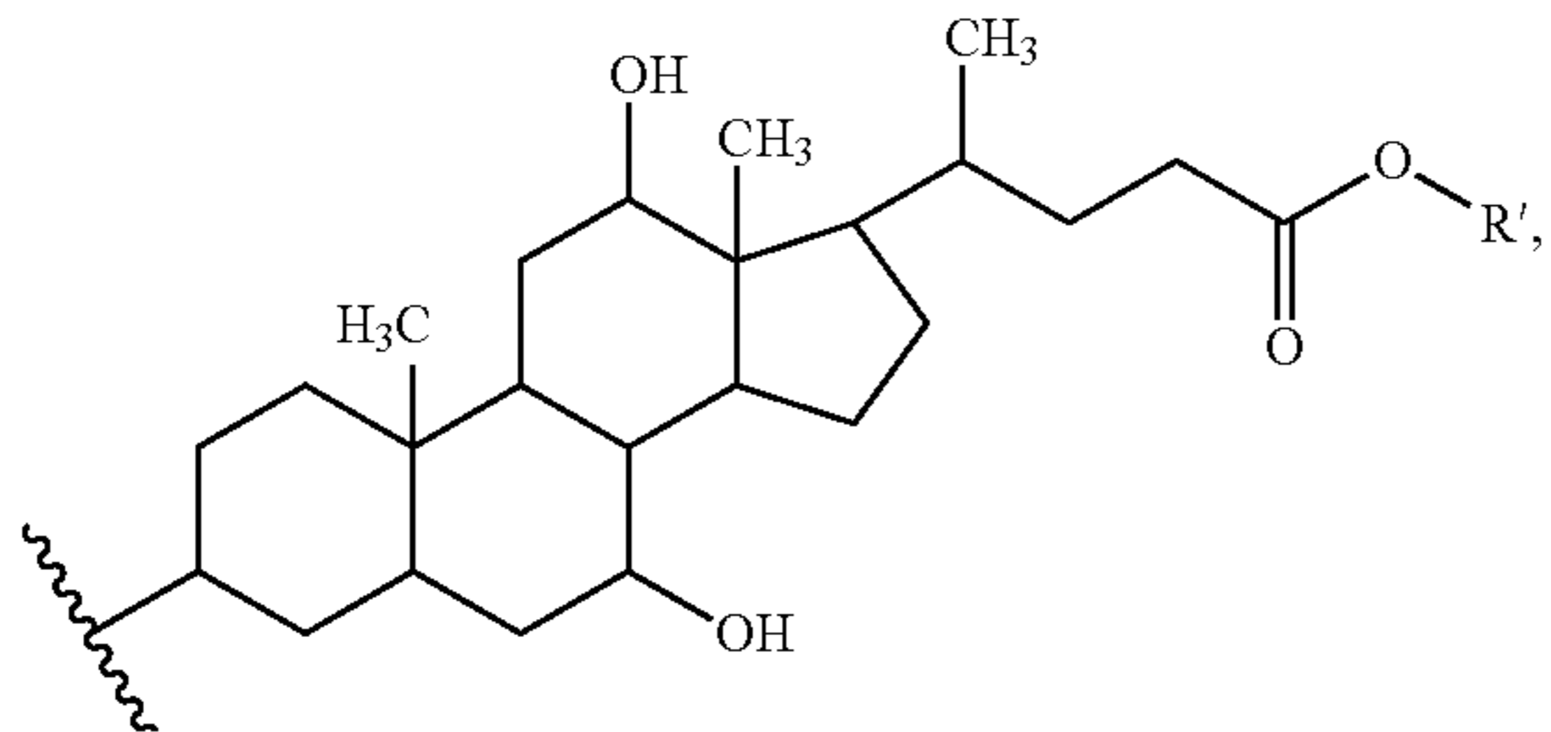
(cholic acid)
