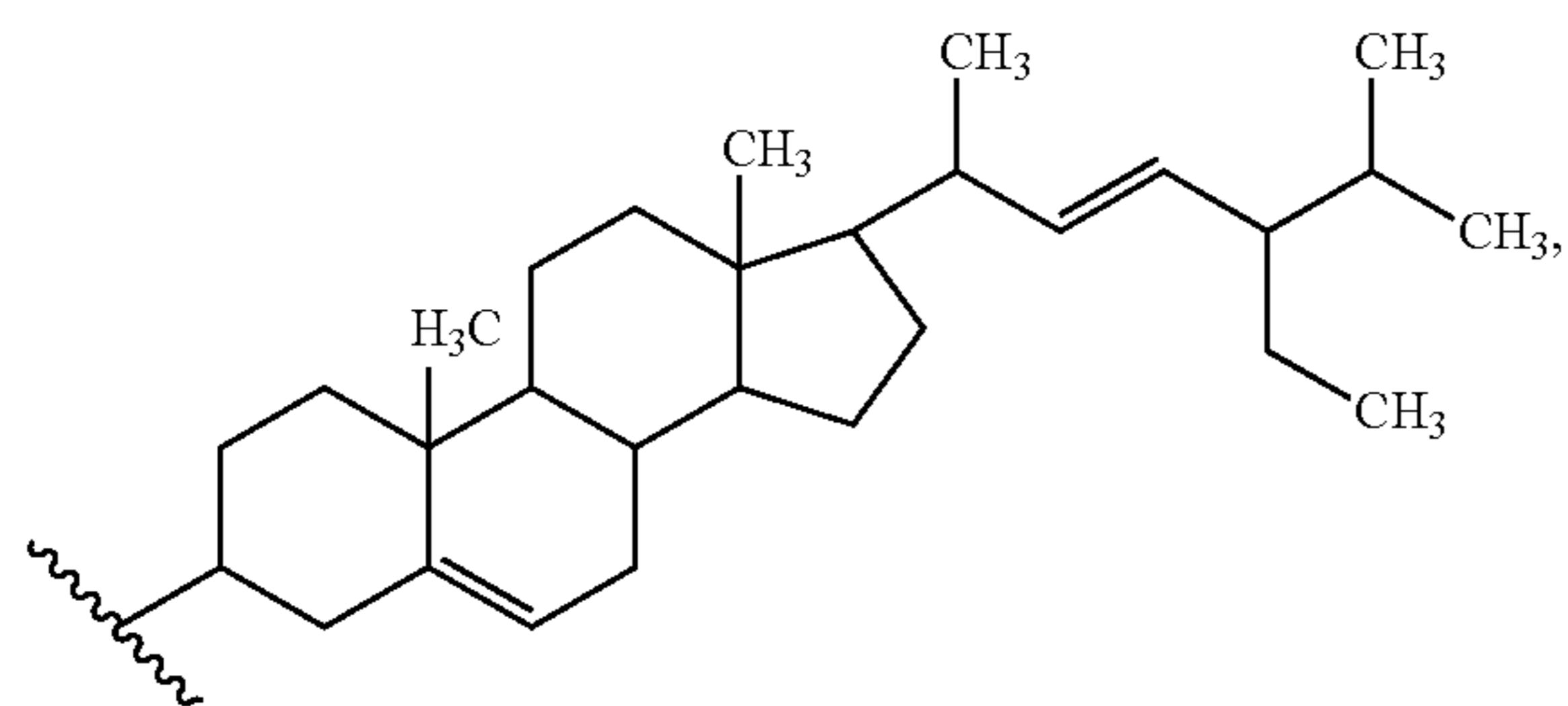
(stigmasterol)
