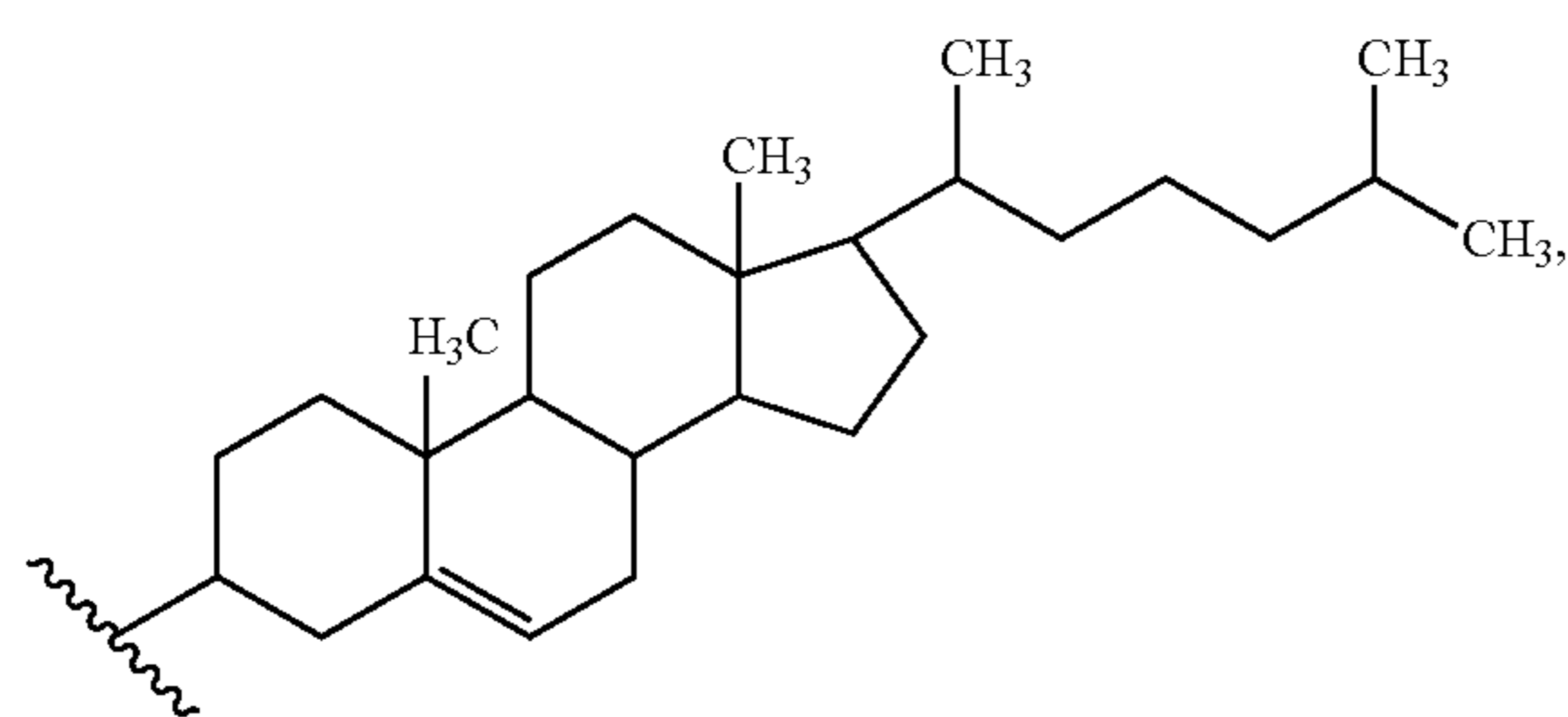
(cholesterol)
