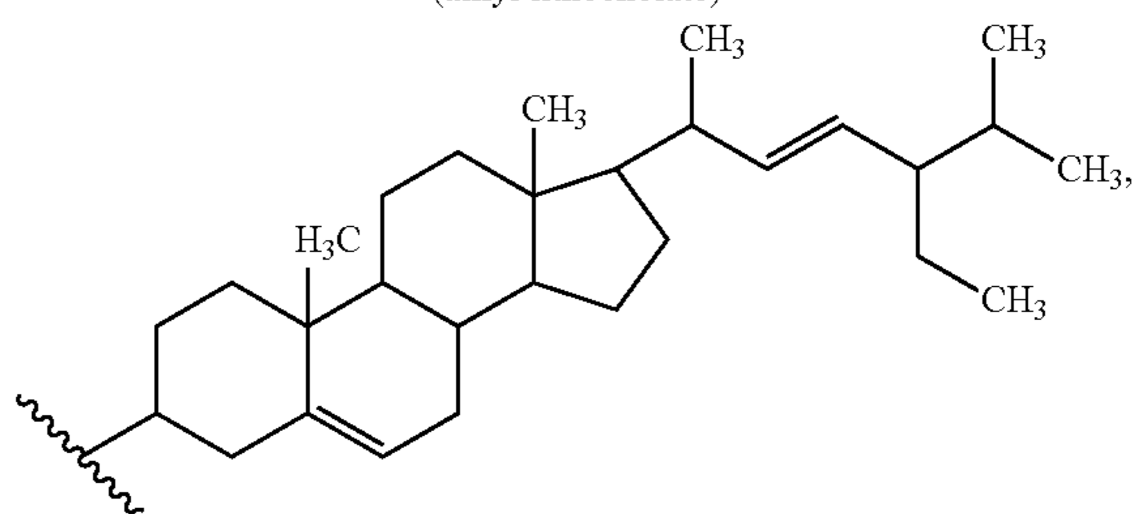
(stigmasterol)
