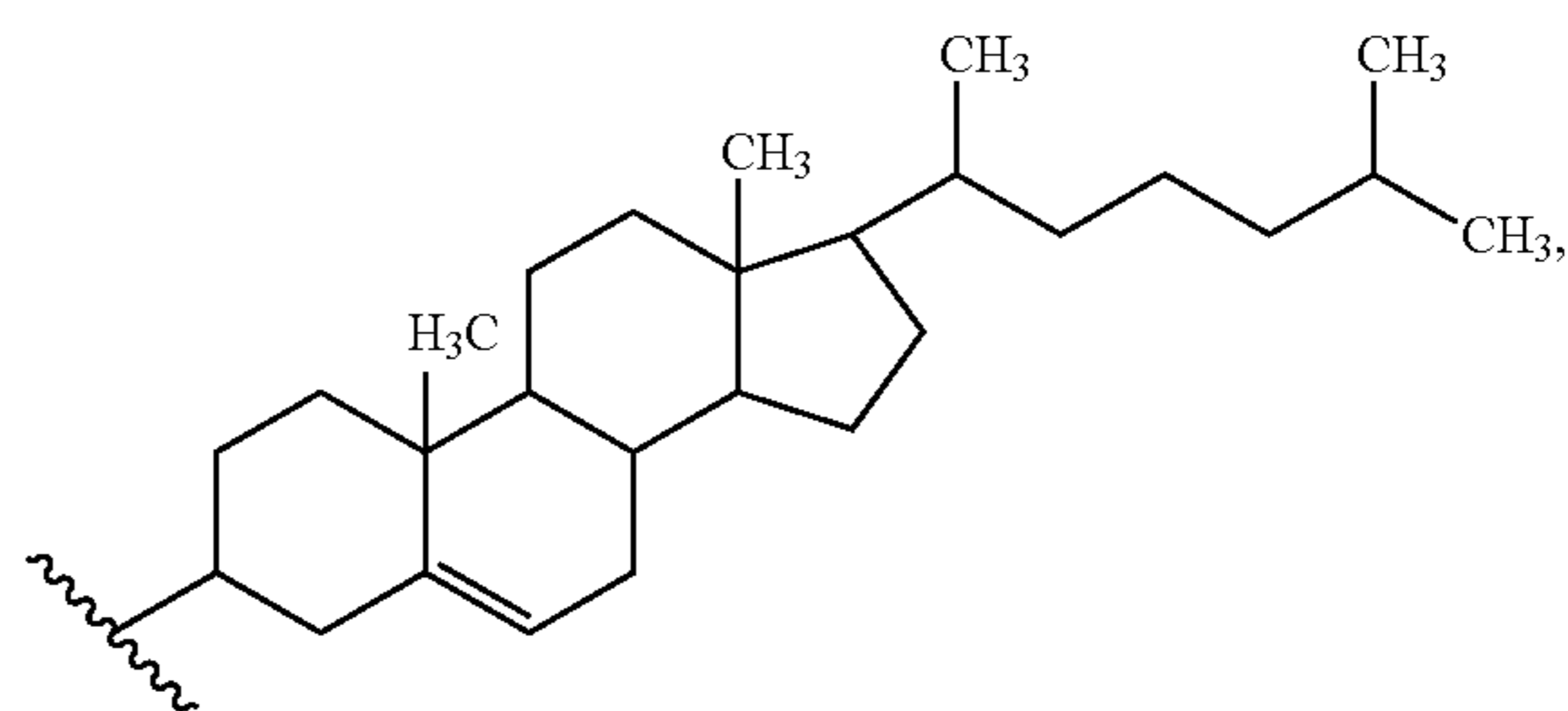
(cholesterol)
