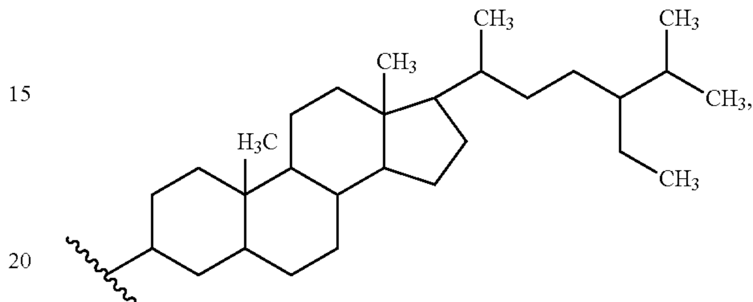
(stigmasterol)
