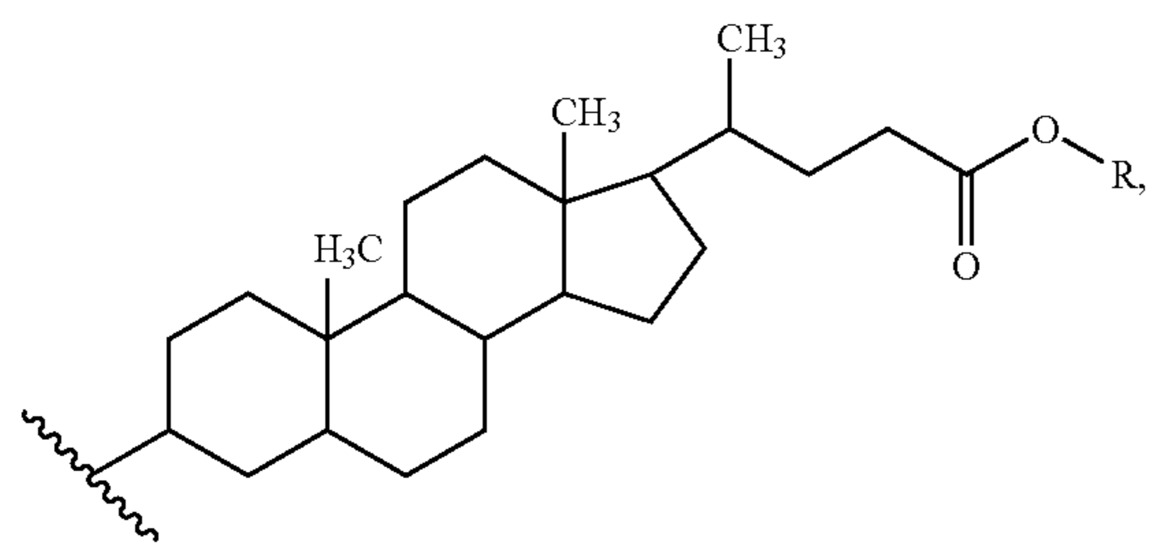
(alkyl lithocholate)
