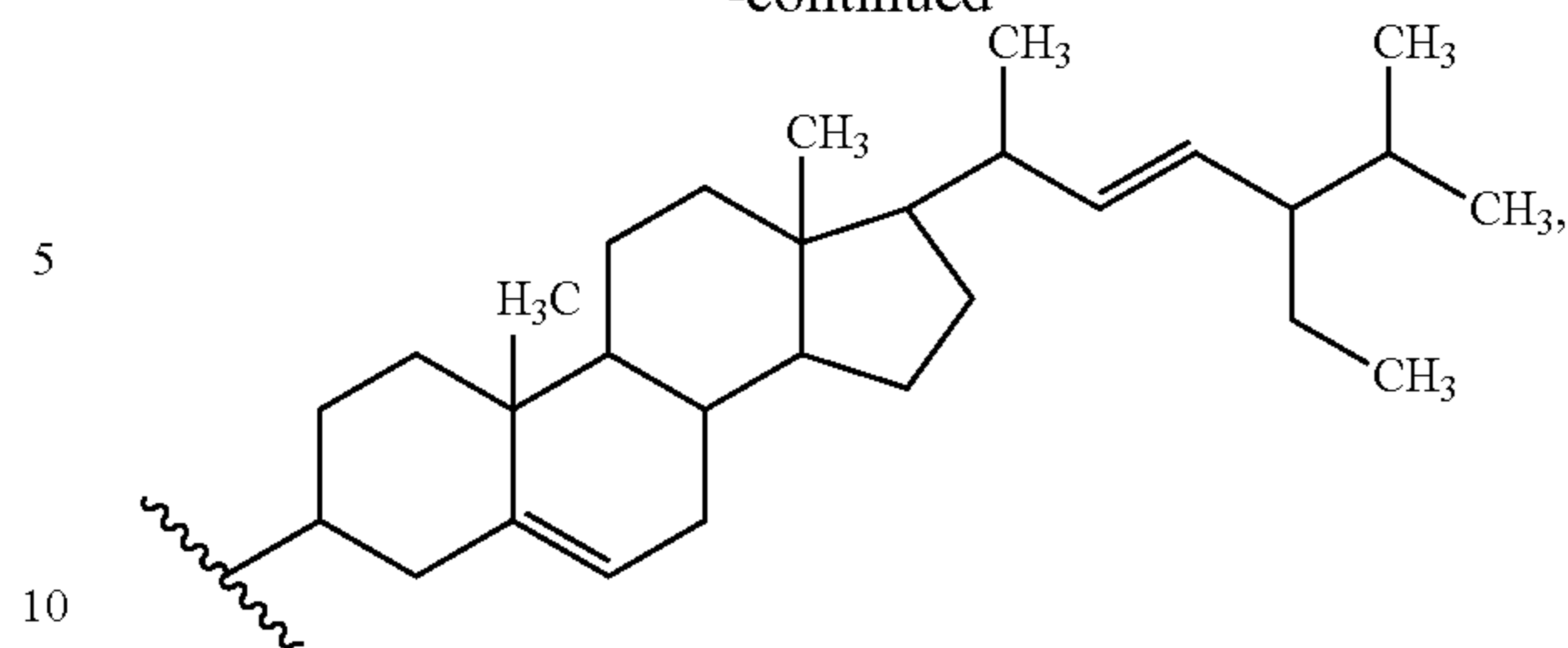
(stigmasterol)
