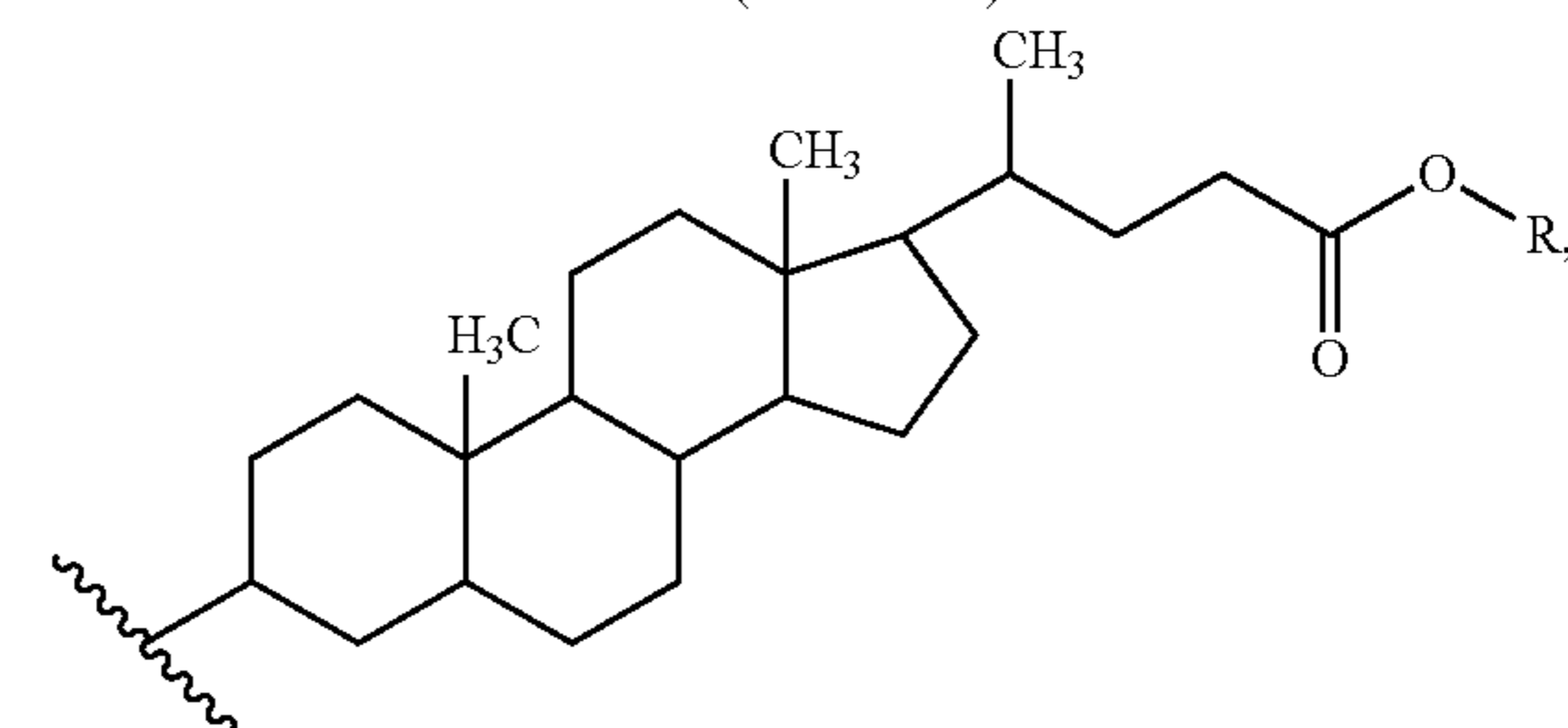
(alkyl lithocholate)
