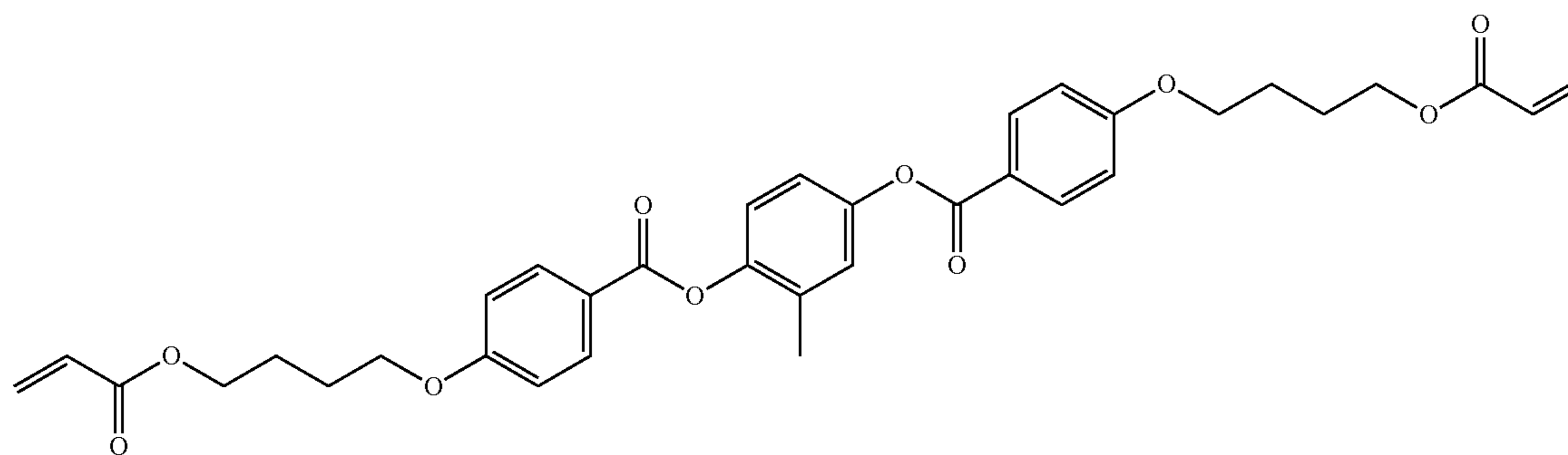
[Rod-like liquid crystal compound-1]
