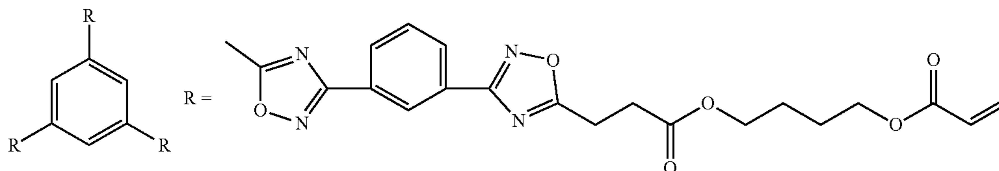
Discotic liquid crystal compound (A)
