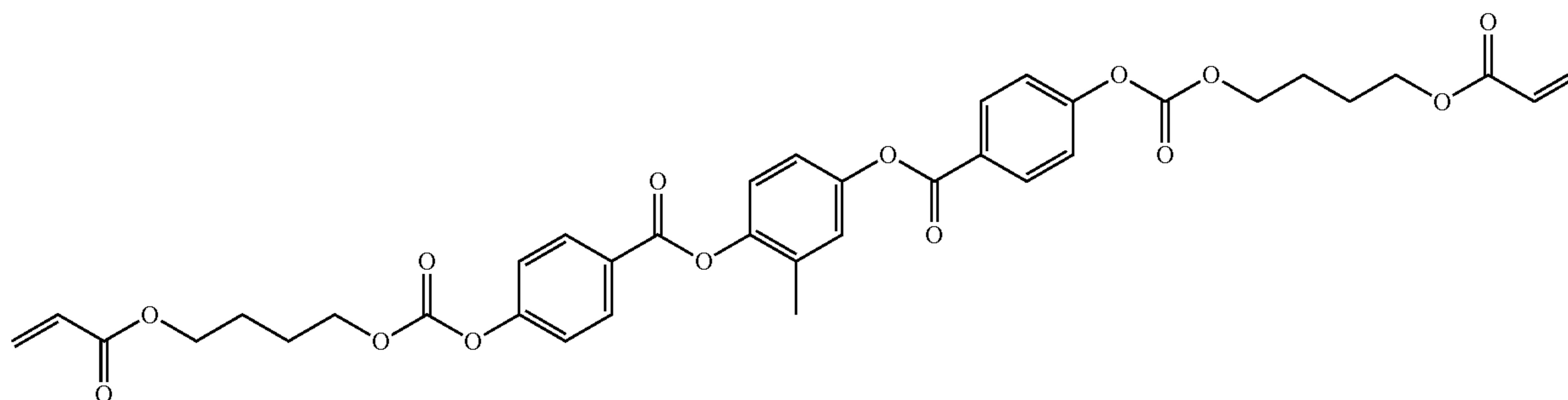
[Rod-like liquid crystal compound-2]
