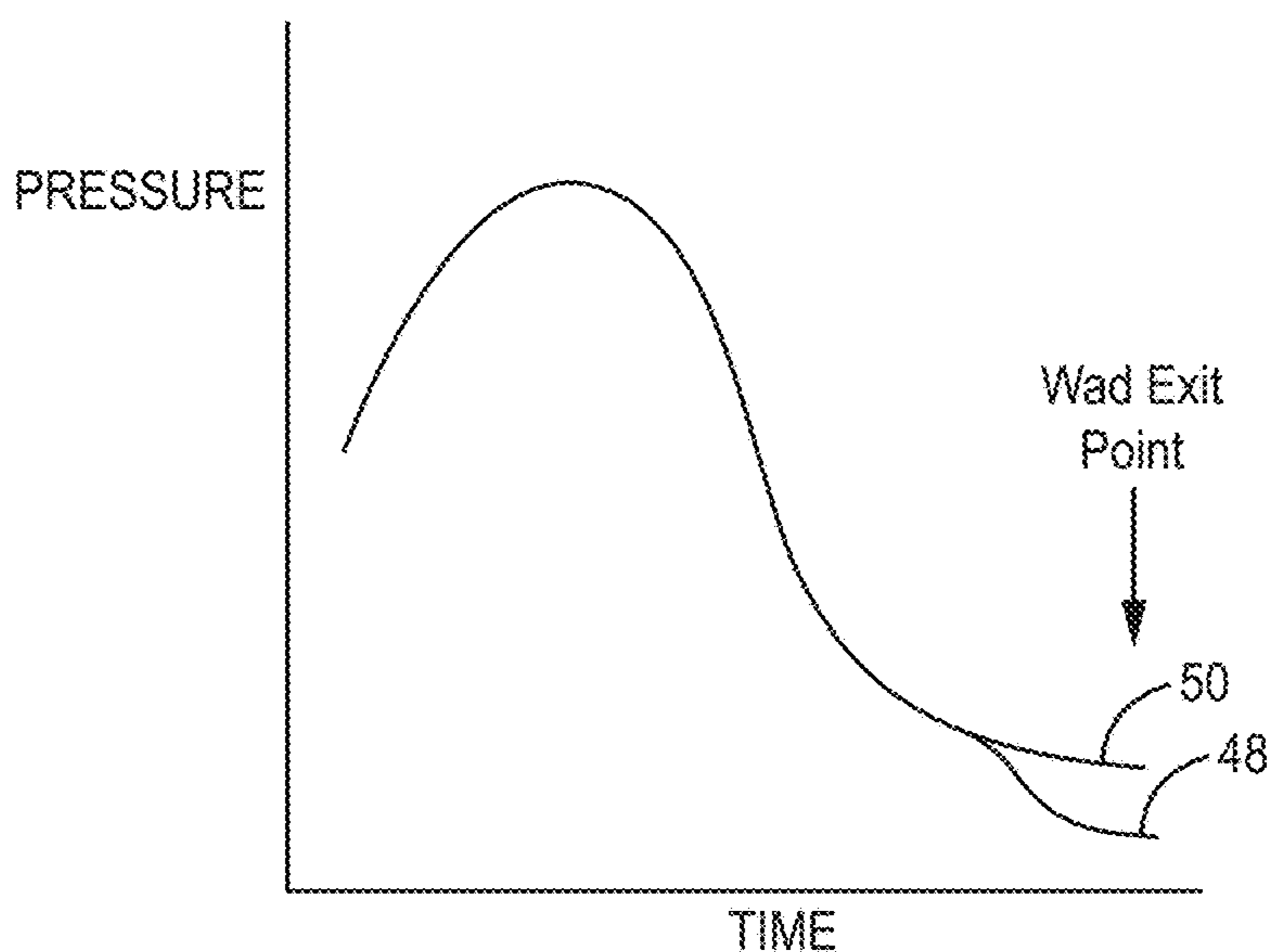
FIG. 5 Prior Art
