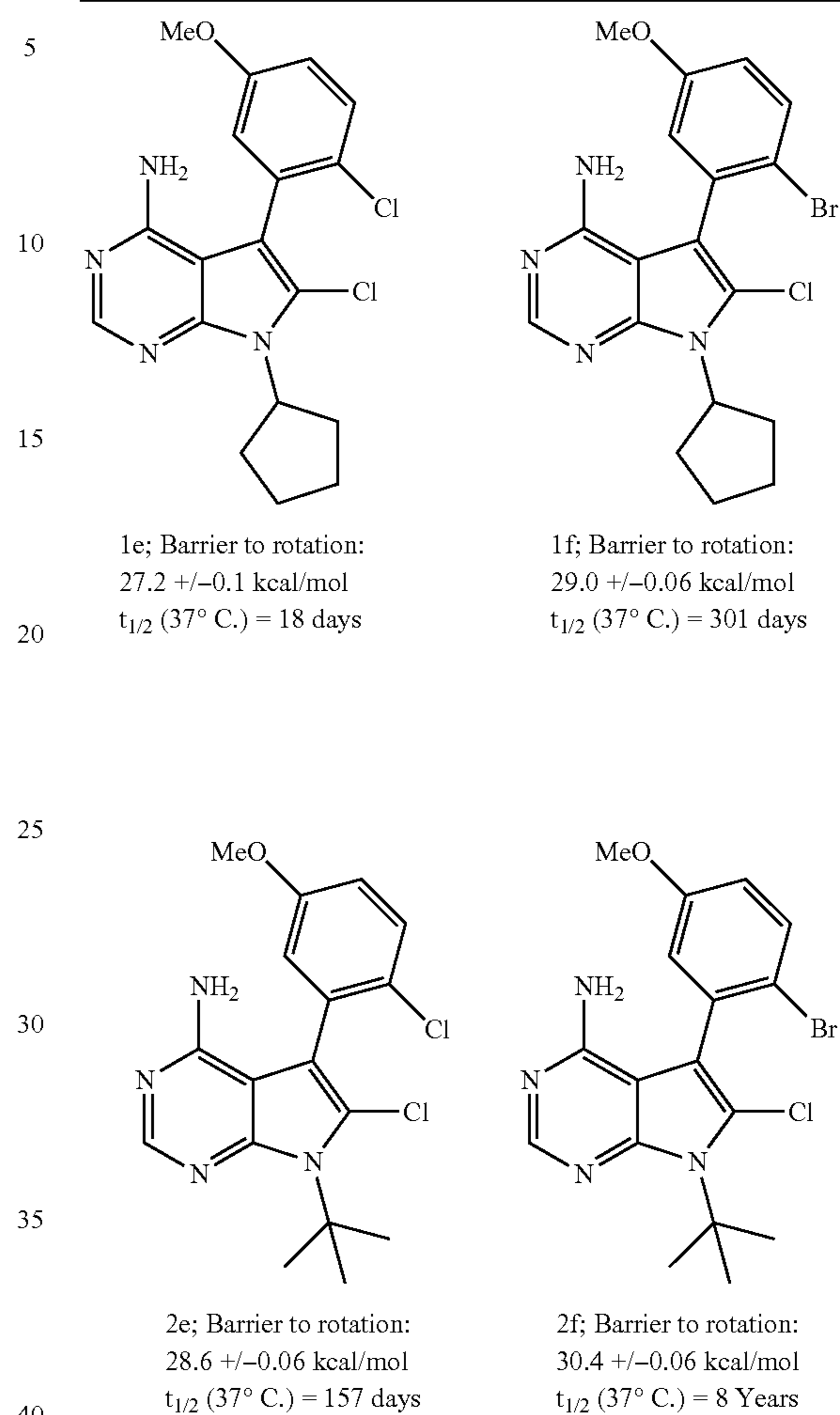
Scheme 2. Experimentally measured barriers to rotation, and extrapolated t 1/2 to racemization at 37° C.
