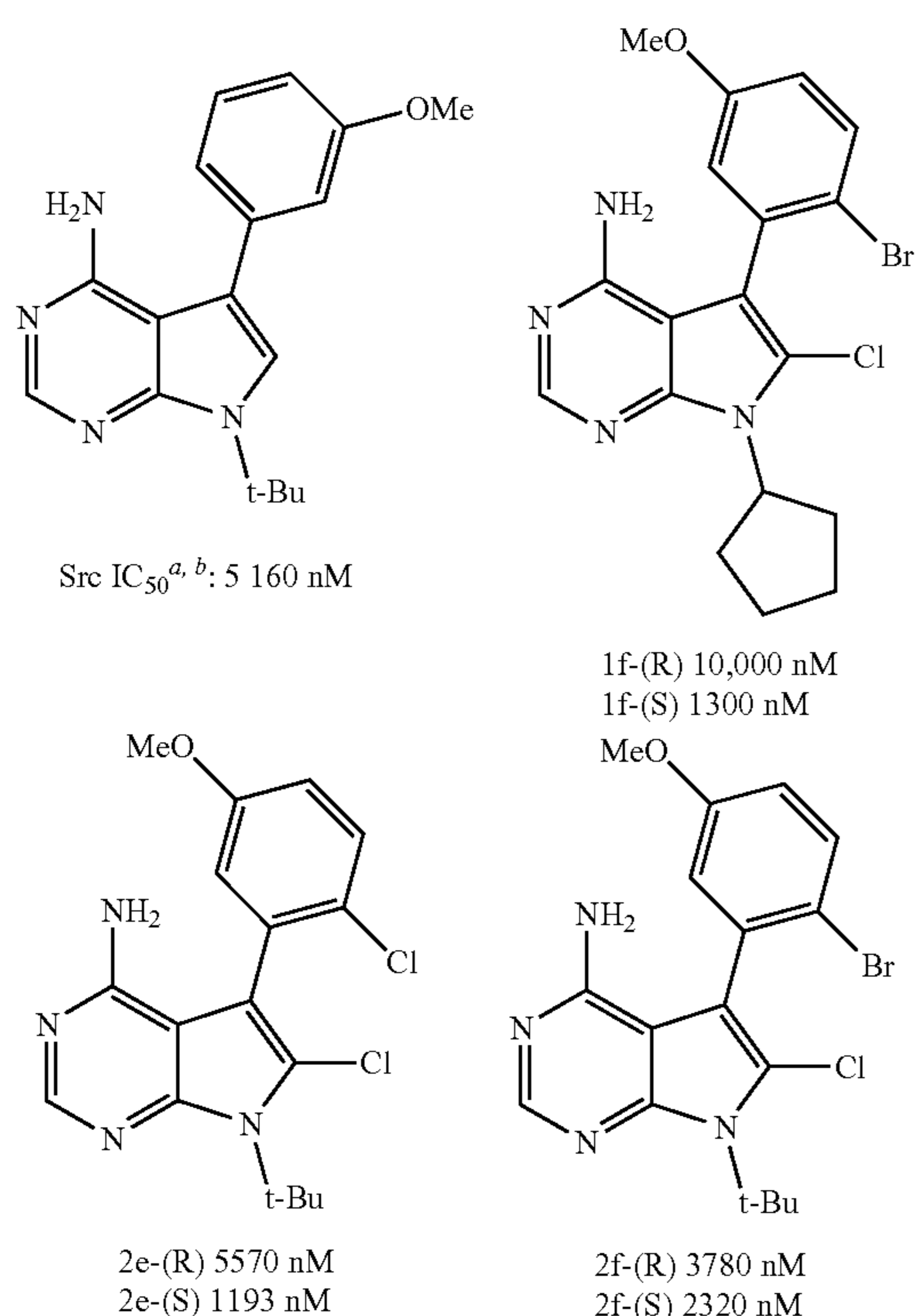
Scheme 3. Differential Src kinase inhibitory activities between atropisomers.
