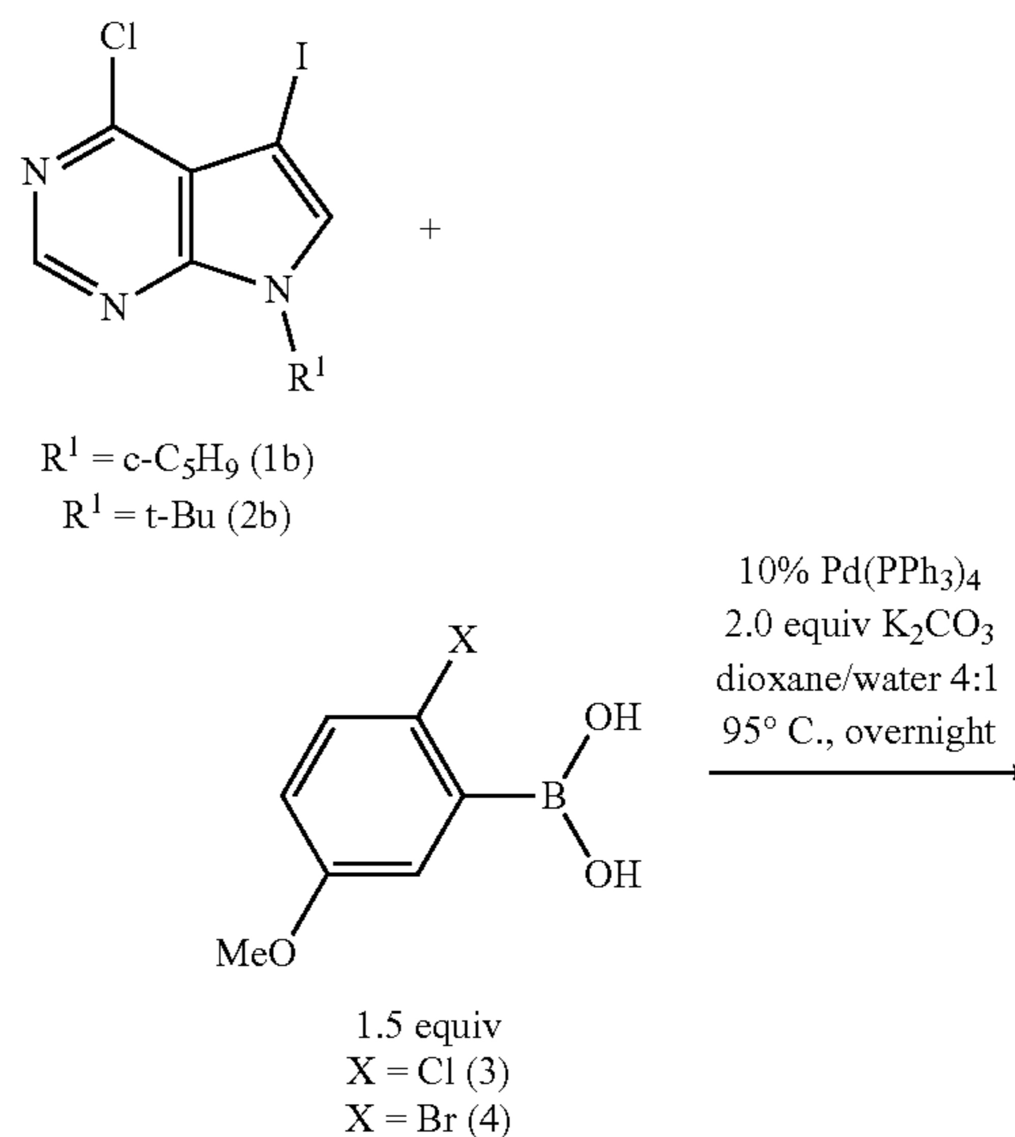
Scheme 1. Synthesis of atropisomerically stable PPY kinase inhibitors.
