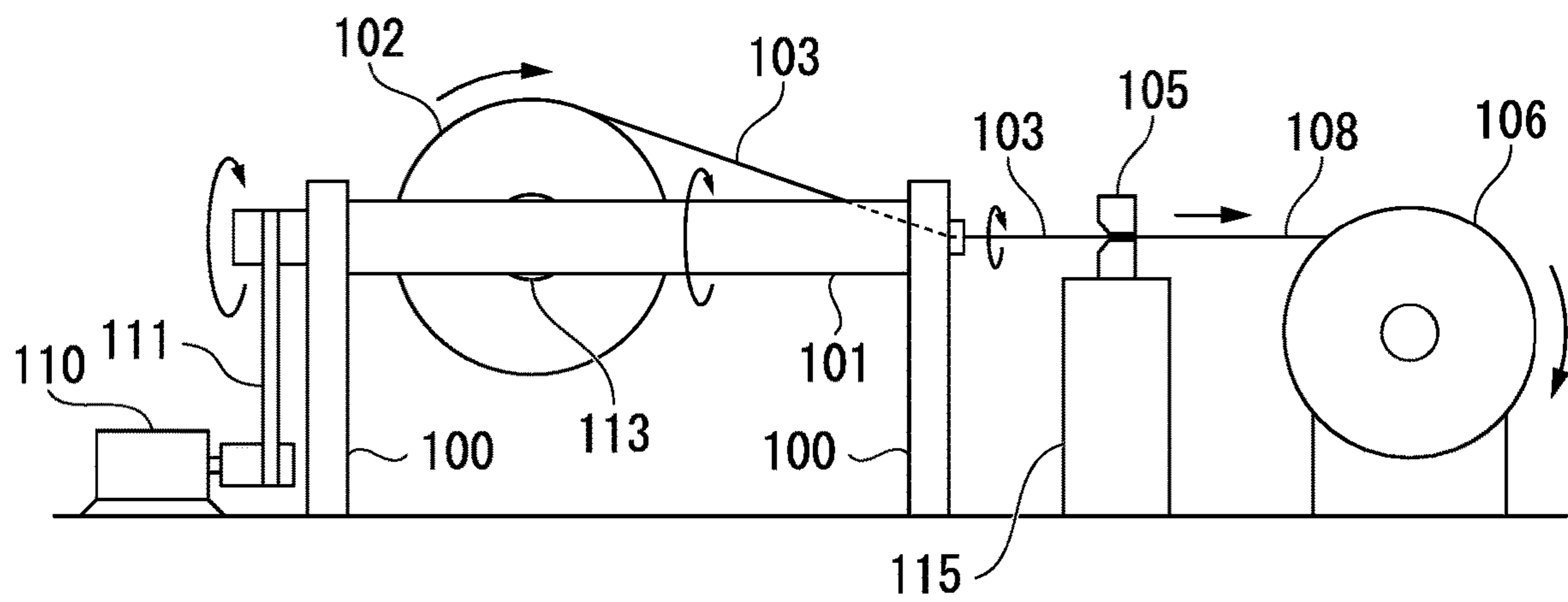
FIG. 14 Prior Art
