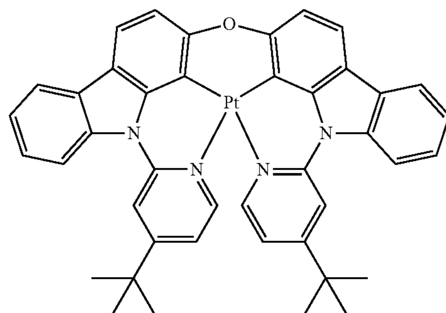
PtNON-dtb
