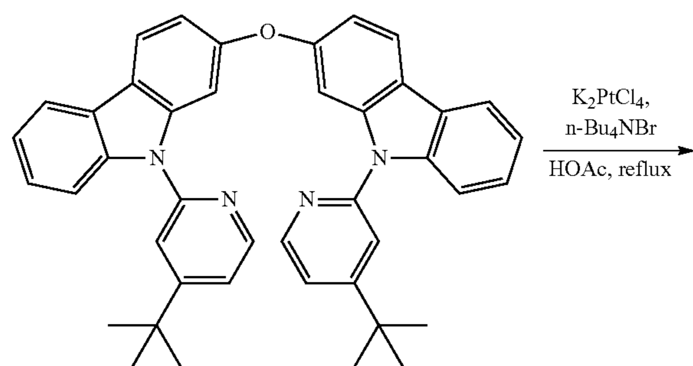
NON-dtb Ligand
