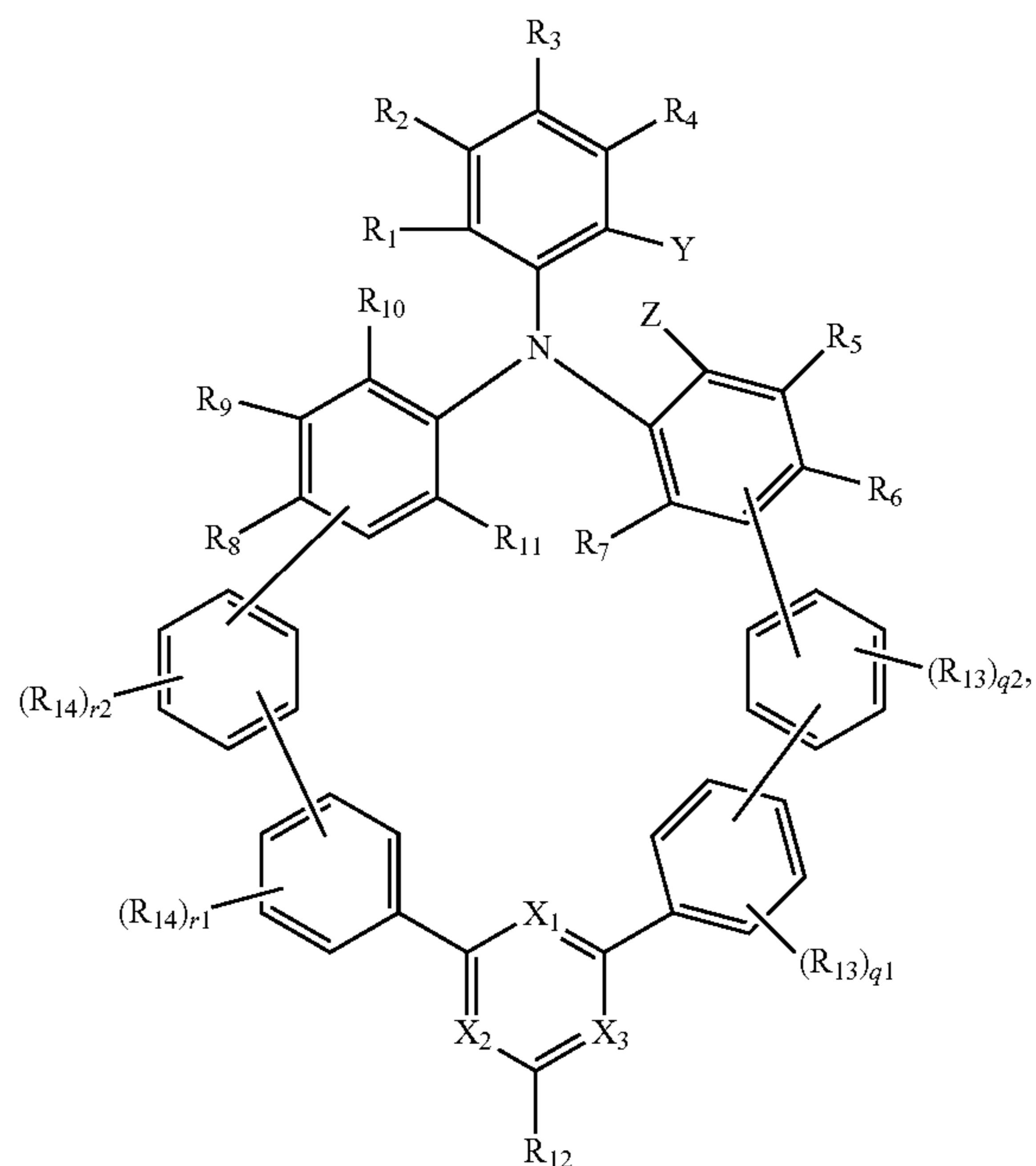
Formula 1-4
