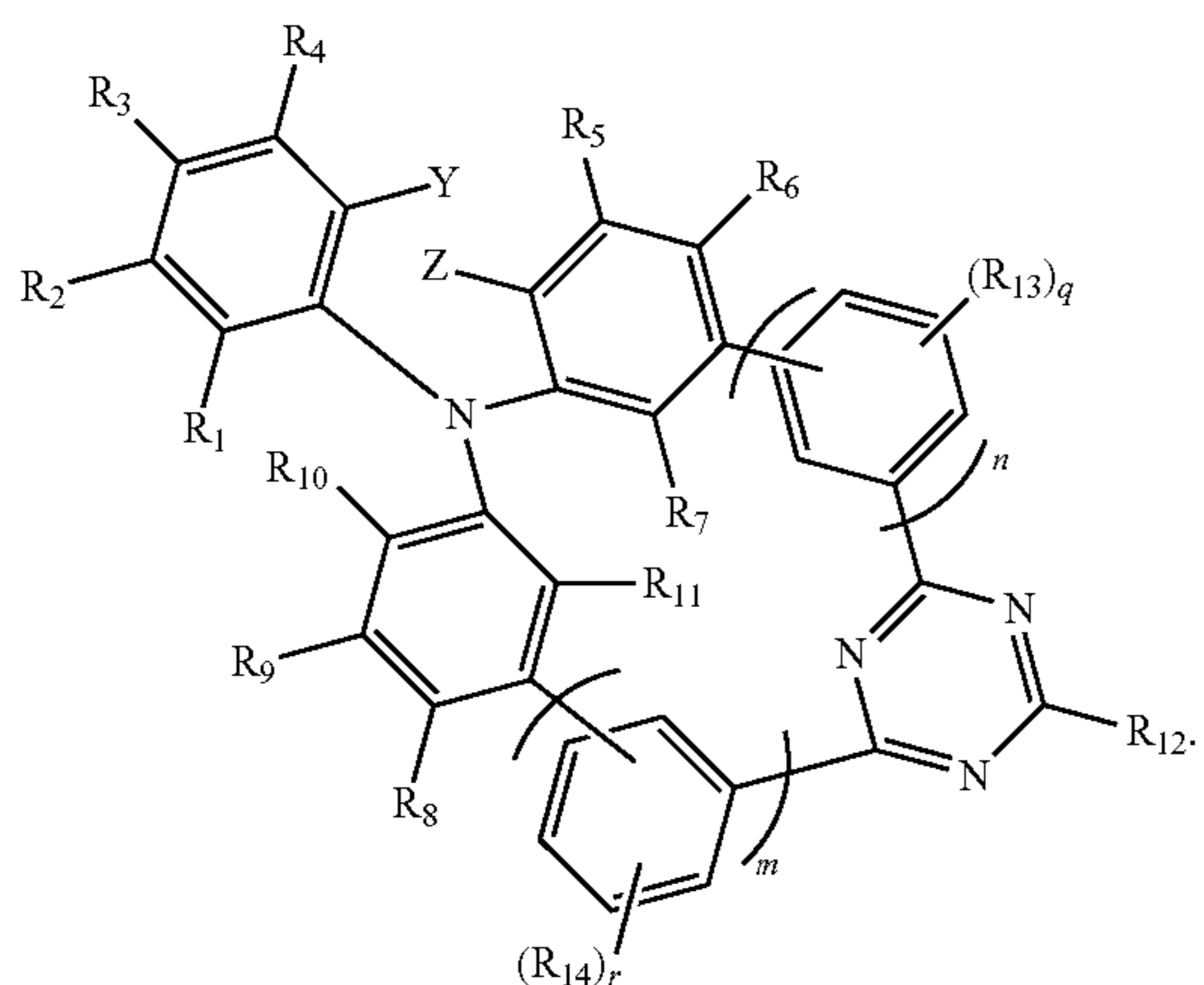
Formula 1-2
