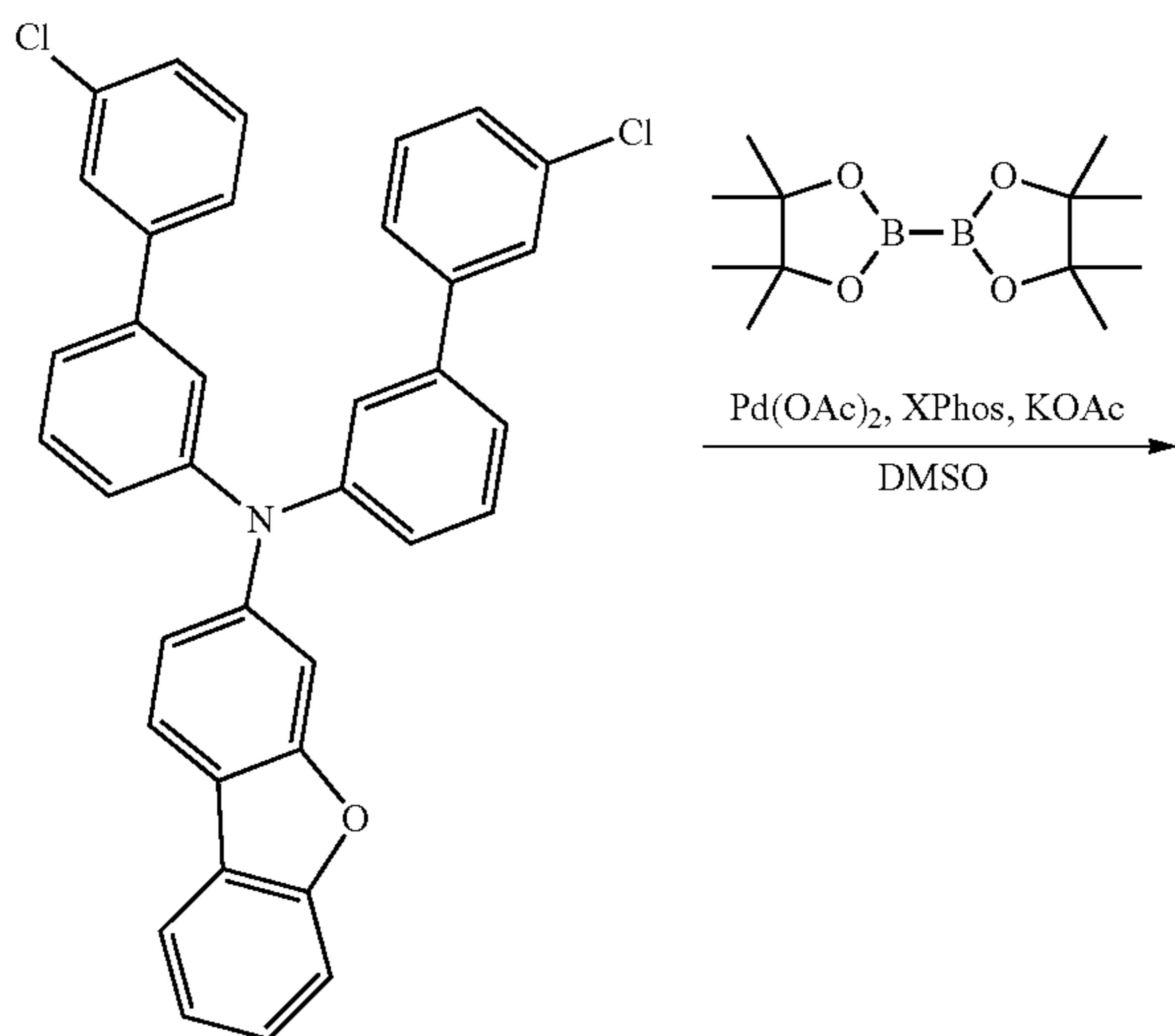
Reaction 4-2
