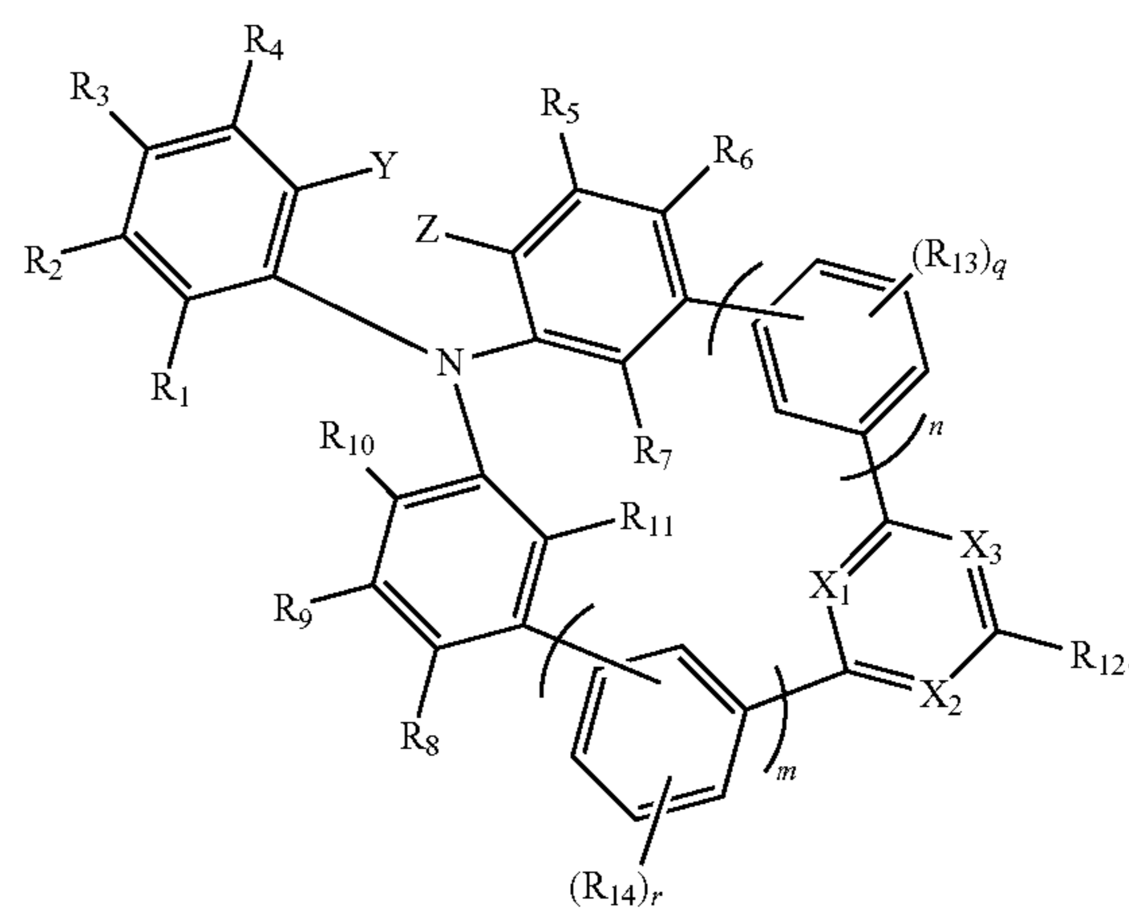
Formula 1
