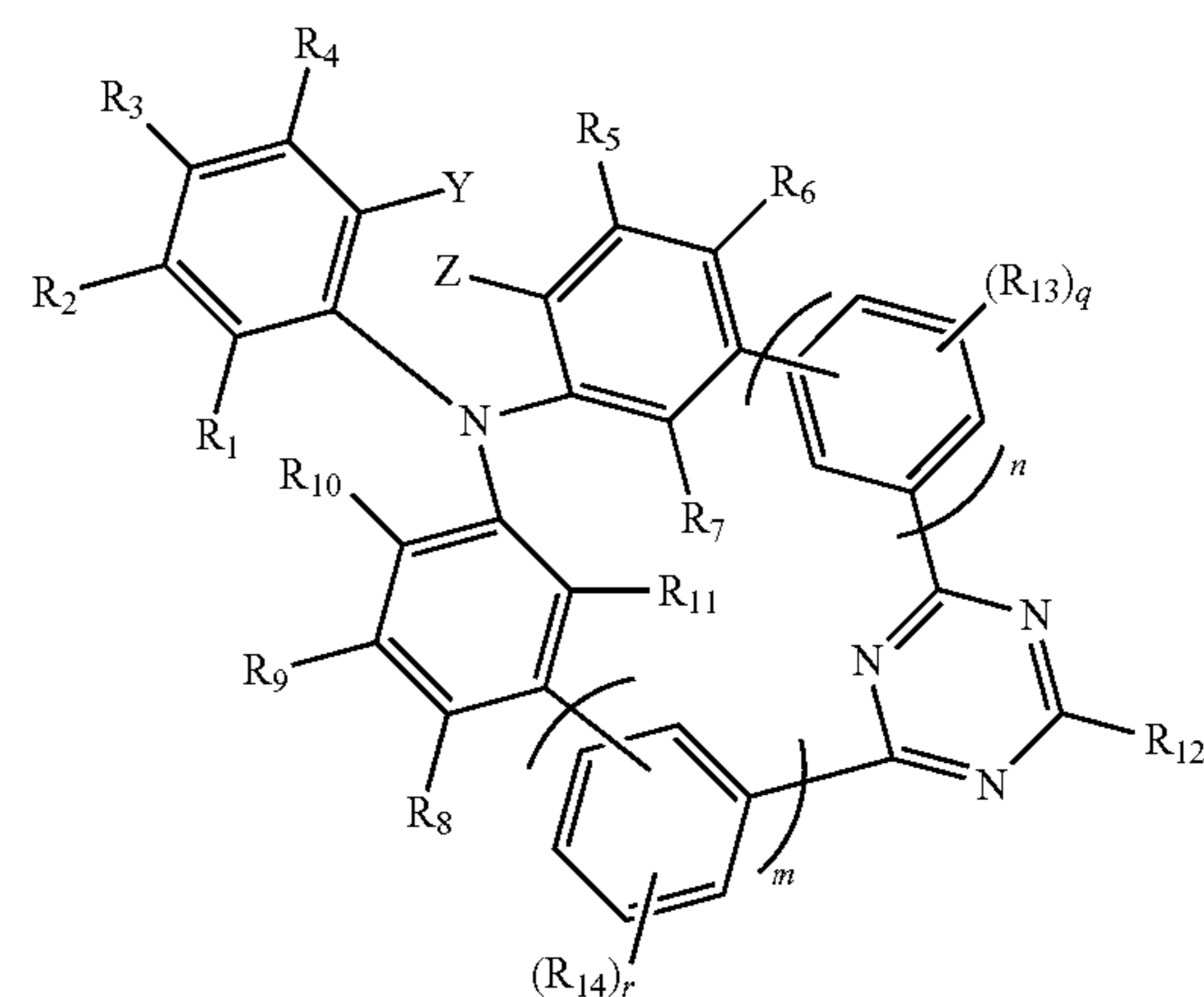
Formula 1-2
