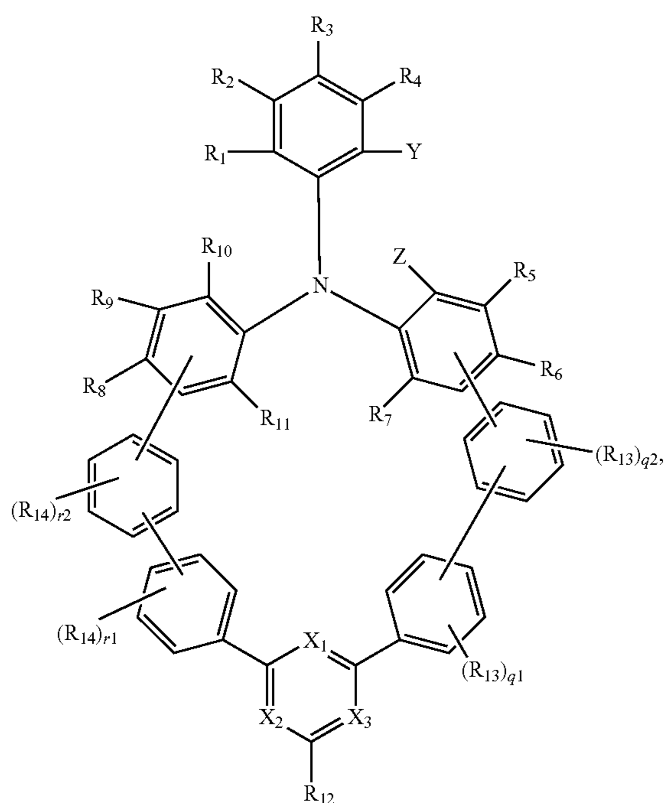
Formula 1-4
