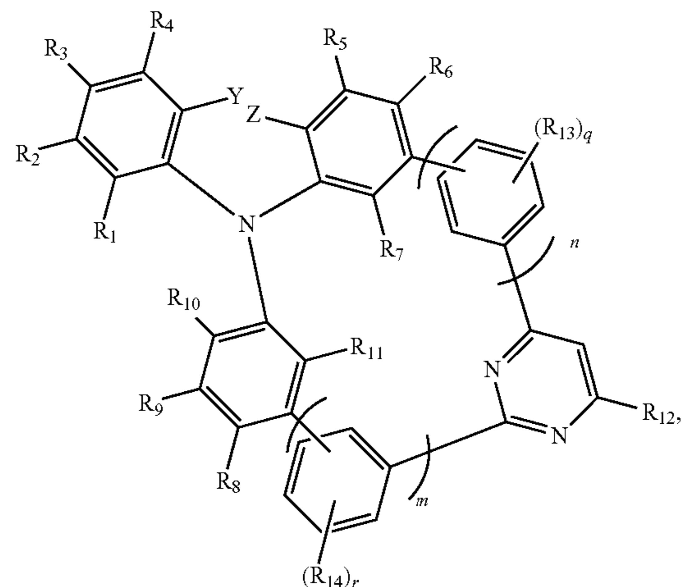
Formula 1-1
