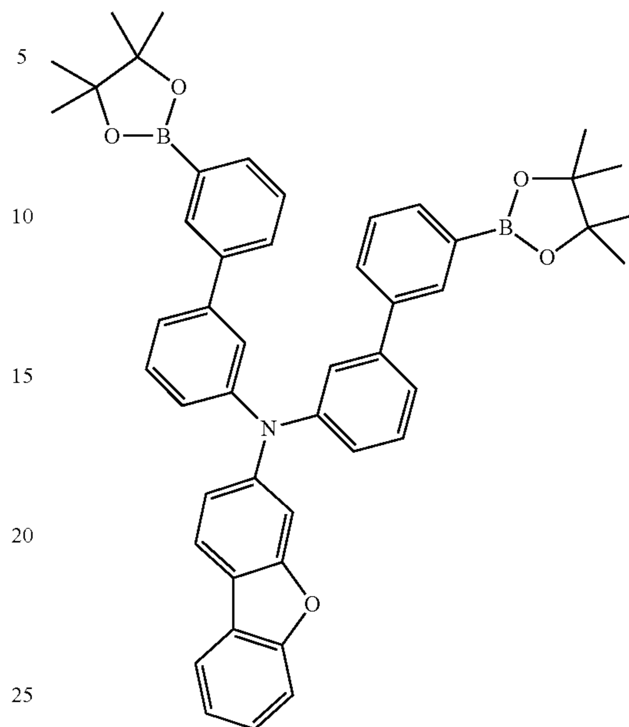
Reaction 4-3
