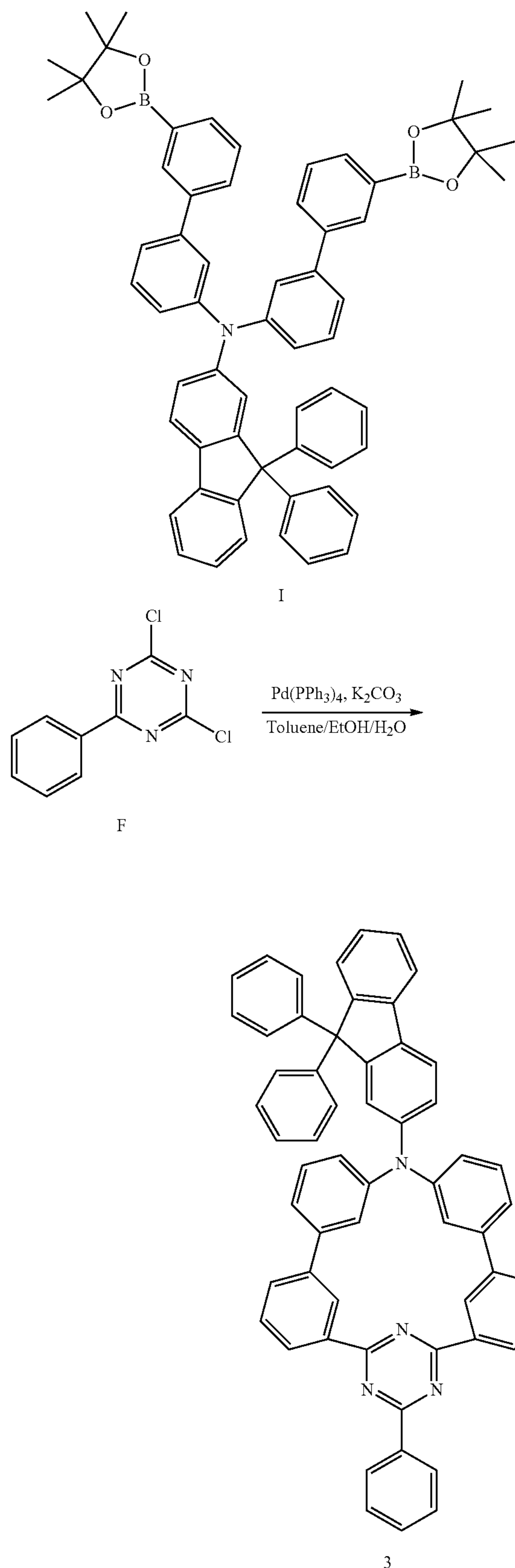
Reaction 3-3
