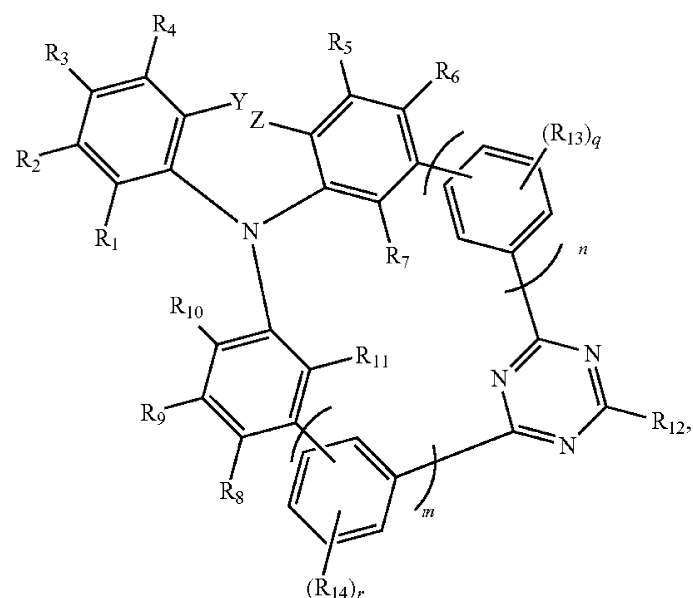
Formula 1-2
