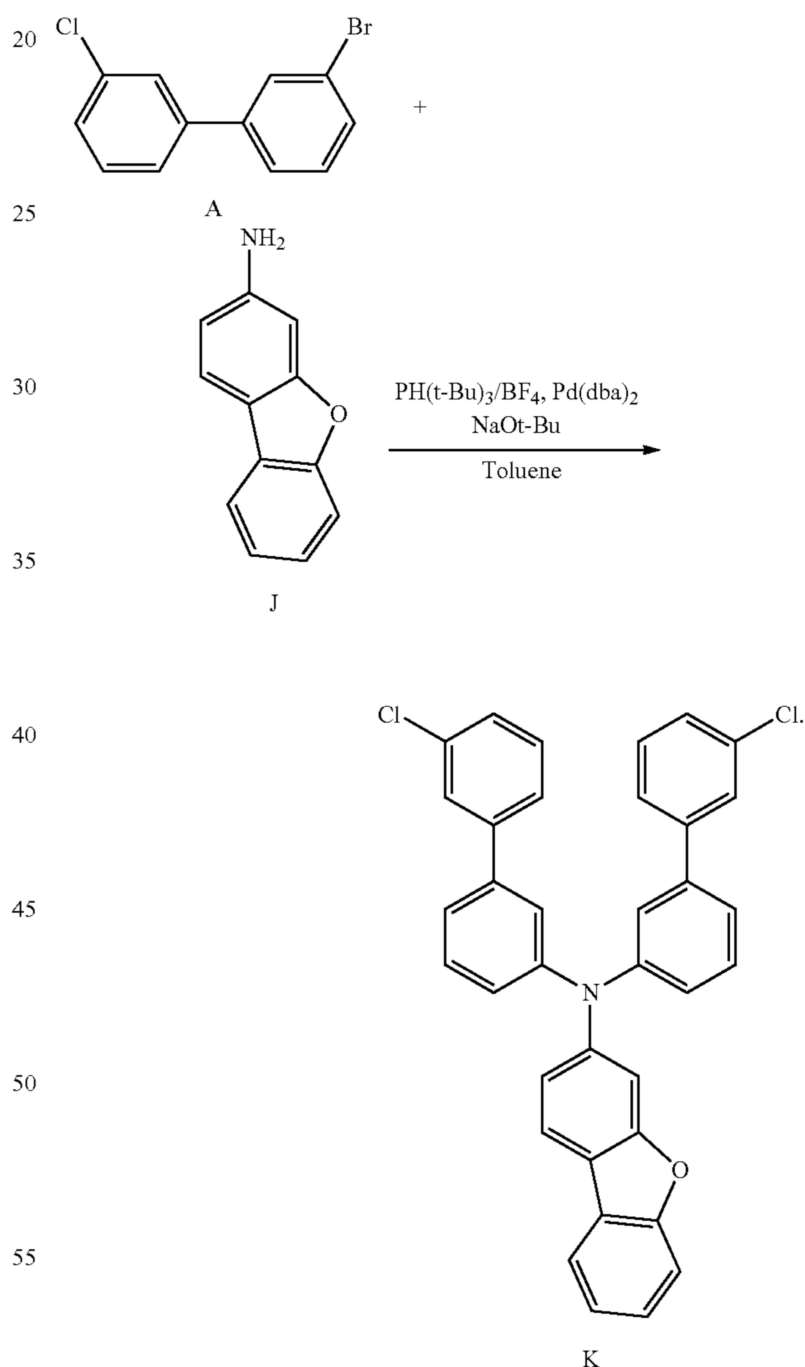
Reaction 4-1
