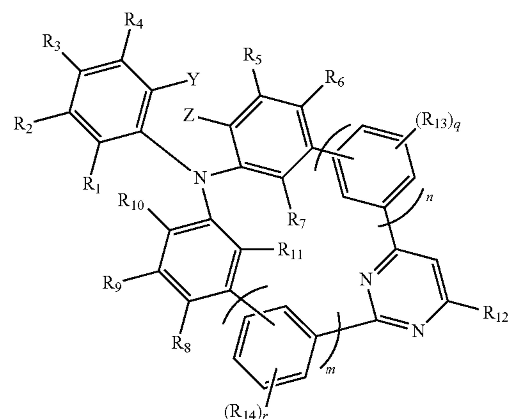
Formula 1-1
