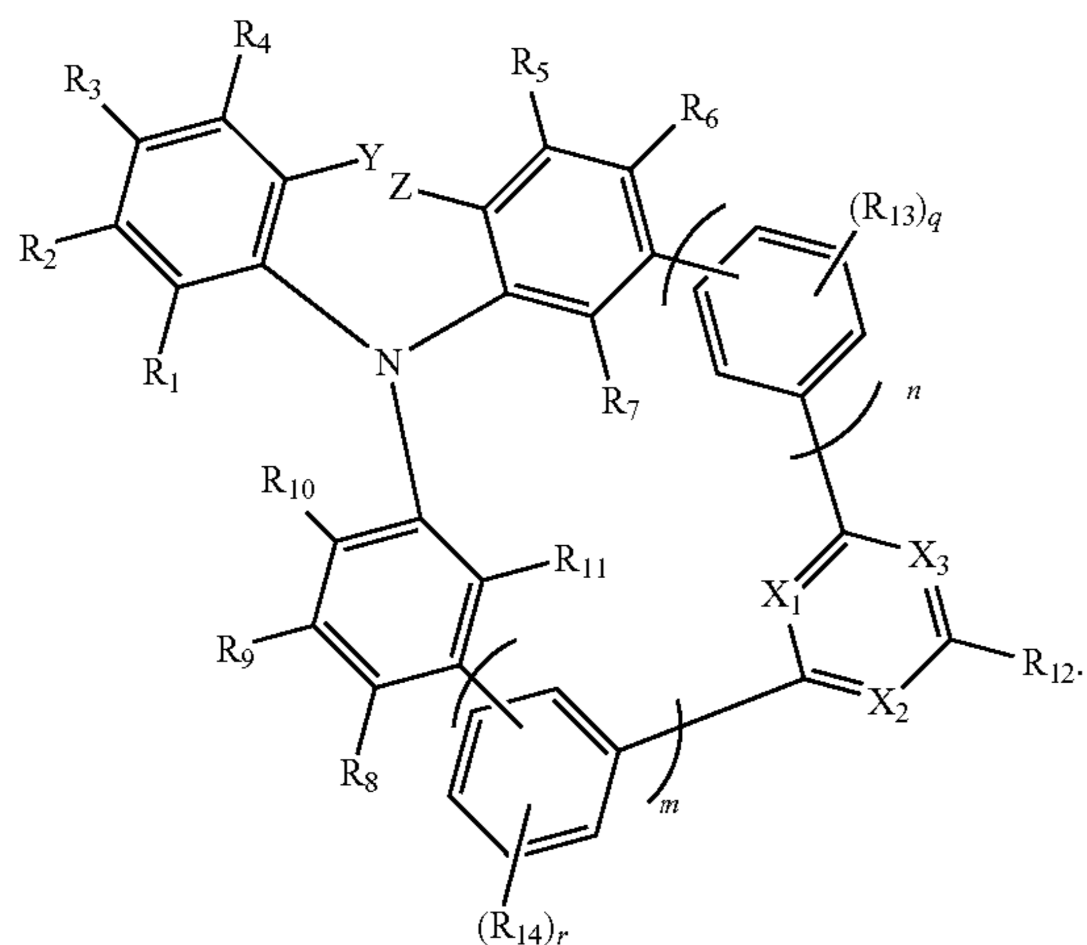
Formula 1
