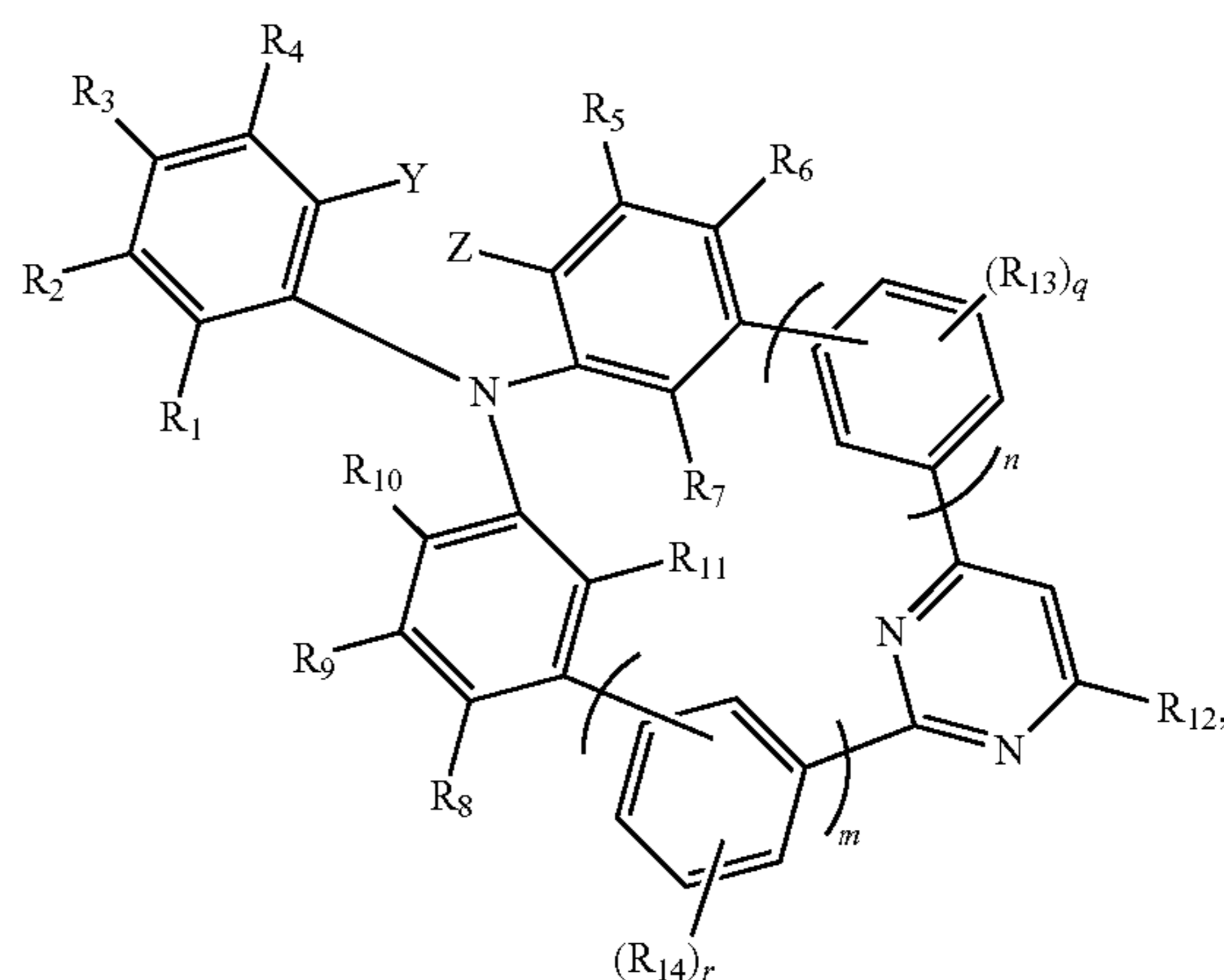
Formula 1-1
