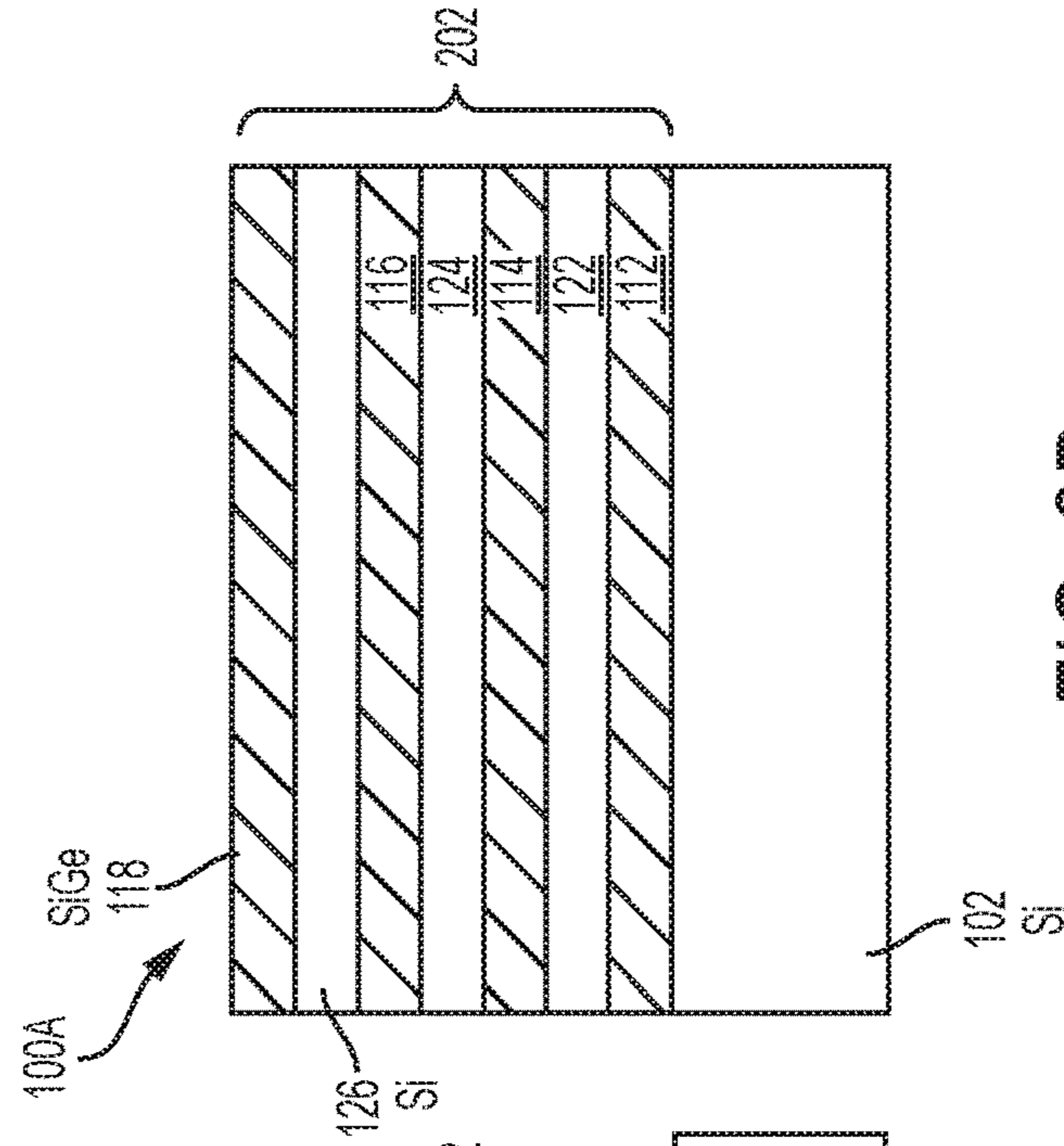
ACROSS-GATE VIEW
