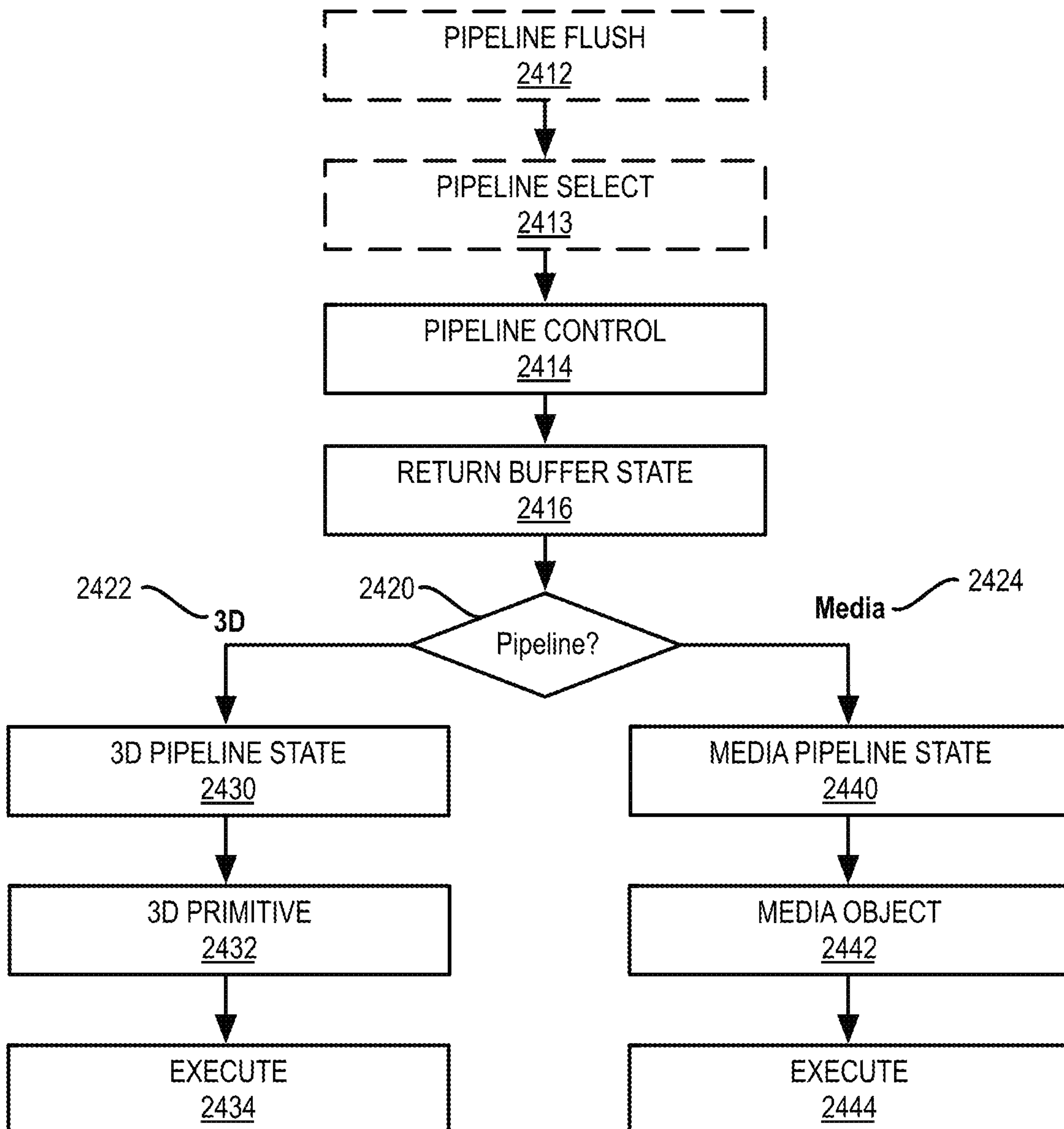
GRAPHICS PROCESSOR COMMAND SEQUENCE 2410
