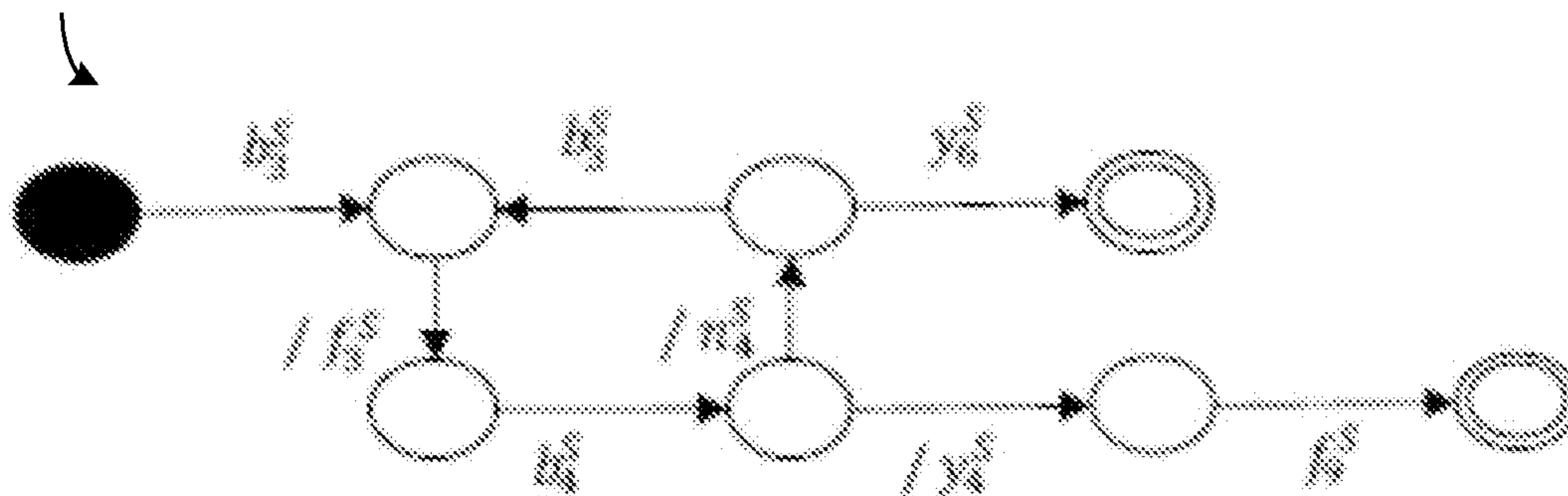
Reduced Statechart for Surveyor
