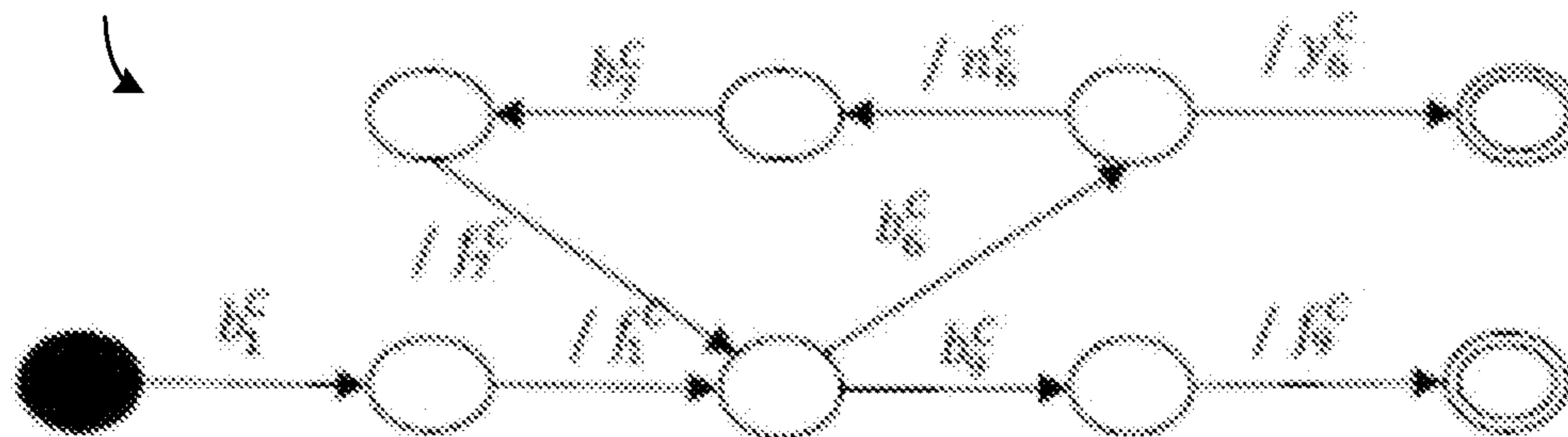
Reduced Statechart for Client
