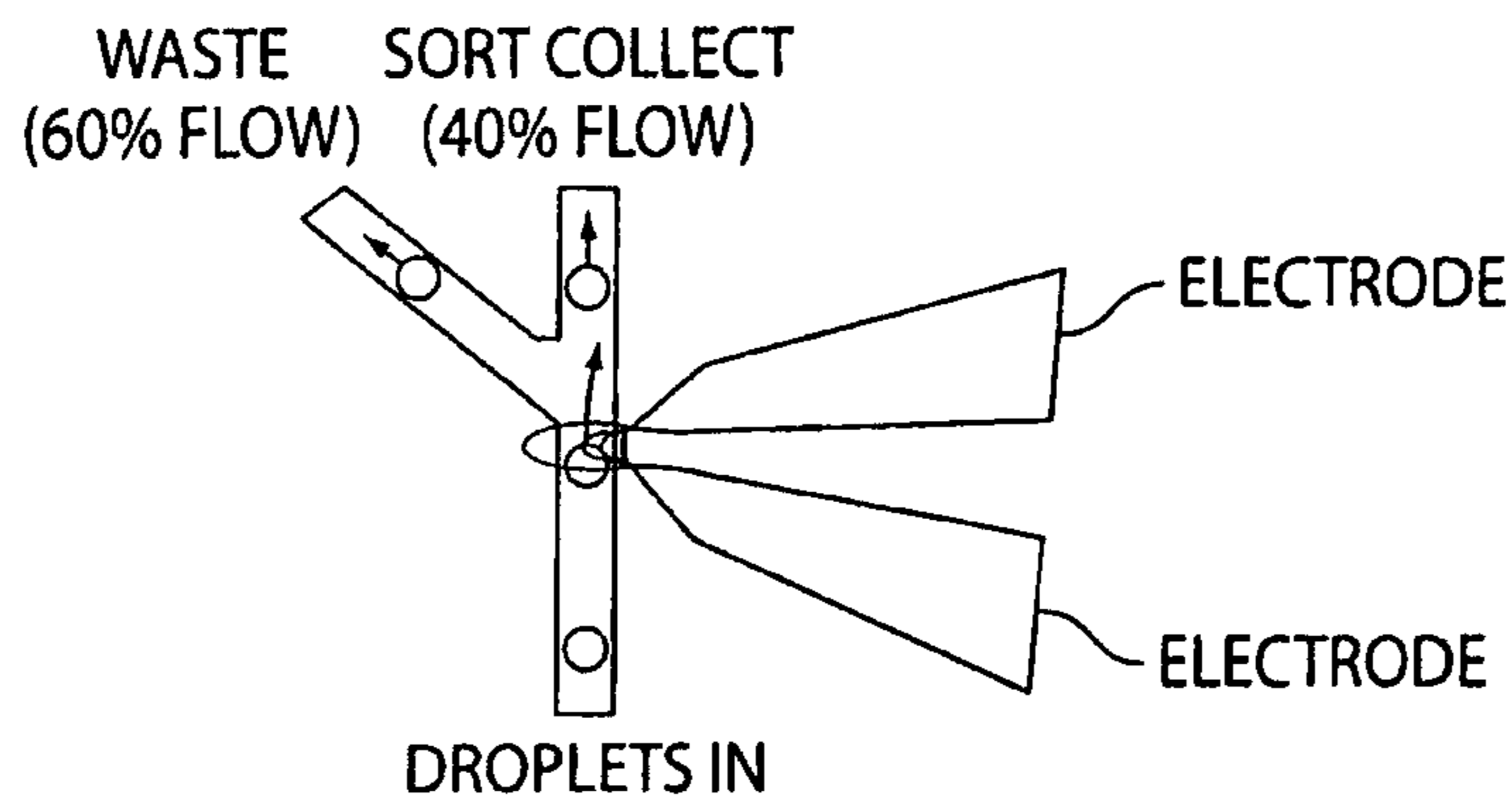
FLIPPED FLUIDIC GEOMETRY (ASYMMETRIC FLOW GEOMETRY)
