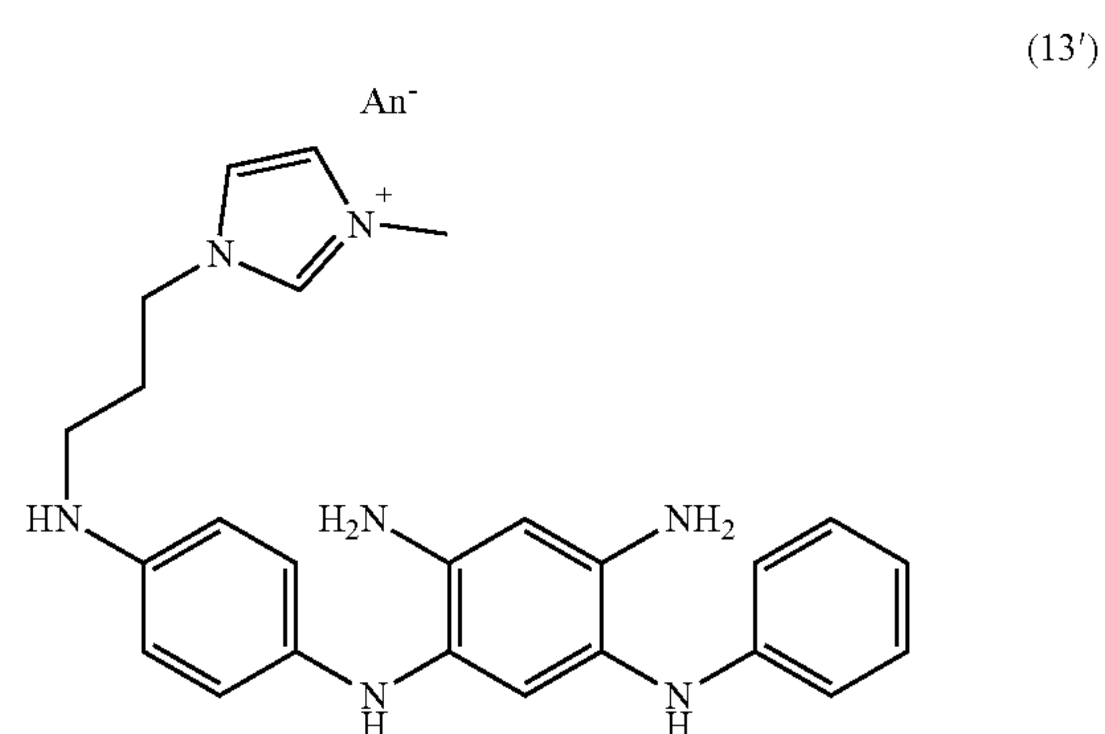
salt of 1-3-([4-([2,4-diamino-5-(phenylamino)phenyl]amino)phenyl]amino]propyl)-3-methyl-1H-imidazol-3-ium
