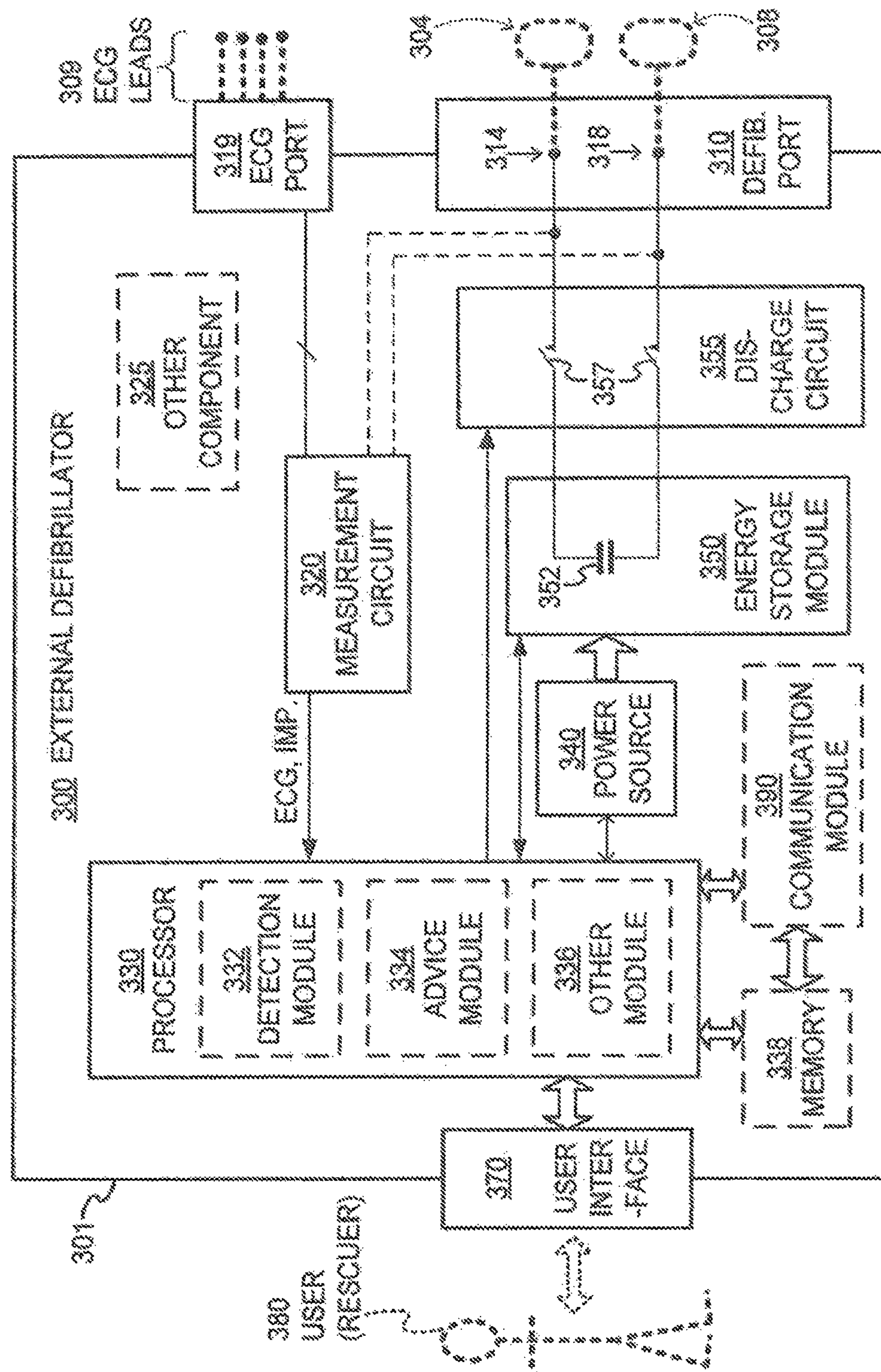
COMPONENTS OF EXTERNAL DEFIBRILLATOR
