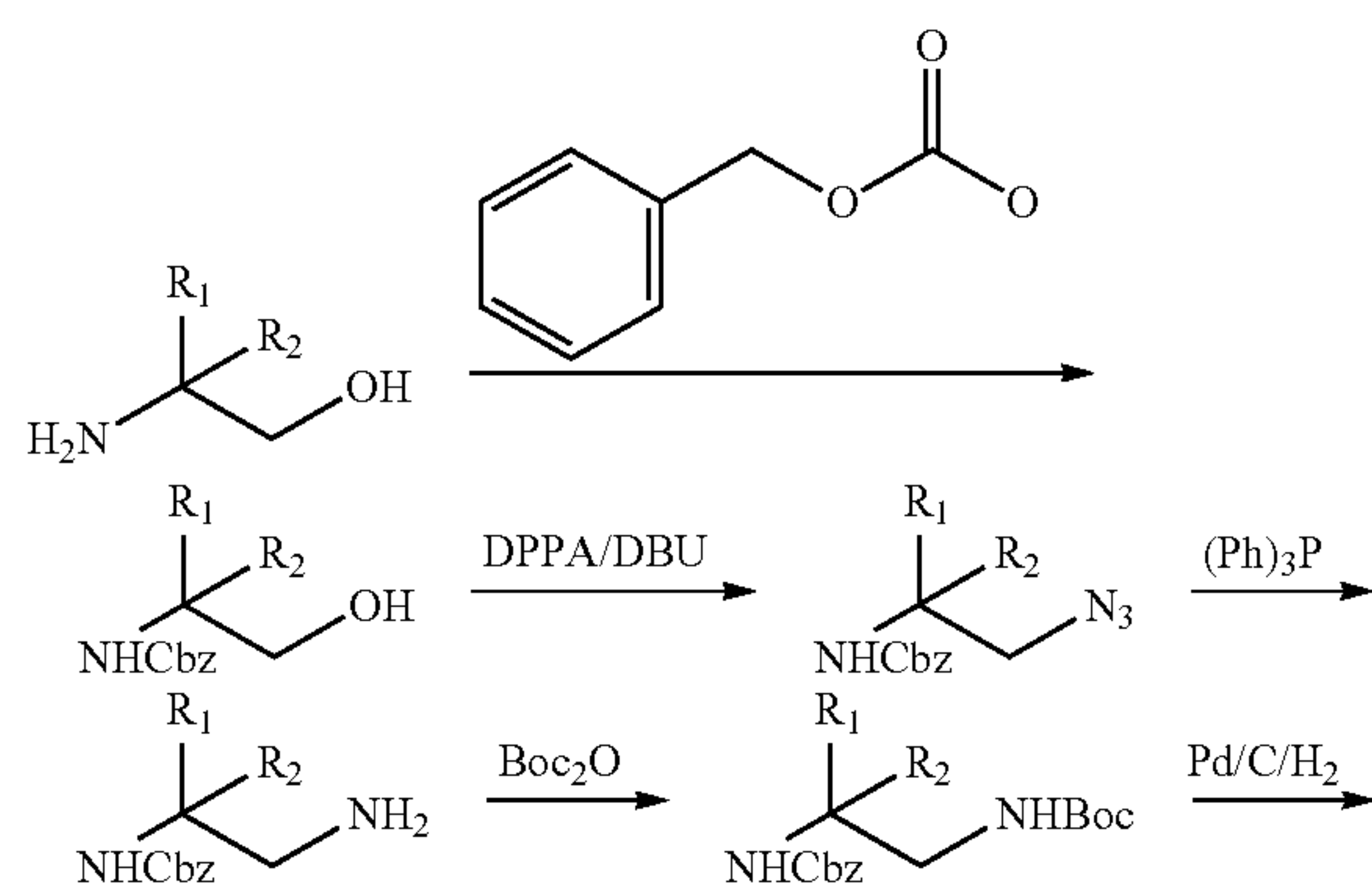
Scheme 4
