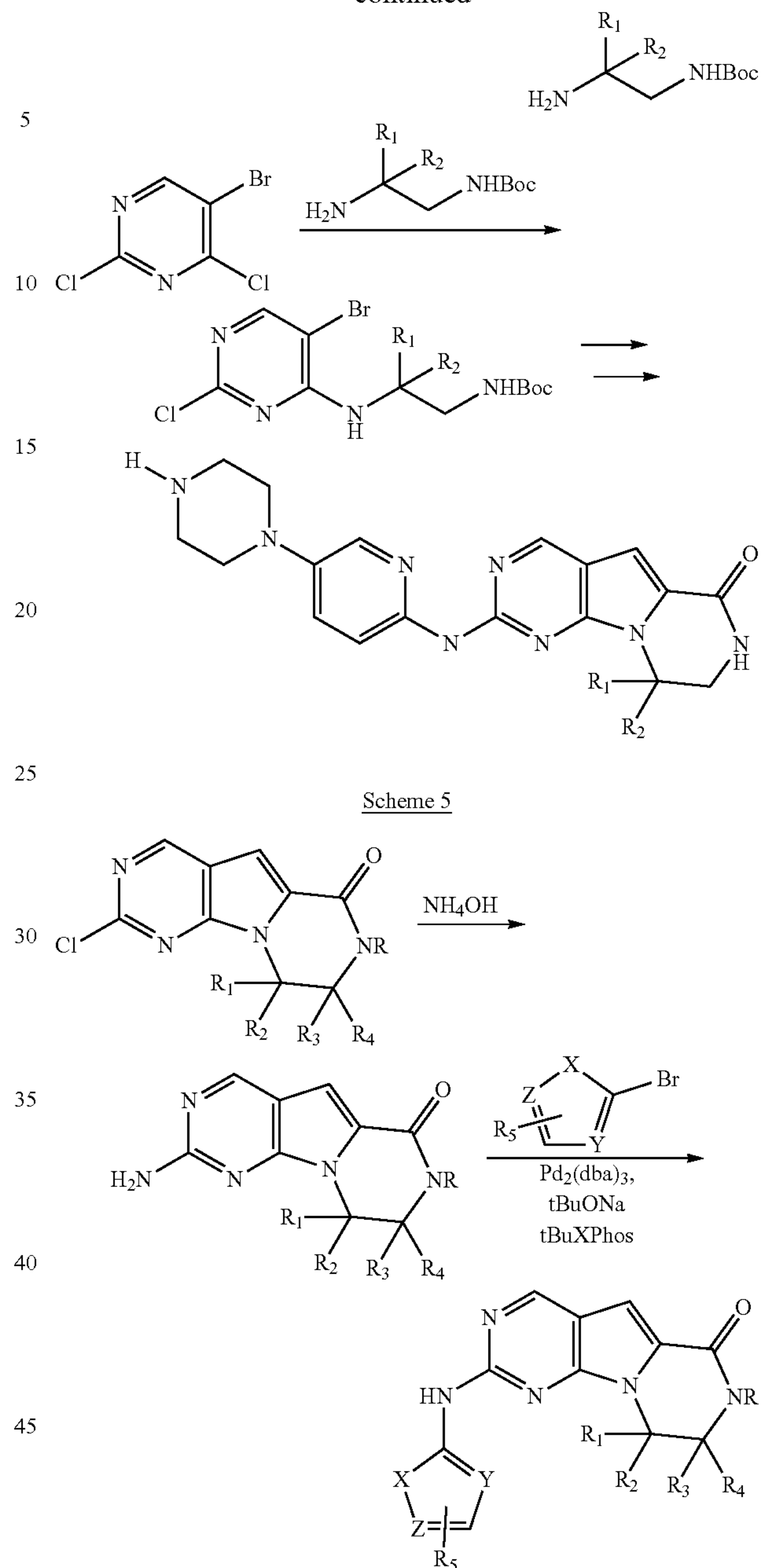
Scheme 6
