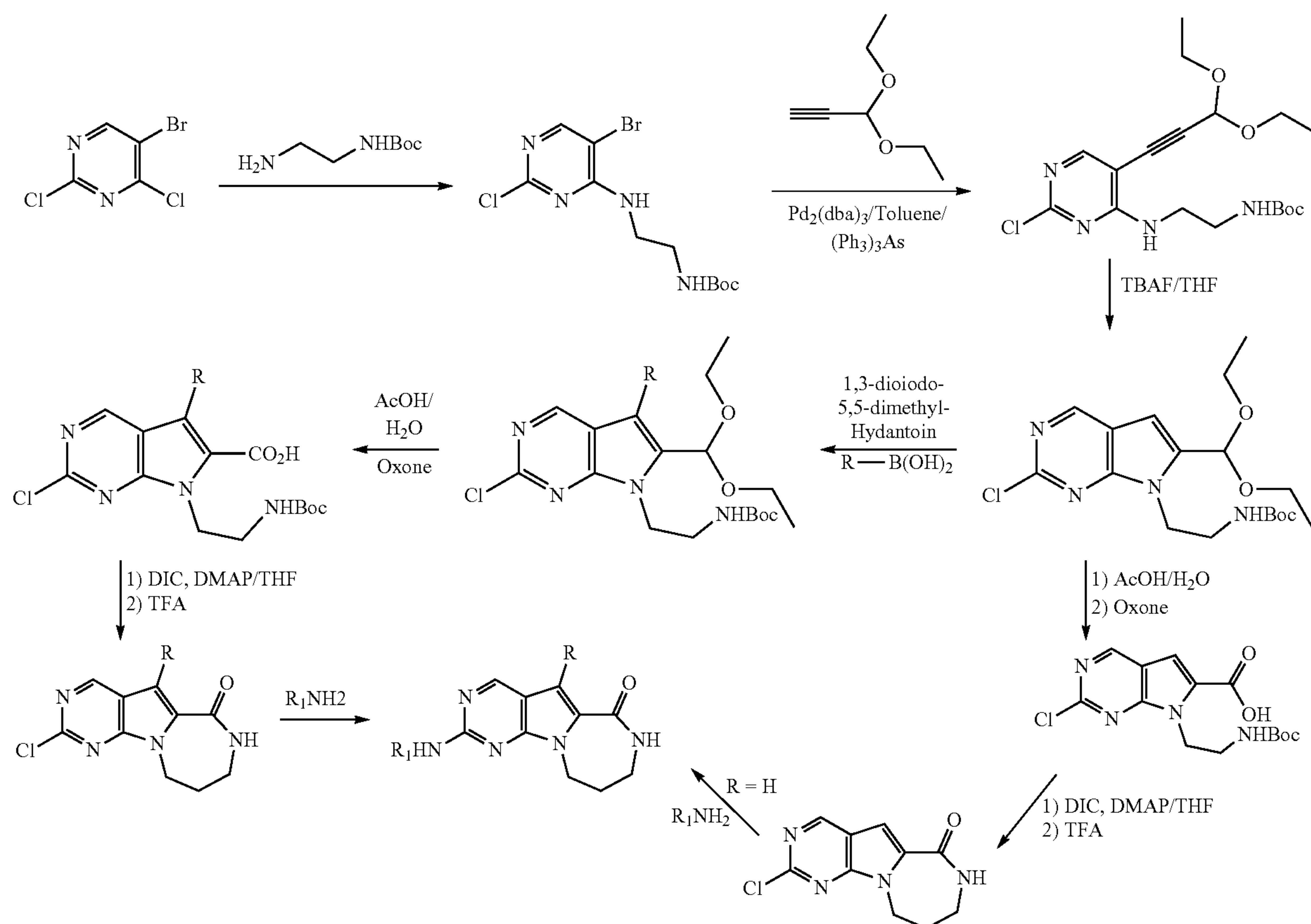
Scheme 7
