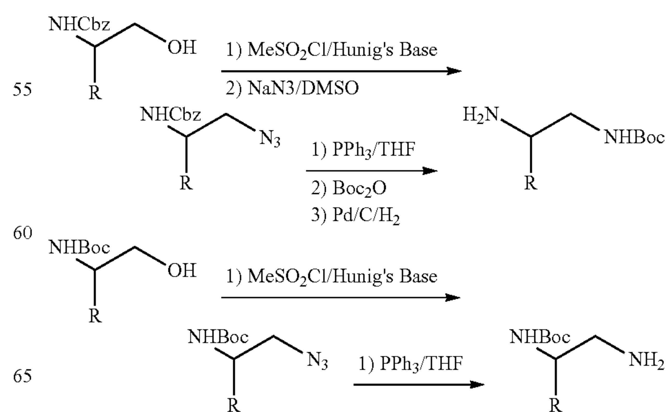
Scheme 6
