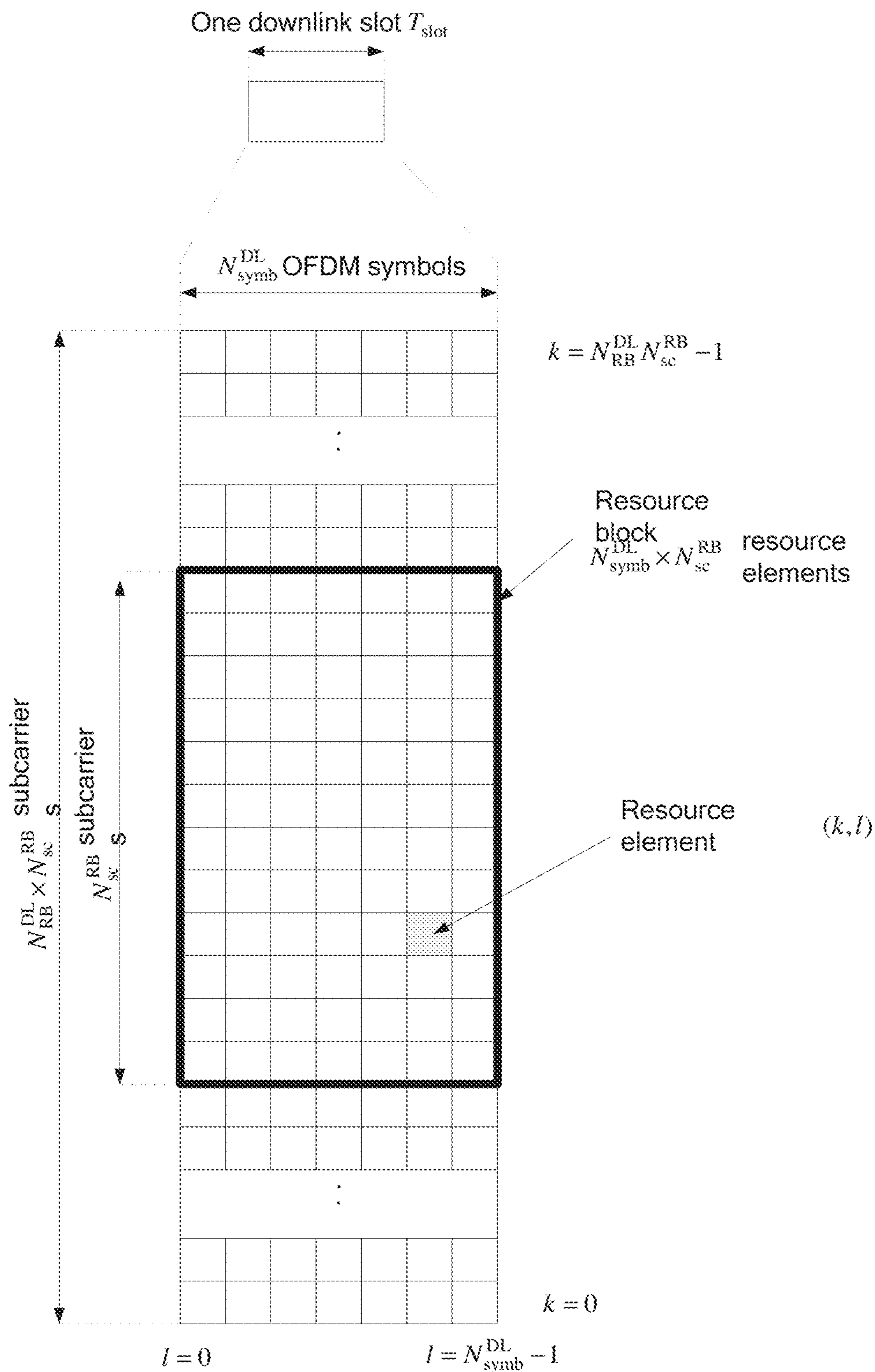
FIG. 10 (PRIOR ART)
