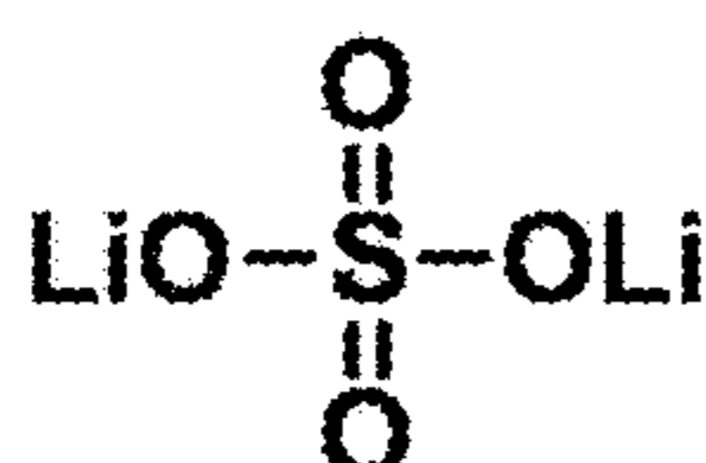
lithium sulfate
