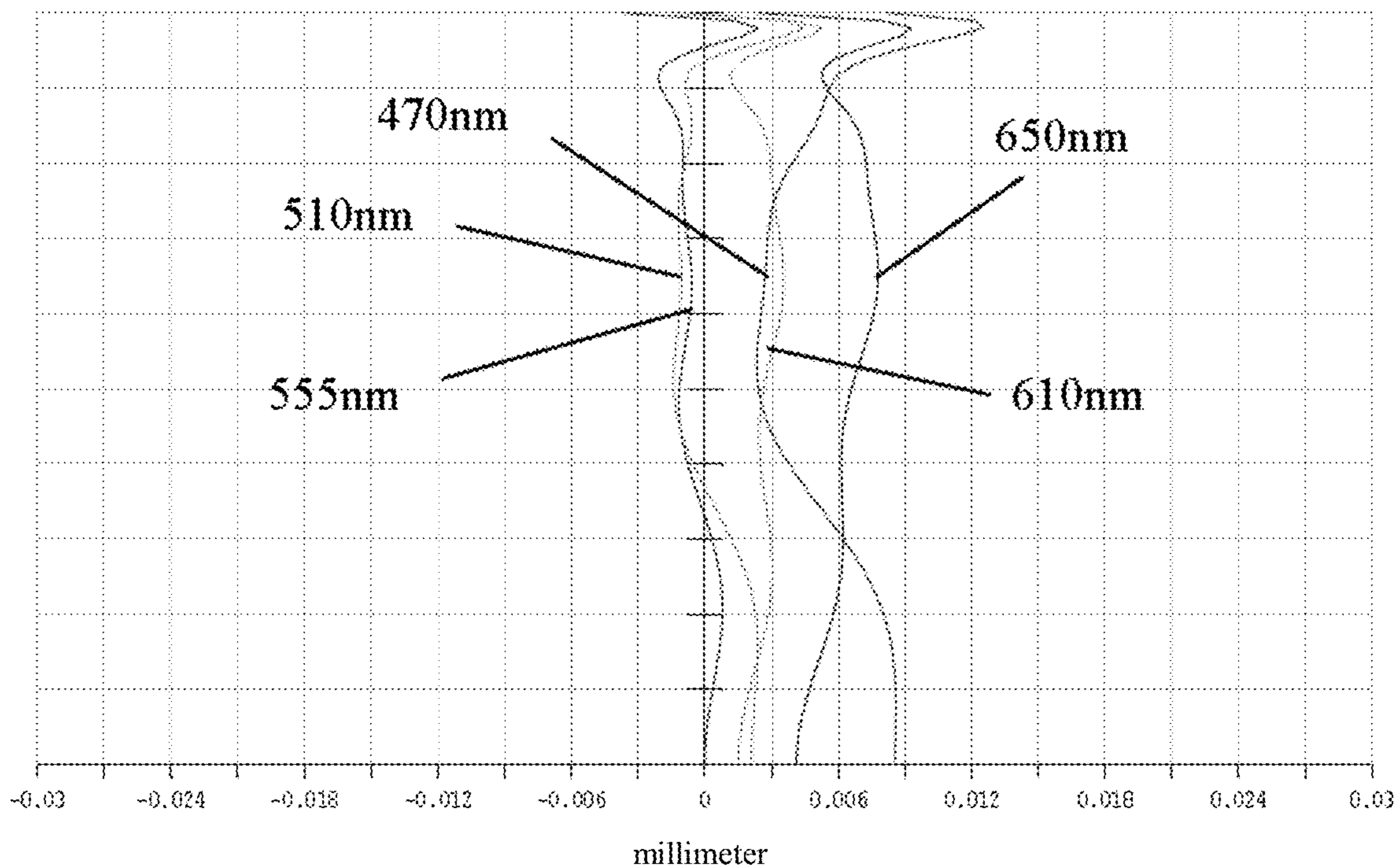
Longitudinal aberration
