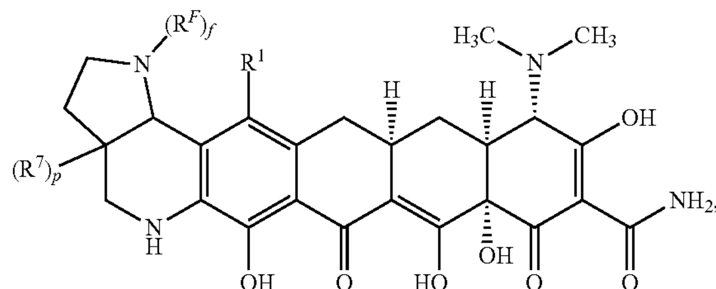
(IIa-1)
