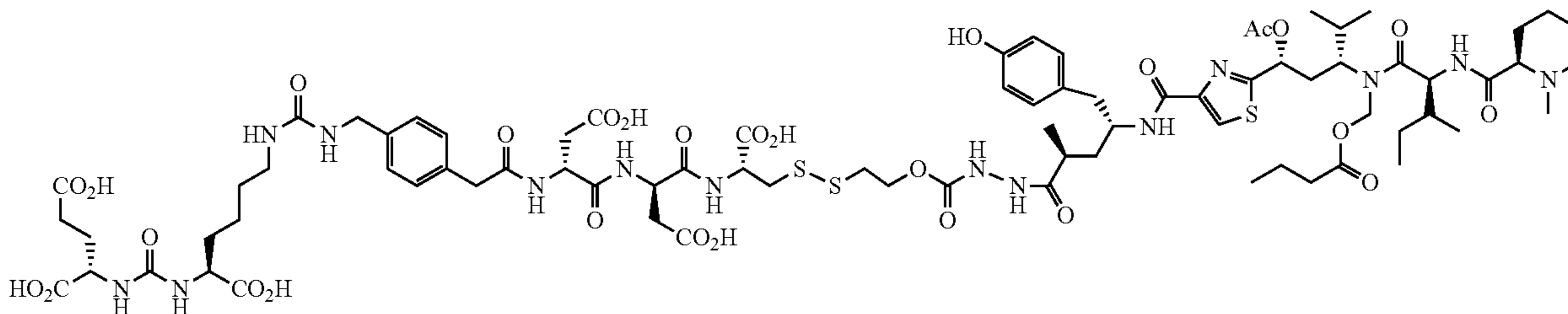
EC1169 (compound 112)
