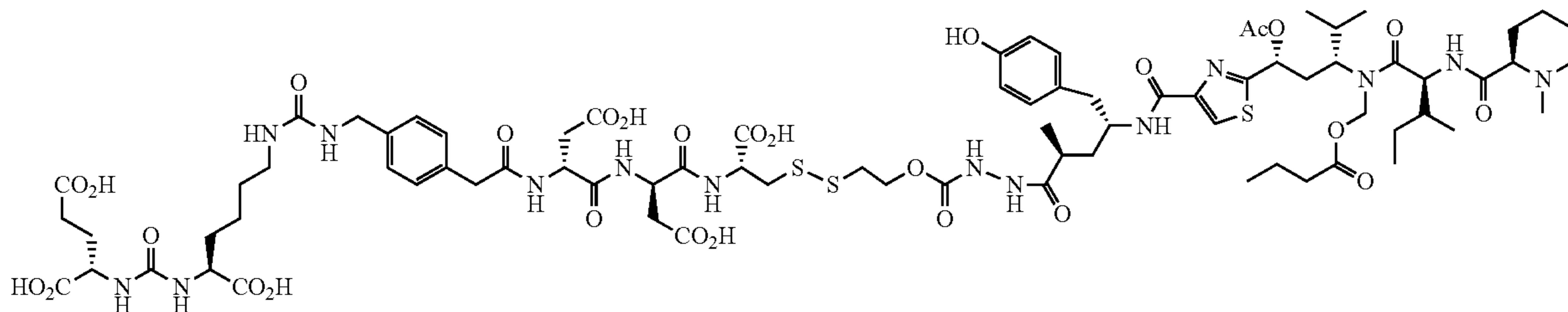
EC1169 (compound 112)
