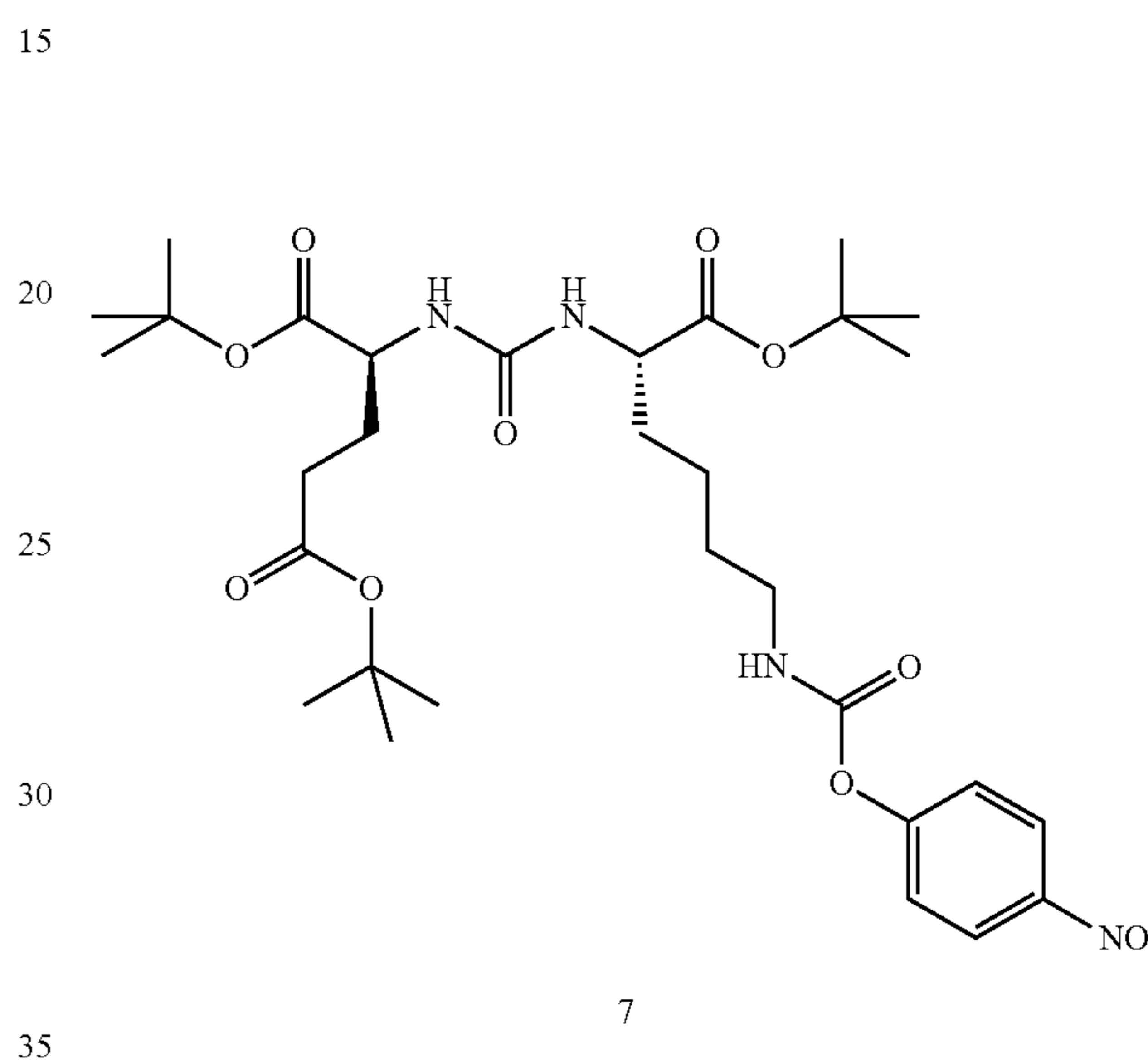
Example. Preparation of Protected Ligand 7, Including Coupling Group
