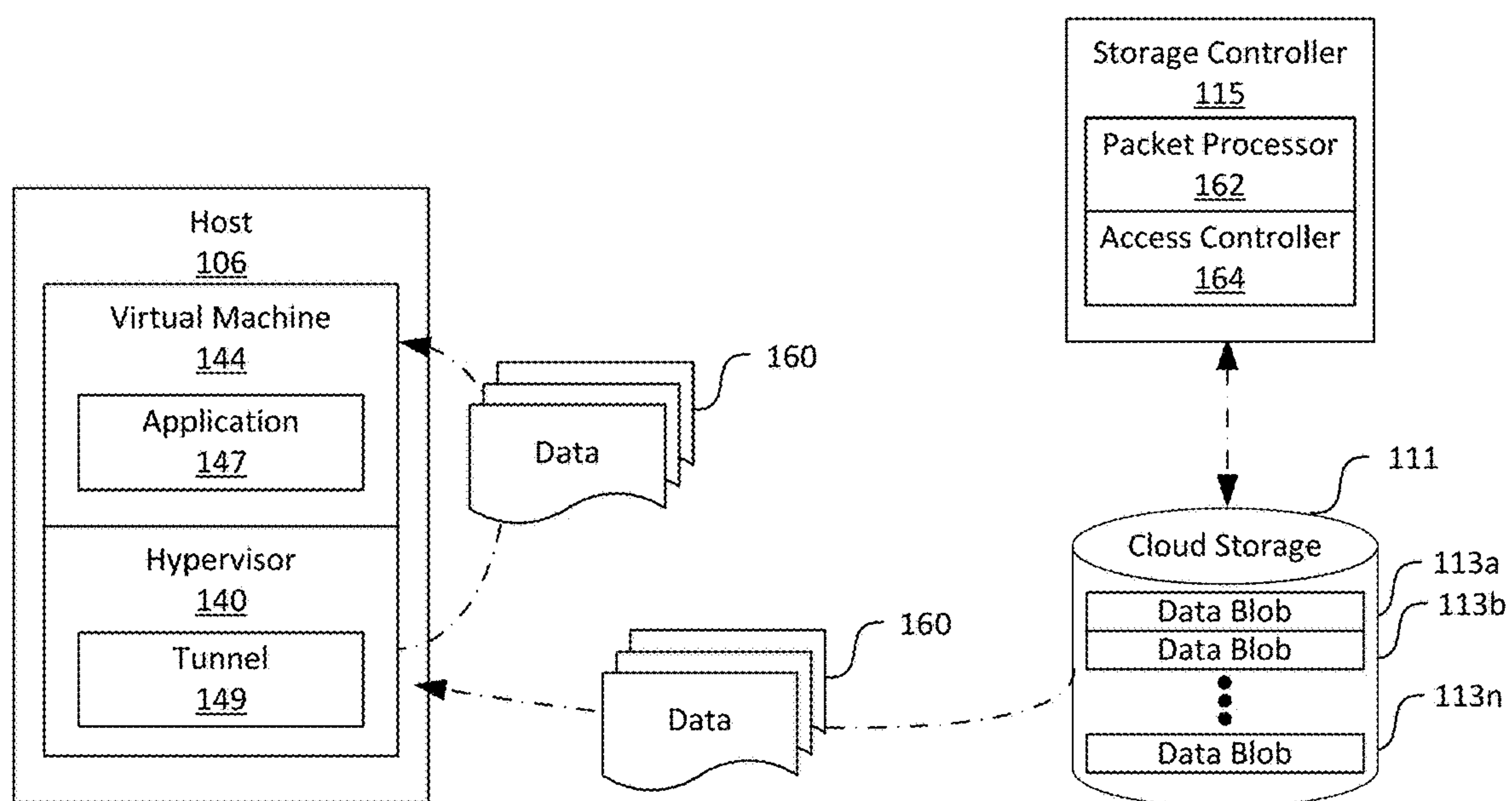
FIG. 3D
