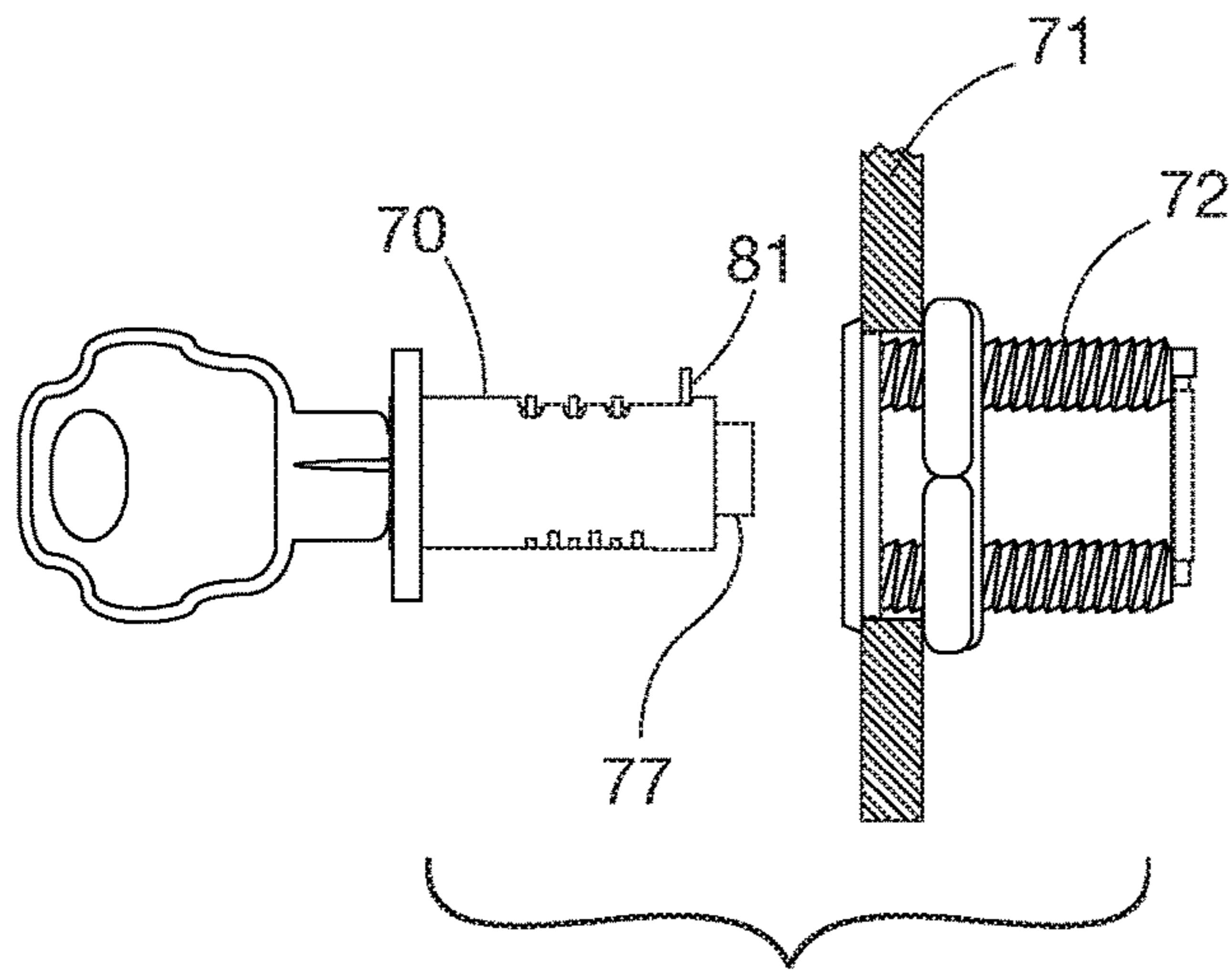
FIG. 6 (PRIOR ART)
