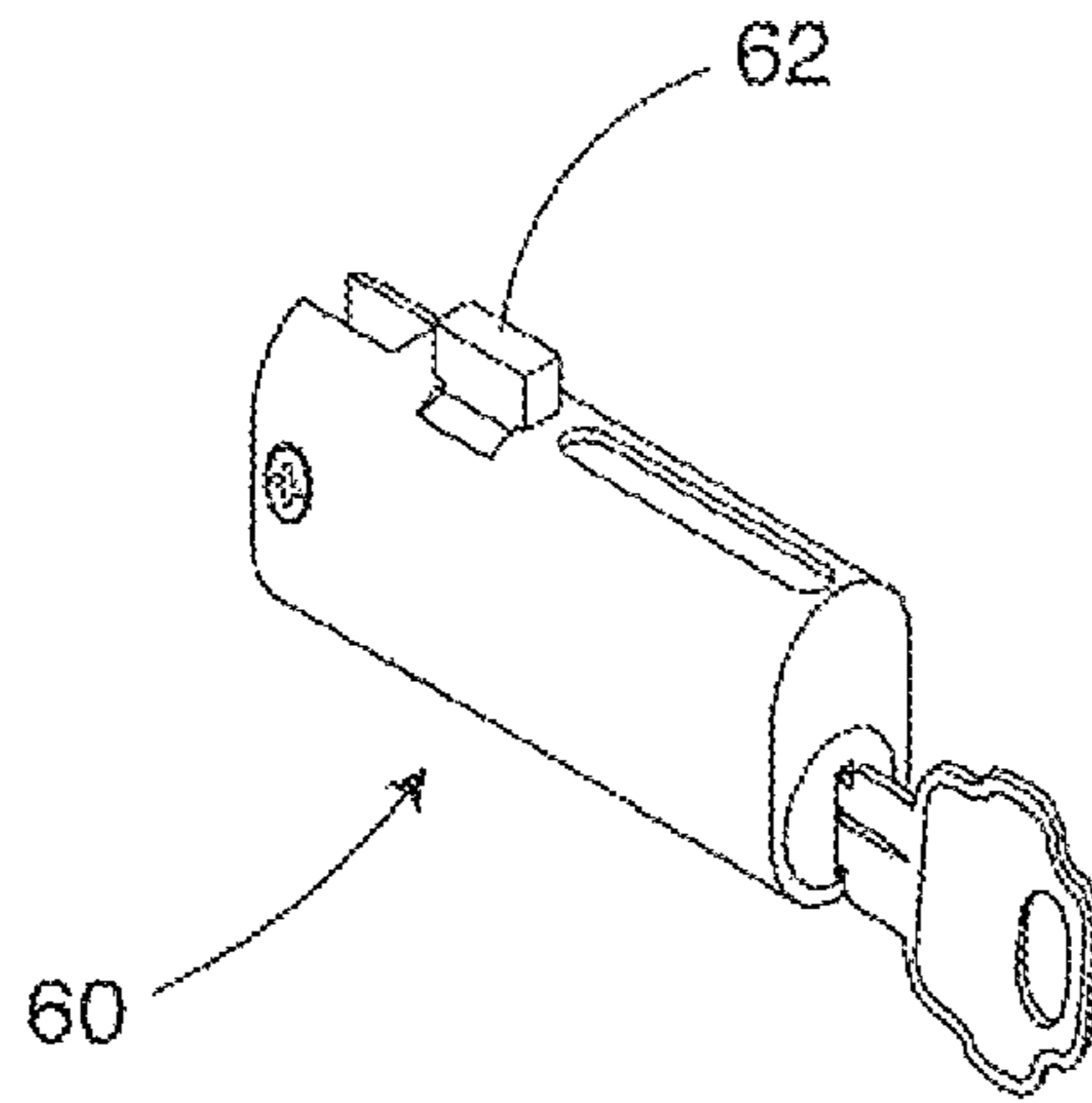
FIG. 24 (PRIOR ART)
