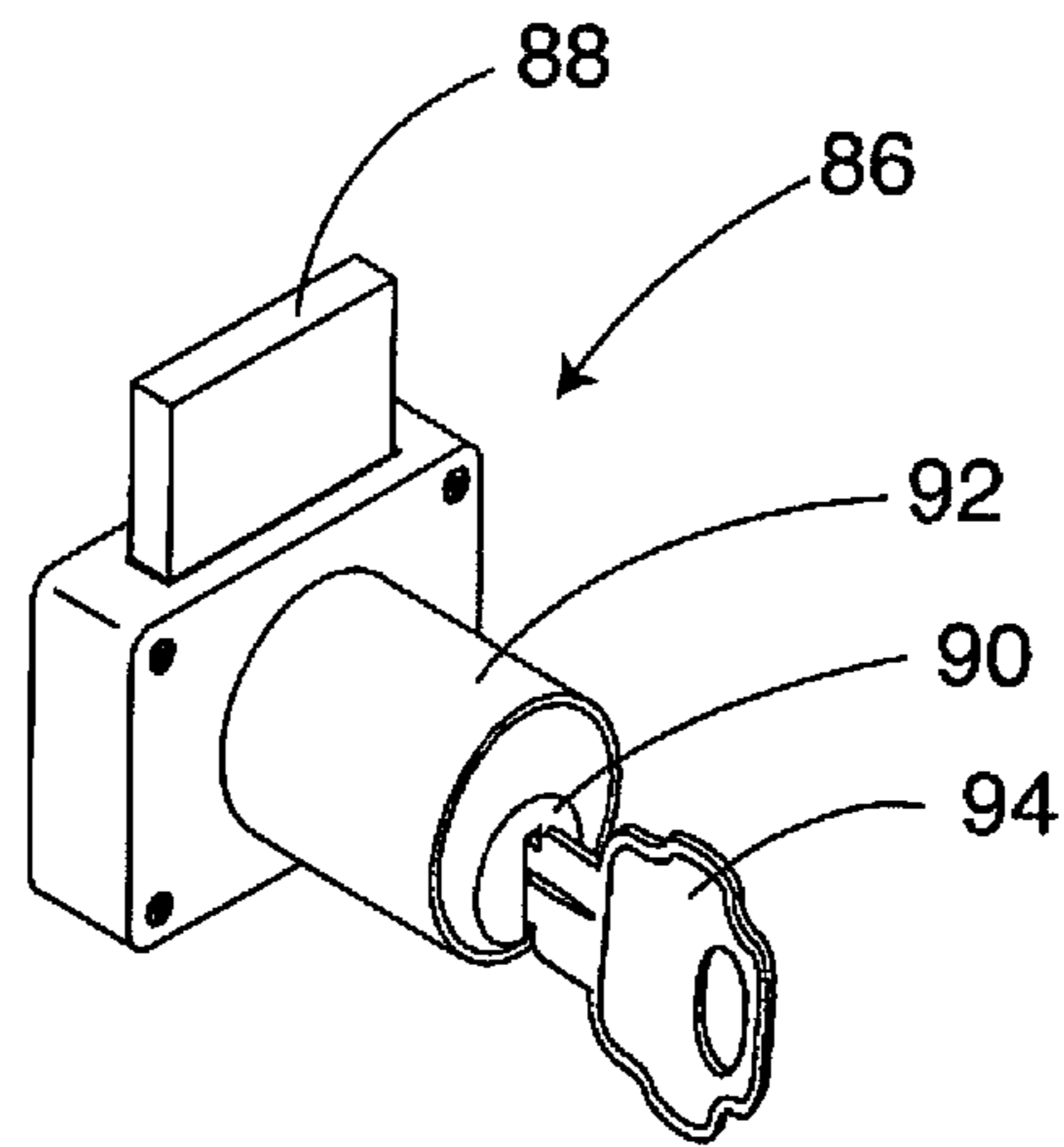
FIG. 26 (PRIOR ART)
