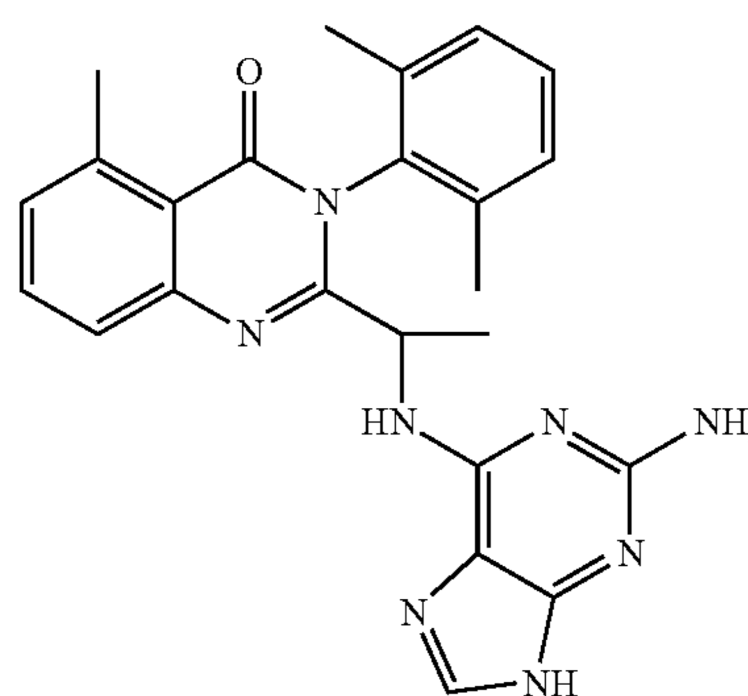
3-(2,6-dimethyl-phenyl)-5-methyl-2-[1-(9H-purin-6-ylamino)-ethyl]-3H-quinazolin-4-one (57)
