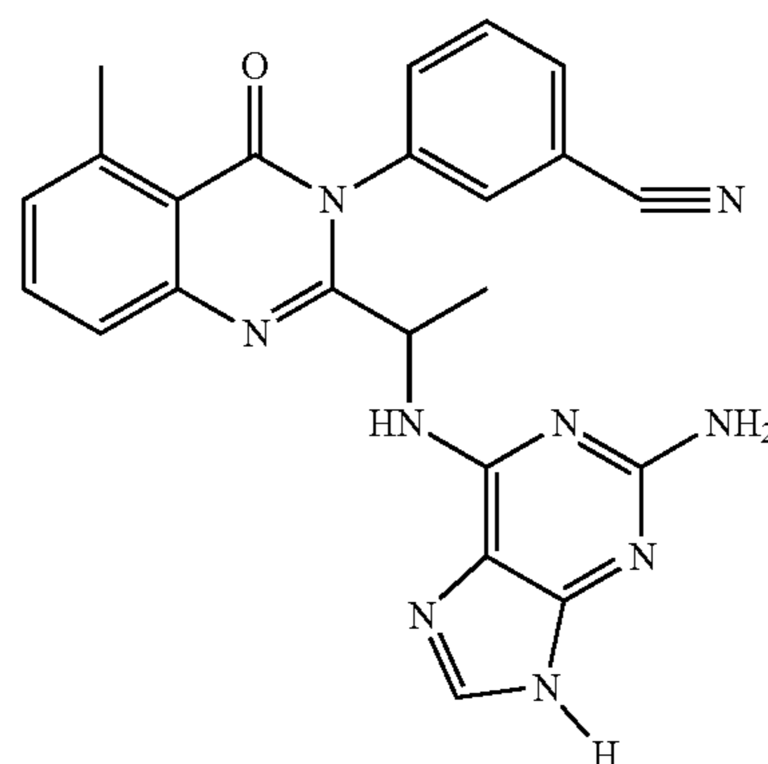
3-(2-[1-(2-Amino-9H-purin-6-ylamino)-ethyl]-5-methyl-4-oxo-4H-quinazolin-3-yl)-benzonitrile
