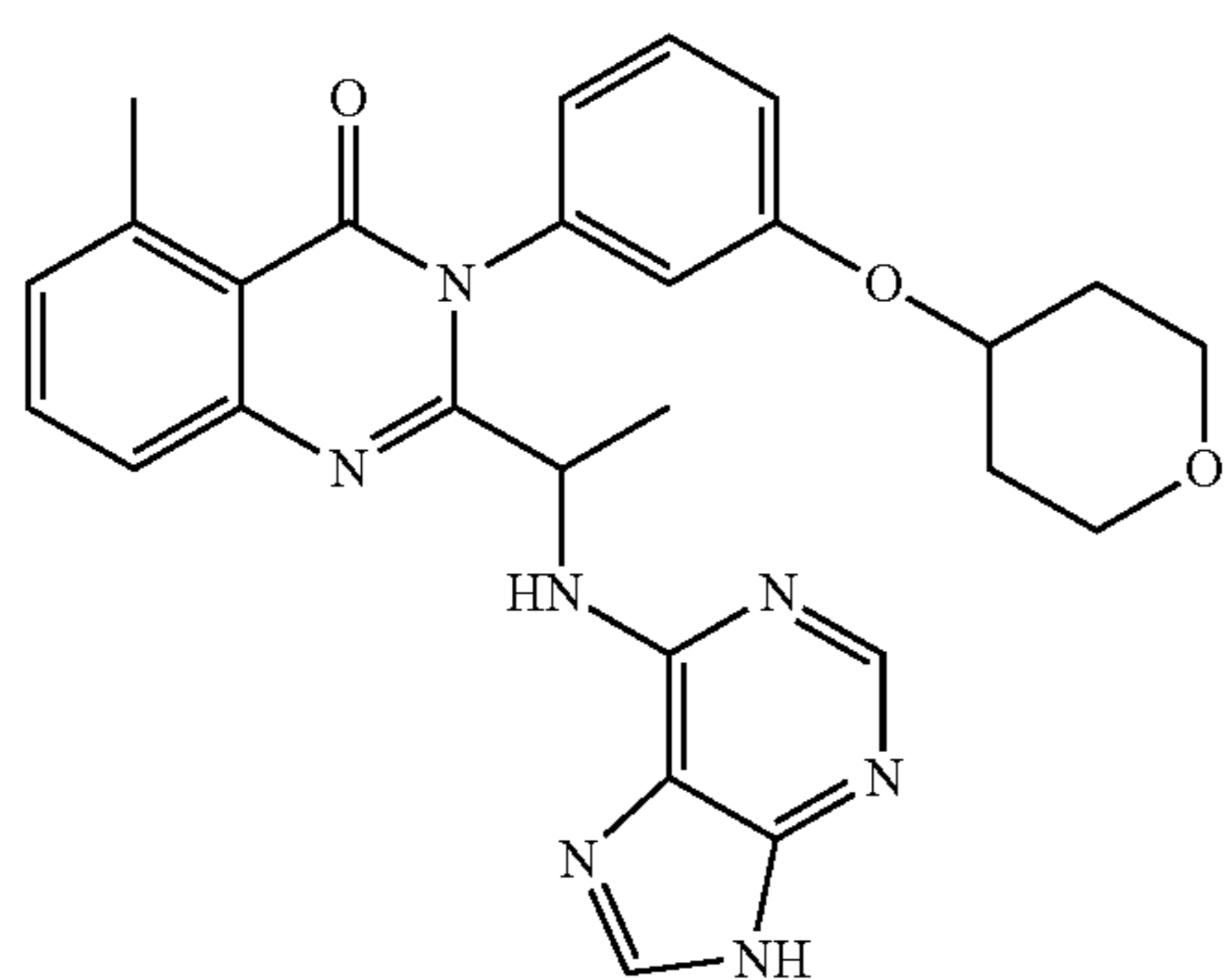
(146) 5-Methyl-2-[1-(9H-purin-6-ylamino)-ethyl]-3-[3-(tetrahydro-pyran-4-yloxy)-phenyl]-3H-quinazolin-4-one
