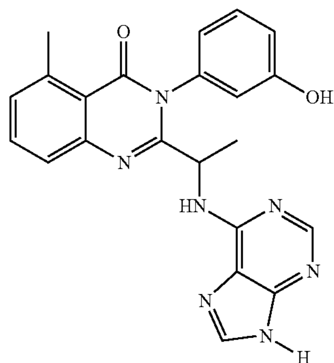
3-(3-Hydroxy-phenyl)-5-methyl-2-[1-(9H-purin-6-ylamino)-ethyl]-3H-quinazolin-4-one
