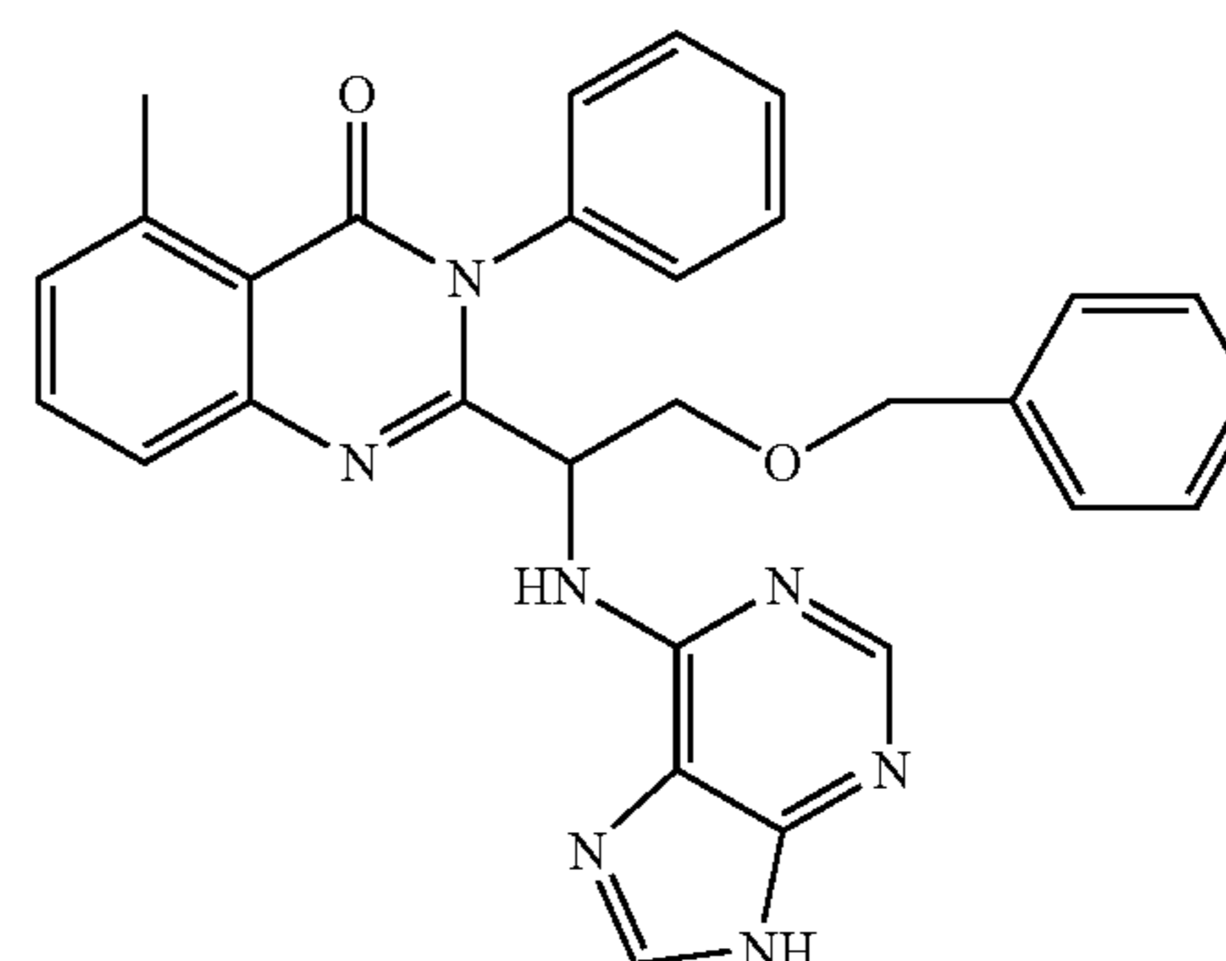
2-(1-(2-amino-9H-purin-6-ylamino)-2-benzyloxyethyl)-5-methyl-3-phenyl-3H-quinazolin-4-one (29)
