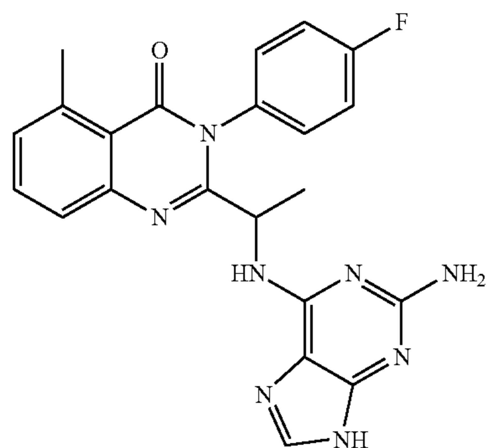
3-(4-fluoro-phenyl)-2-[1-(2-fluoro-9H-purin-6-ylamino)-ethyl]-5-methyl-3H-quinazolin-4-one (34)
