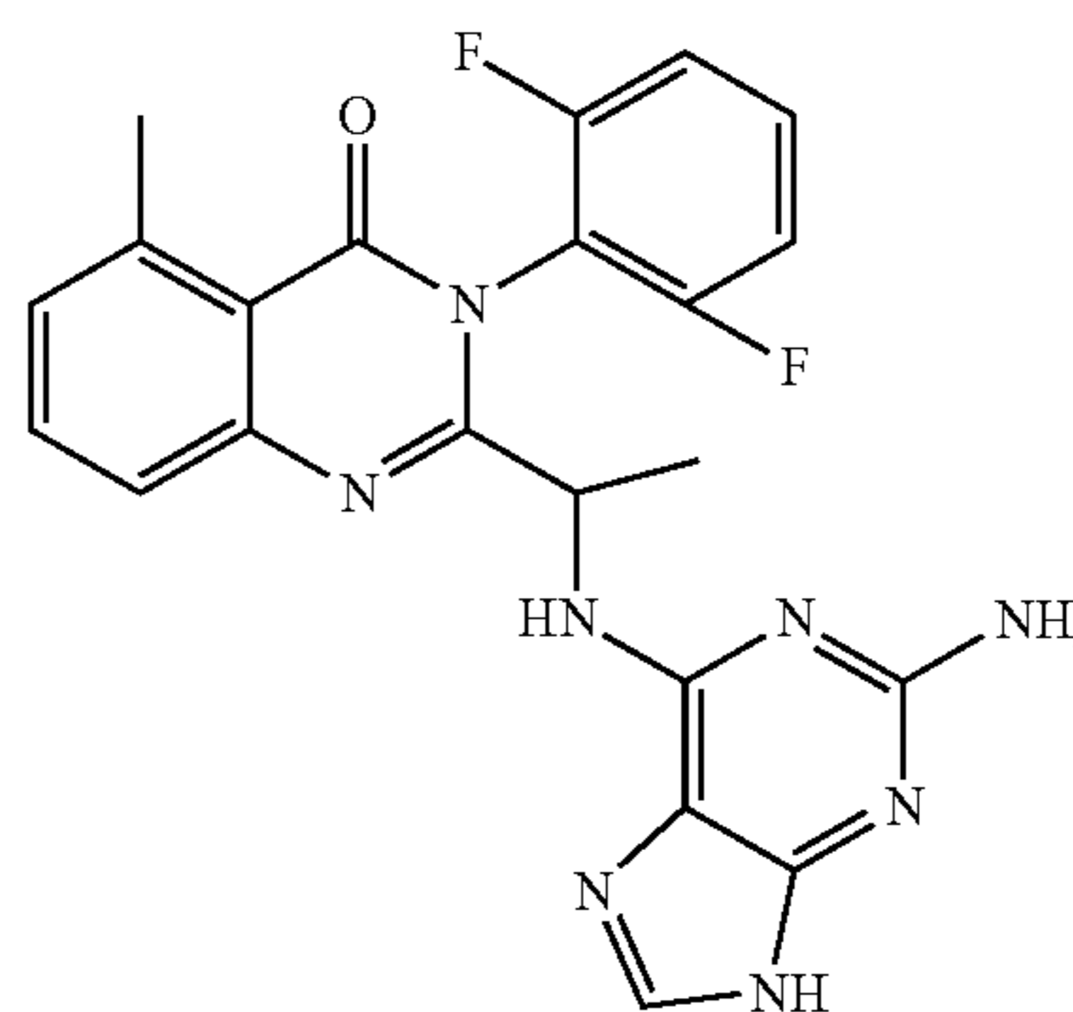
3-(3,5-dichloro-phenyl)-5-methyl-2-[1-(9H-purin-6-ylamino)-ethyl]-3H-quinazolin-4-one (79)
