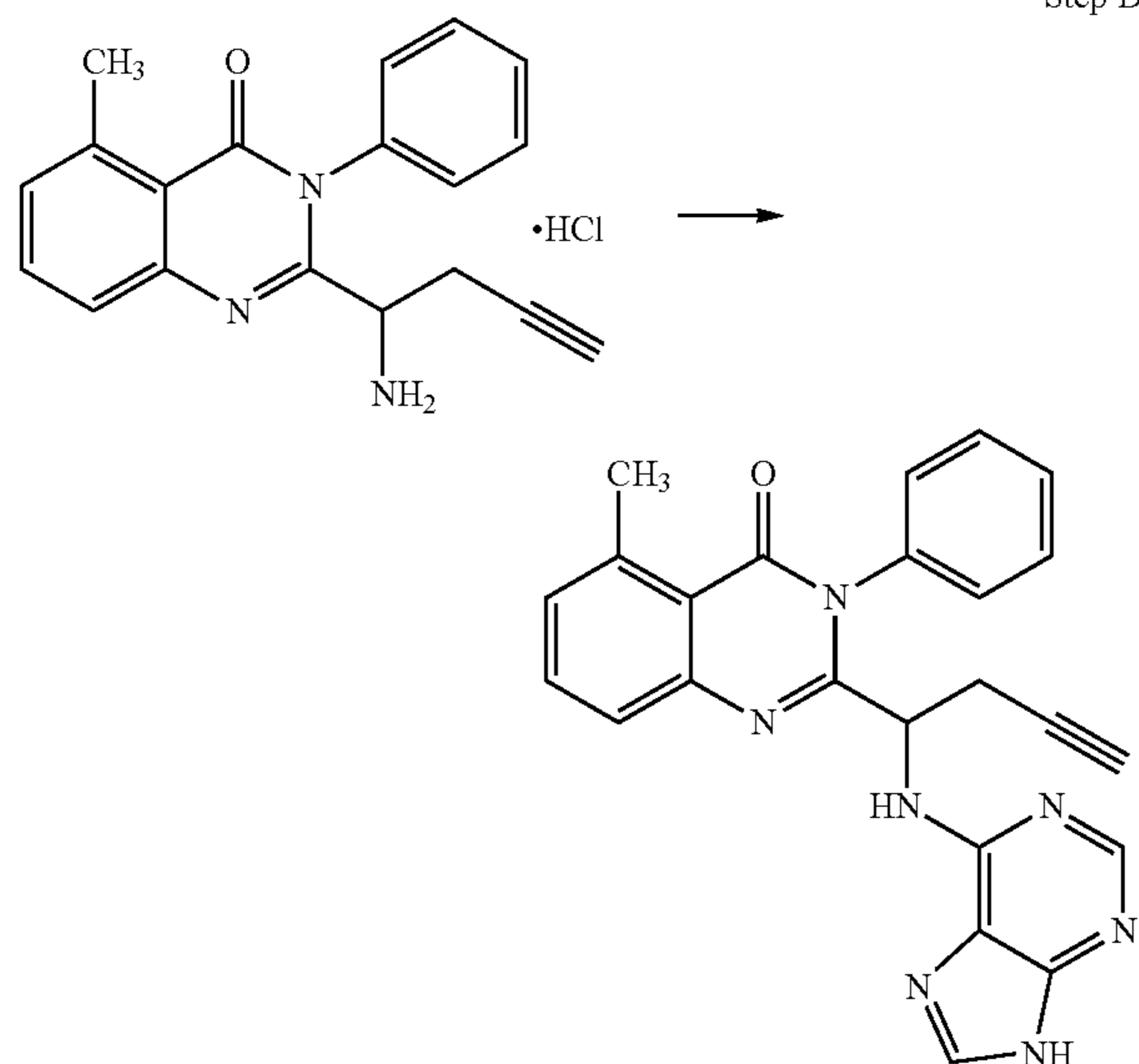
2-[1-(2-amino-9H-purin-6-ylamino)-but-3-ynyl]-5-methyl-3-phenyl-3H-quinazolin-4-one (161)
