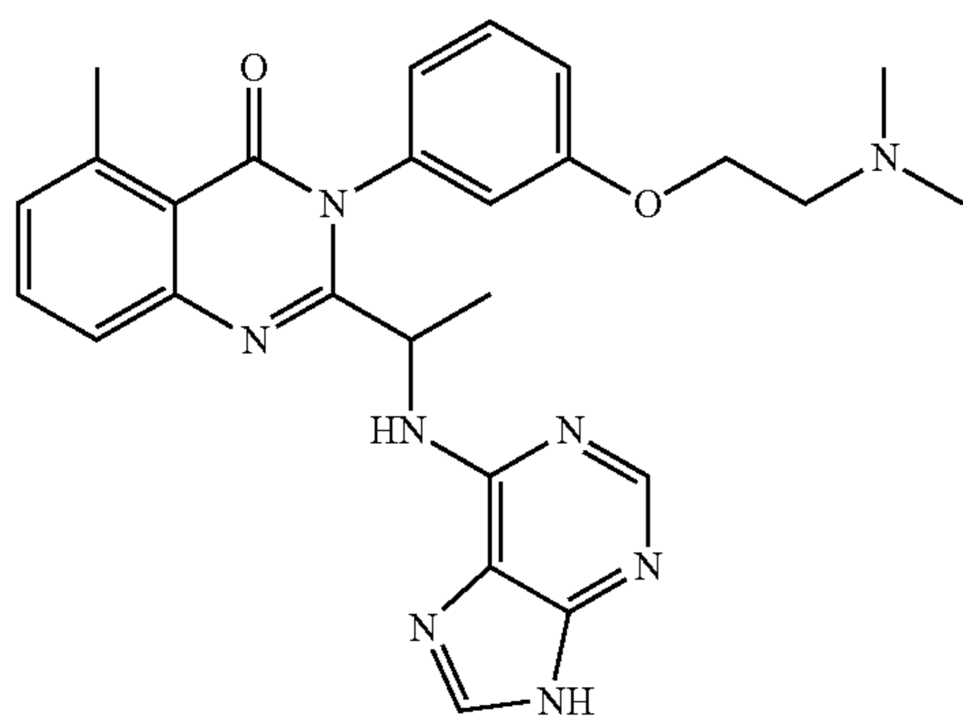
3-[3-(2-Dimethylamino-ethoxy)-phenyl]-5-2-[1-(9H-purin-6-ylamino)-ethyl]-3H-quinazolin-4-one
