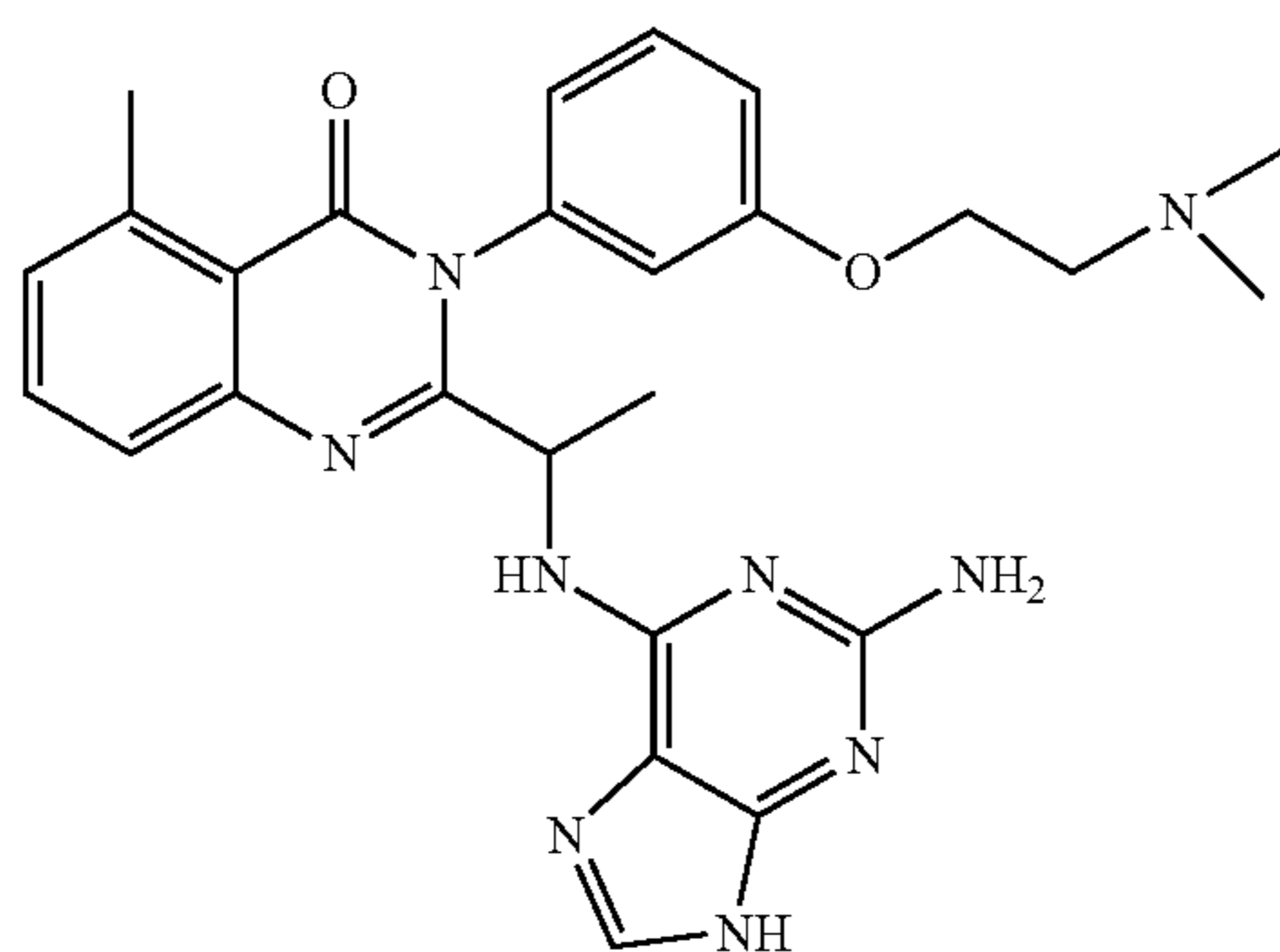
2-[1-(2-Amino-9H-purin-6-ylamino)-ethyl]-3-[3-(2-dimethylamino-ethoxy)-phenyl]-5-methyl-3H-quinazolin-4-one
