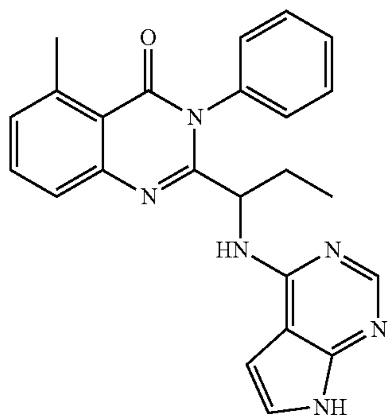
2-[1-(2-fluoro-9H-purin-6-ylamino)-propyl]-5-methyl-3-phenyl-3H-quinazolin-4-one (25)
