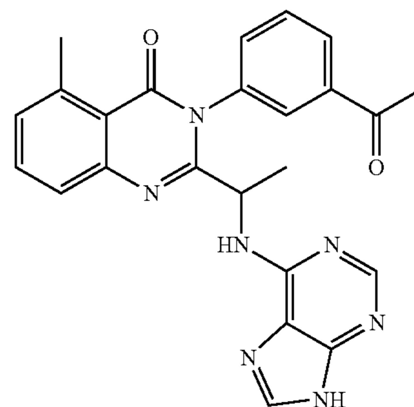
3-(3-Acetyl-phenyl)-5-methyl-2-[1-(9H-purin-6-ylamino)-ethyl]-3H-quinazolin-4-one
