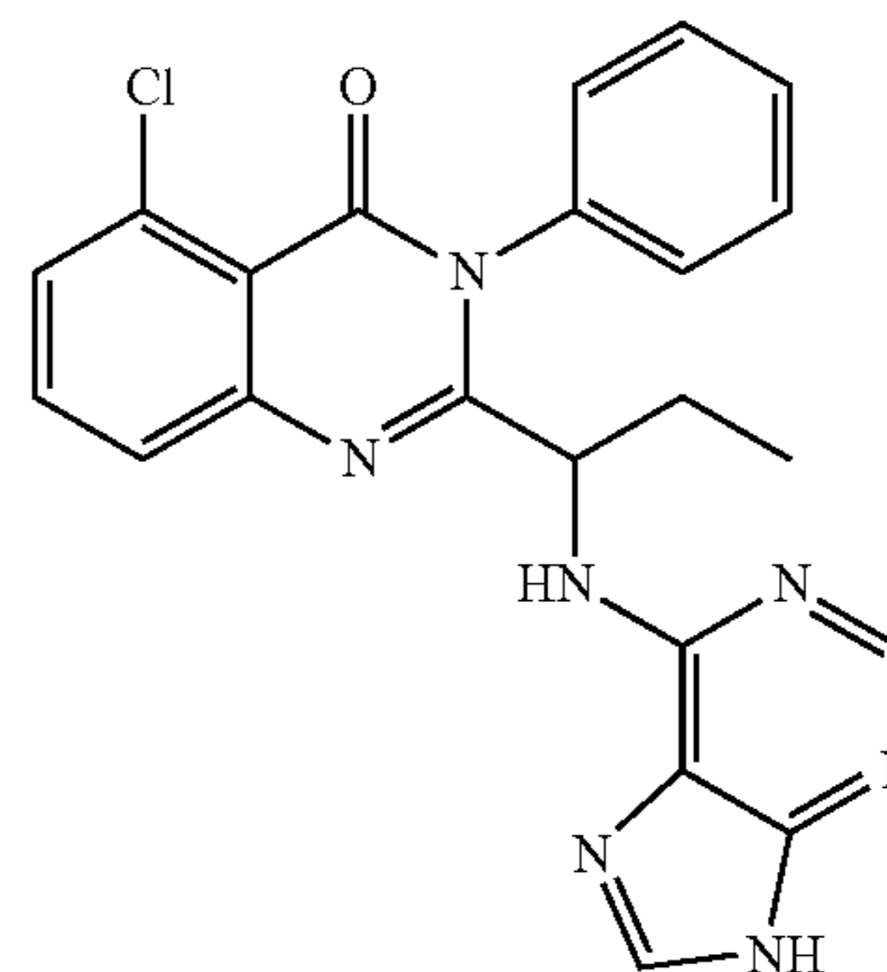
2-[1-(2-amino-9H-purin-6-ylamino)-propyl]-5-chloro-3-phenyl-3H-quinazolin-4-one (83)
