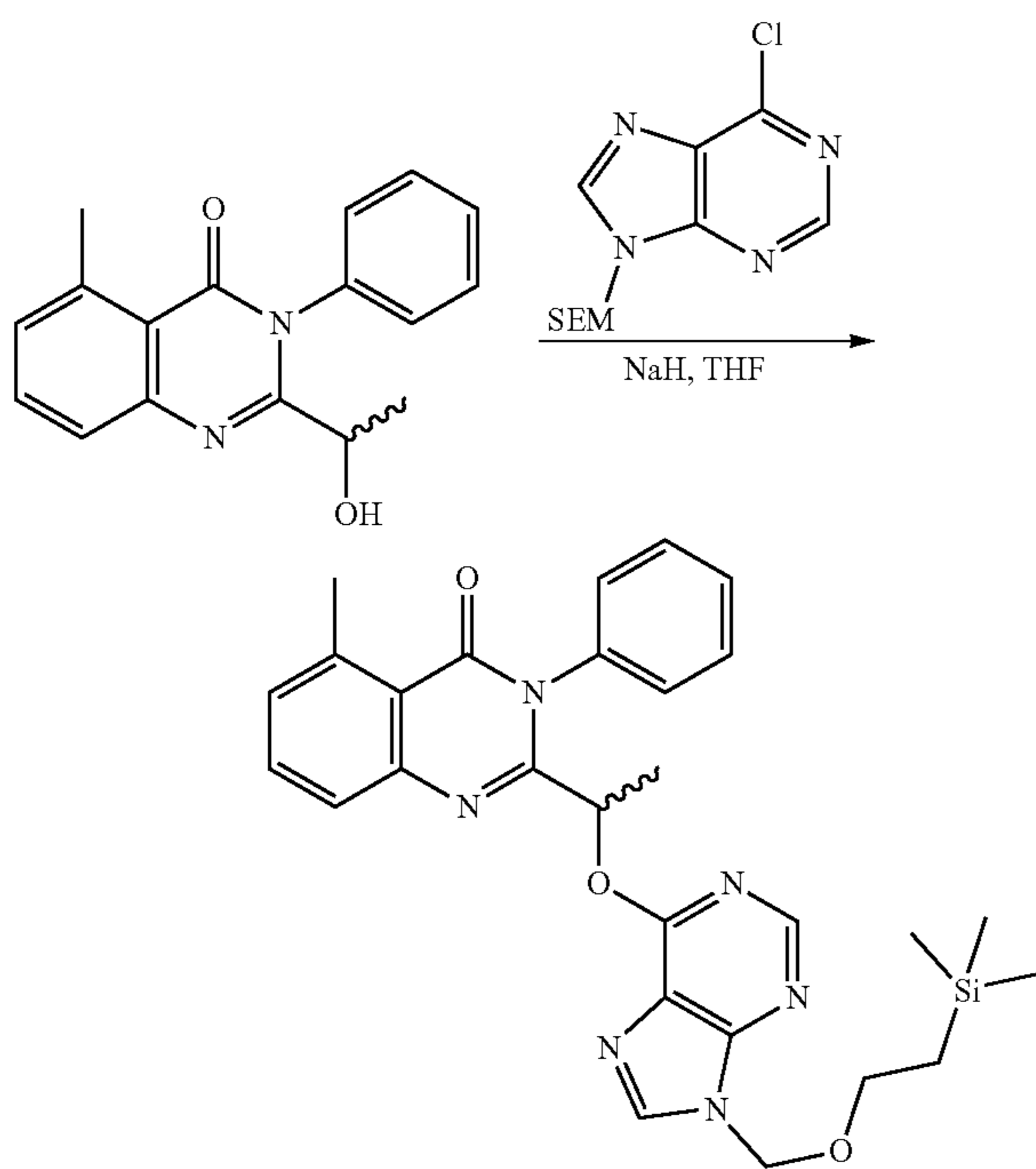
5-Methyl-3-phenyl-2-[1-(9H-purin-6-yl)oxy]ethyl-3H-quinazolin-4-one (176)
