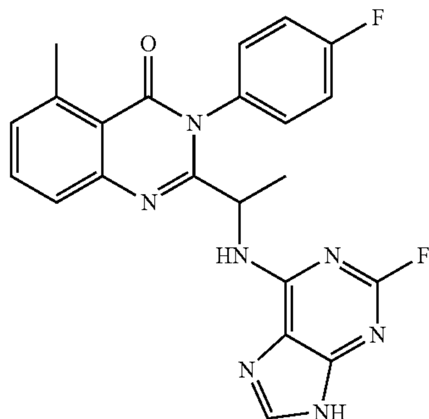
3-(4-fluoro-phenyl)-5-methyl-2-[1-(7H-pyrrolo[2,3-d]pyrimidin-4-ylamino)-ethyl]-3H-quinazolin-4-one (35)
