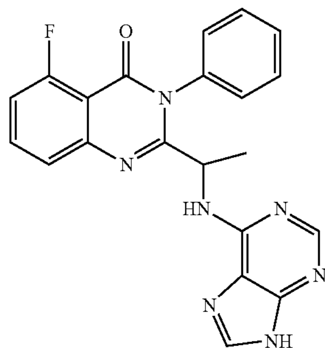
2-[1-(2-amino-9H-purin-6-ylamino)-ethyl]-5-fluoro-3-phenyl-3H-quinazolin-4-one (47)
