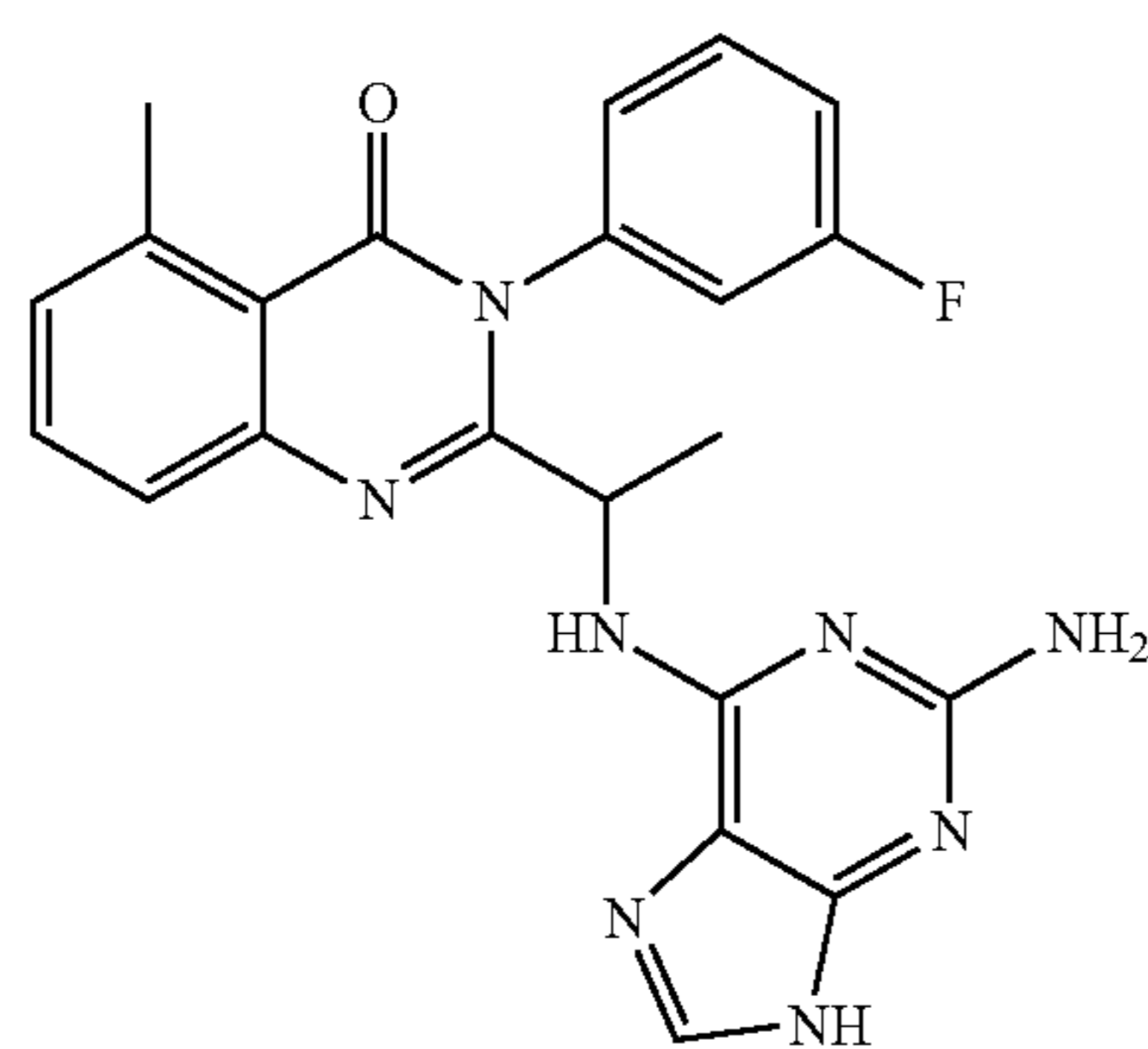
3-(3-fluoro-phenyl)-5-methyl-2-[1-(7H-pyrrolo[2,3-d]pyrimidin-4-ylamino)-ethyl]-3H-quinazolin-4-one (39)
