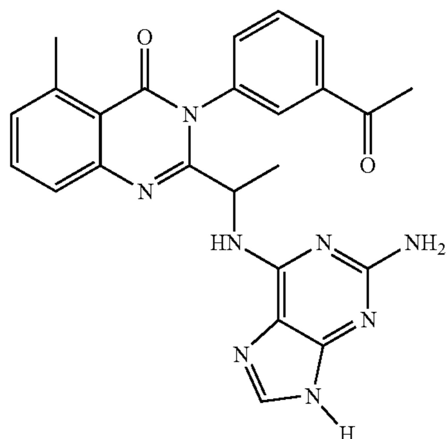
3-(3-Acetyl-phenyl)-2-[1-(2-amino-9H-purin-6-ylamino)-ethyl]-5-methyl-3H-quinazolin-4-one
