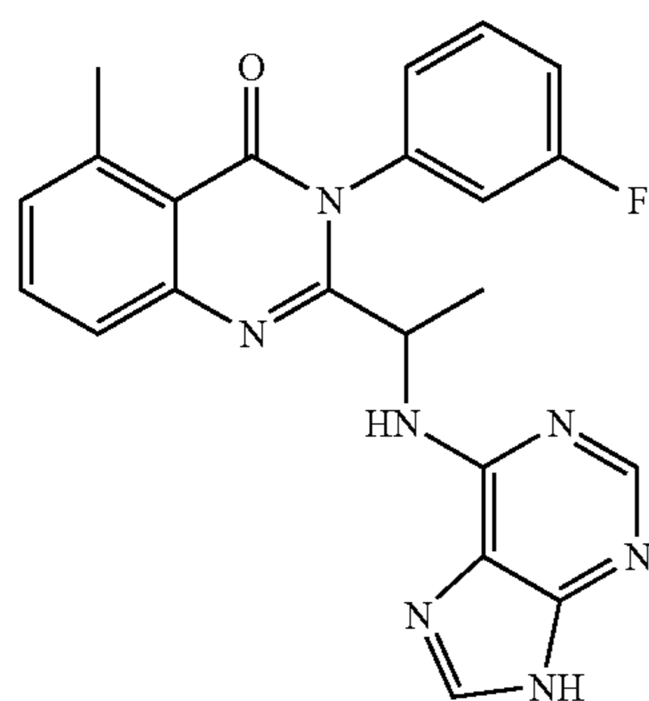
2-[1-(2-amino-9H-purin-6-ylamino)-ethyl]-3-(3-fluoro-phenyl)-5-methyl-3H-quinazolin-4-one (38)
