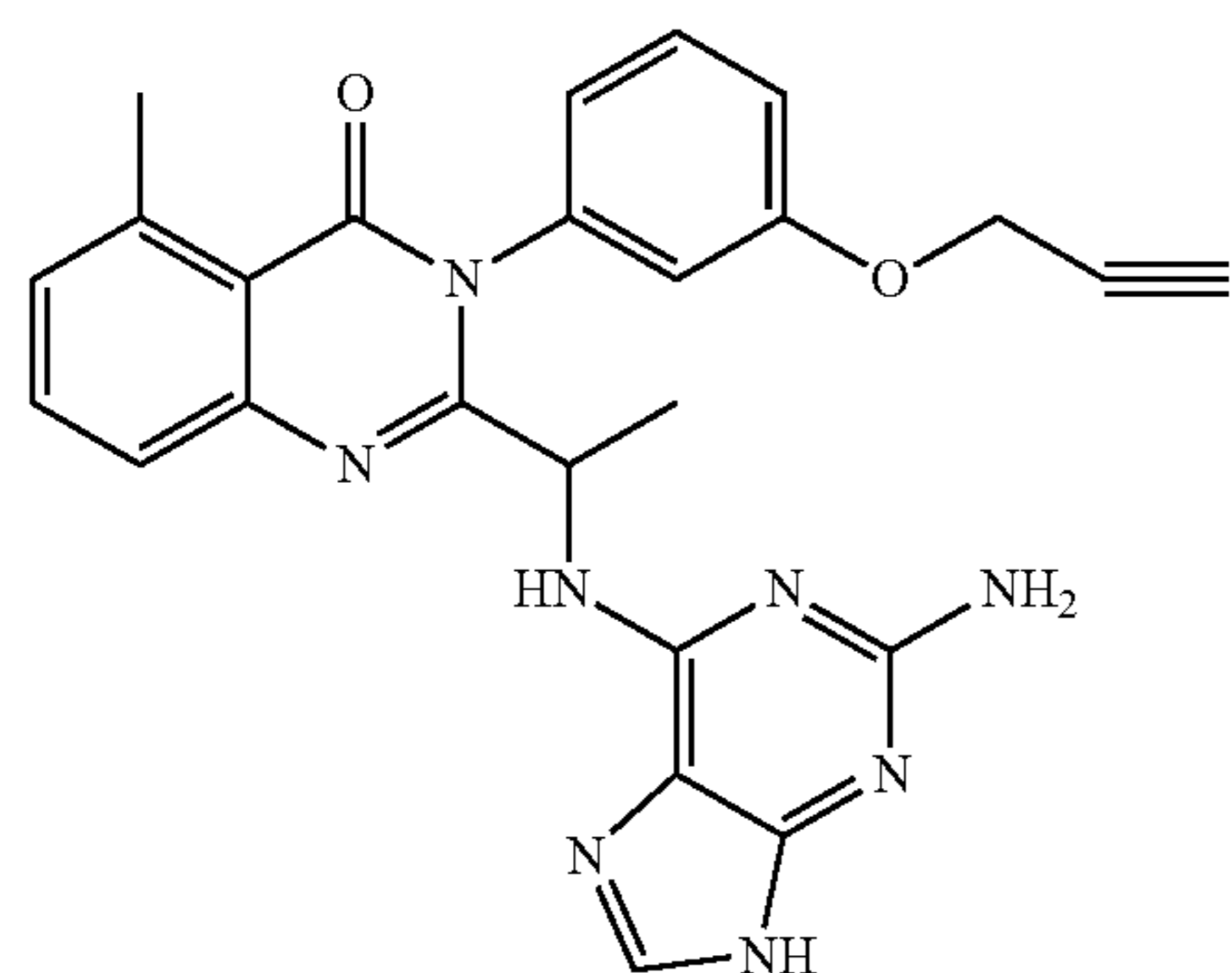
2-[1-(2-Amino-9H-purin-6-ylamino)-ethyl]- 5-methyl-3-(3-prop-2-ynyloxy-phenyl)-3H-quinazolin-4-one
