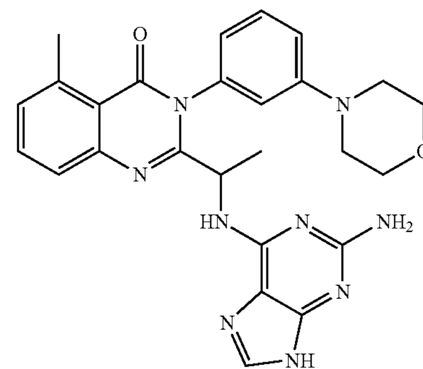
2-[1-(2-Amino-9H-purin-6-ylamino)-ethyl]-5-methyl-3-(3-morpholin-4-yl-phenyl)-3H-quinazolin-4-one
