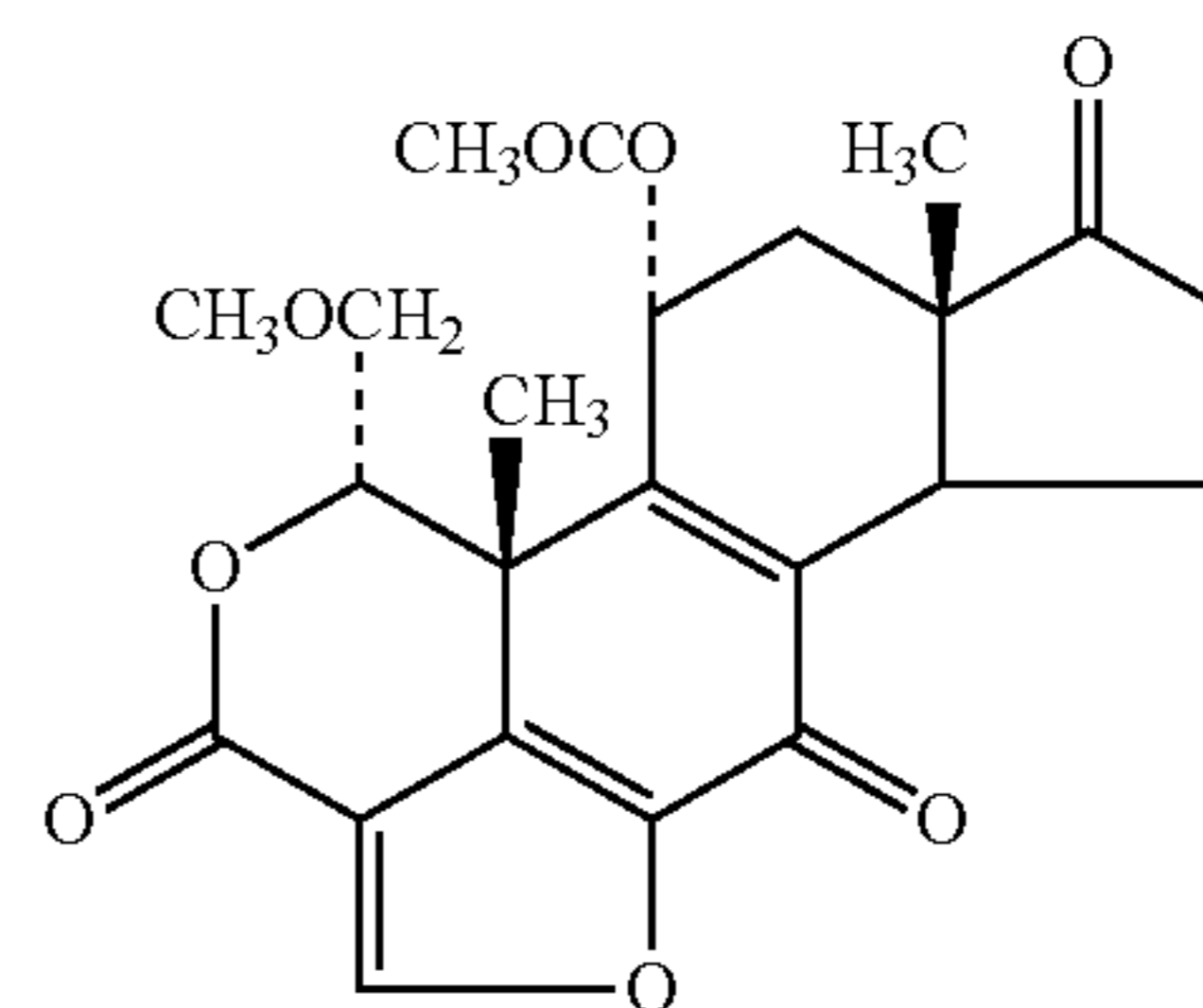
wortmannin
