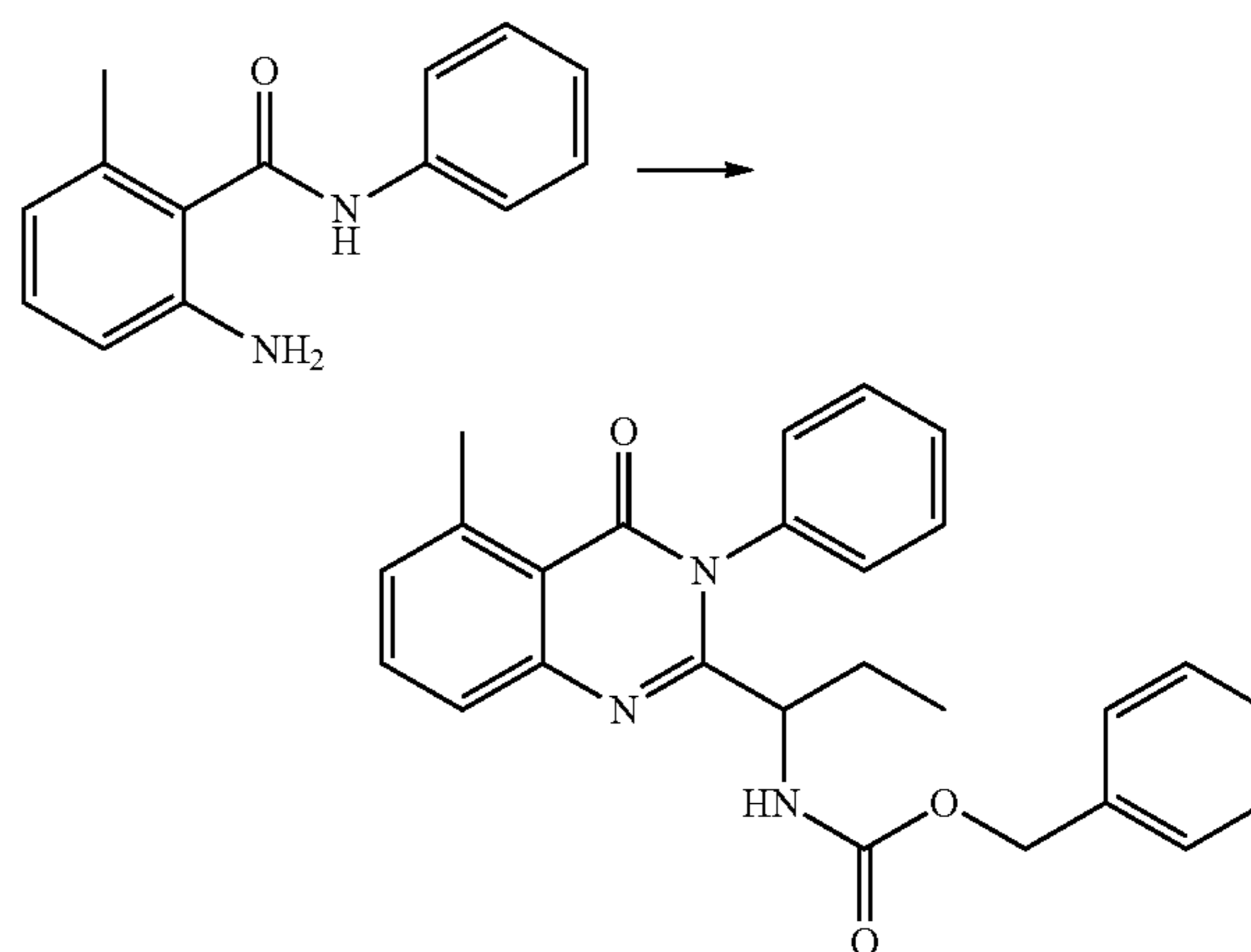
2-(1-amino-propyl)-5-methyl-3-phenyl-3H-quinazolin-4-one (17)
