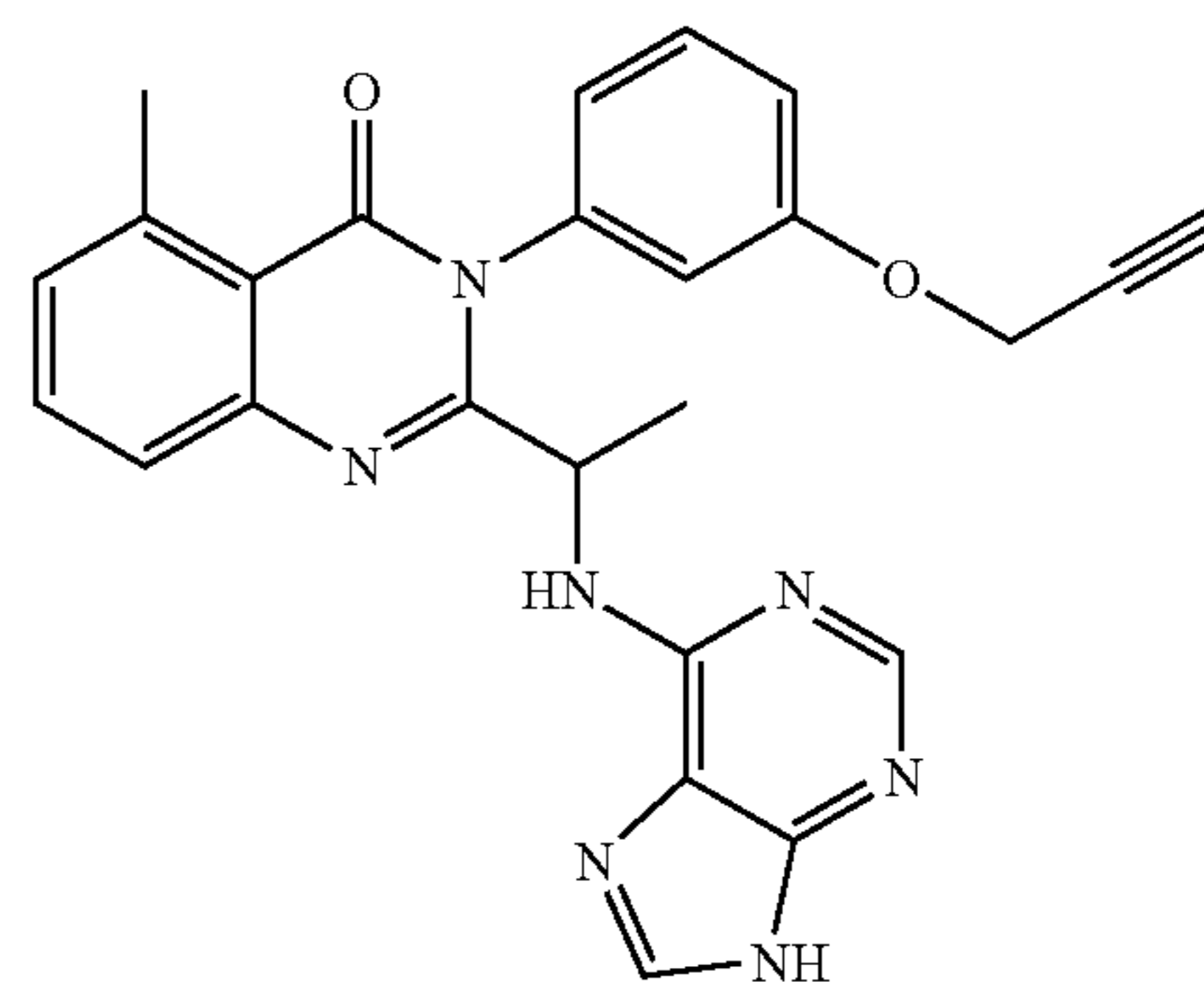
5-Methyl-3-(3-prop-2-ynyloxy-phenyl)[1-(9H-purin-6-ylamino)-ethyl]3H-quinazolin-4-one
