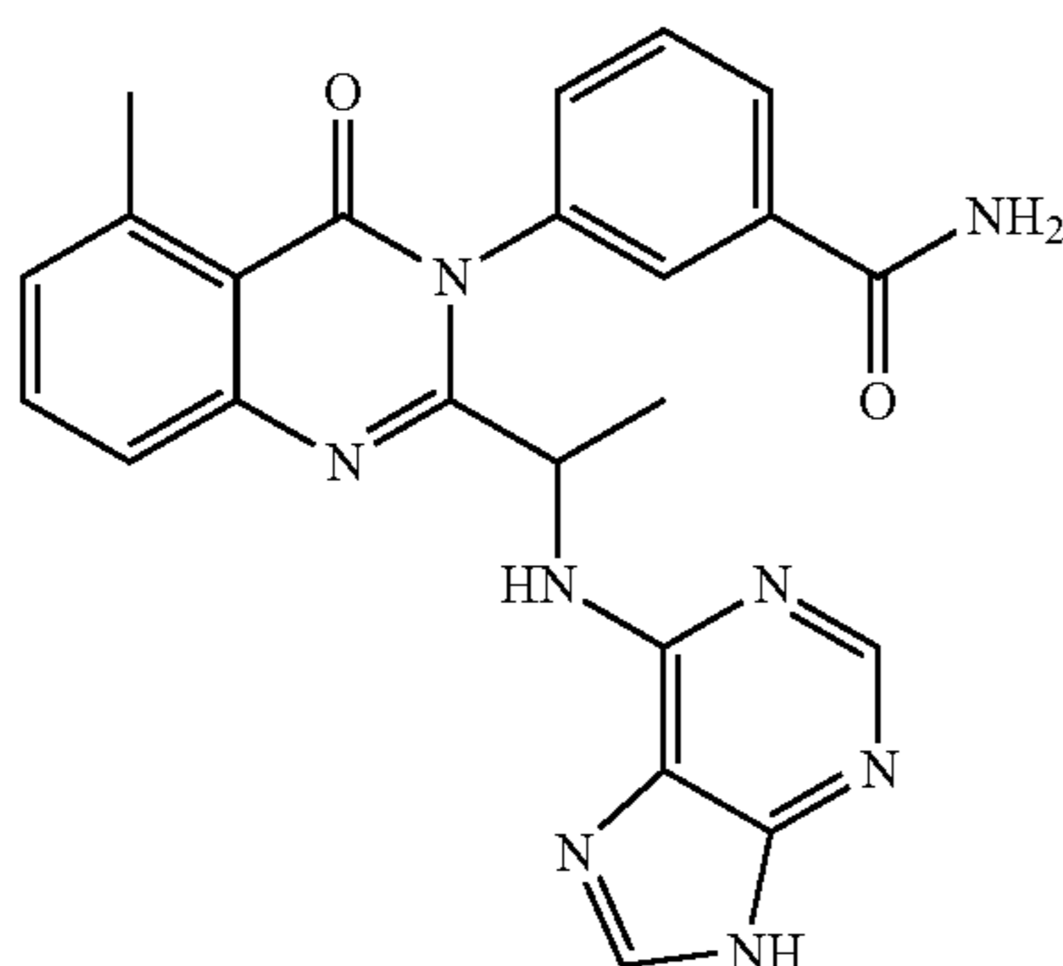
3-(5-Methyl-4-oxo-2-[1-(9H-purin-6-ylamino)-ethyl]-4H-quinazolin-3-yl)benzamide
