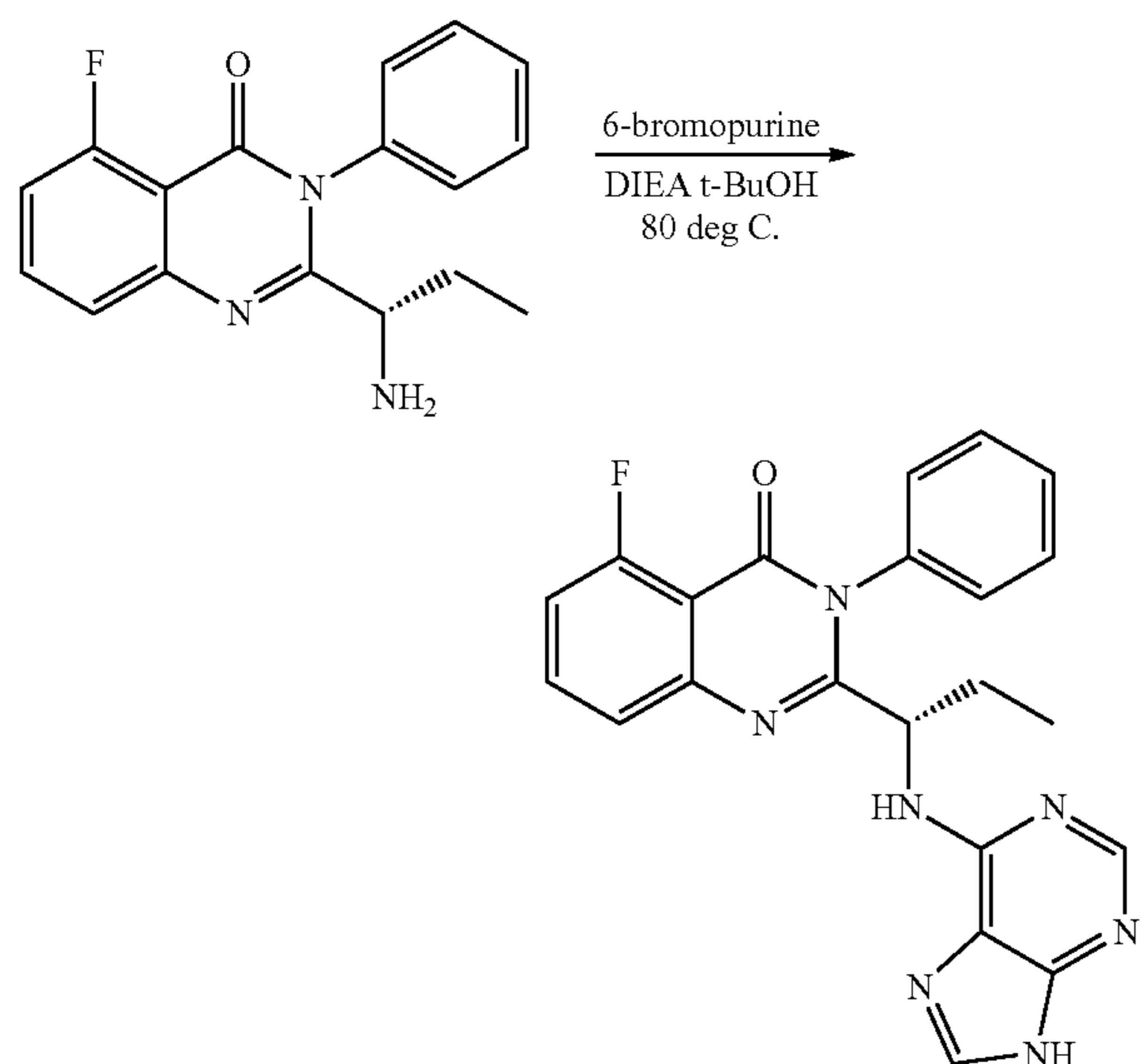
(S)-3-phenyl-2-[1-(9H-purin-6-ylamino)-ethyl]-3H-quinazolin-4-one (112)
