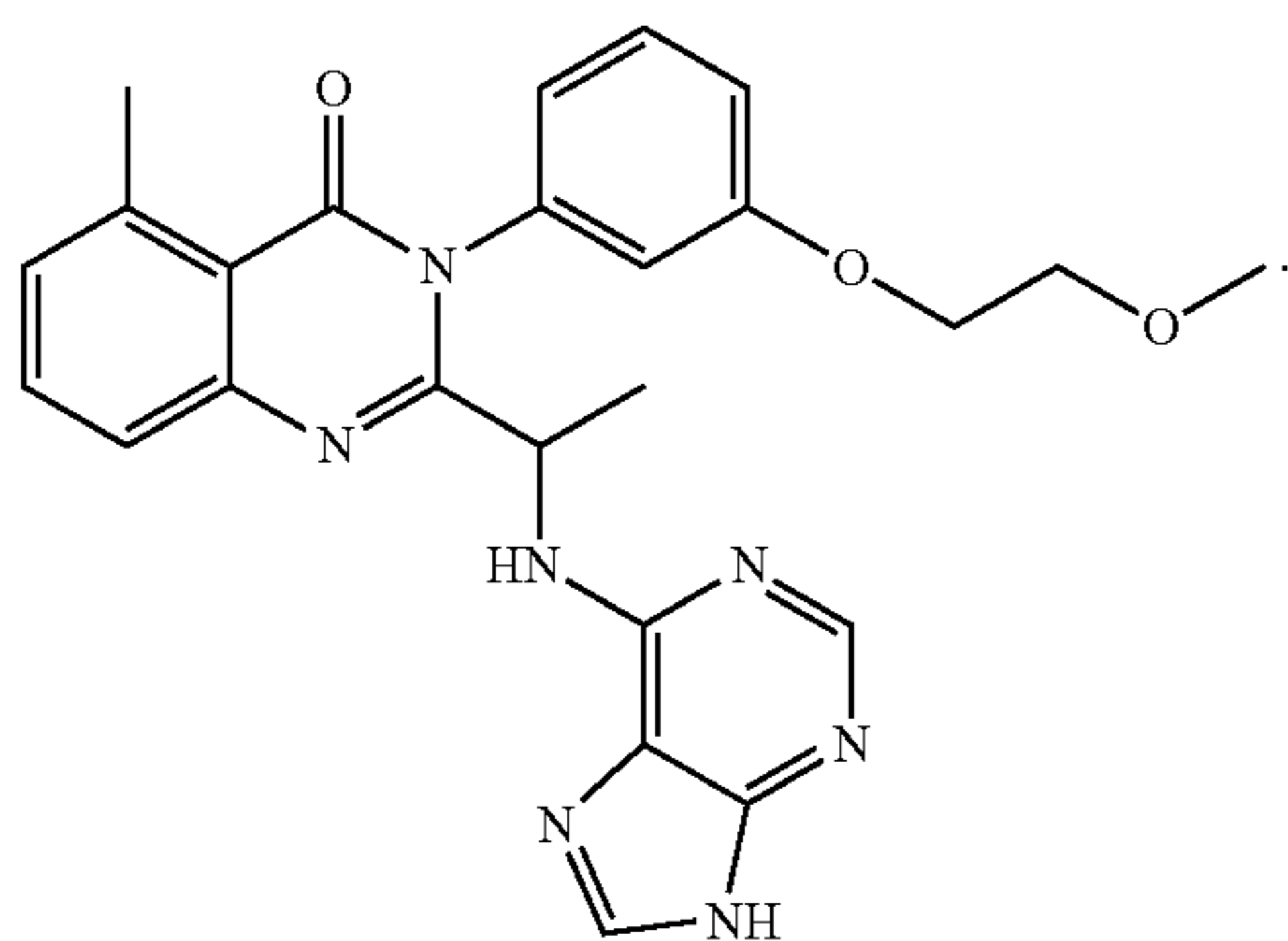
(147) 3-[3-(2-Methoxy-ethoxy)-phenyl]-5-methyl-2-[1-(9H-purin-6-ylamino)-ethyl]-3H-quinazolin-4-one
