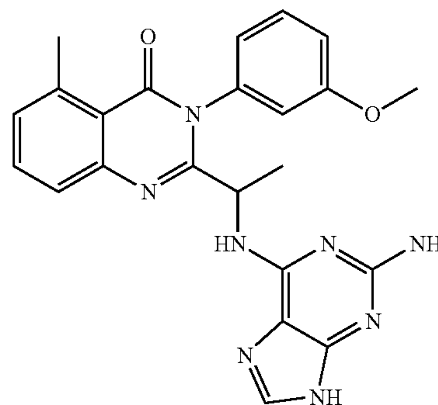
2-[1-(2-Amino-9H-purin-6-ylamino)-ethyl]-3-(3-methoxy-phenyl)-5-methyl-3H-quinazolin-4-one
