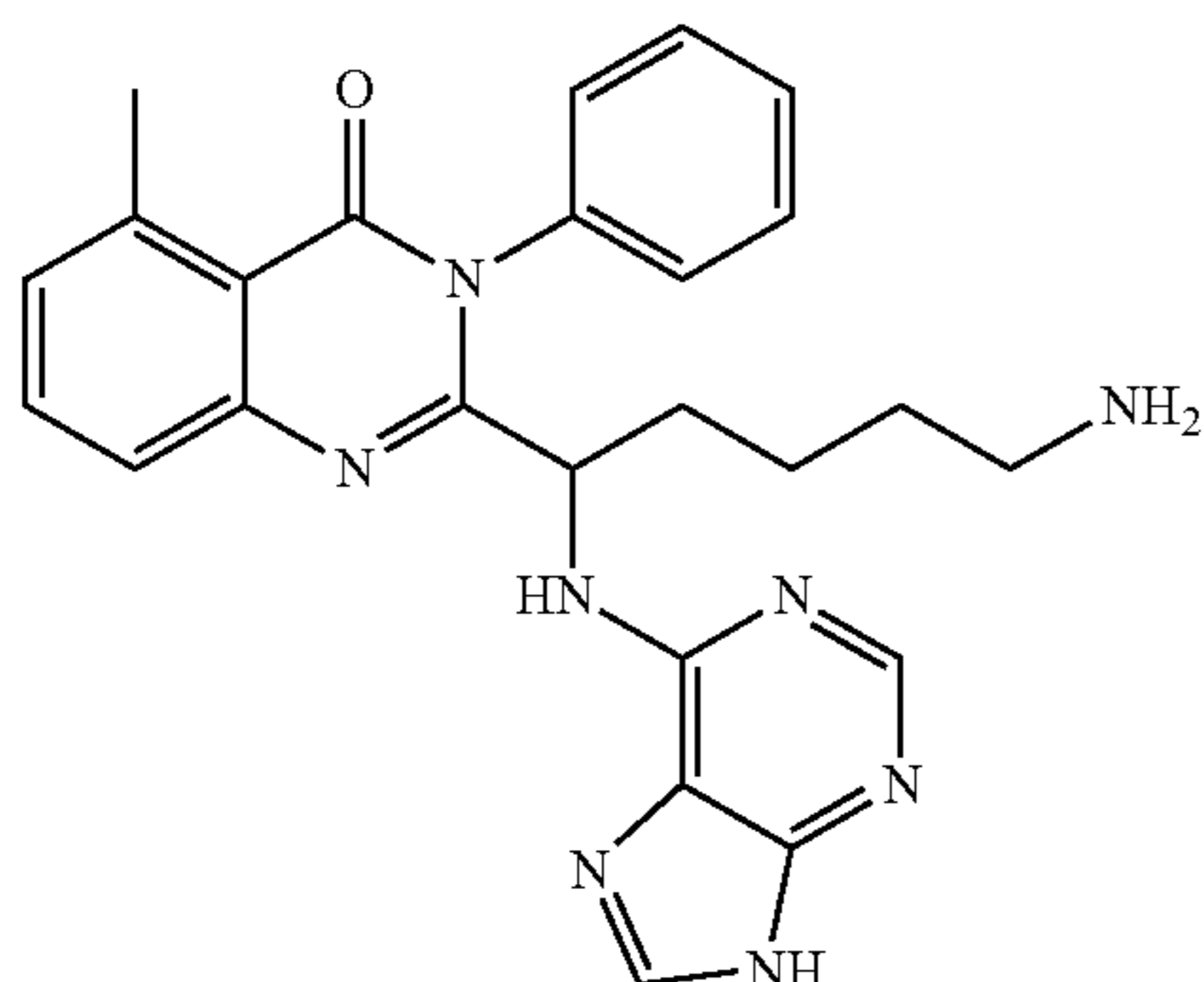
2-[5-amino-1-(2-amino-9H-purin-6-ylamino)-pentyl]-5-methyl-3-phenyl-3H-quinazolin-4-one (55)
