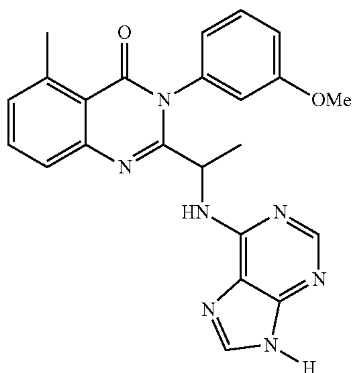
3-(3-Methoxy-phenyl)-5-methyl-2-[1-(9H-purin-6-ylamino)-ethyl]-3H-quinazolin-4-one
