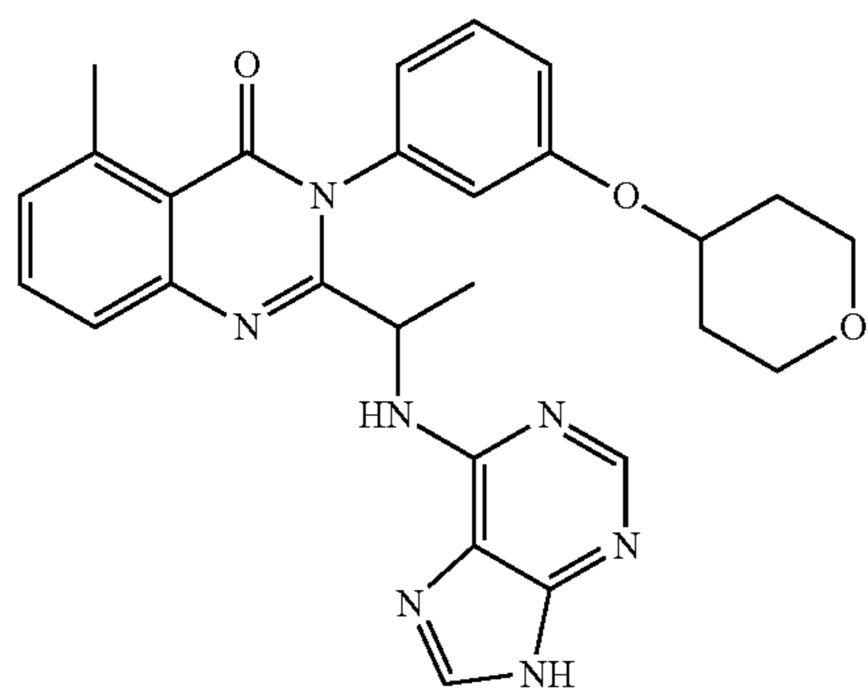
(146) 5-Methyl-2-[1-(9H-purin-6-ylamino)-ethyl]-3-[3-(tetrahydro-pyran-4-yloxy)-phenyl]-3H-quinazolin-4-one
