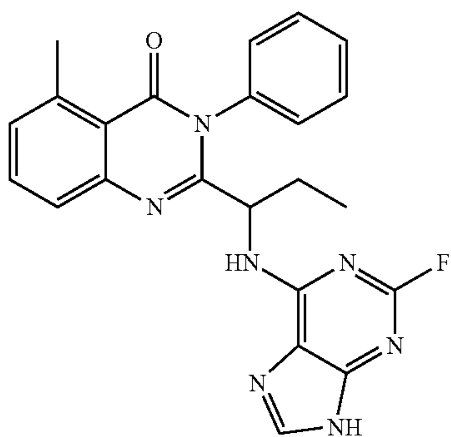
5-methyl-3-phenyl-2-[1-(9H-purin-6-ylamino)-ethyl]-3H-quinazolin-4-one (26)
