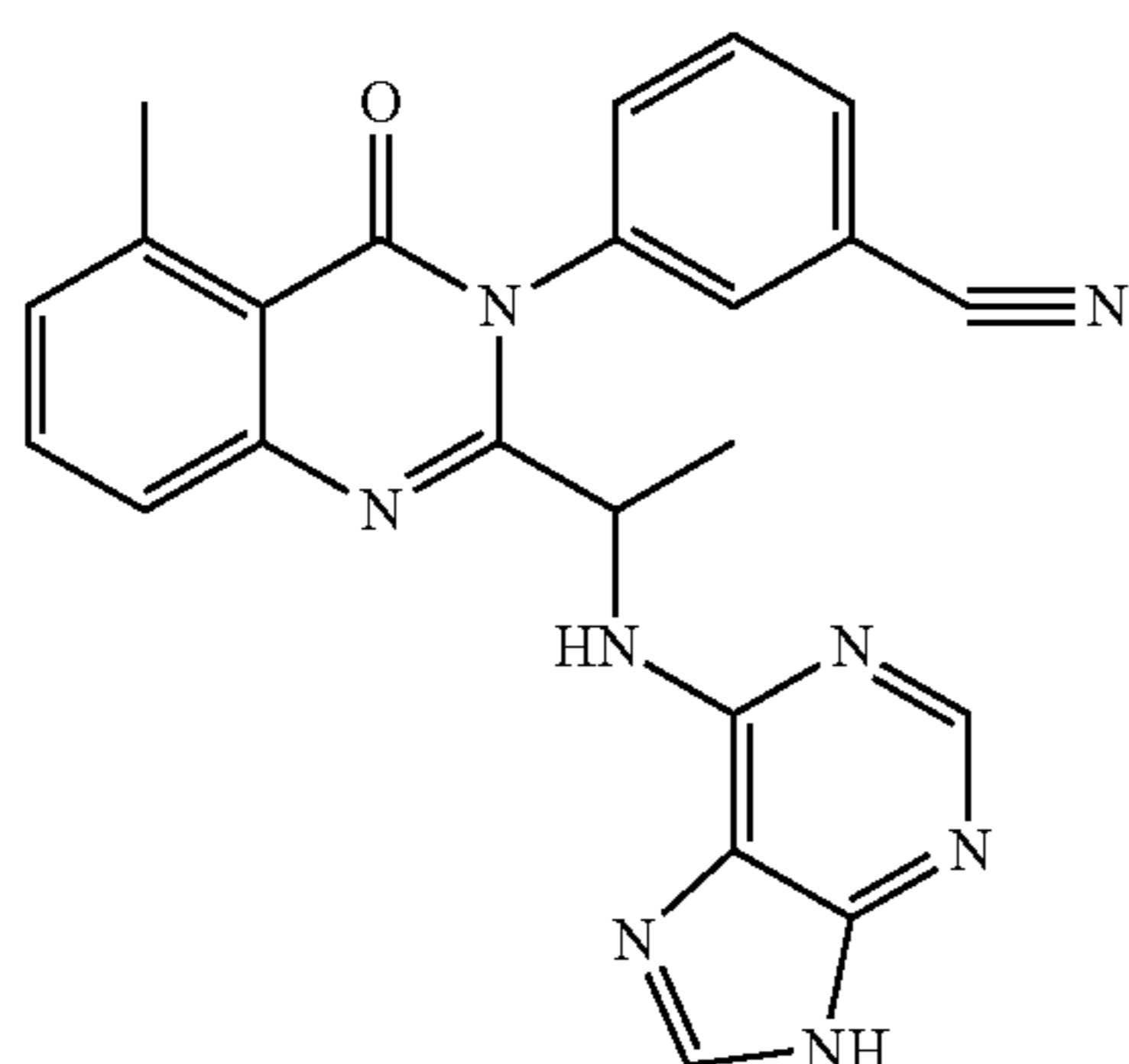
3-(5-Methyl-4-oxo-2-[1-(9H-purin-6-ylamino)-ethyl]-4H-quinazolin-3-yl)-benzotrile
