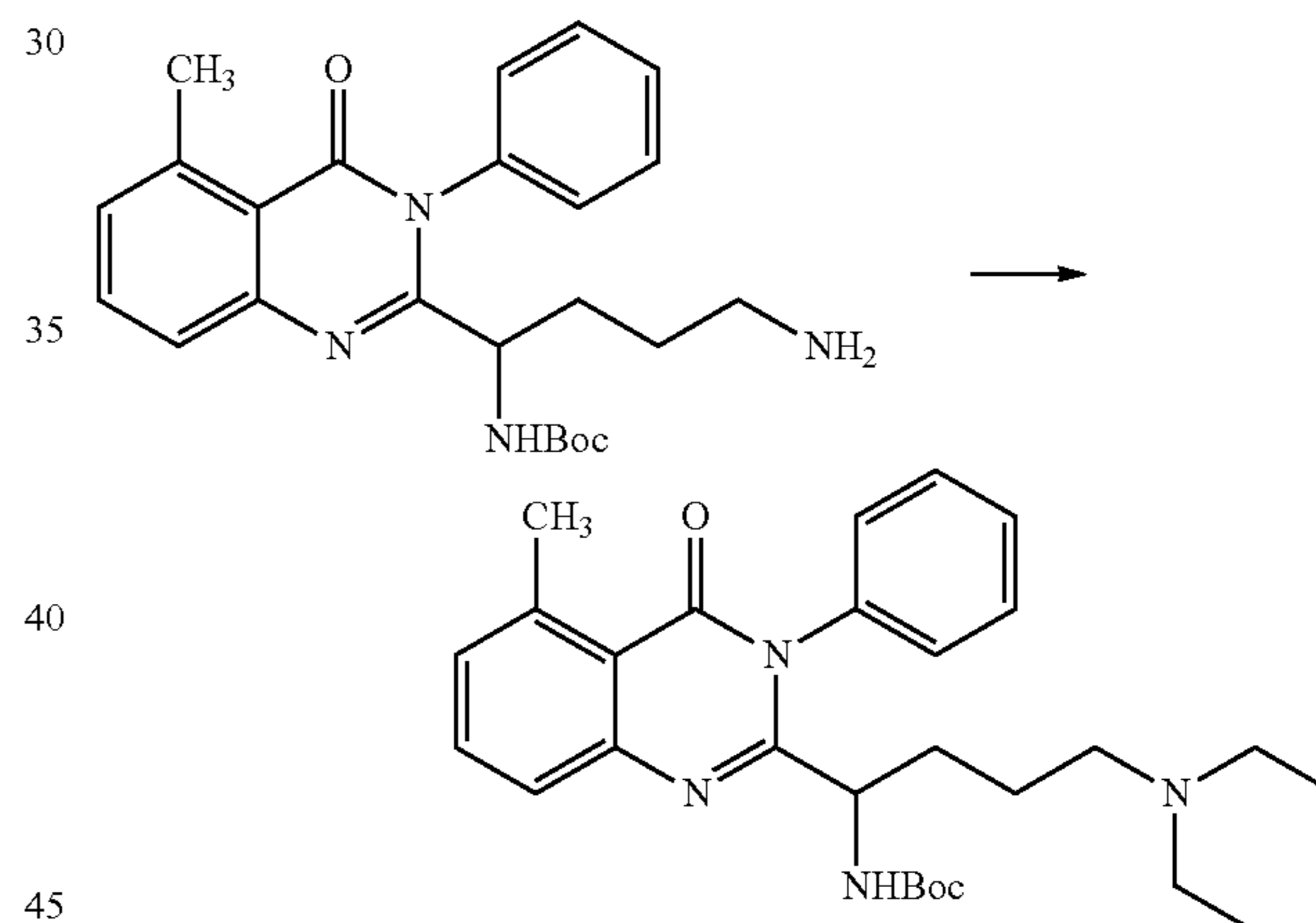
2-(1-amino-4-diethylamino-butyl)-5-methyl-3-phenyl-3H-quinazolin-4-one (106)
