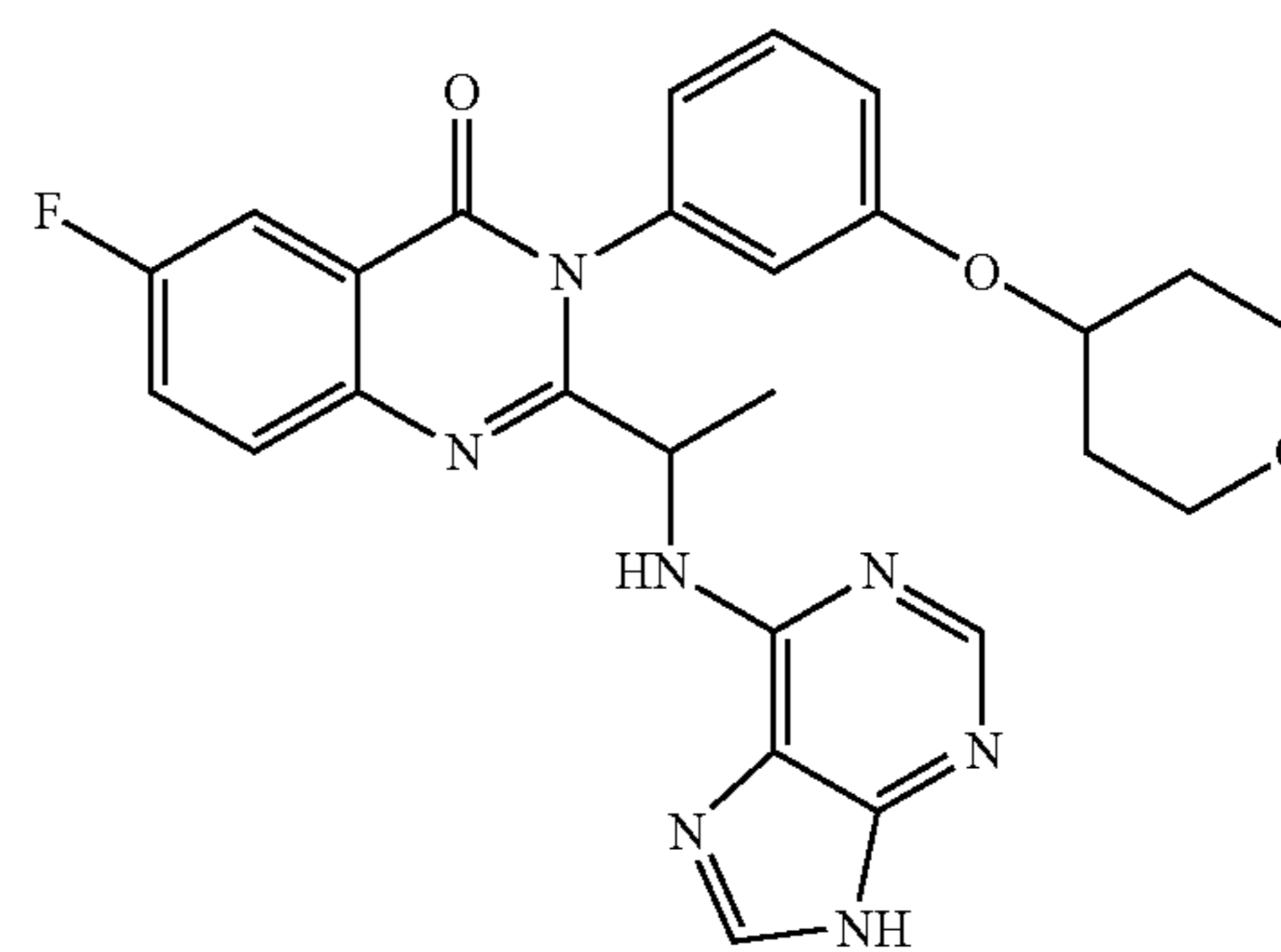
(148) 6-Fluoro-2-[1-(9H-purin-6-ylamino)-ethyl]-3-[3-(tetrahydro-pyran-4-yloxy)-phenyl]-3H-quinazolin-4-one
