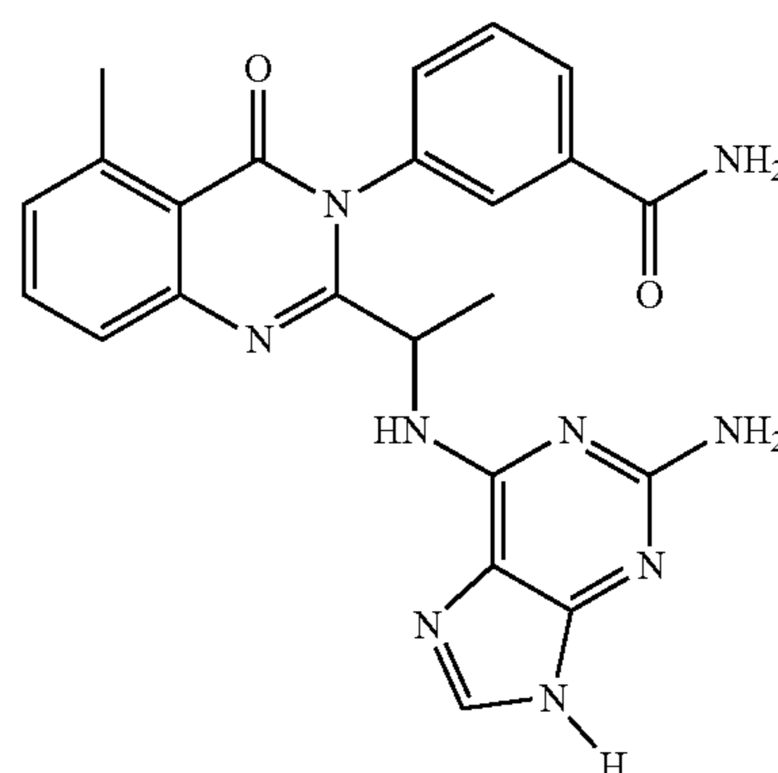
3-(2-[1-(2-Amino-9H-purin-6-ylamino)-ethyl]-5-methyl-4-oxo-4H-quinazolin-3-yl)-benzamide
