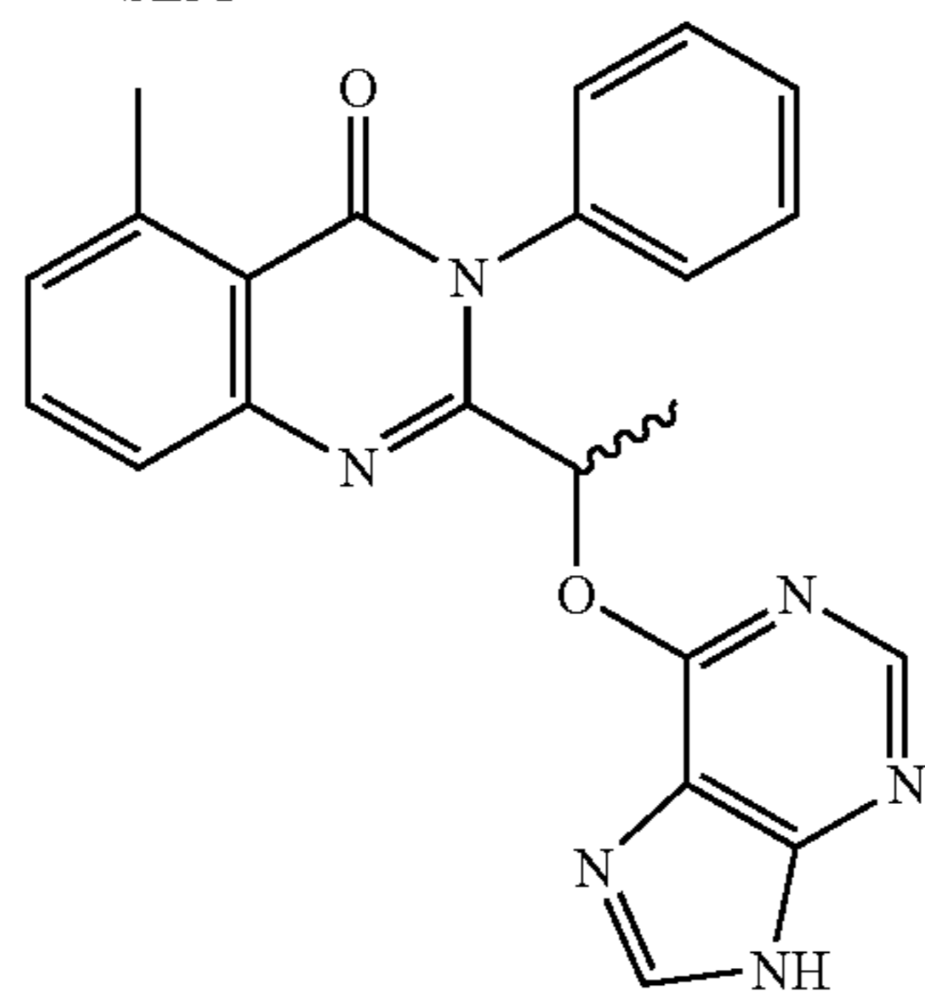
5-methyl-3-phenyl-2-[1-(9H-purin-6-yloxy)-ethyl]- 3H-quinazolin-4-one (176)
