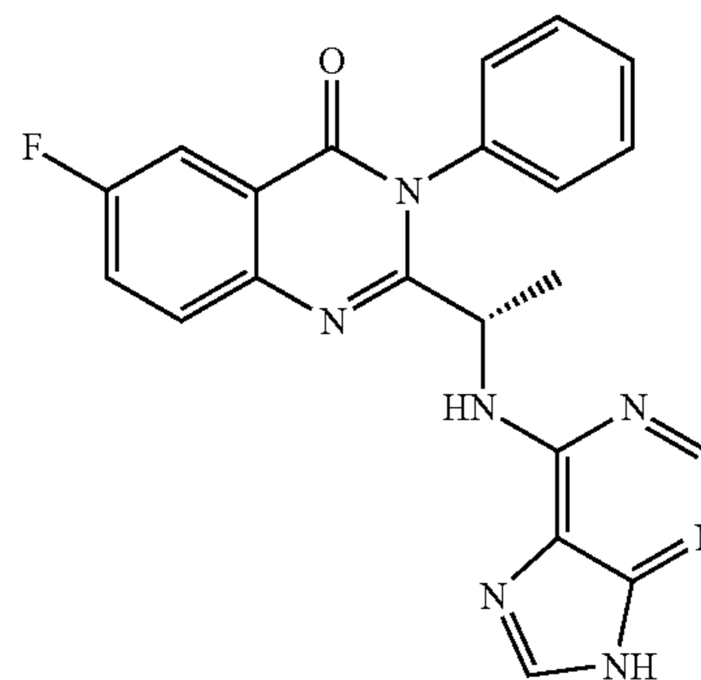
(S)-3-(3,5-difluoro-phenyl)-5-methyl-2-[1-(9H-purin-6-ylamino)-ethyl]-3H-quinazolin-4-one (114)
