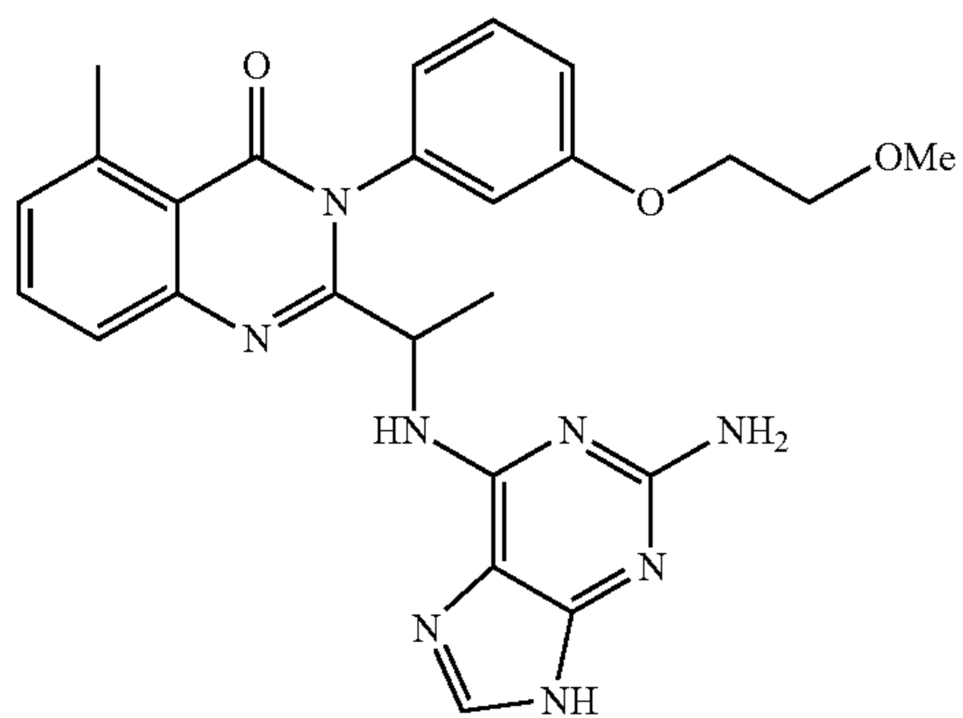
2-[1-(2-Amino-9H-purin-6-ylamino)-ethyl]-3-[3-(2-methoxy-ethoxy)-phenyl]-5-methyl-3H-quinazolin-4-one
