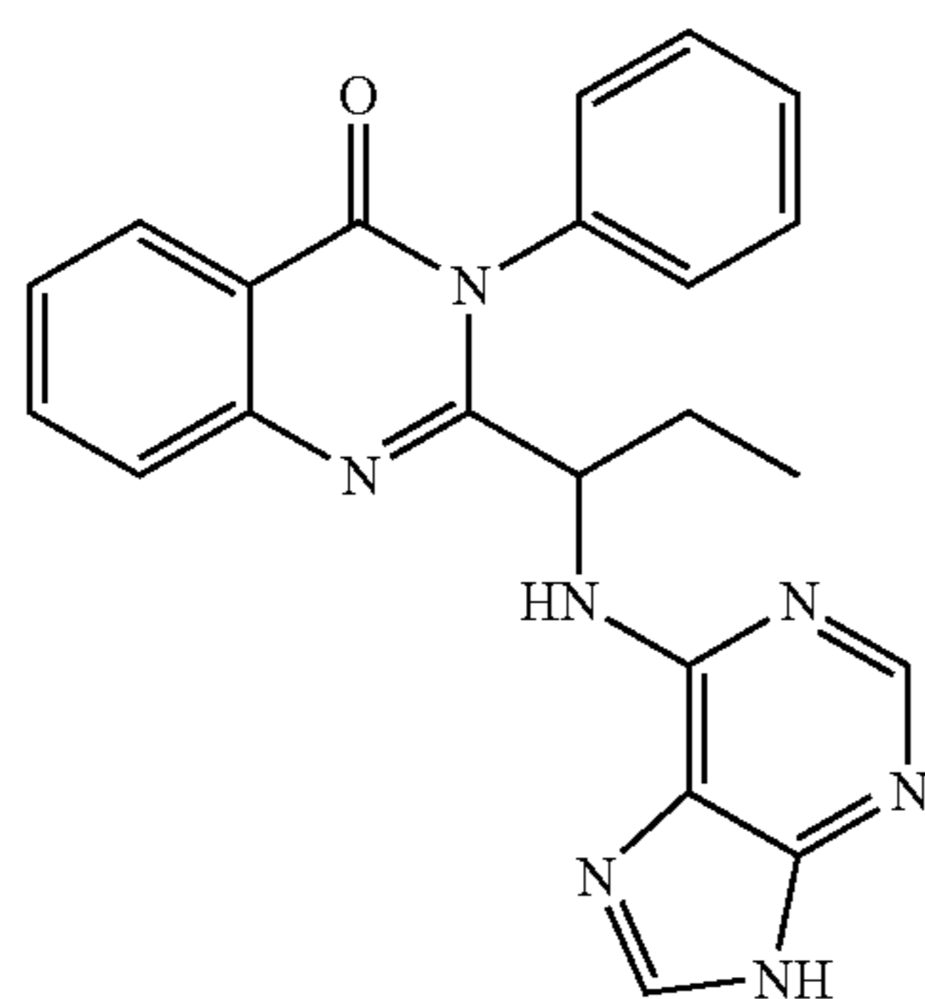
2-[1-(2-amino-9H-purin-6-ylamino)-ethyl]-3-(3,5-difluoro-phenyl)-3H-quinazolin-4-one (99)
