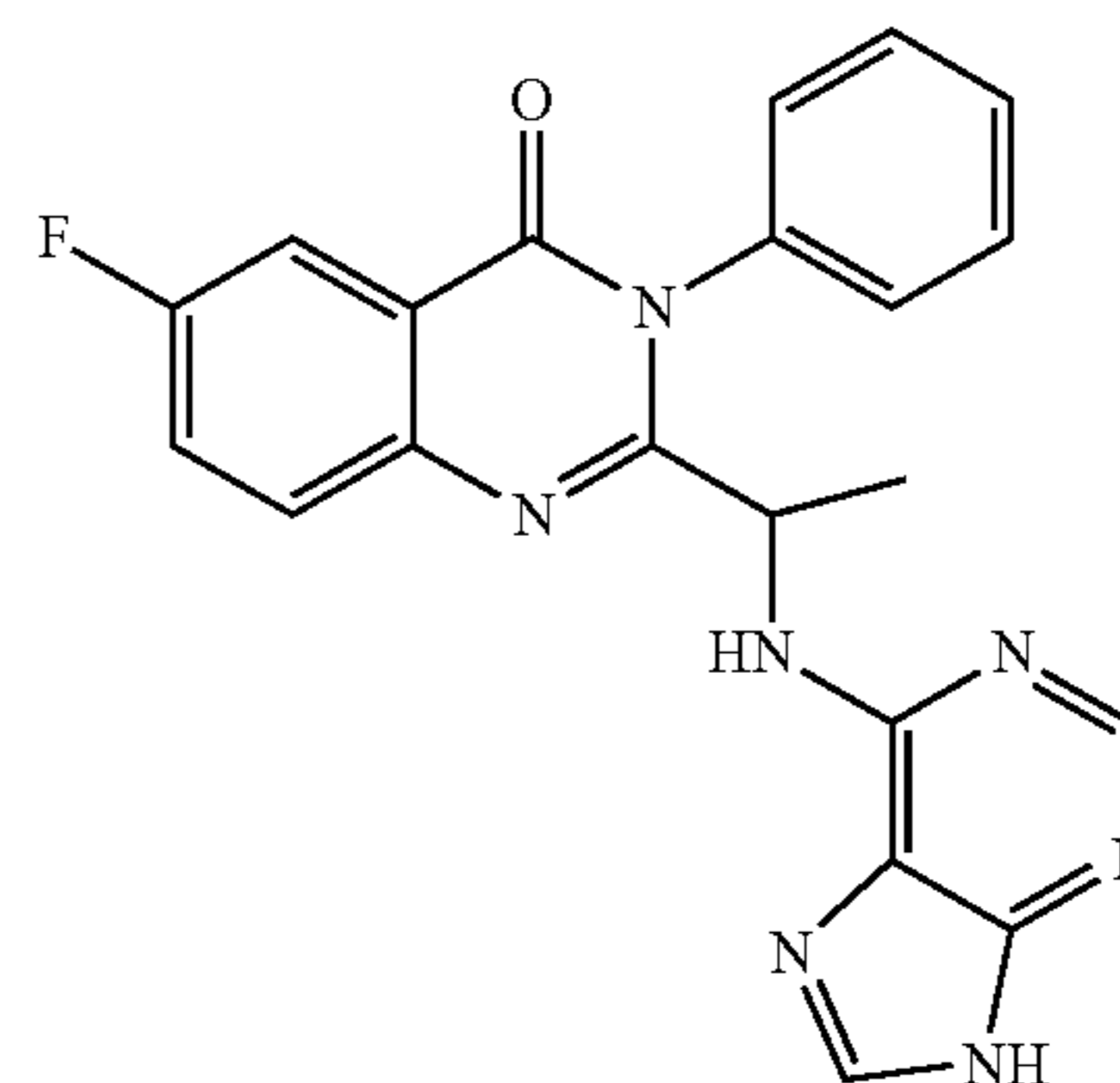
2-[1-(2-amino-9H-purin-6-ylamino)-ethyl]-6-fluoro-3-phenyl-3H-quinazolin-4-one (62)
