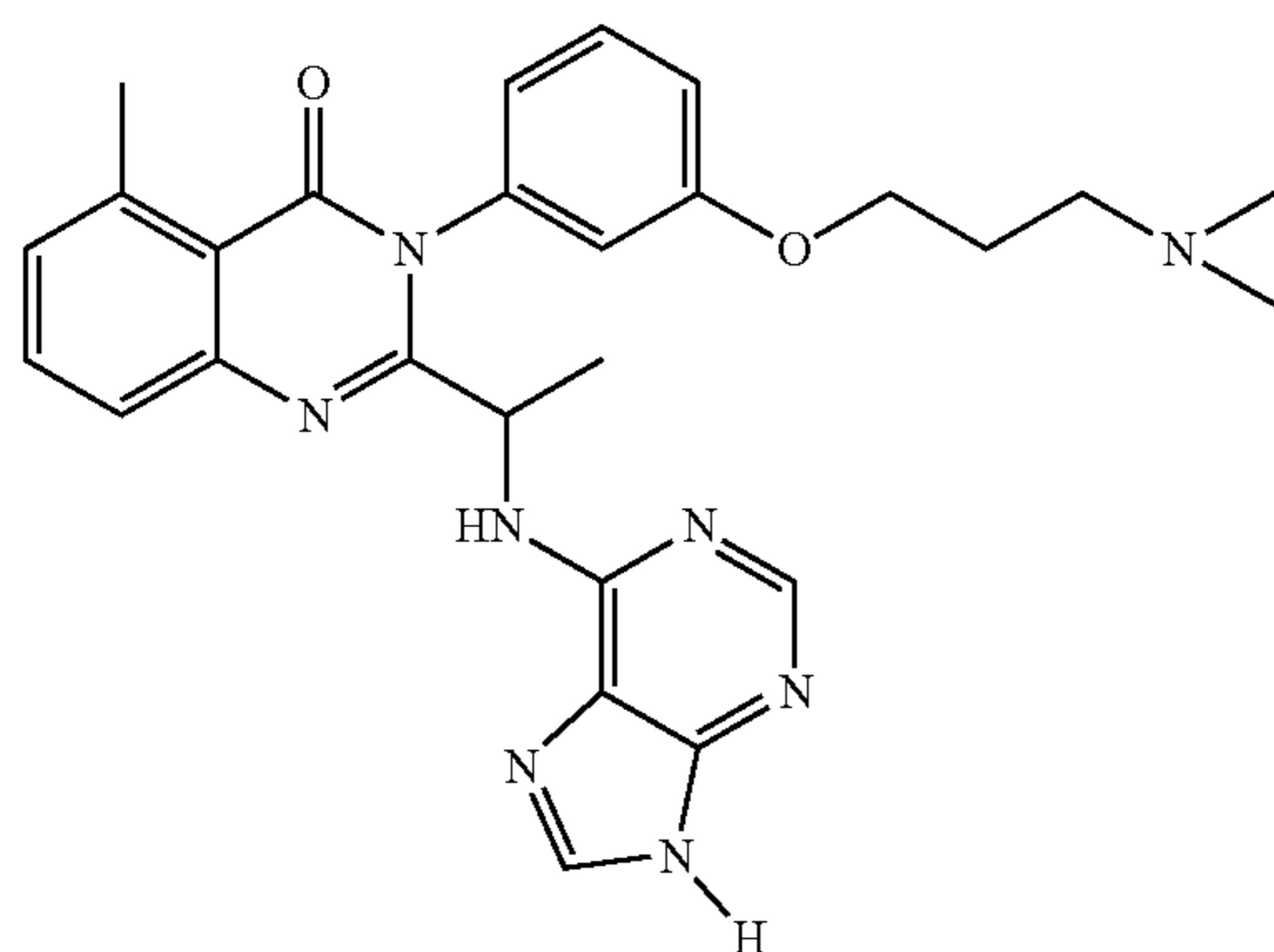
3-[3-(3-Dimethylamino-propoxy)-phenyl]-5-methyl-2-[1-(9H-purin-6-ylamino)-ethyl]-3H-quinazolin-4-one
