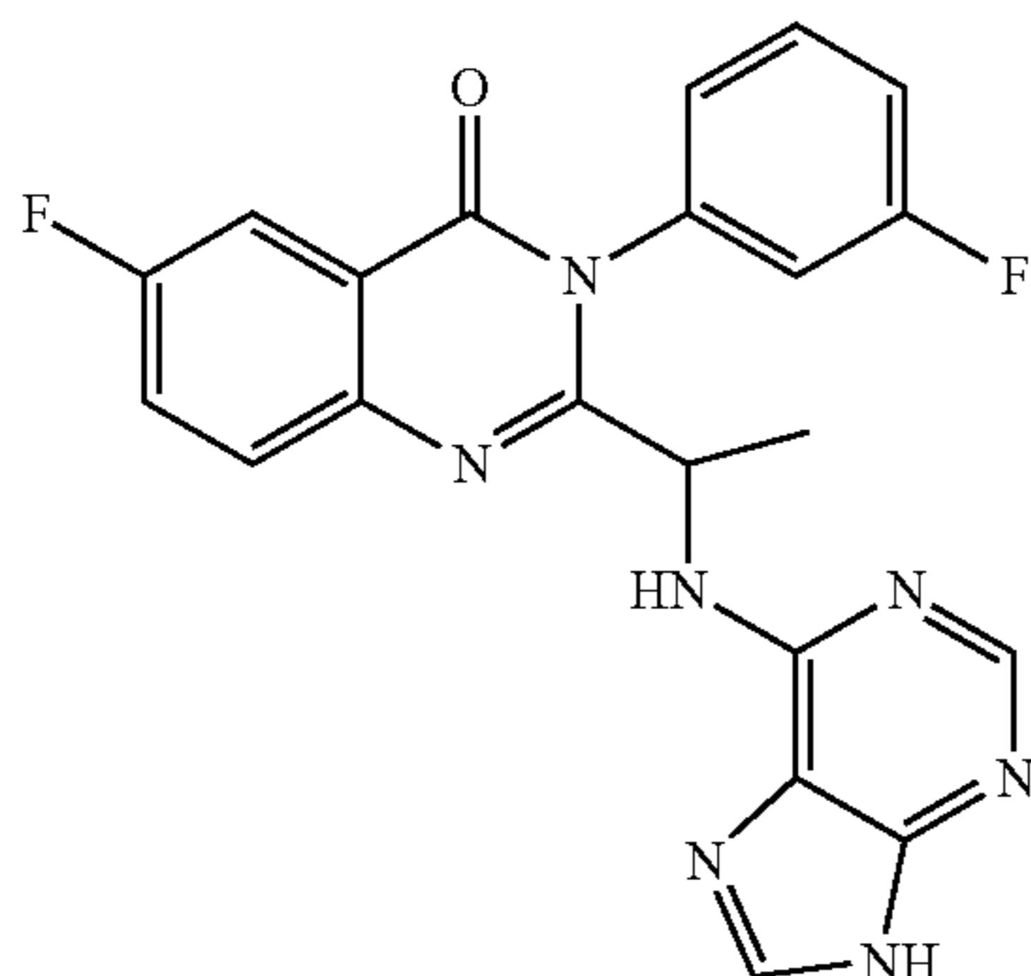
2-[4-diethylamino-1-(9H-purin-6-ylamino)-butyl]-5-methyl-3-phenyl-3H-quinazolin-4-one (103)
