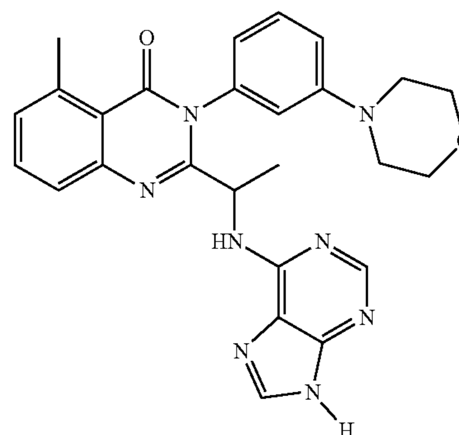
5-Methyl-3-(3-morpholin-4-yl-phenyl)-2-[1-(9H-purin-6-ylamino)-ethyl]-3H-quinazolin-4-one
