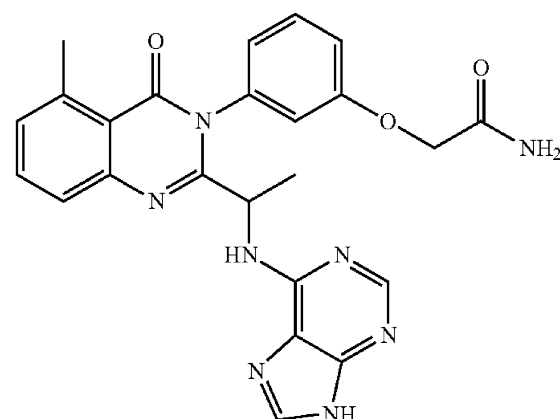
2-(3-[5-Methyl-4-oxo-2-[1-(9H-purin-6-ylamino)-ethyl]-4H-quinazolin-3-yl]-phenoxy)-acetamide
