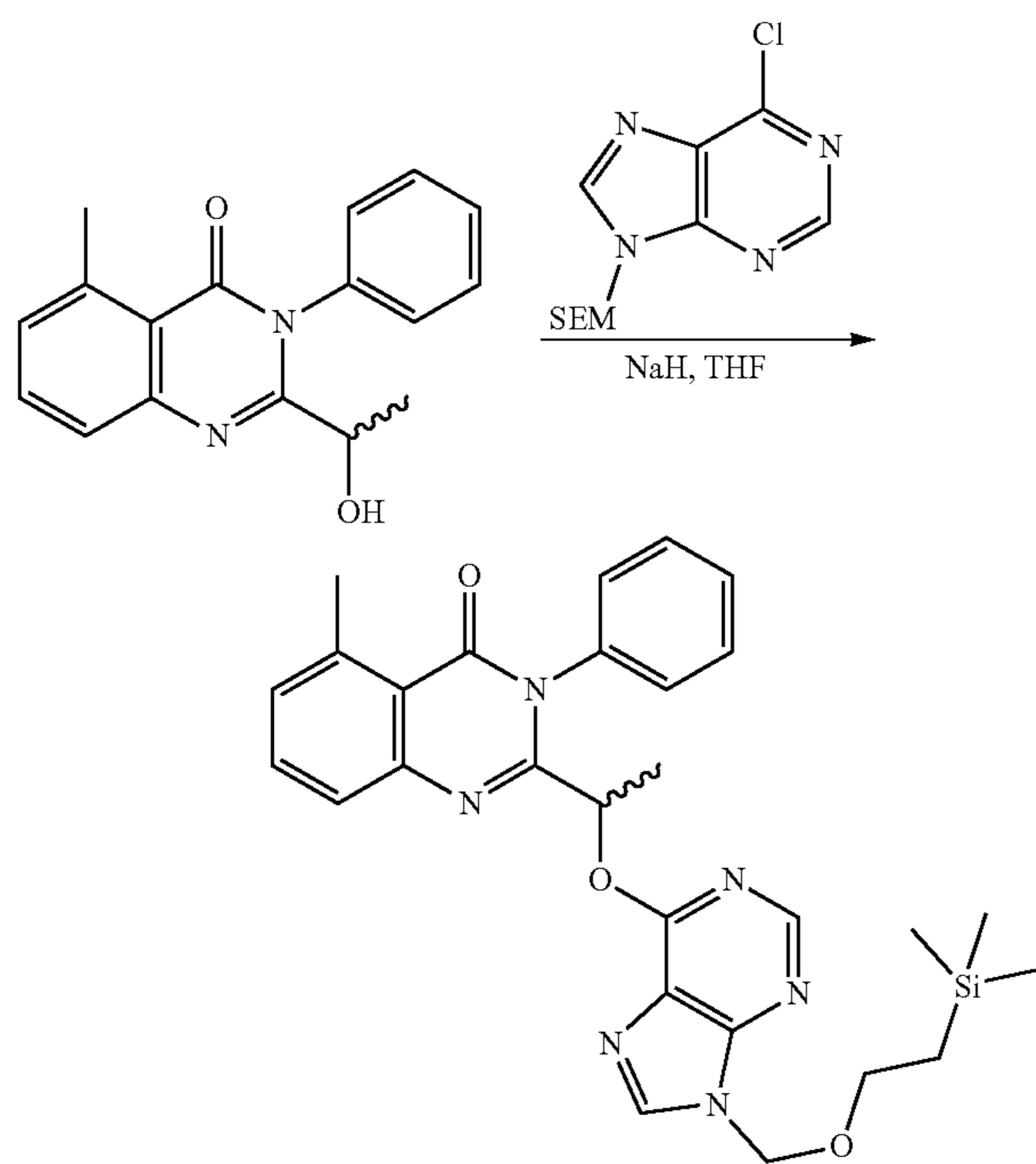
5-Methyl-3-phenyl-2-[1-(9H-purin-6-yloxy)-ethyl]-3H-quinazolin-4-one (176)
