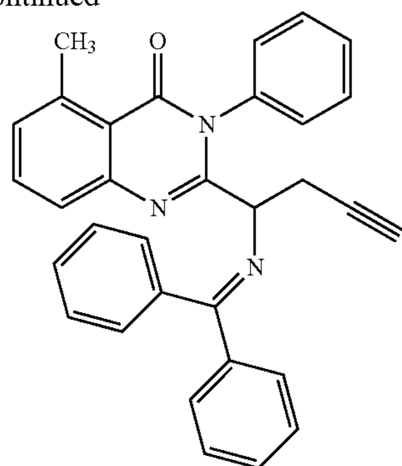
2-(1-amino-but-3-ynyl)-5-methyl-3-phenyl-3H-quinazolin-4-one (164)
