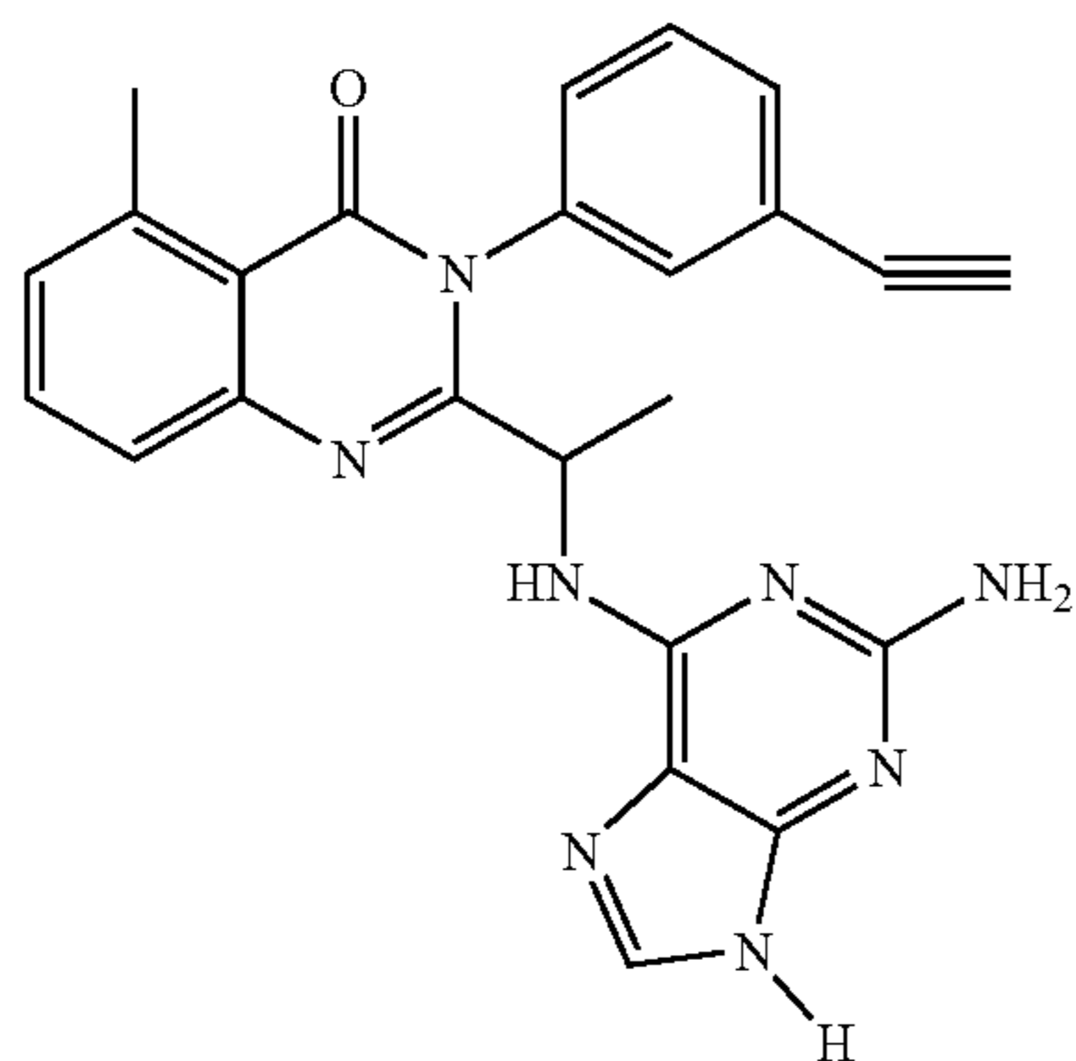
2-[1-(2-Amino-9H-purin-6-ylamino)-ethyl]-3-(3-ethynyl-phenyl)-5-methyl-3H-quinazolin-4-one
