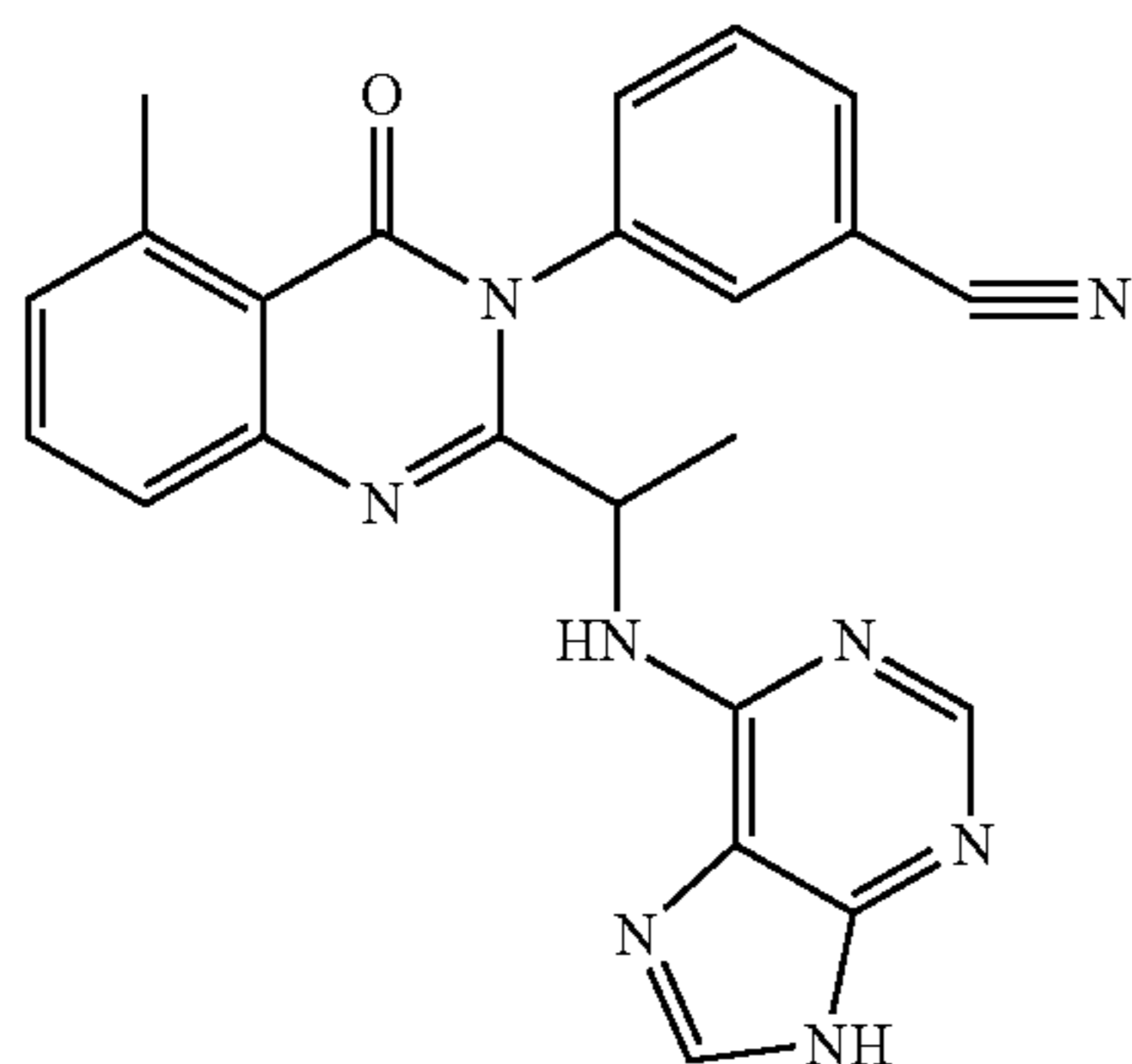
3-(5-Methyl-4-oxo-2-[1-(9H-purin-6-ylamino)-ethyl]-4H-quinazolin-3-yl)-benzotrile
