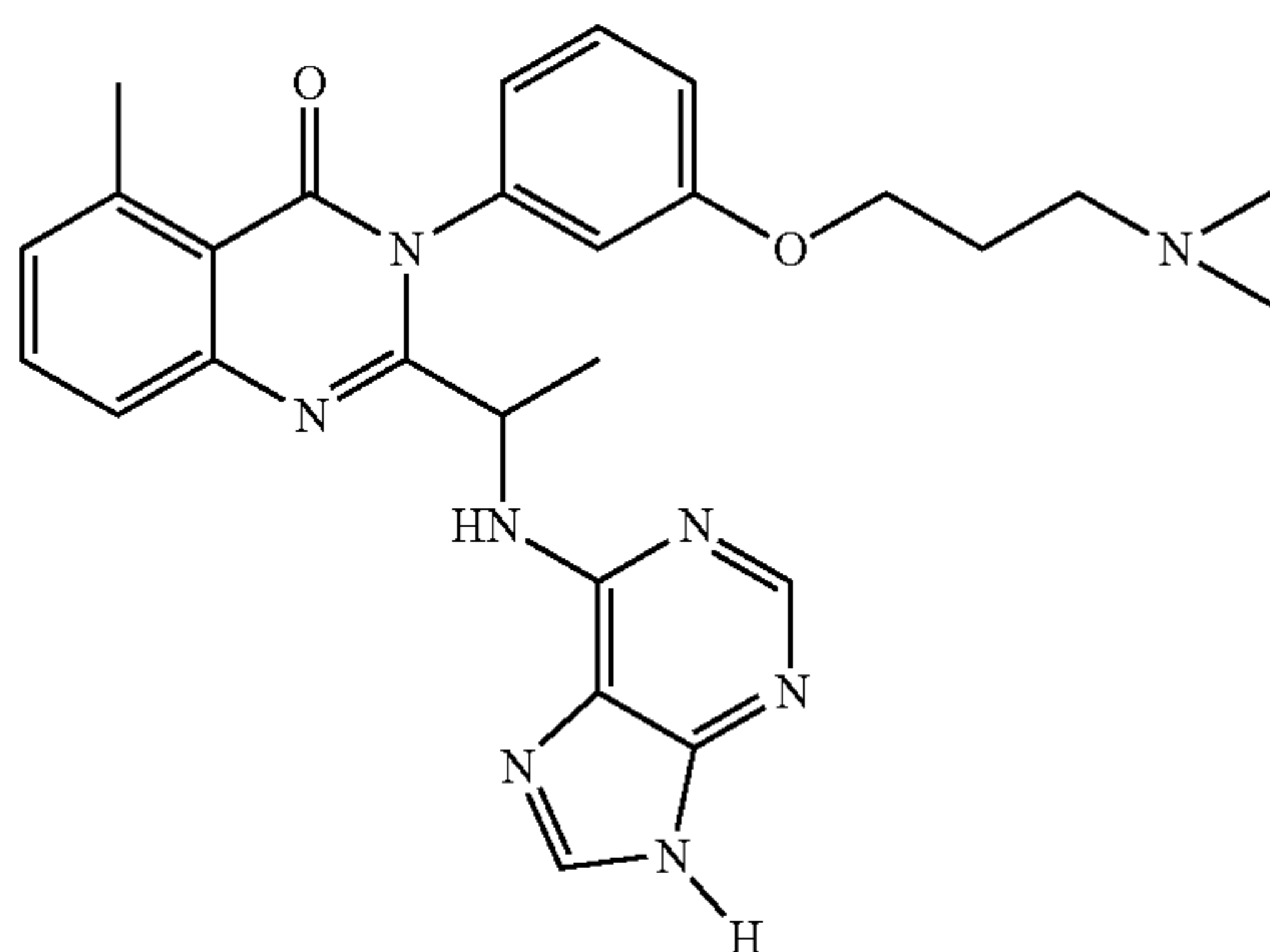
3-[3-(3-Dimethylamino-propoxy)-phenyl]-5-methyl-2-[1-(9H-purin-6-ylamino)-ethyl]-3H-quinazolin-4-one
