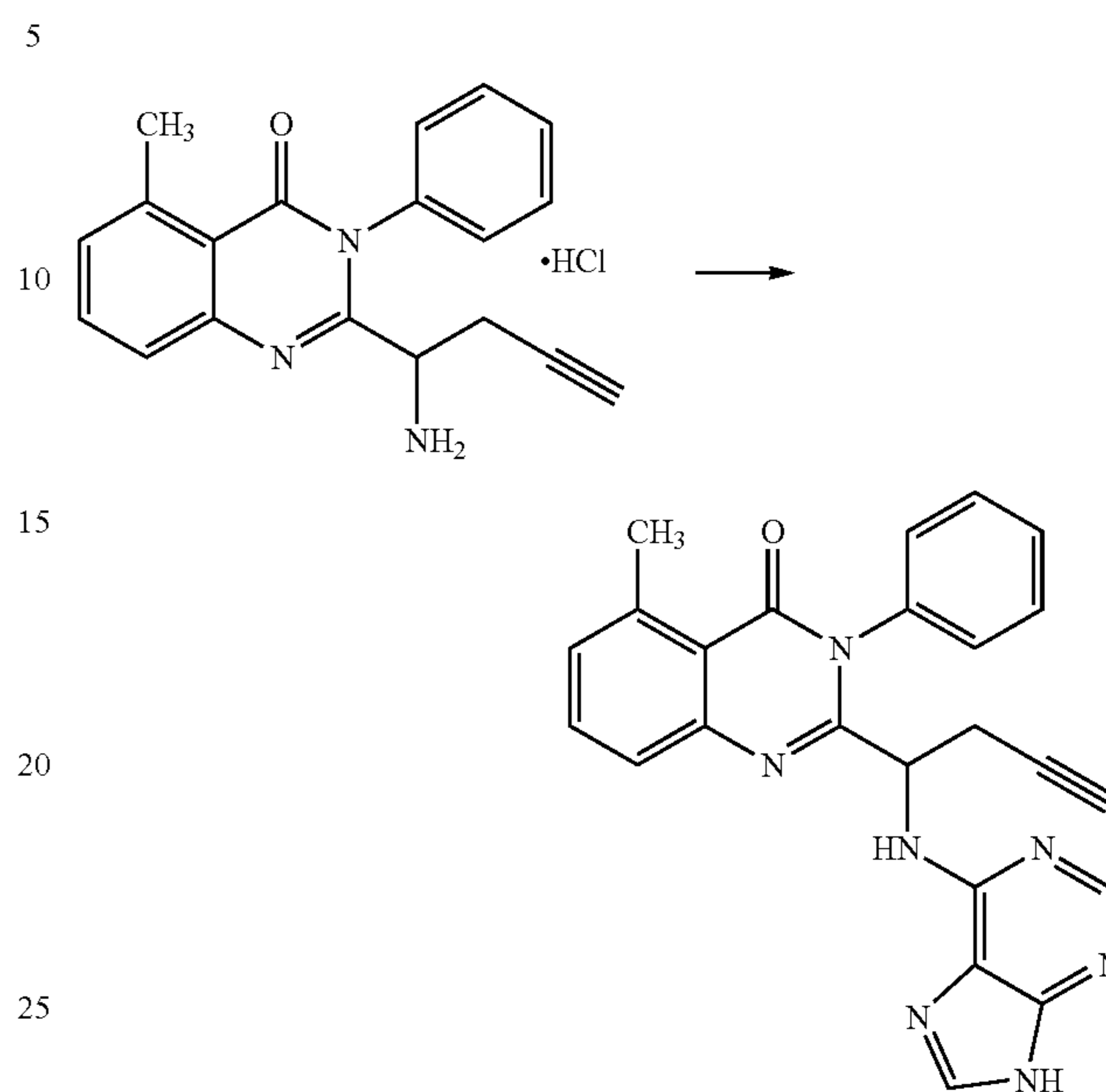
2-(1-amino-but-3-ynyl)-5-methyl-3-phenyl-3H-quinazolin-4-one (164)
