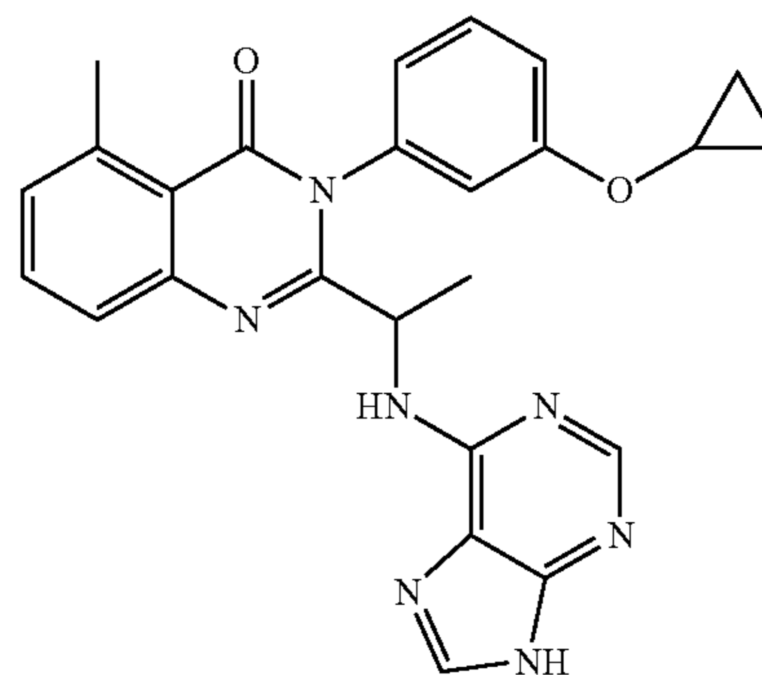
3-[3-Cyclopropylmethoxy-phenyl]-5-methyl-2-[1-(9H-purin-6-ylamino)-ethyl]-3H-quinazolin-4-one
