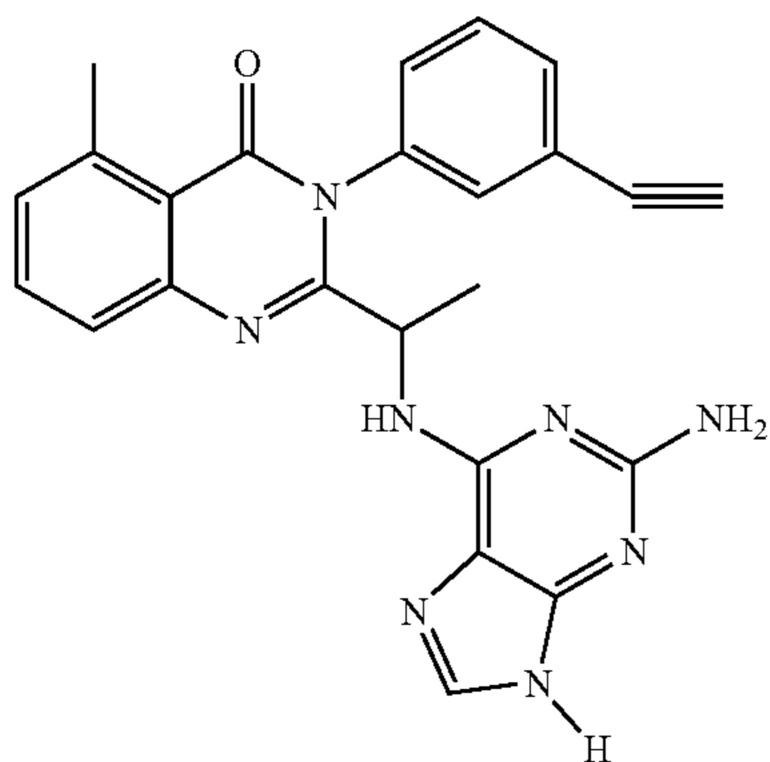
2-[1-(2-Amino-9H-purin-6-ylamino)-ethyl]-3-(3-ethynyl-phenyl)-5-methyl-3H-quinazolin-4-one
