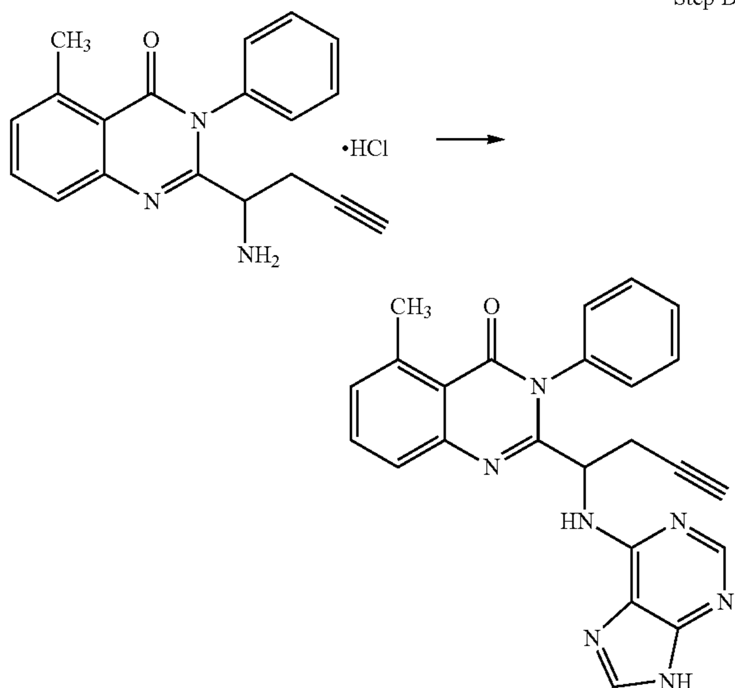
2-[1-(2-amino-9H-purin-6-ylamino)-but-3-ynyl]-5-methyl-3-phenyl-3H-quinazolin-4-one (161)
