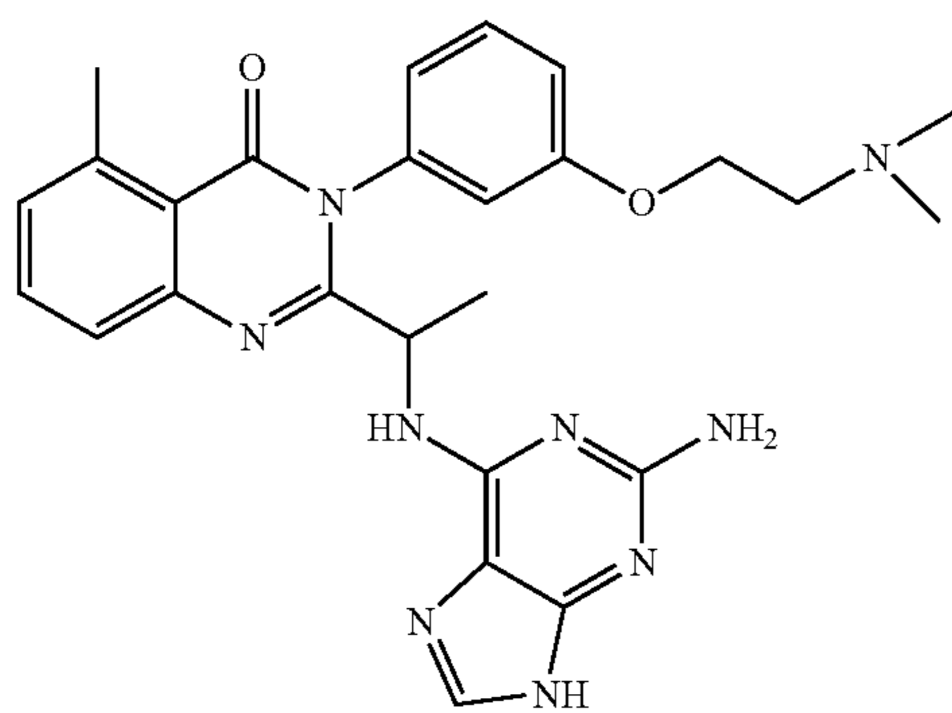
2-[1-(2-Amino-9H-purin-6-ylamino)-ethyl]-3-[3-(2-dimethylamino-ethoxy)-phenyl]-5-methyl-3H-quinazolin-4-one
