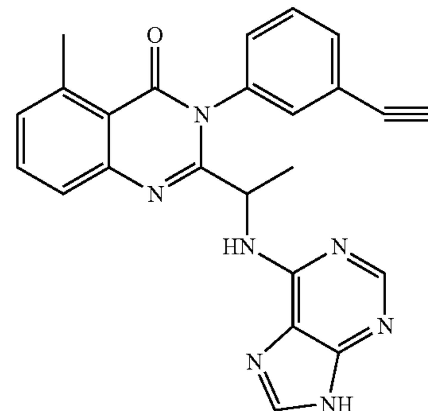
3-(3-Ethynyl-phenyl)-5-methyl-2-[1-(9H-purin-6-ylamino)-ethyl]-3H-quinazolin-4-one
