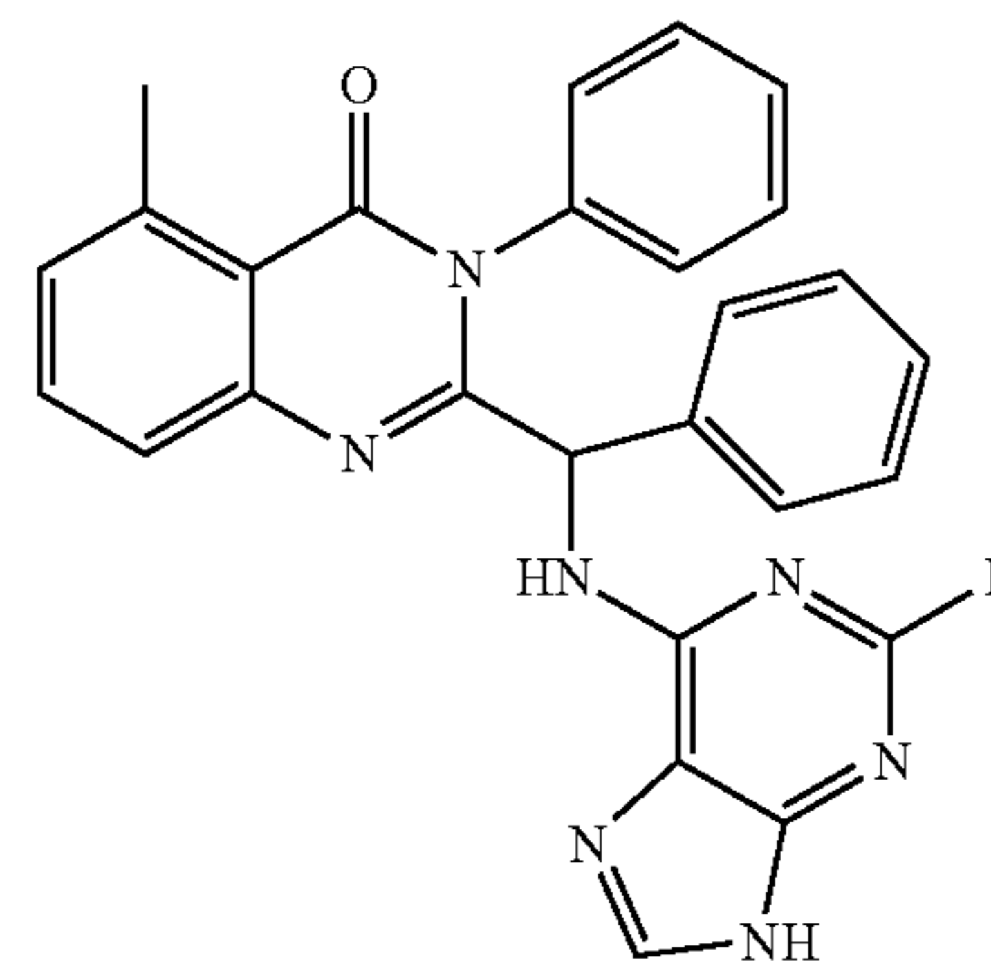
5-methyl-3-phenyl-2-[phenyl-(7H-pyrrolo[2,3-d]pyrimidin-4-ylamino)-methyl]-3H-quinazolin-4-one (45)
