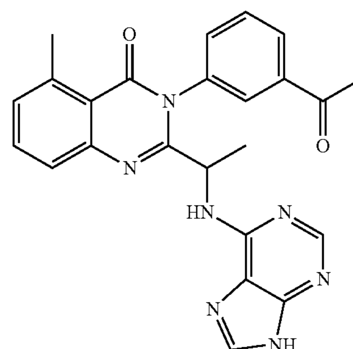
3-(3-Acetyl-phenyl)-5-methyl-2-[1-(9H-purin-6-ylamino)-ethyl]-3H-quinazolin-4-one
