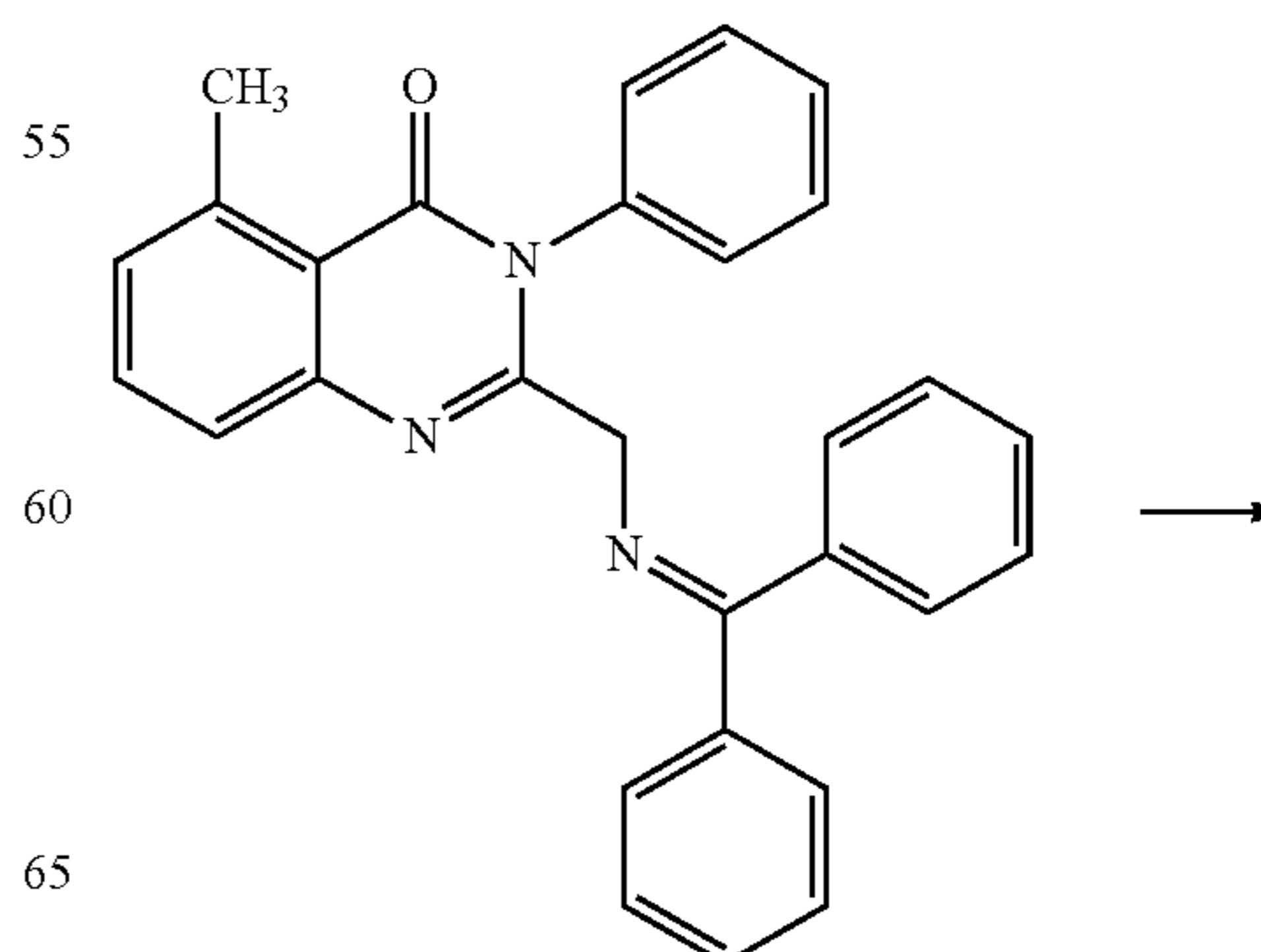
2-[(Benzhydrylidene-amino)-methyl]-5-methyl-3-phenyl-3H-quinazolin-4-one (162)
