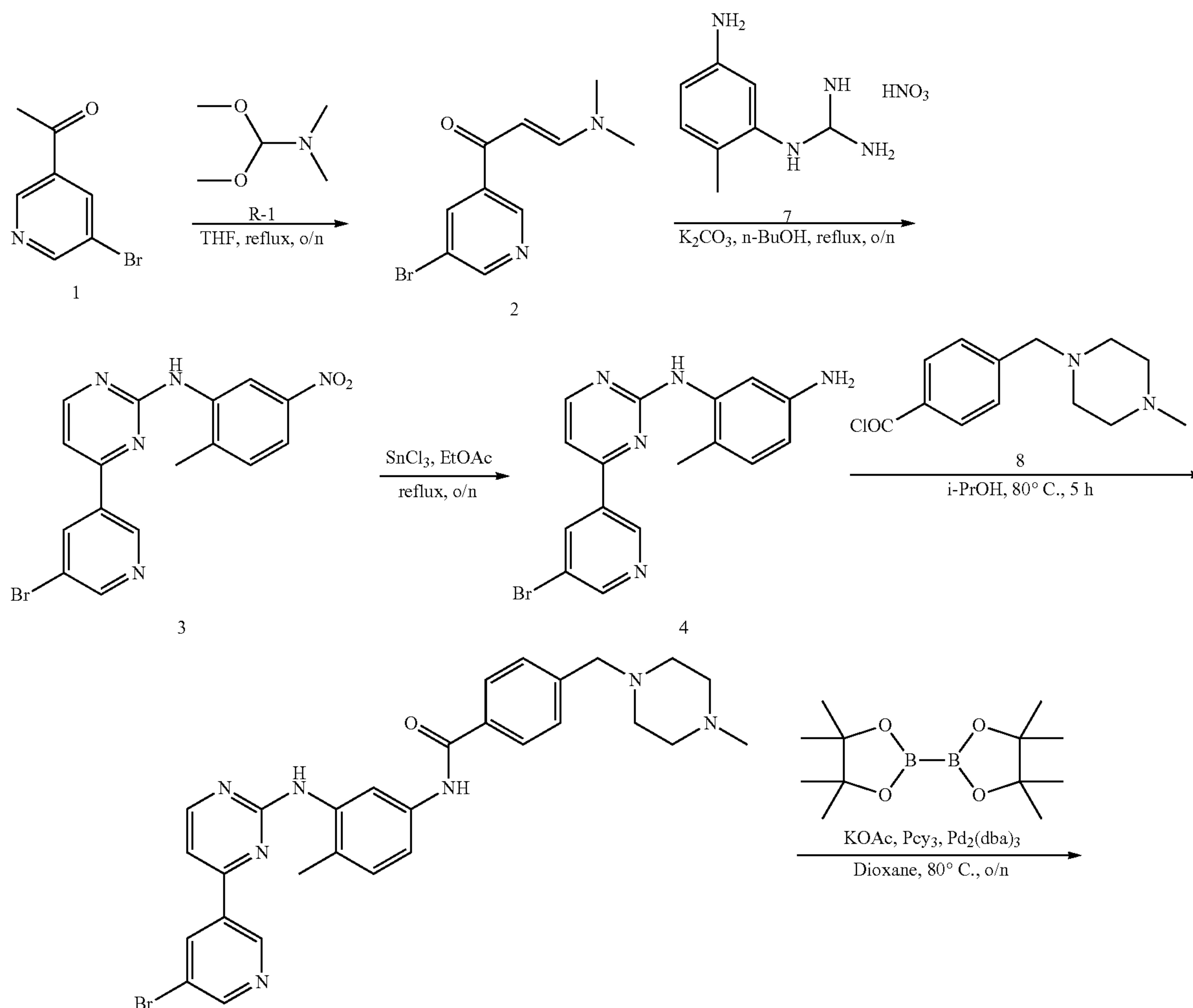
Scheme 1: Synthesis of Intermediates 5 and 6
