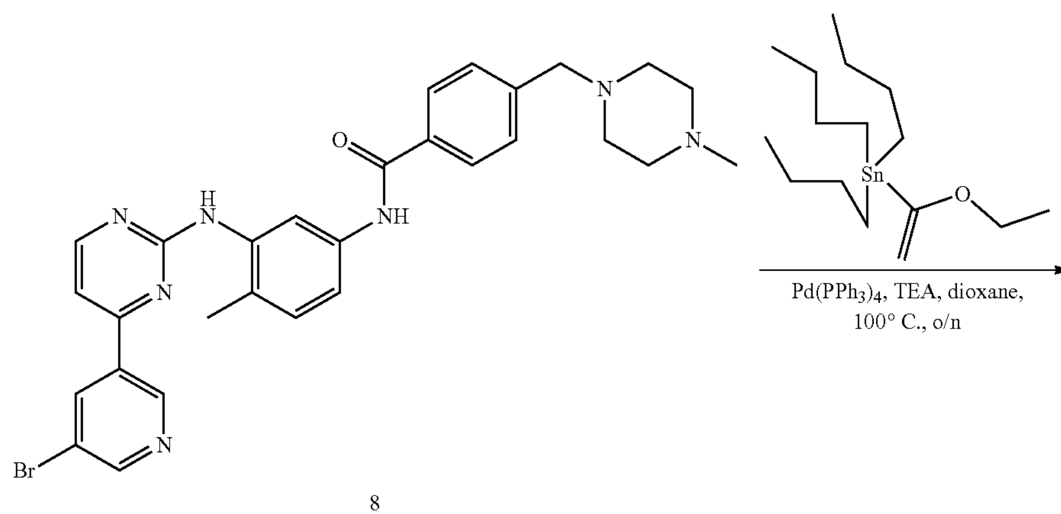
Scheme 2: Synthesis of Intermediates 7, 8 and 9
