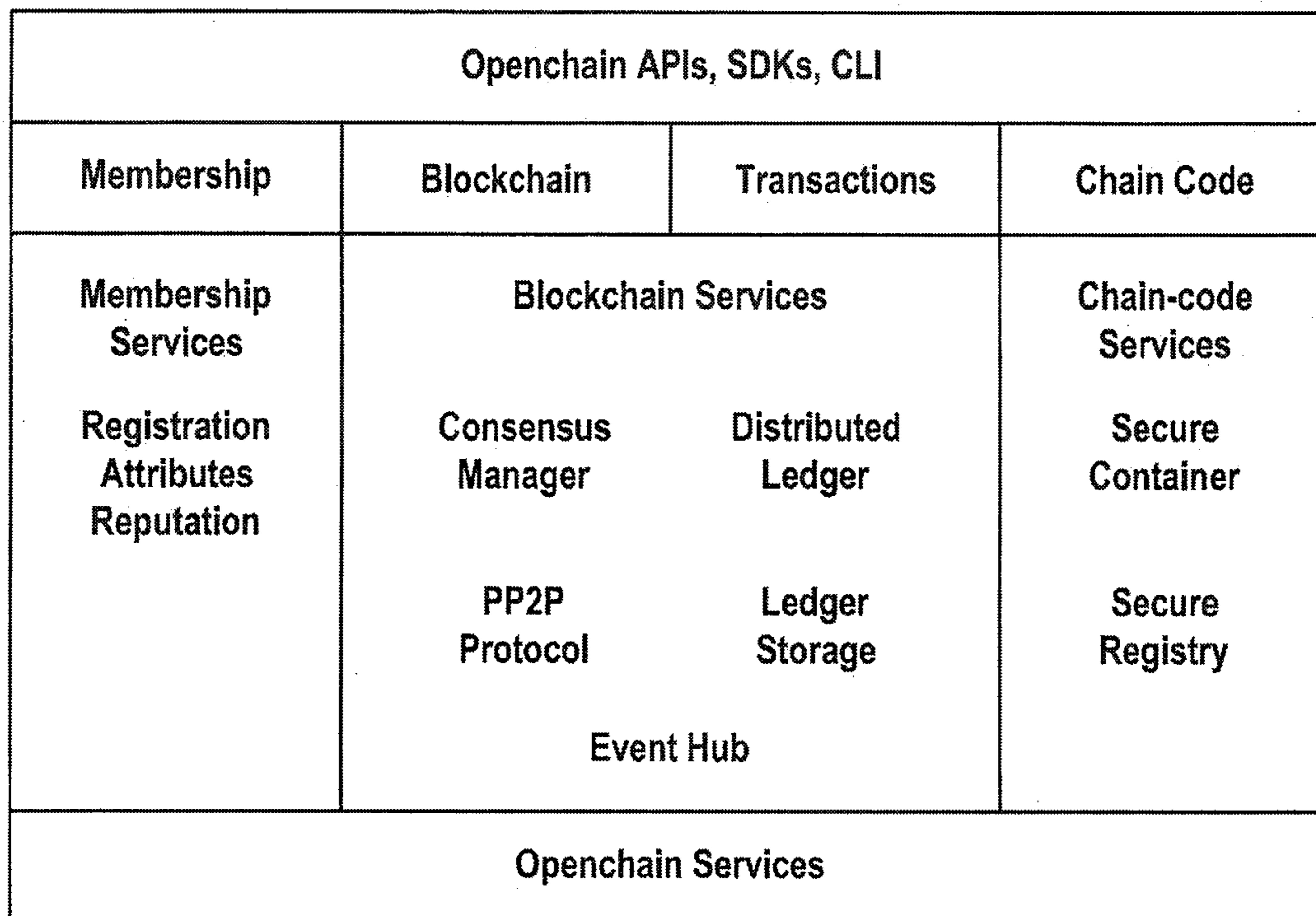
Platform
