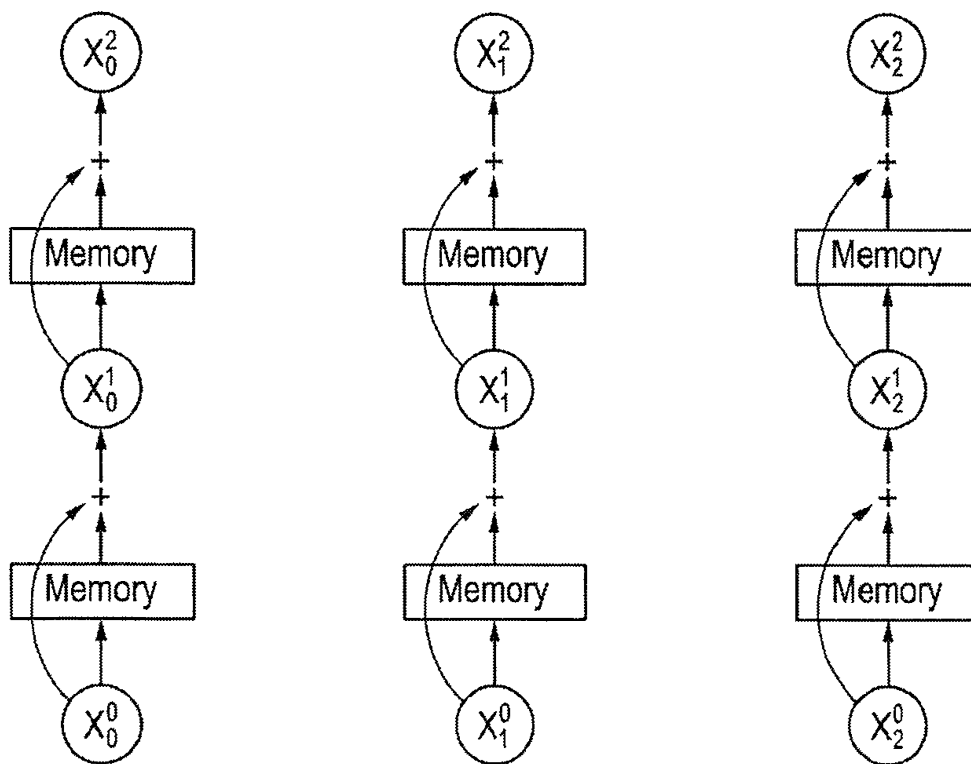
Neural Network
