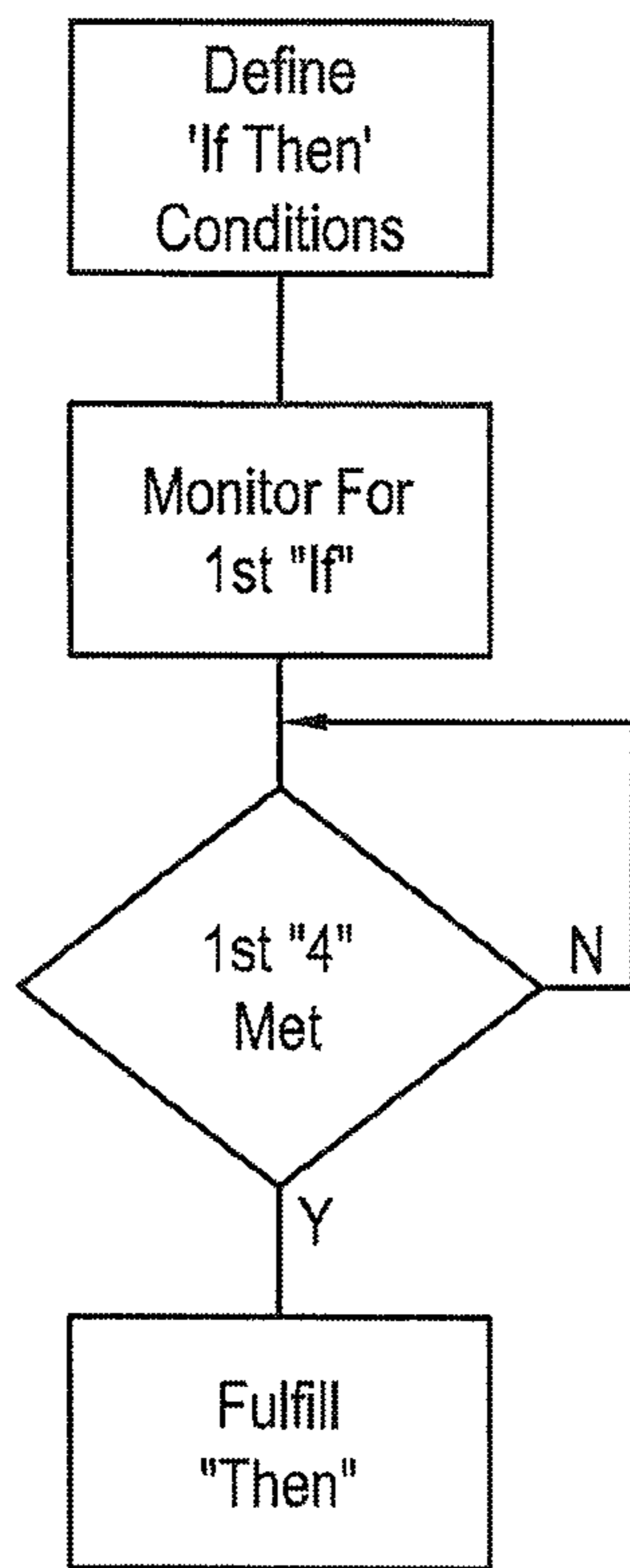
Smart Contract
