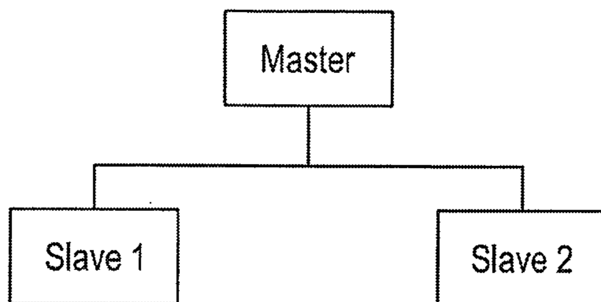
Hierarchical Systems
