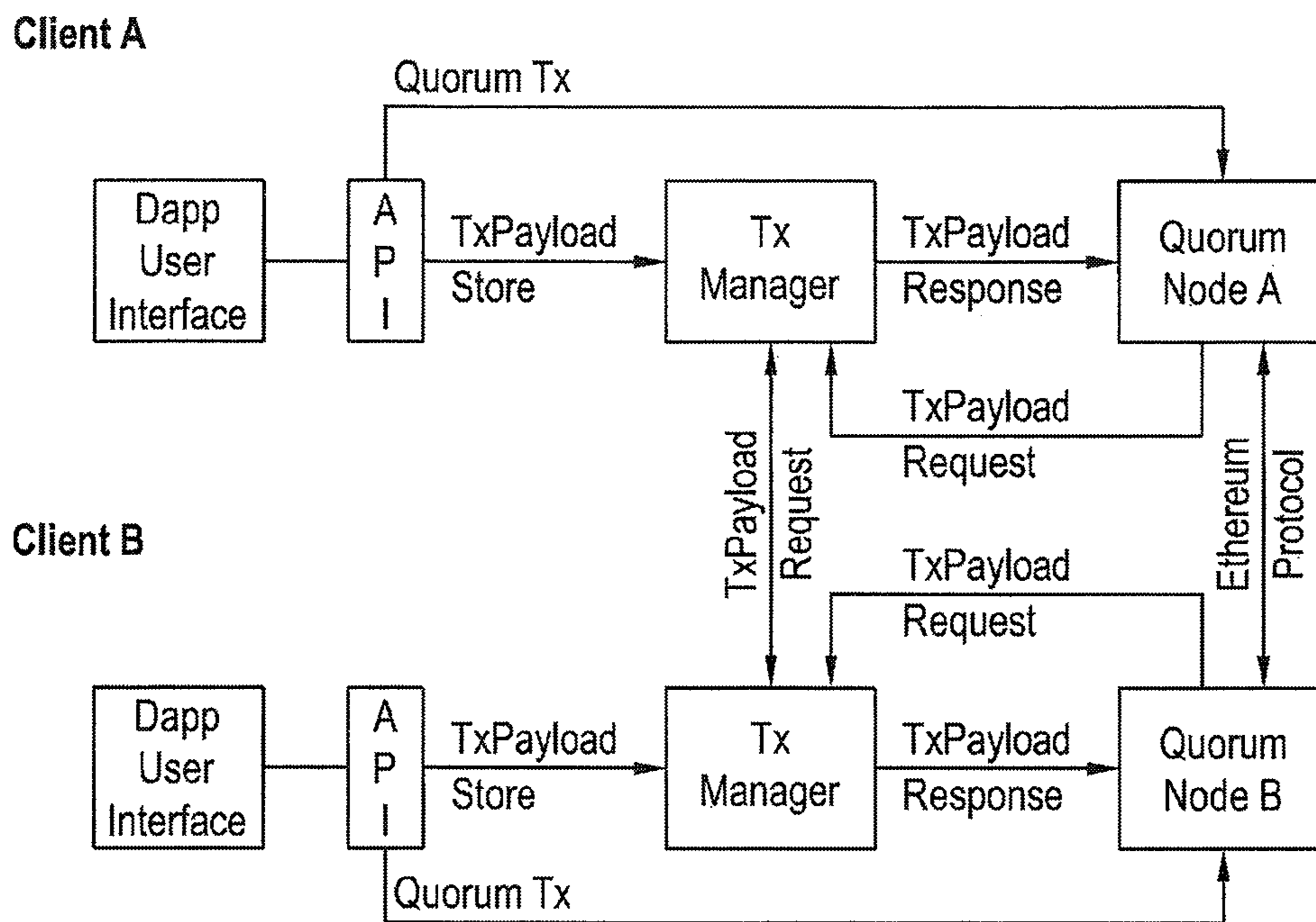
Permissioned System
