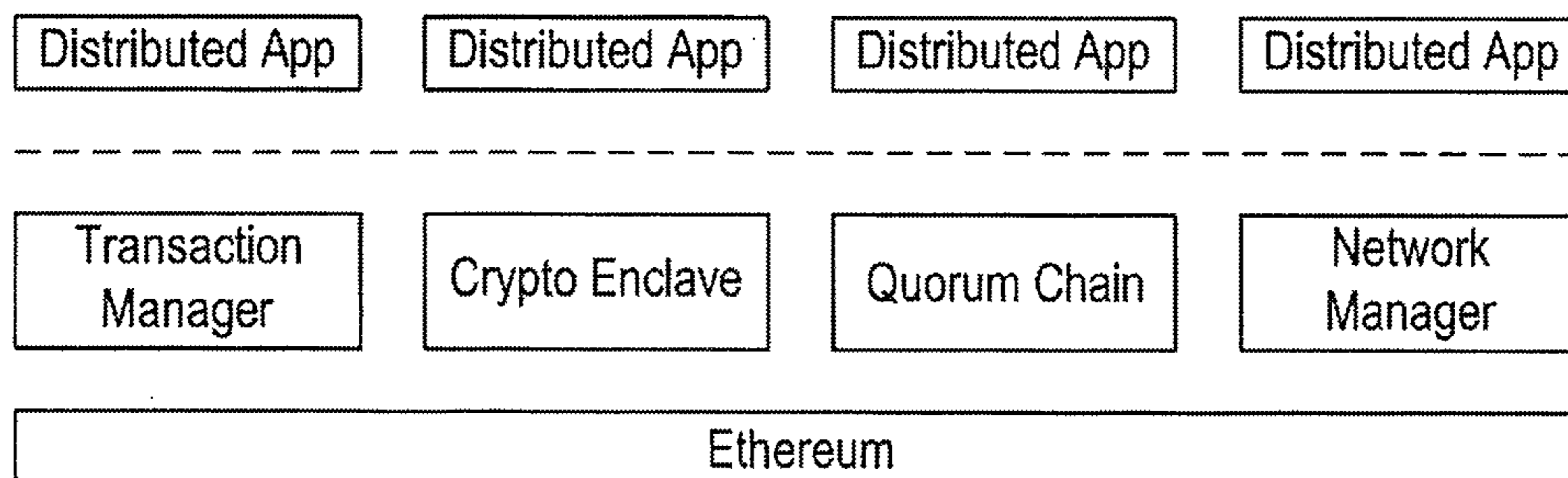
Architecture
