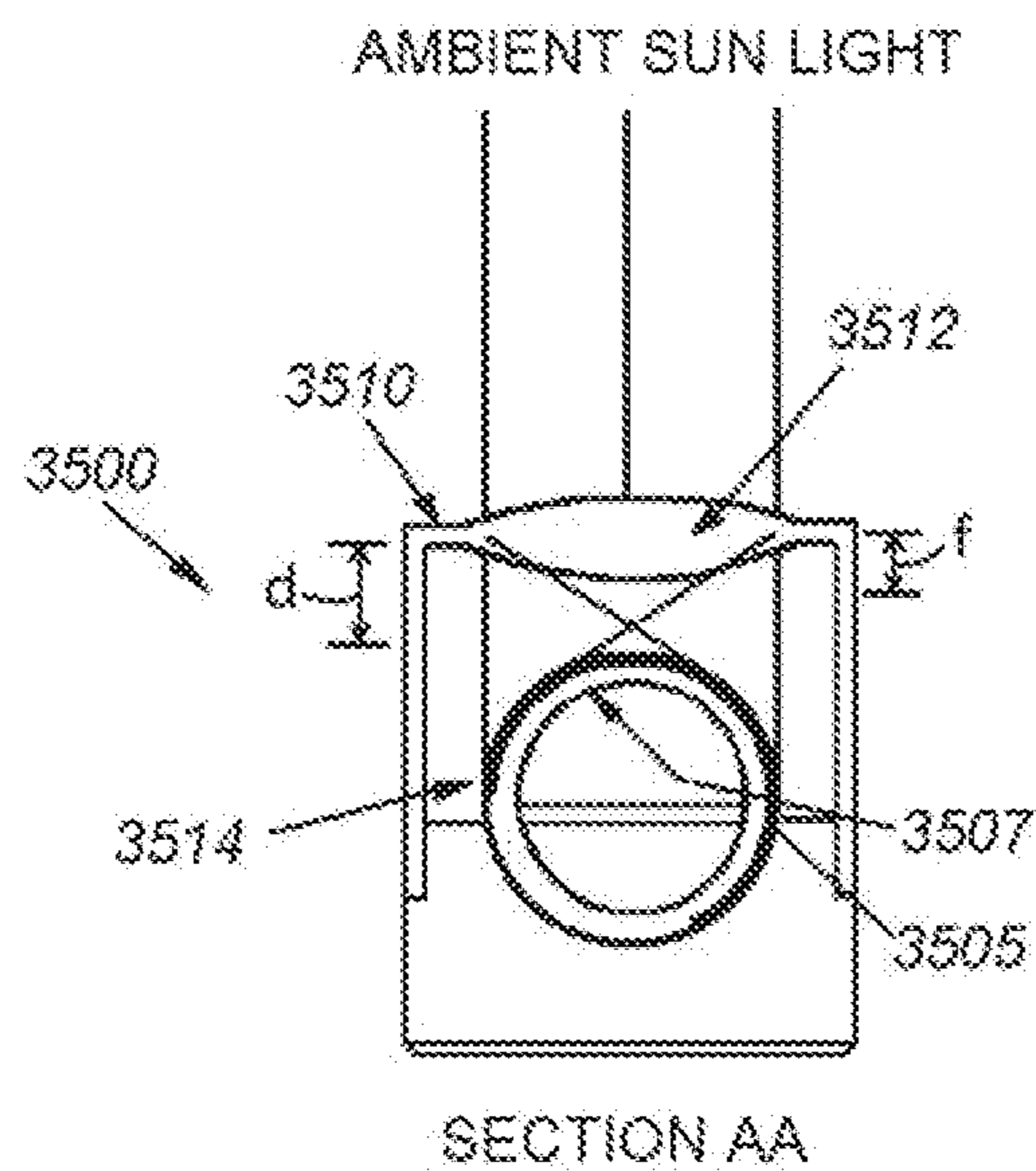
SECTION AA FIG. 35C
