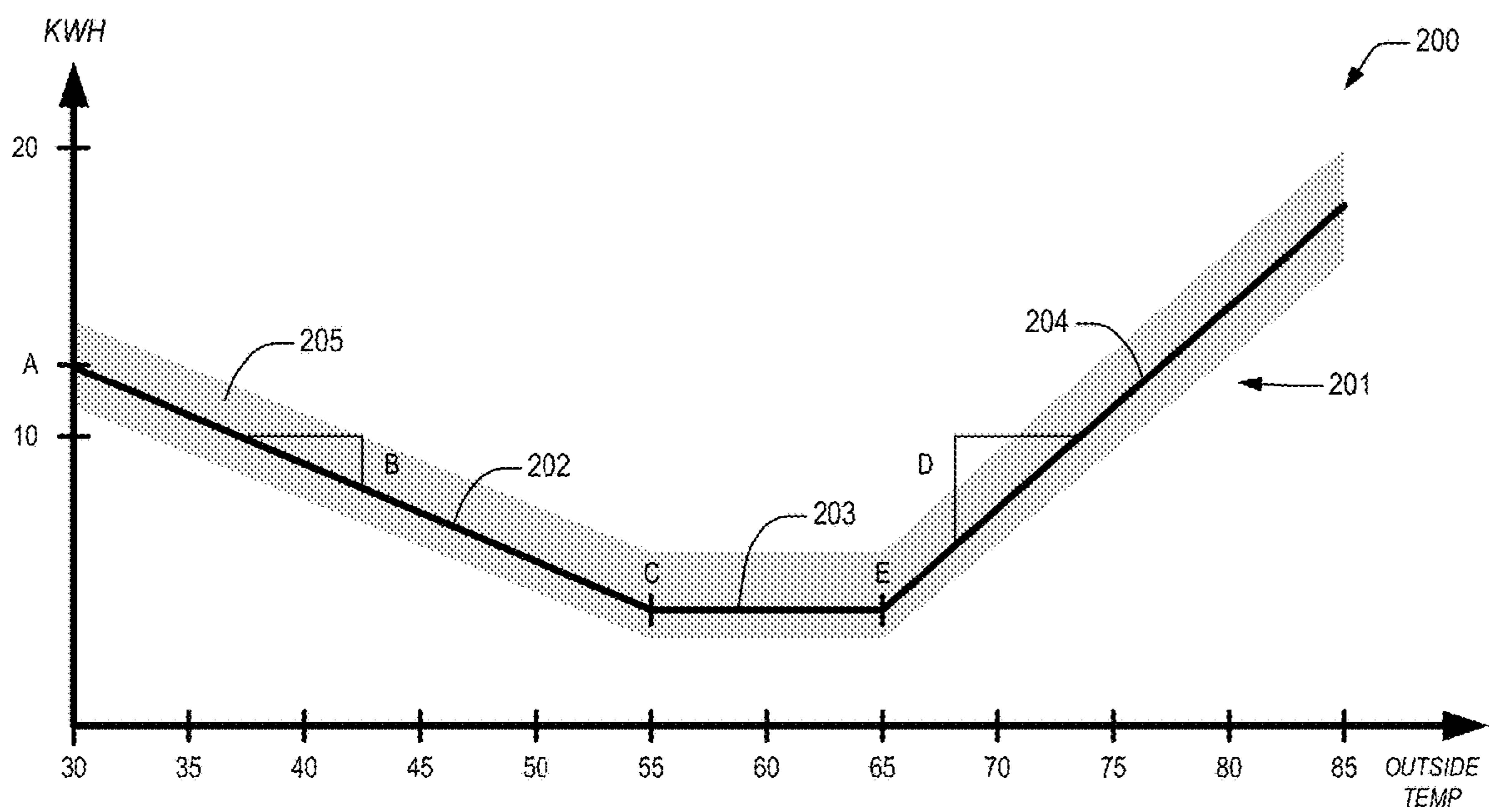
COARSE-GRAINED 5-PARAMETER REGRESSION BASELINE MODEL
