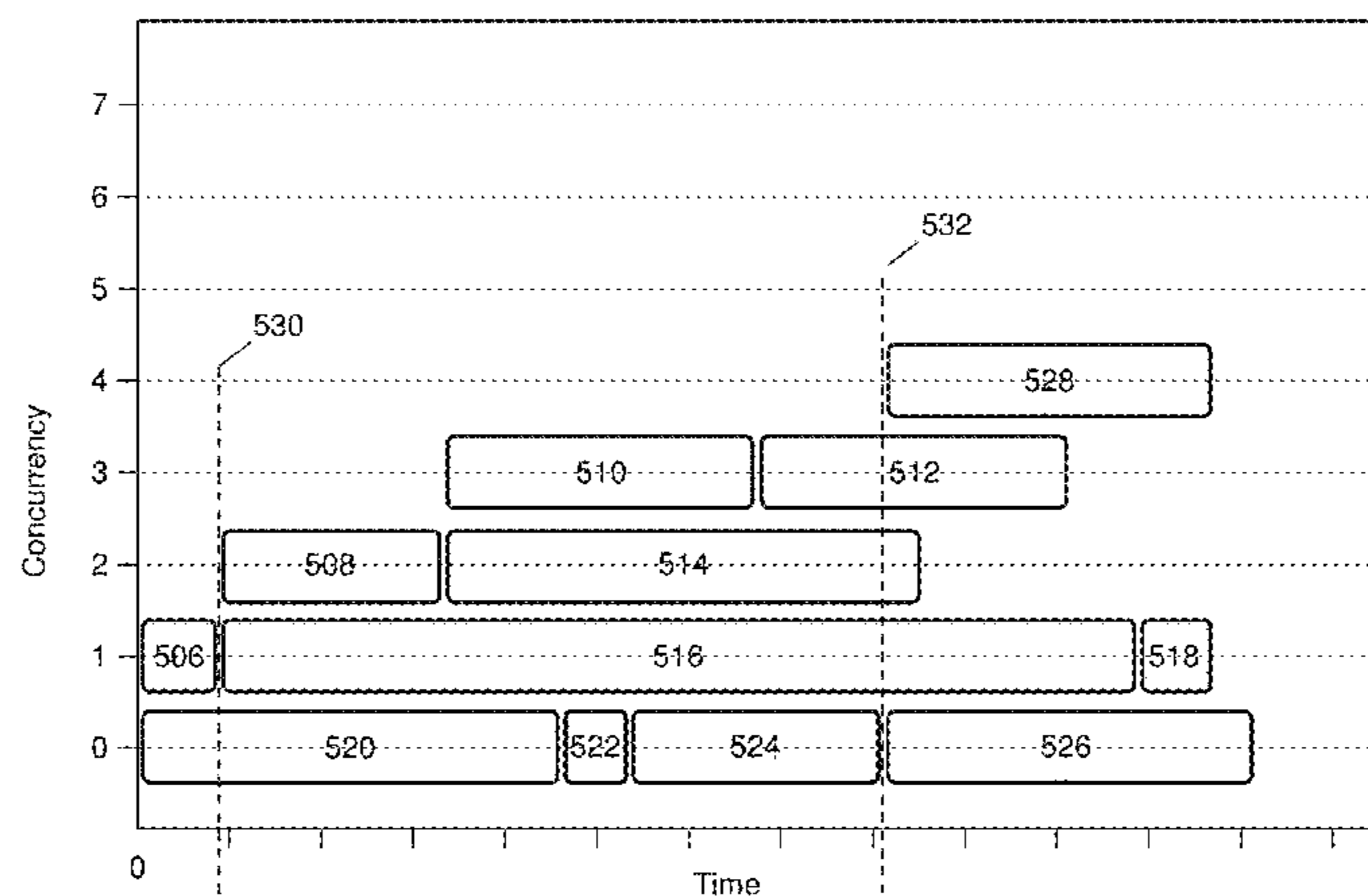
Performance Visualization 500
