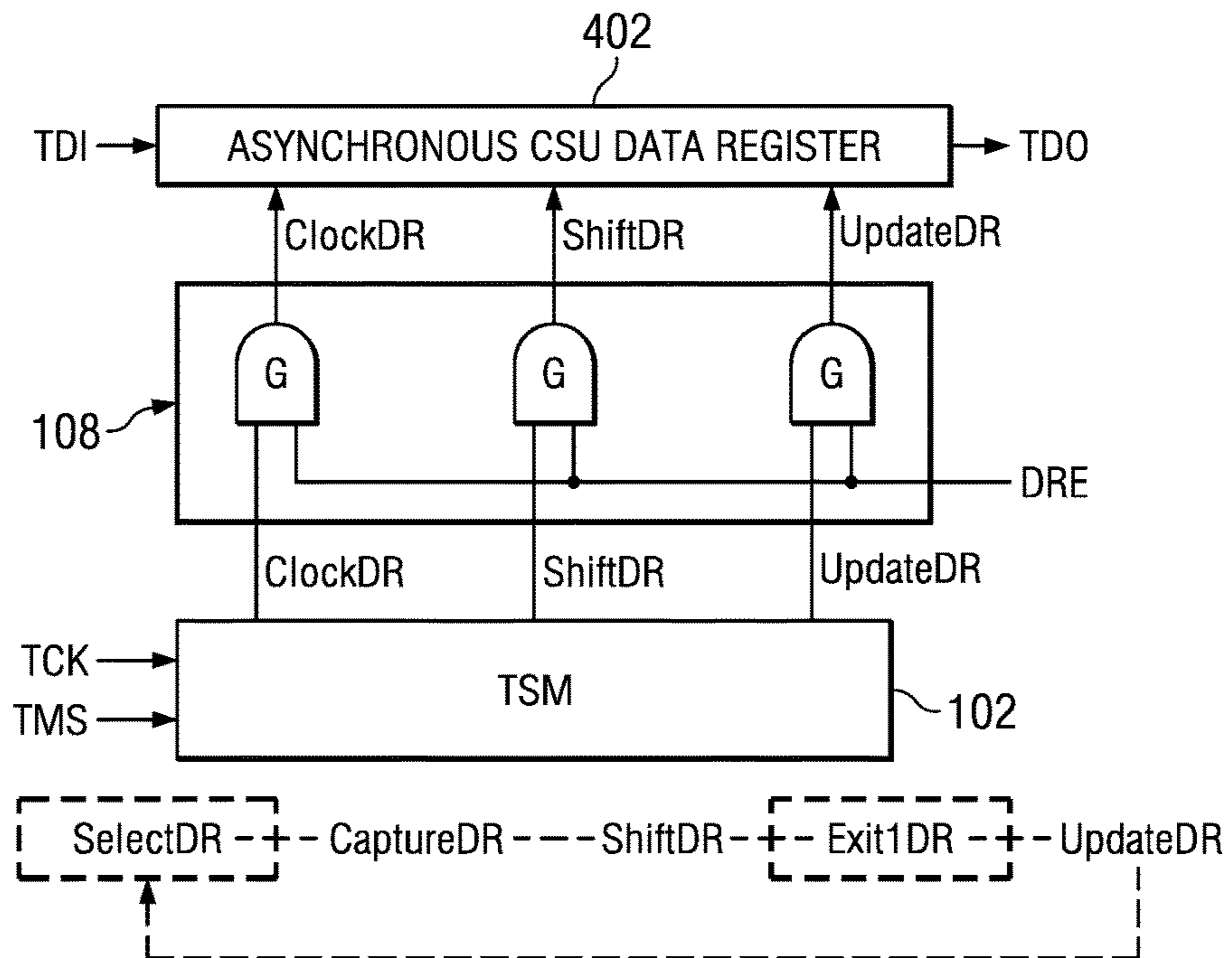
FIG. 4 (PRIOR ART)
