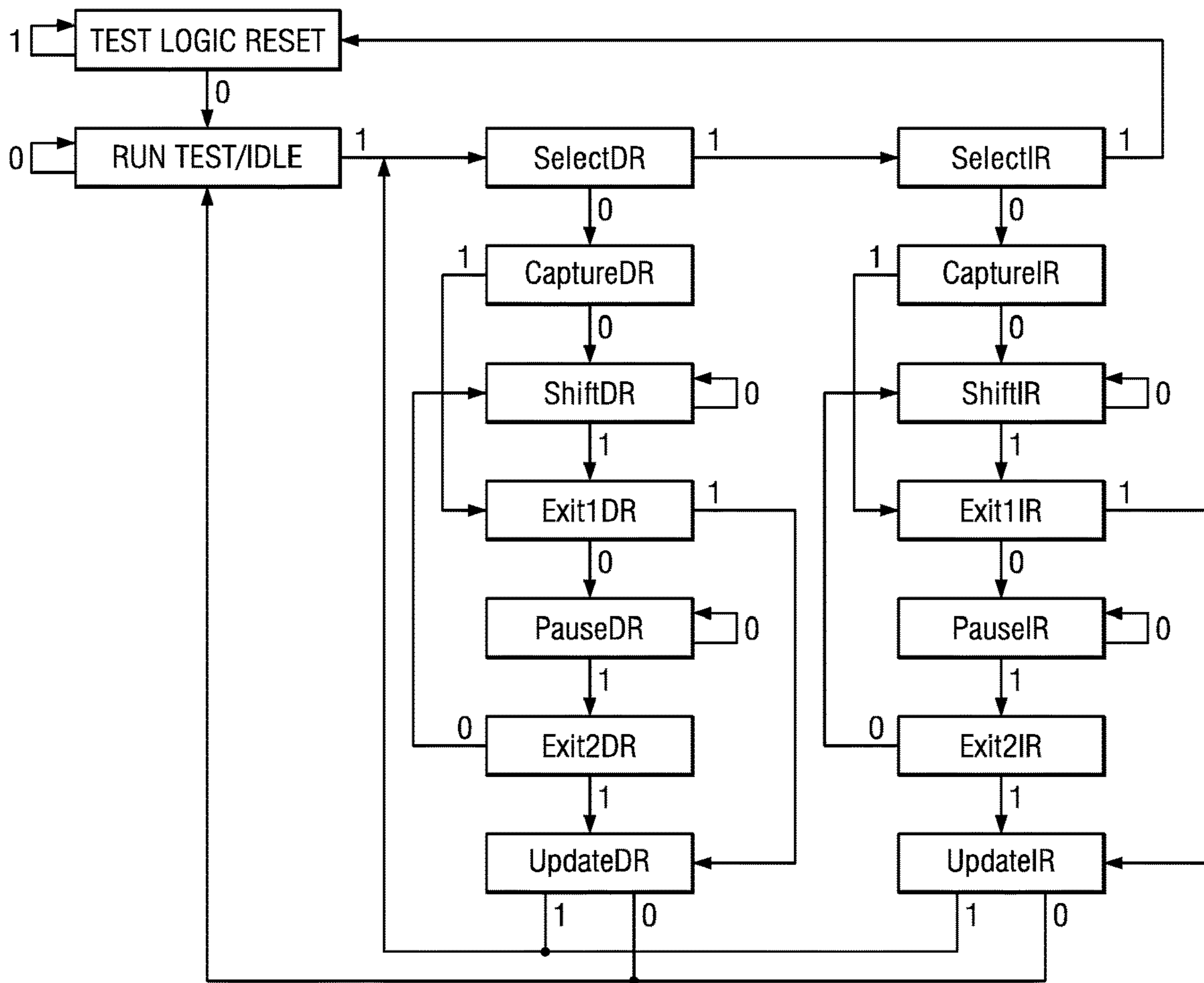
FIG. 3 (PRIOR ART)
