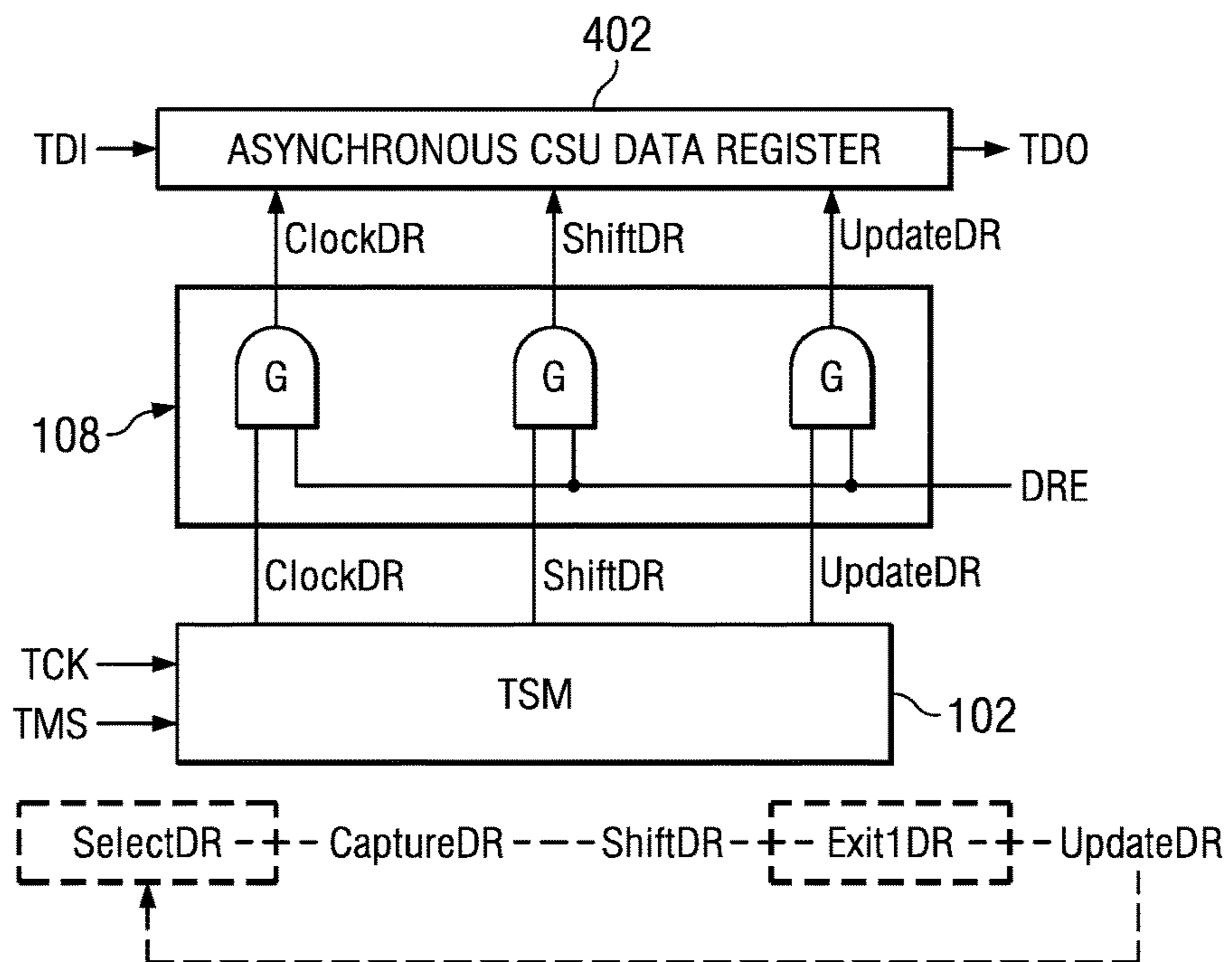
FIG. 4 (PRIOR ART)
