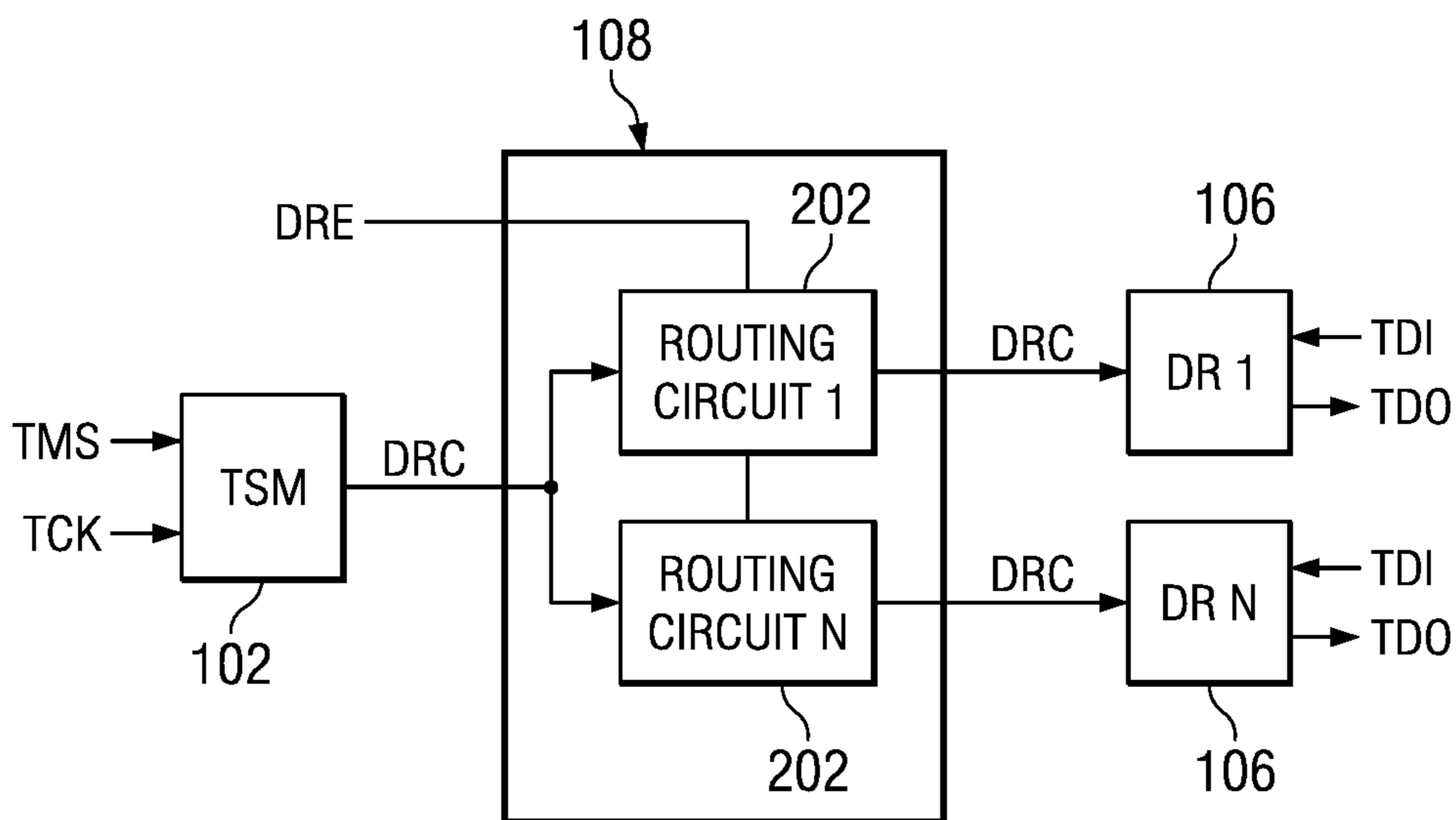
FIG. 2 (PRIOR ART)
