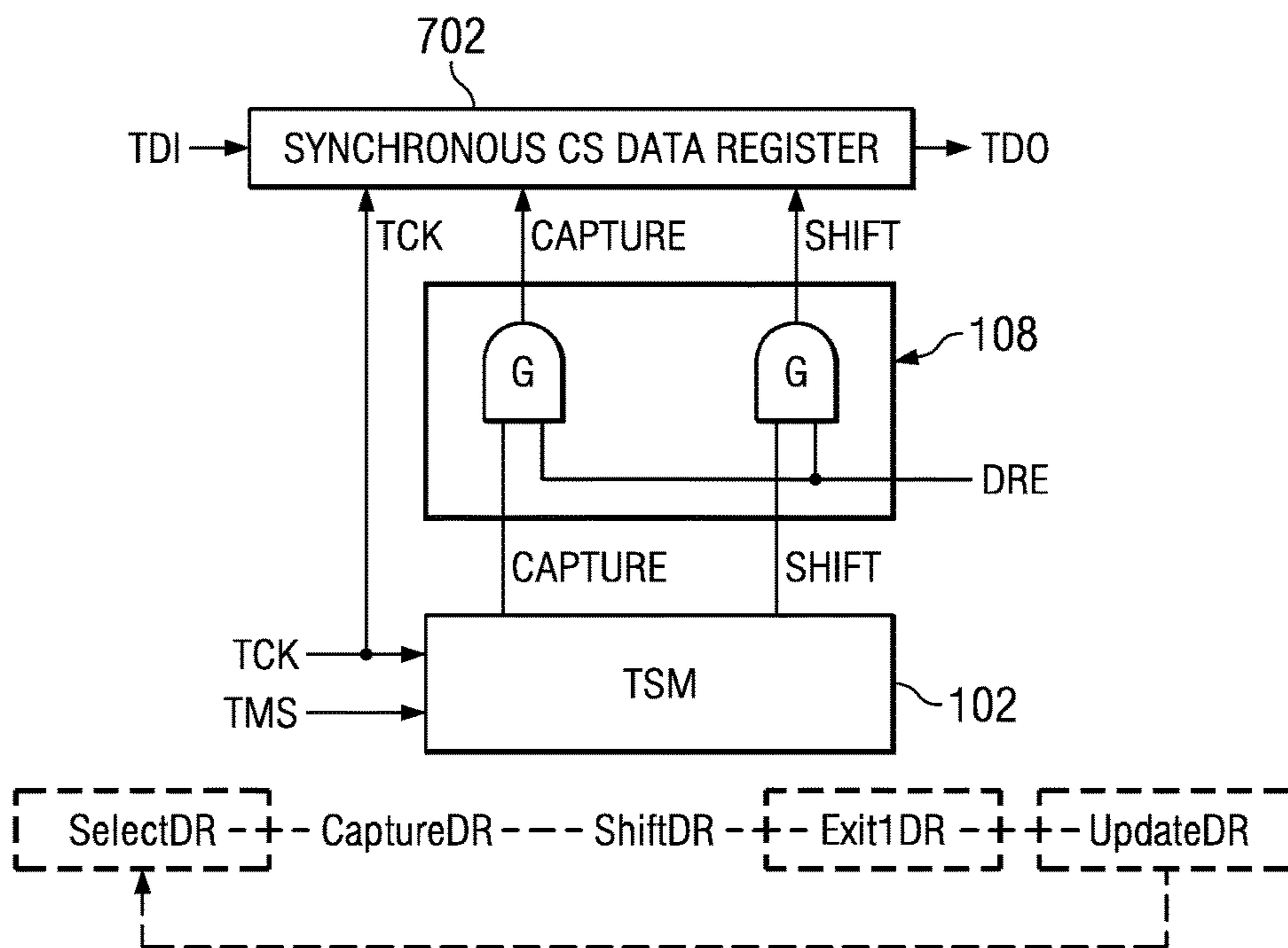
FIG. 7 (PRIOR ART)
