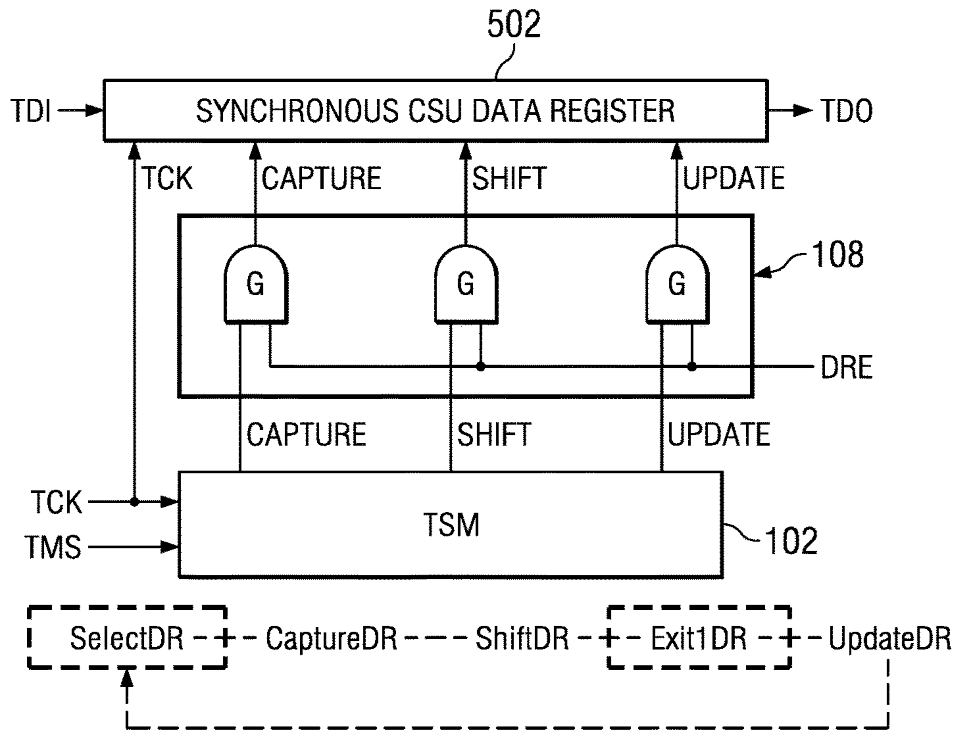
FIG. 5 (PRIOR ART)
