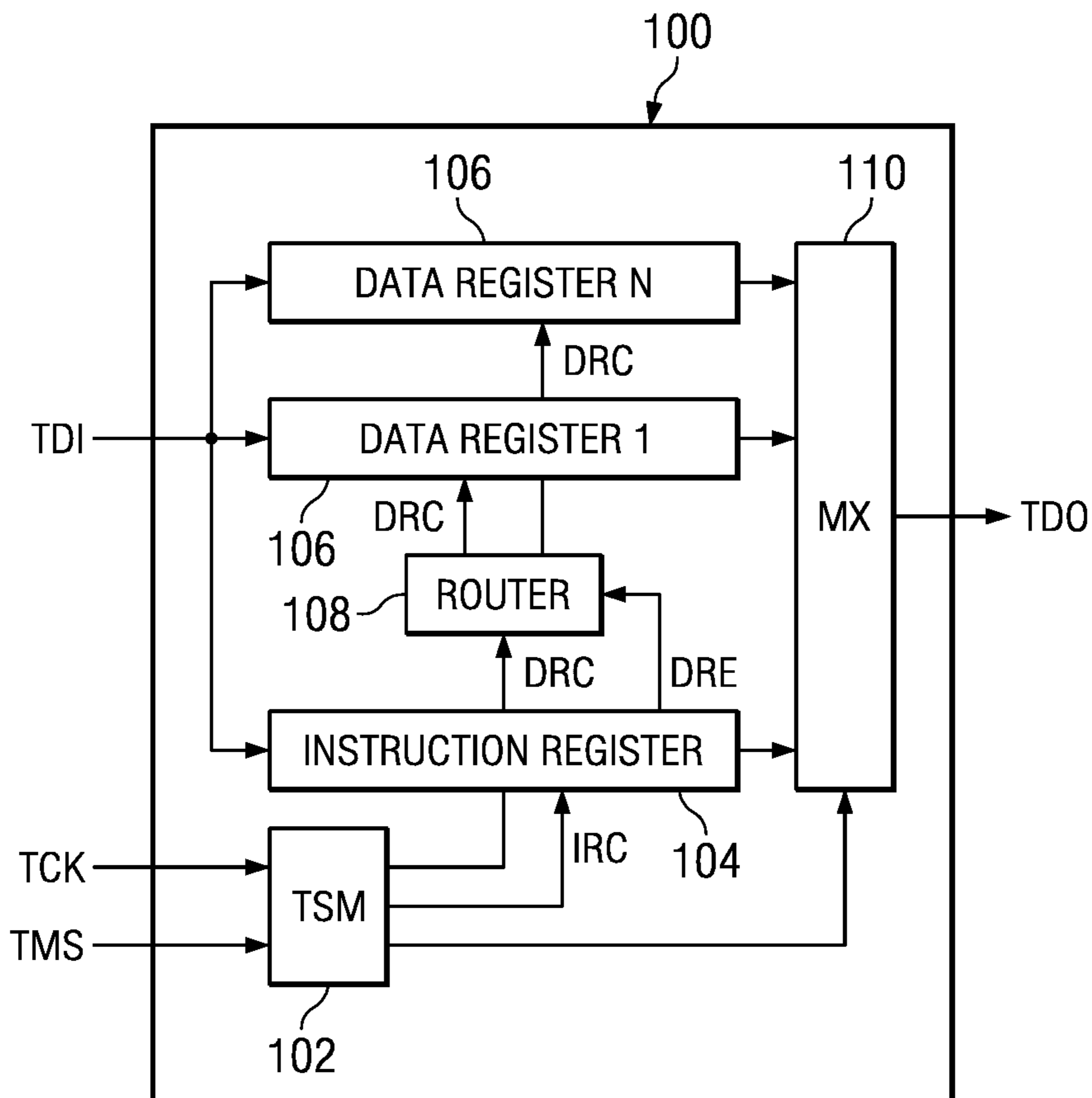
FIG. 1 (PRIOR ART)
