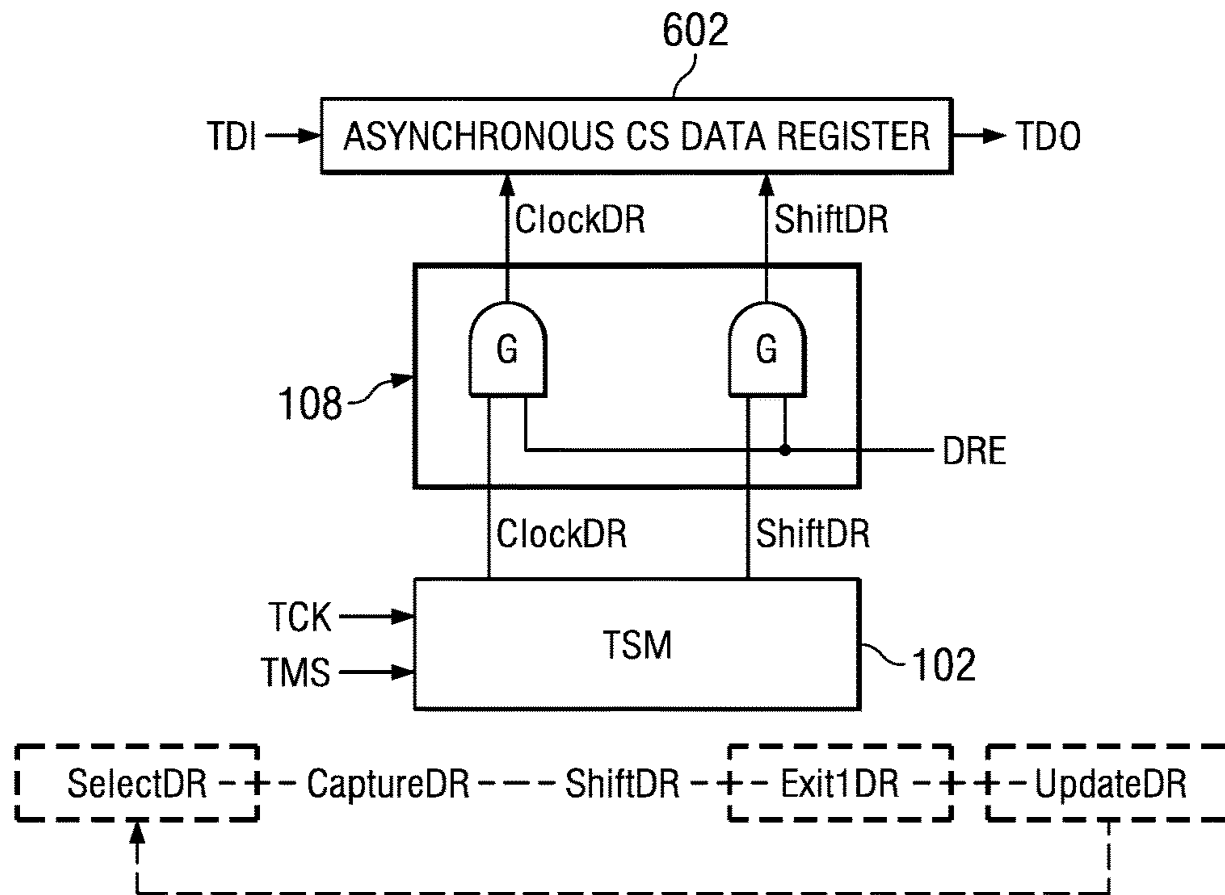
FIG. 6 (PRIOR ART)
