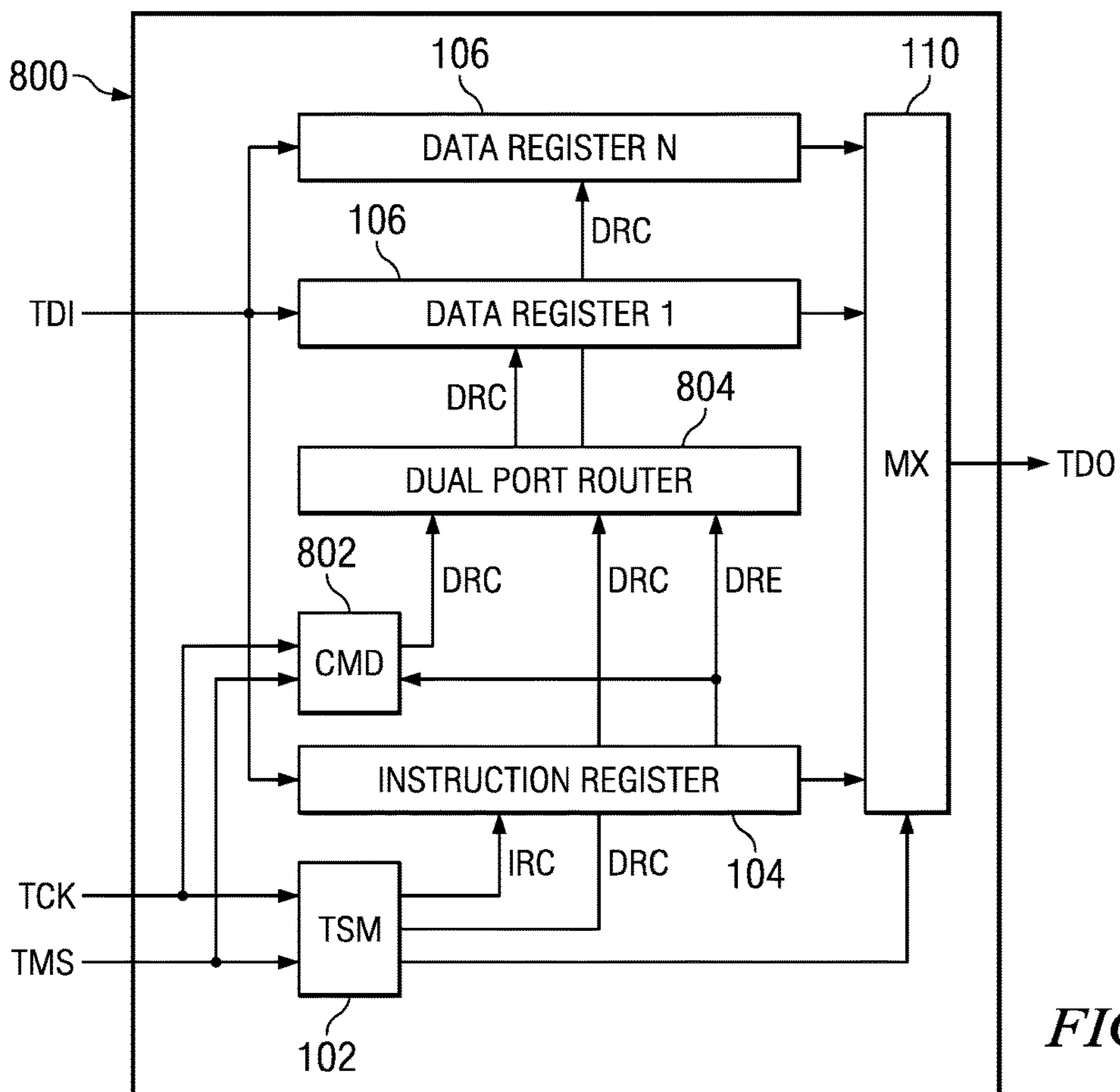
FIG. 7 (PRIOR ART)
