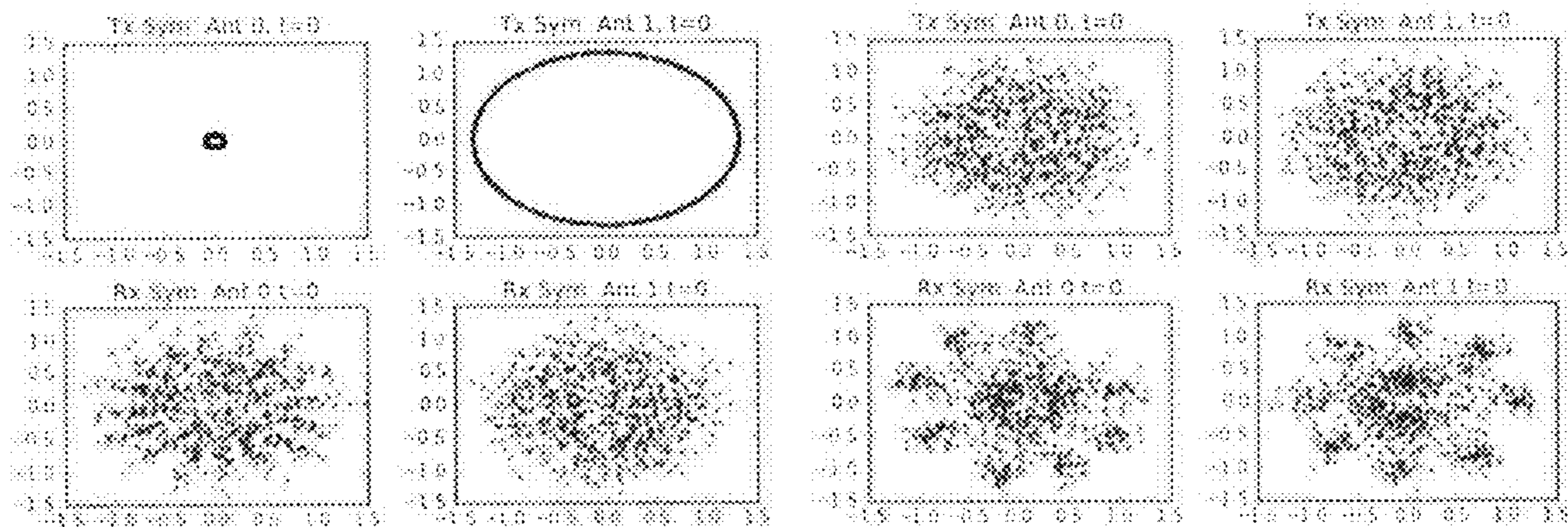
Learned 2x2 Scheme 1-bit CSI Random Channels
