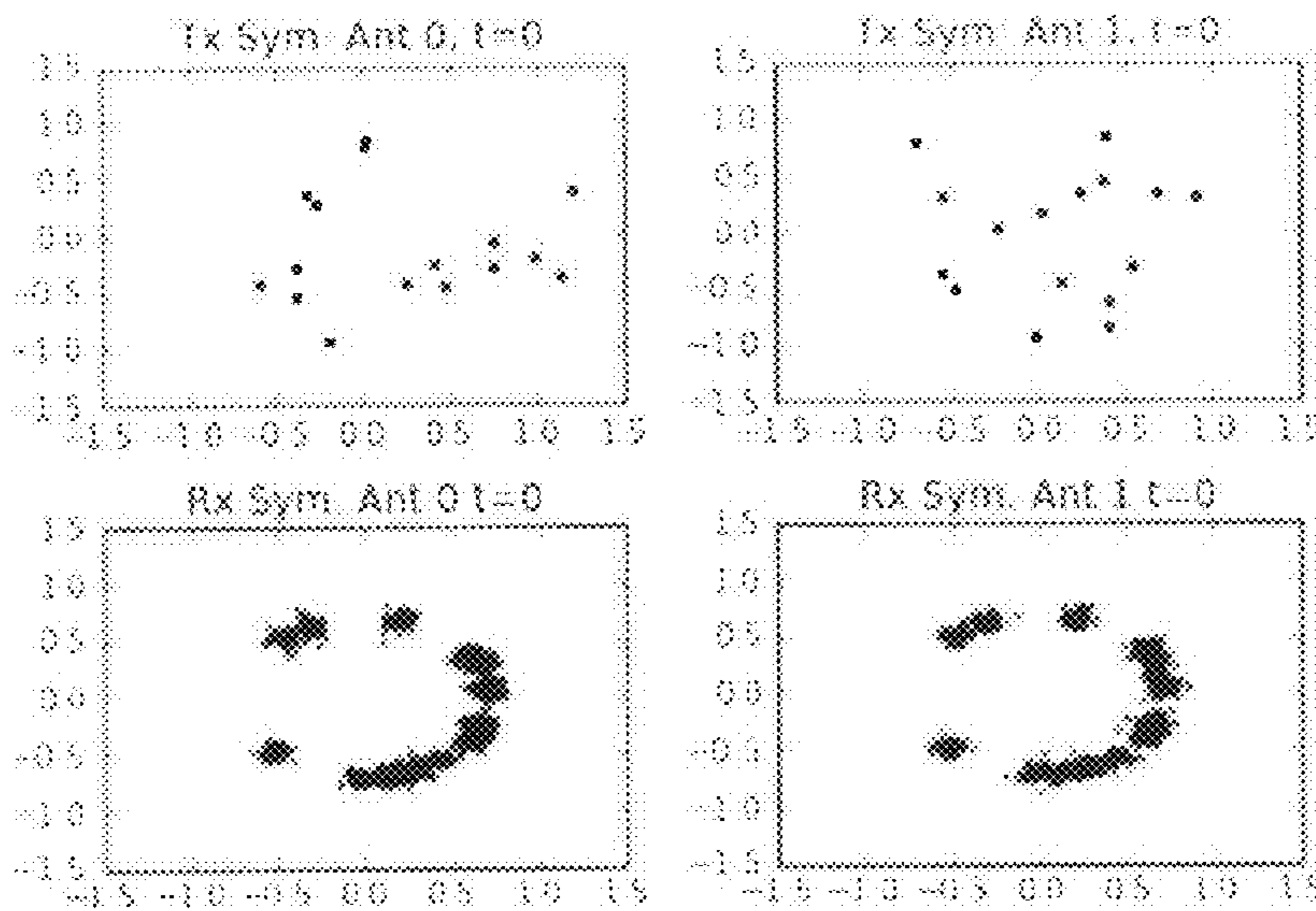
Learned 2x2 Scheme, All-Ones Channel.
