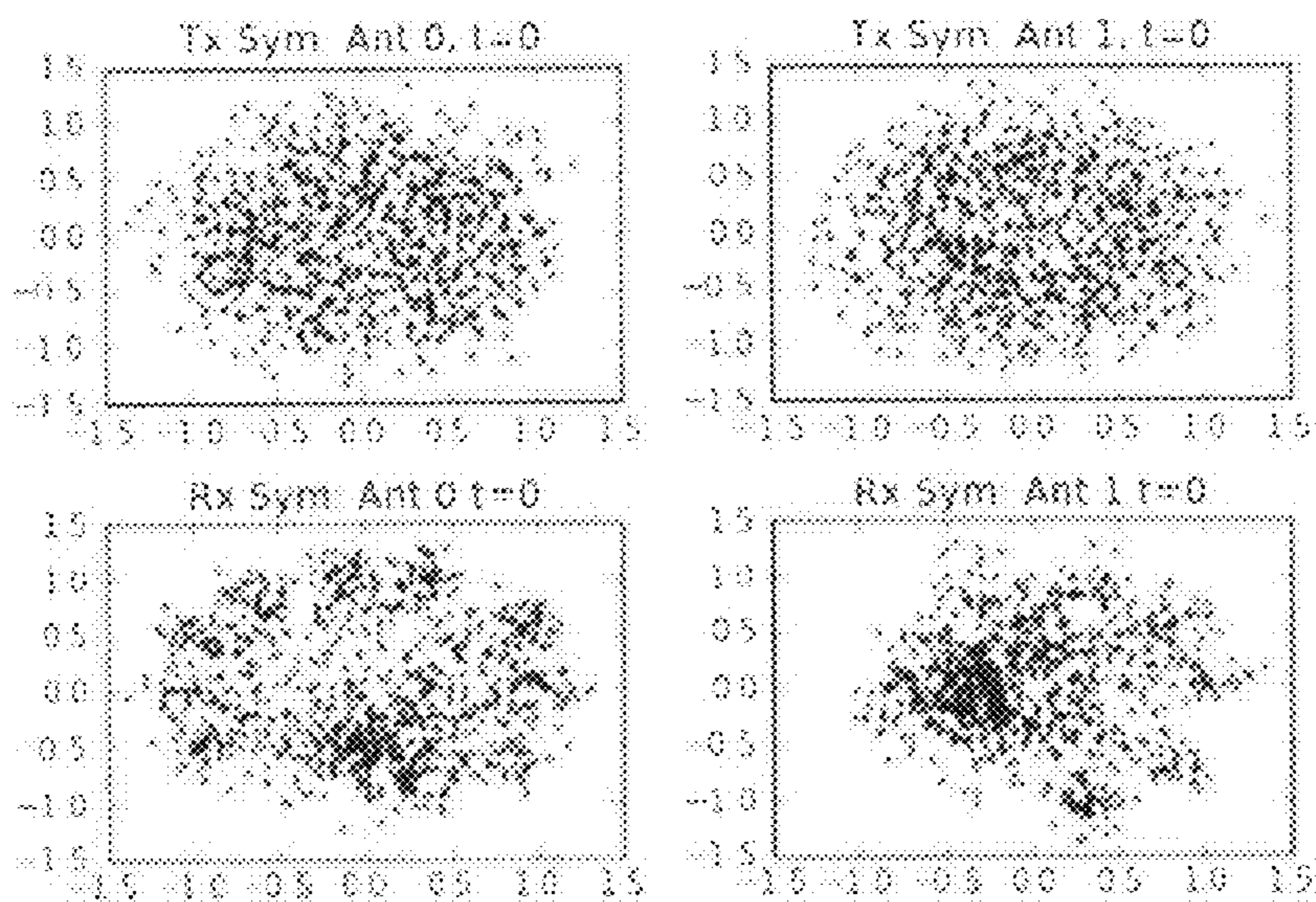
Learned 2x2 Scheme, Random Channels.
