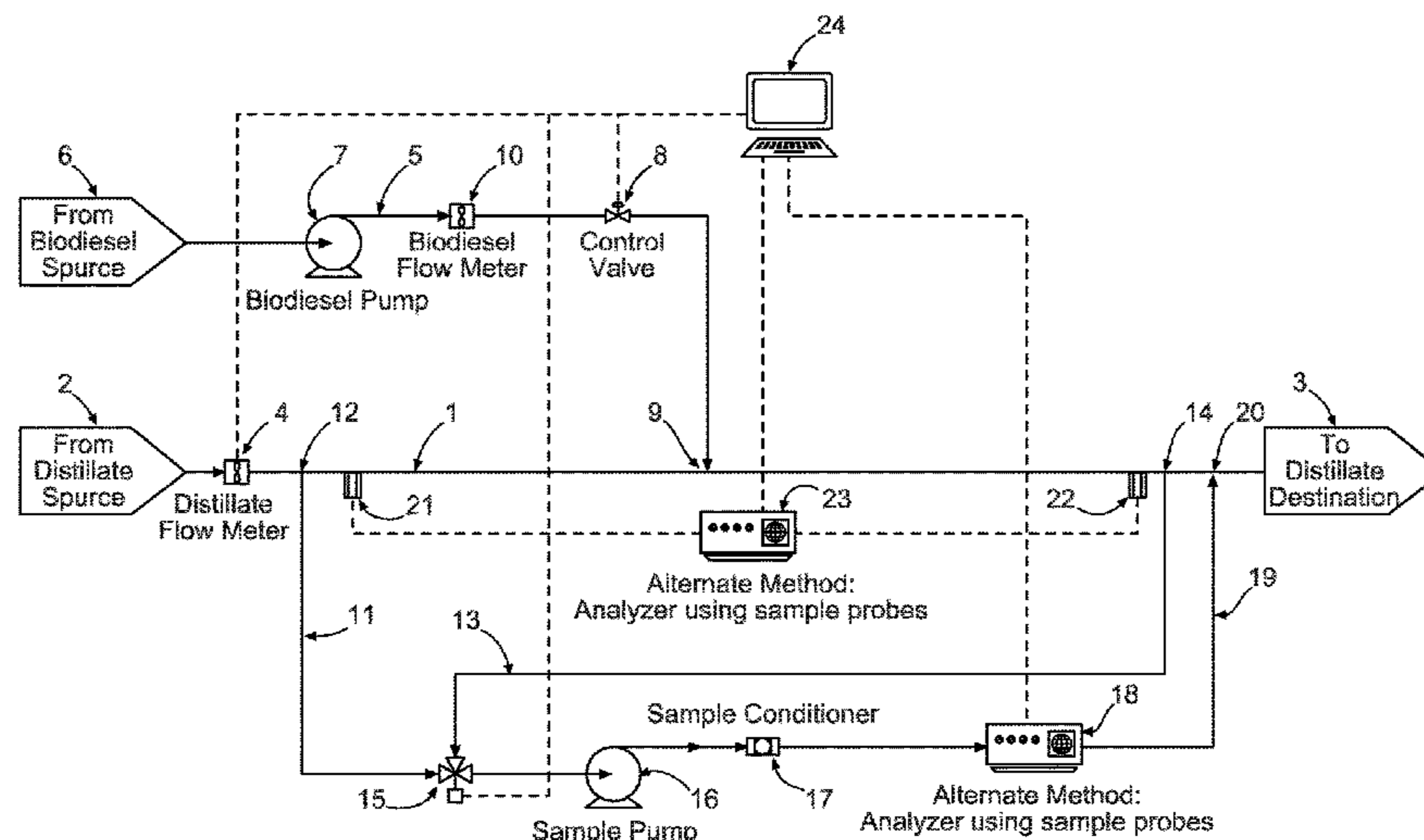
Controlled Blending of Biodiesel into Distillate Streams
