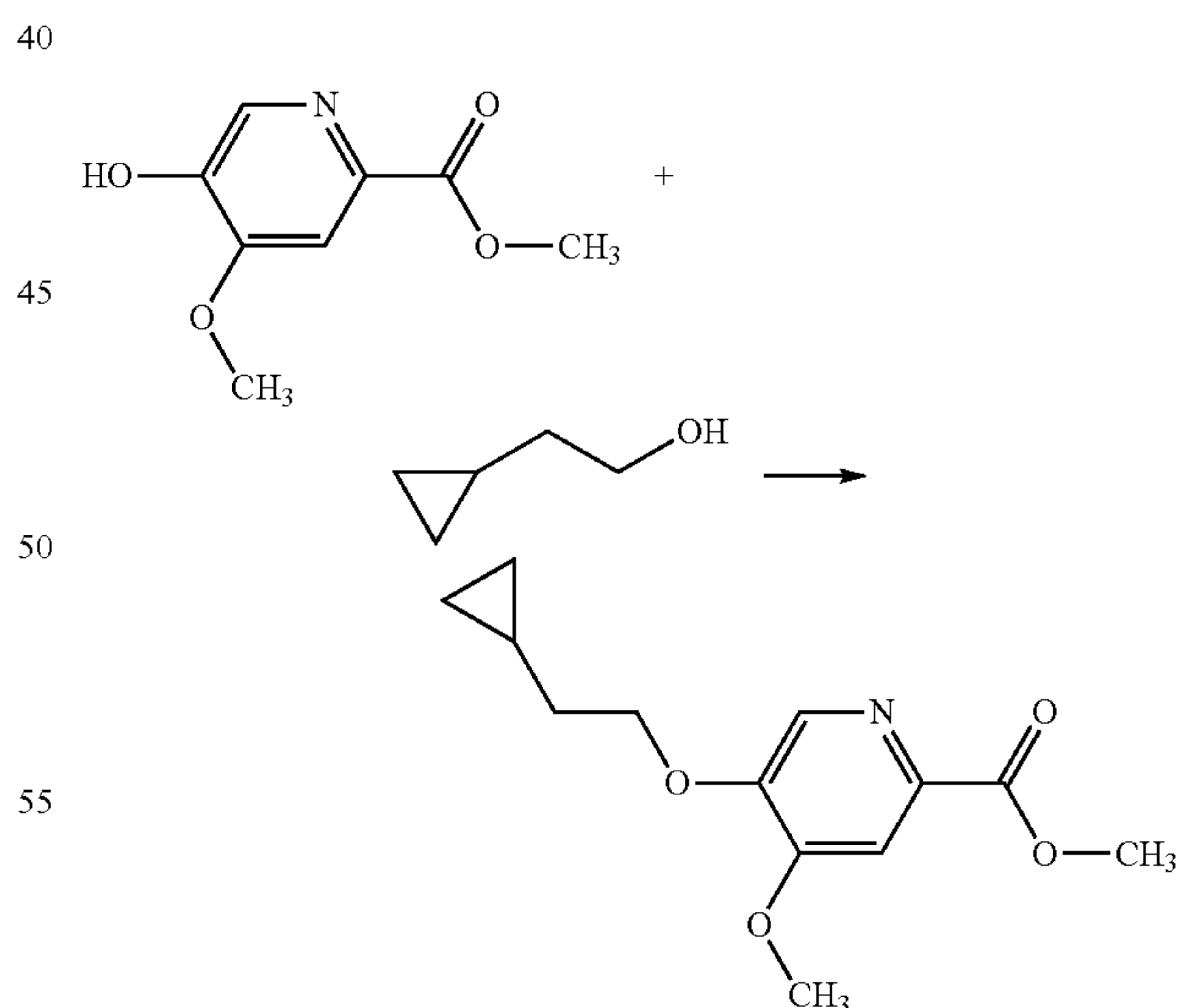
5-(2-Cyclopropyl-ethoxy)-4-methoxy-pyridine-2- carboxylic acid methyl ester
