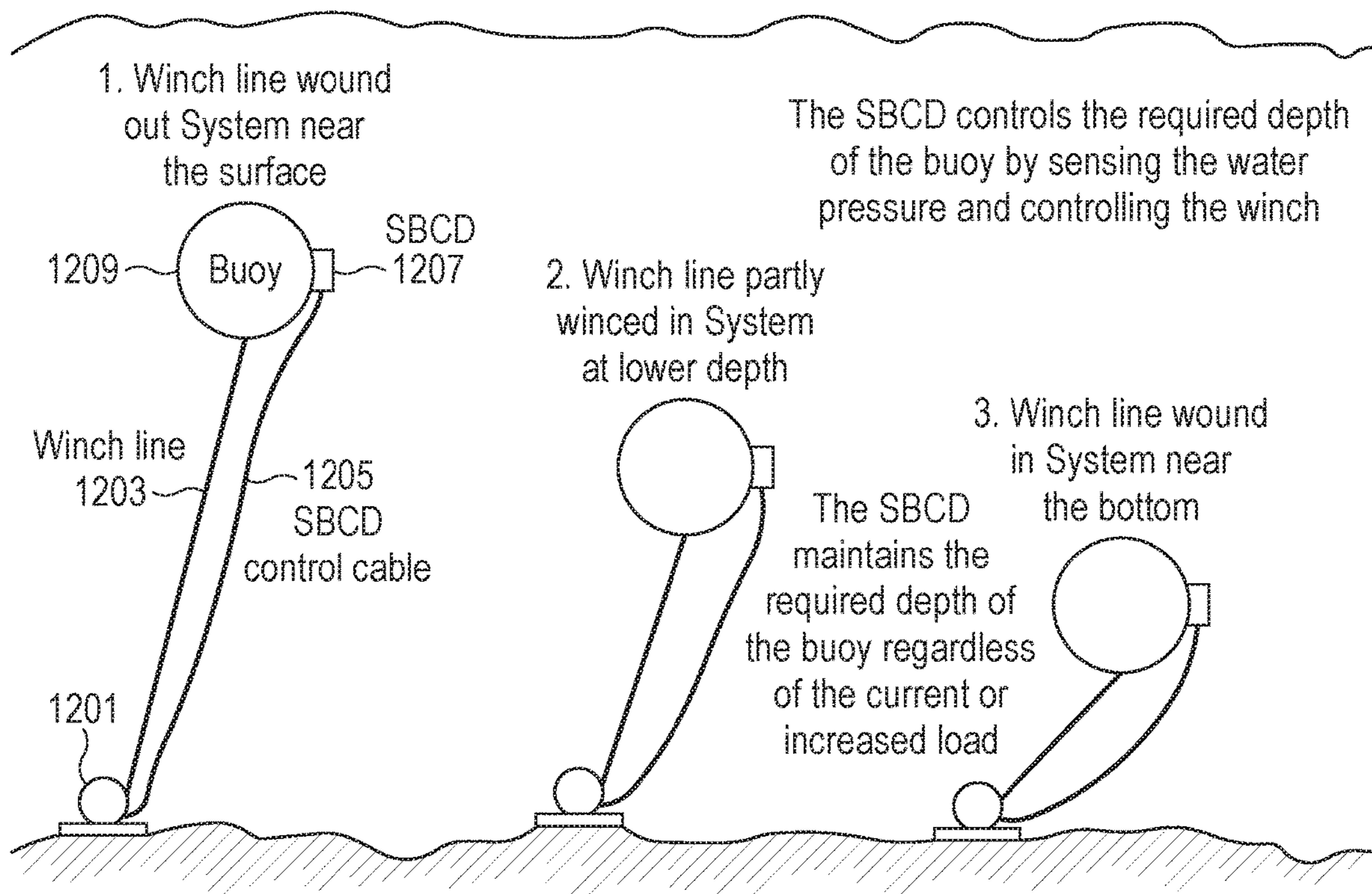
SBCD controlled winch
