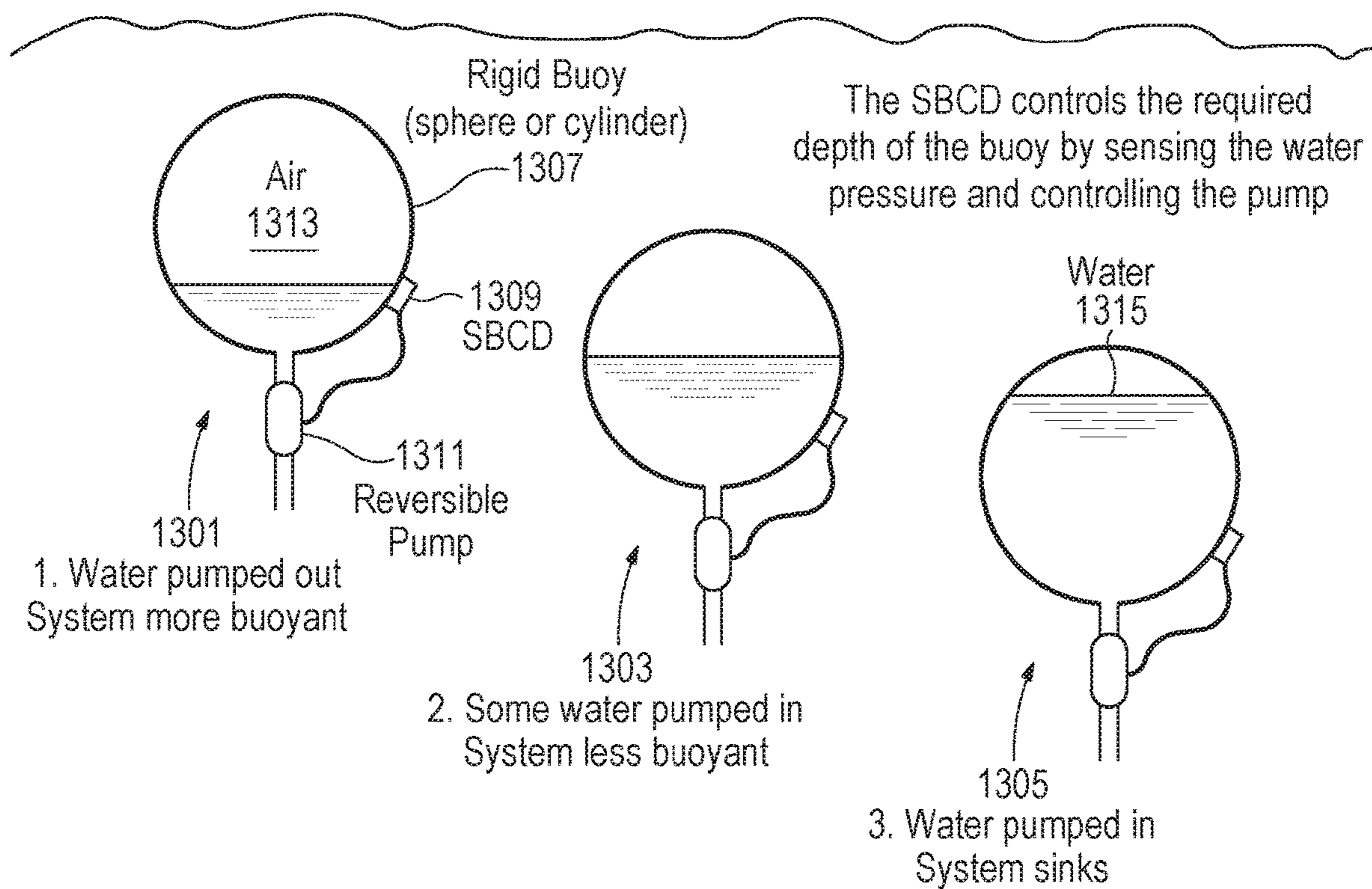
Rigid shell buoy with SBCD controlled pump
