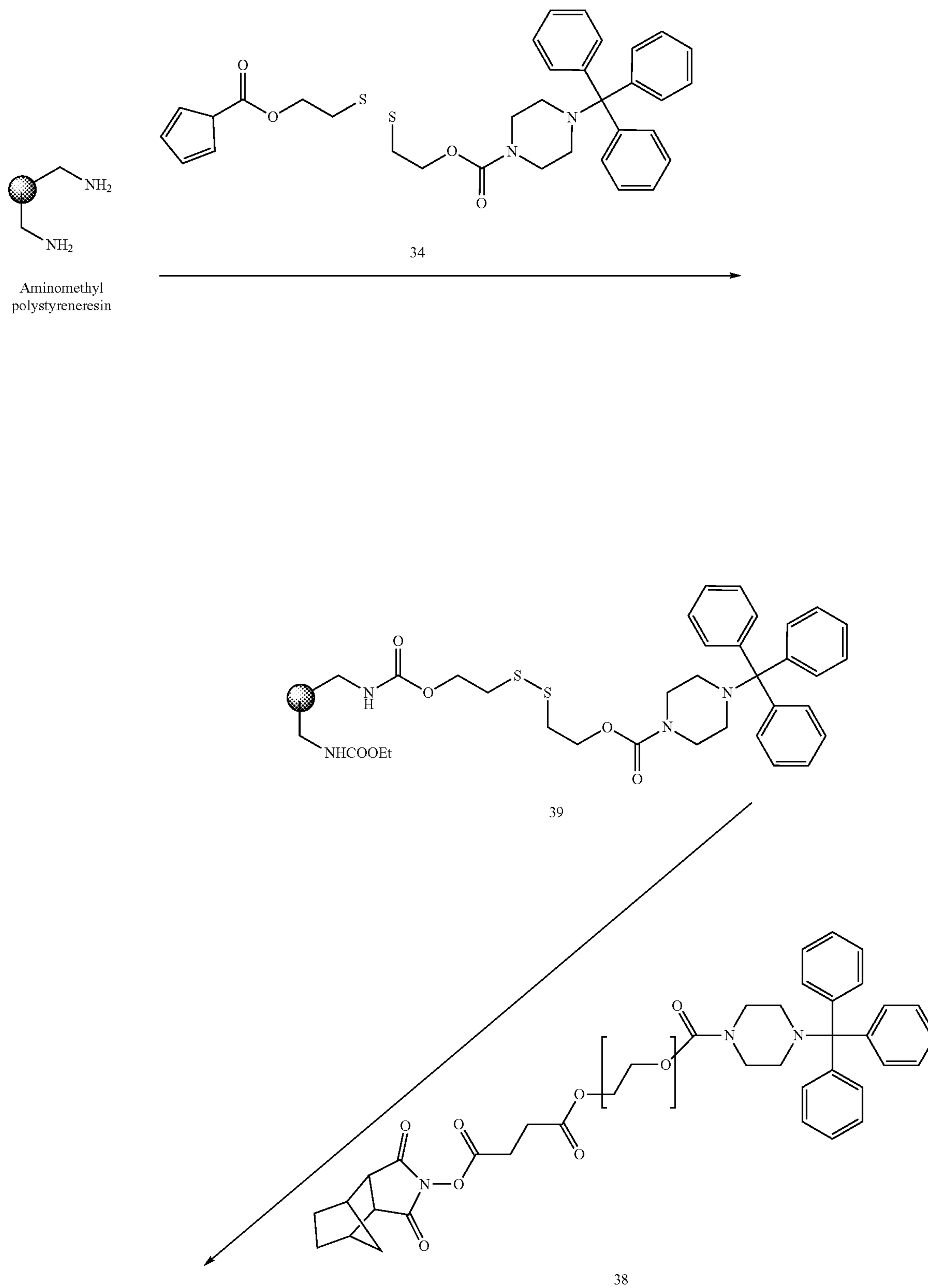
Scheme 3: Preparation of the Solid Support for Synthesis of Morpholino Oligomers
