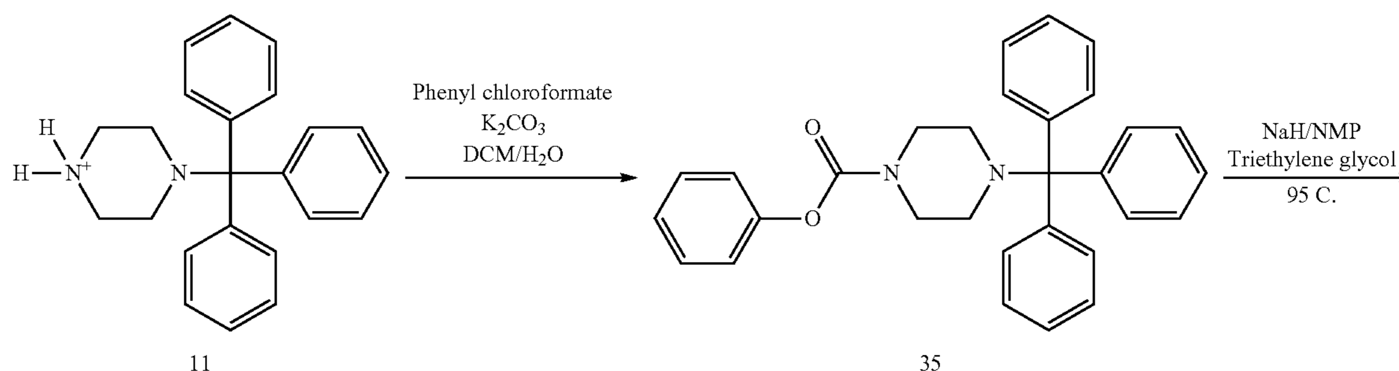
Scheme 2: Preparation of Activated Tail Acid
