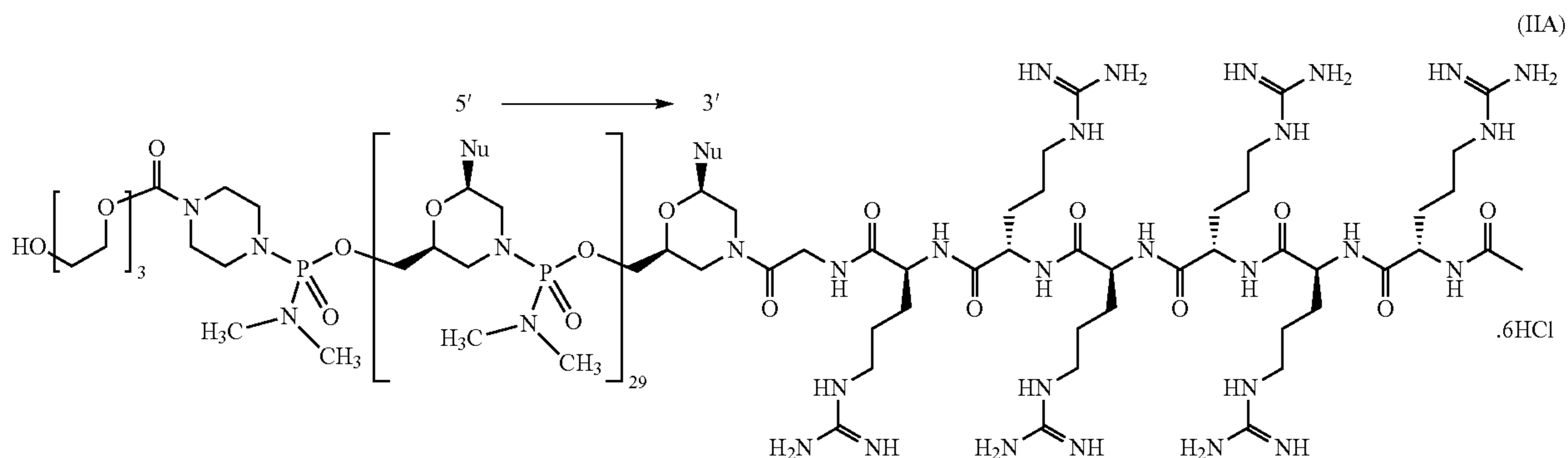
(peptide is SEQ ID NO: 4)
