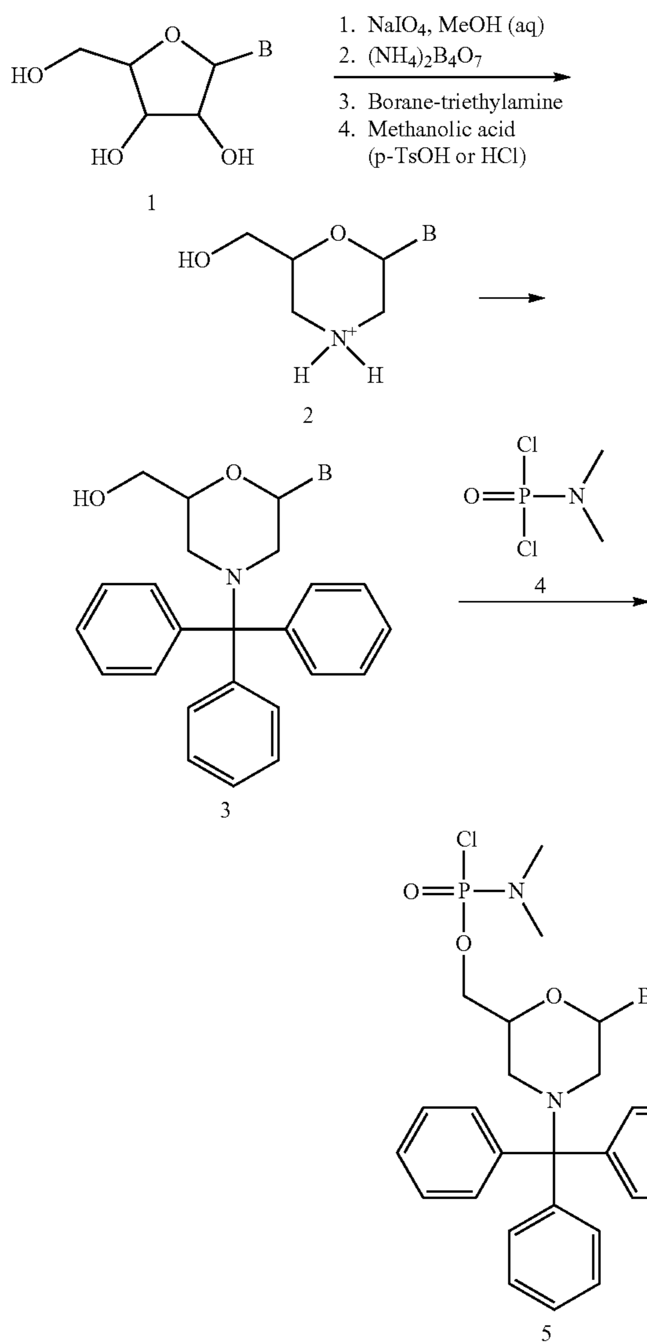
Scheme 1: General synthetic route to PMO Subunits
