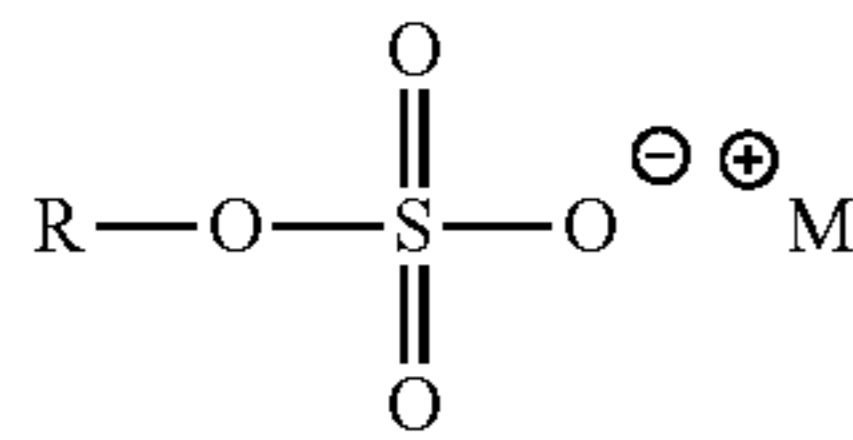
Alkyl sulfates
