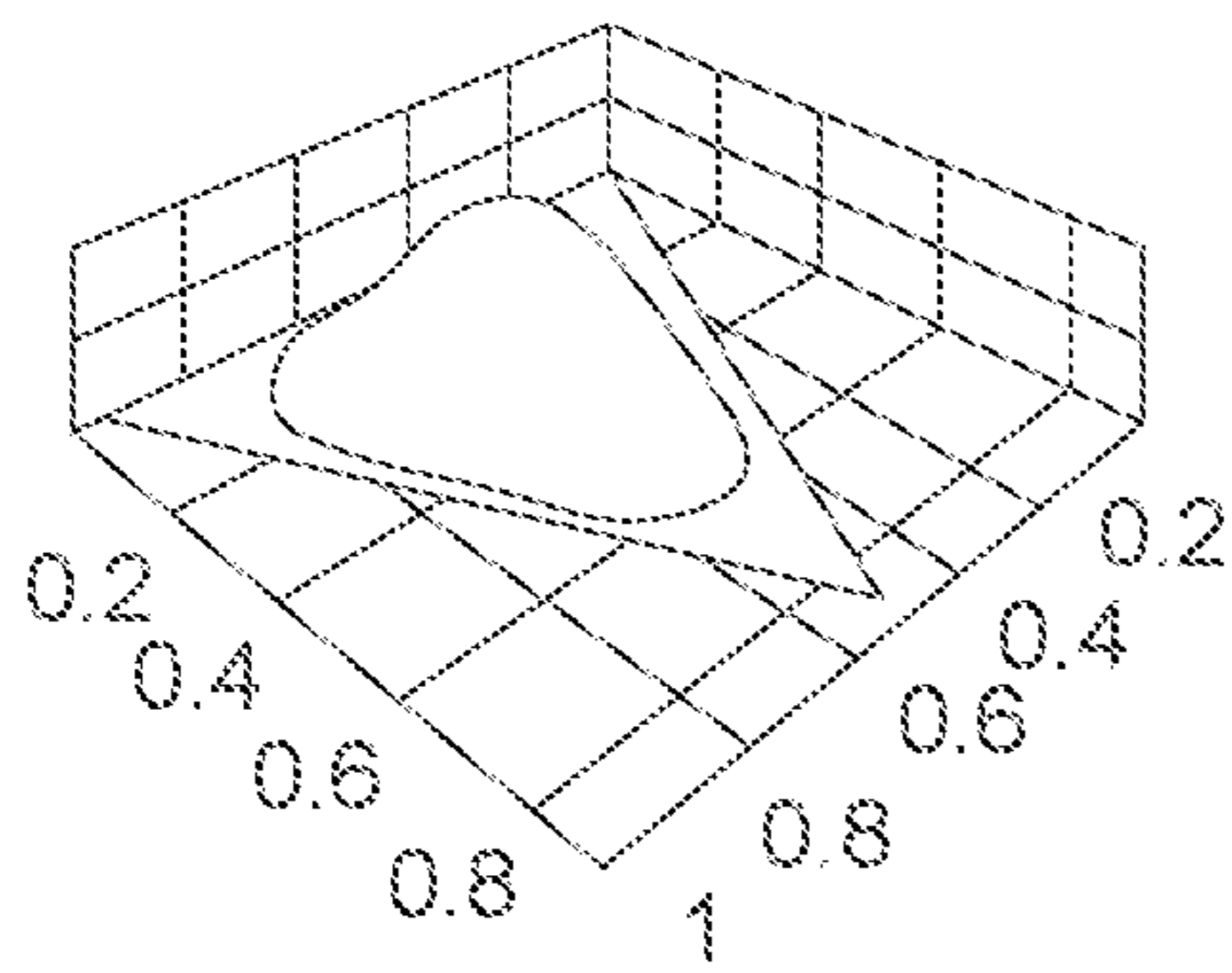
p(y_1|\alpha_1) DISTRIBUTION
