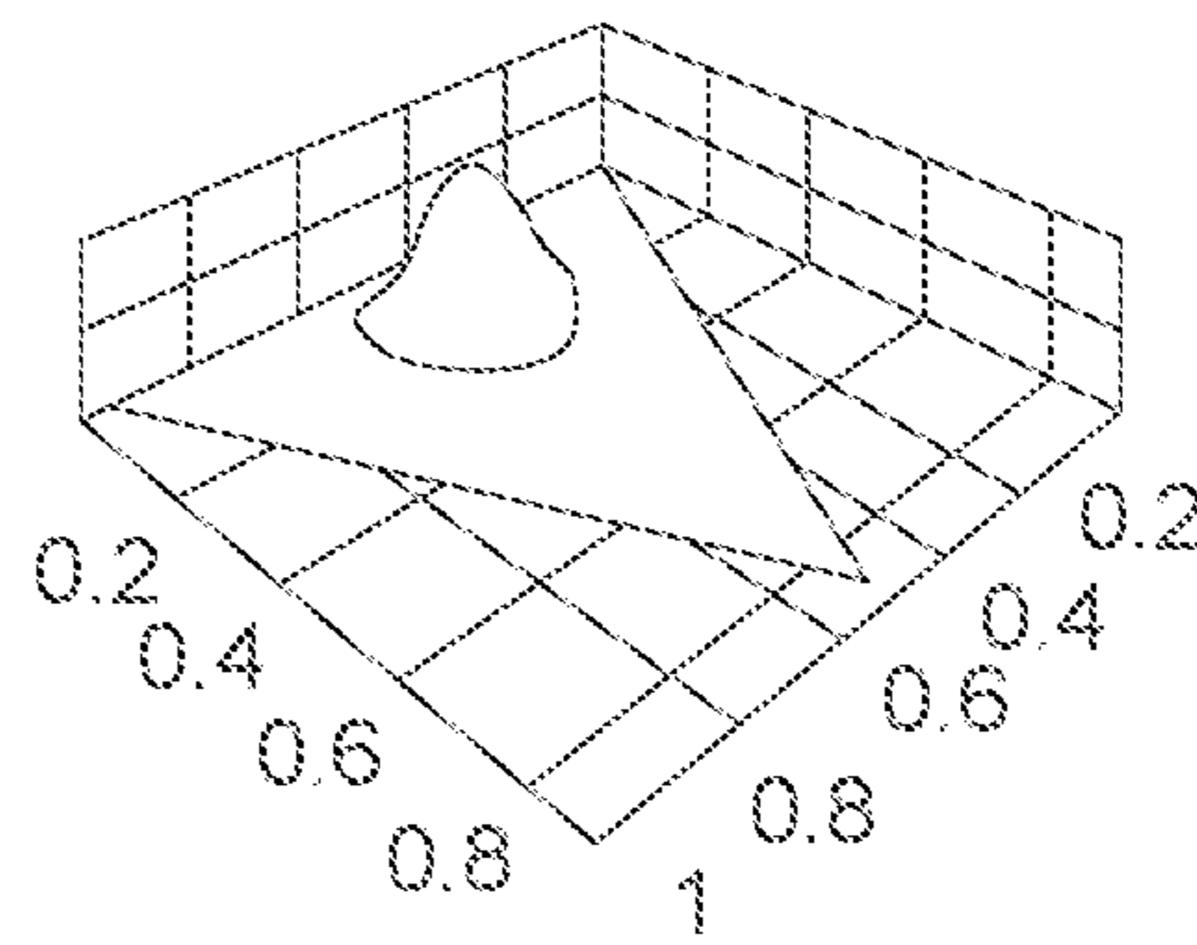
p(y_2|\alpha_2) DISTRIBUTION
