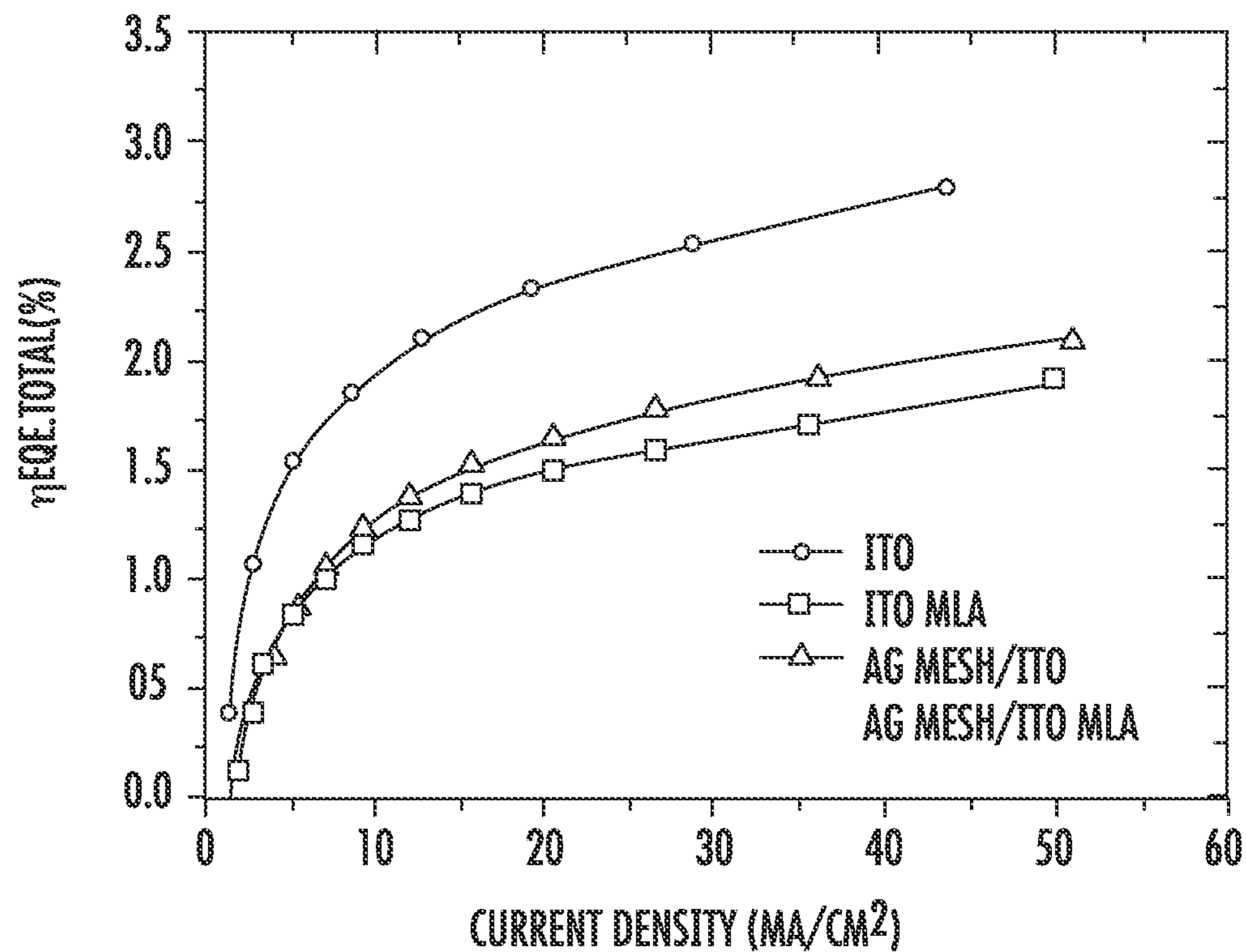
FIGURE 59. PLOT OF EXTERNAL QUANTUM EFFICIENCY VS CURRENT DENSITY WITH DIFFERENT SUBSTRATES
