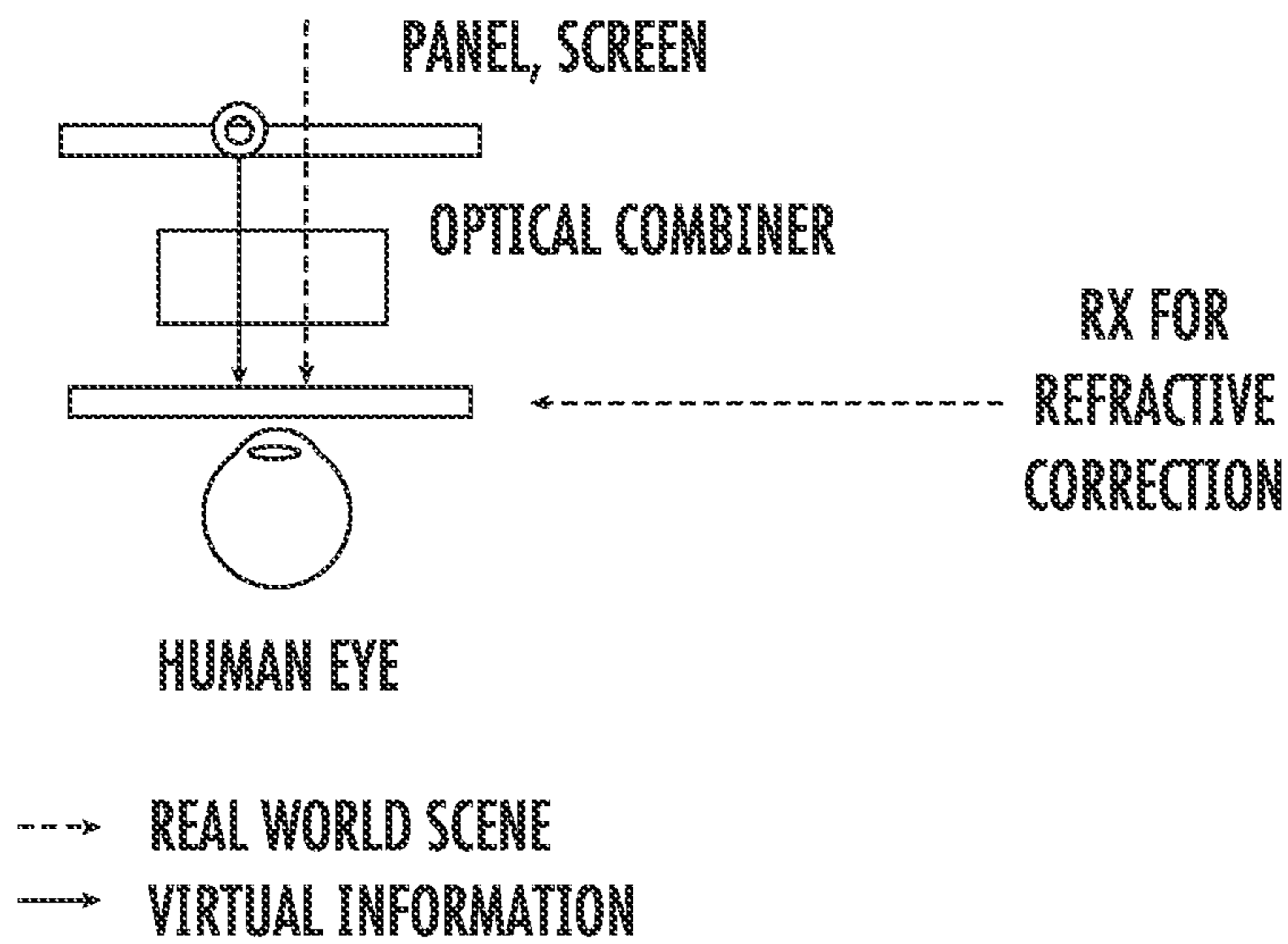
FIGURE 58. USE OF A SEMI-TRANSPARENT OLED SCREEN AS A COMBINER
