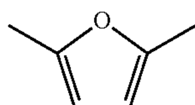
2,5-dimethylfuran
