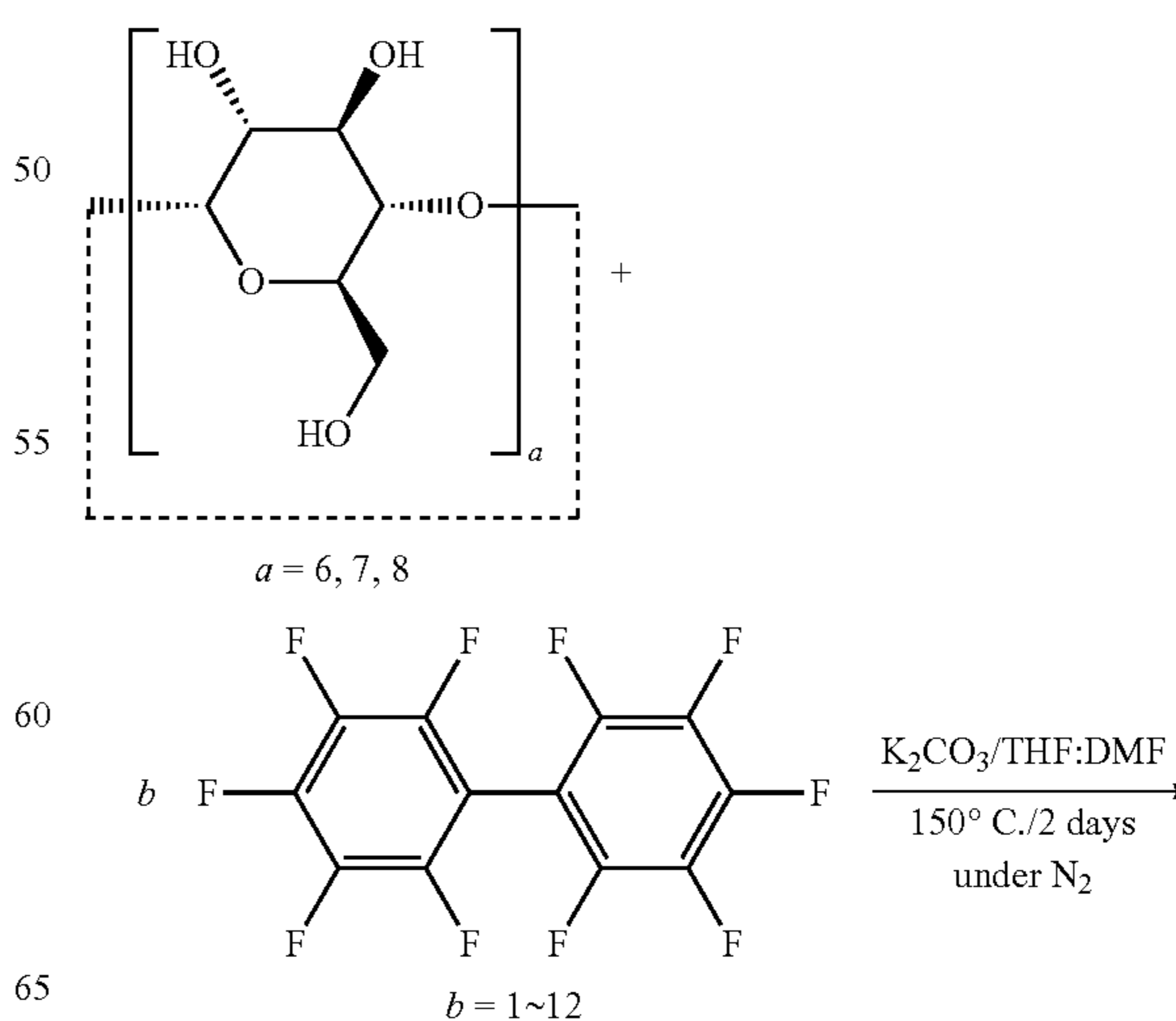
Scheme 2. Synthesis of LX-113
