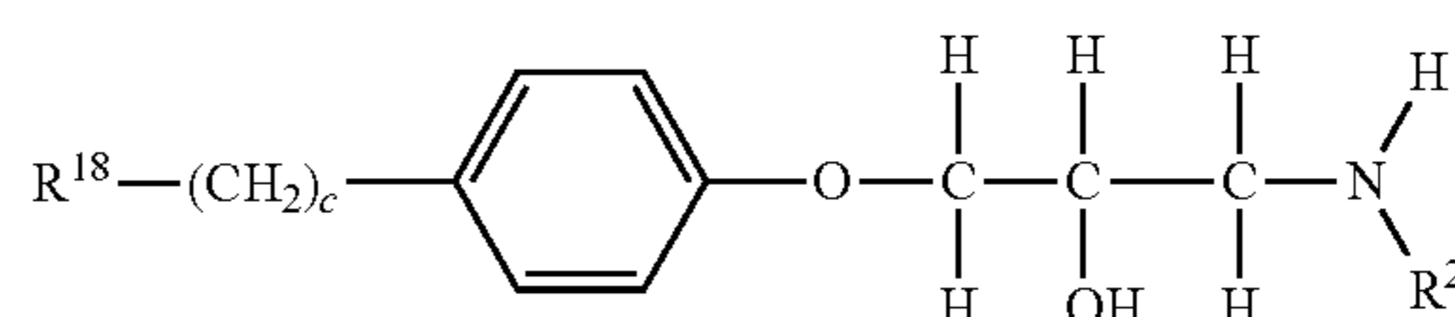
(Formula Ih)
