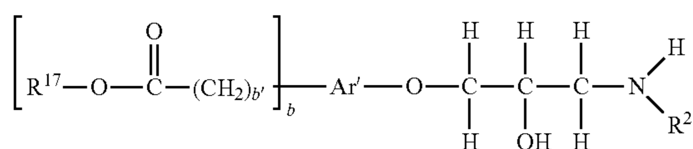
(Formula If)
