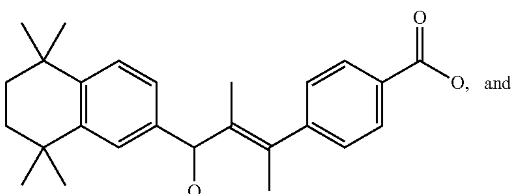
CD666
