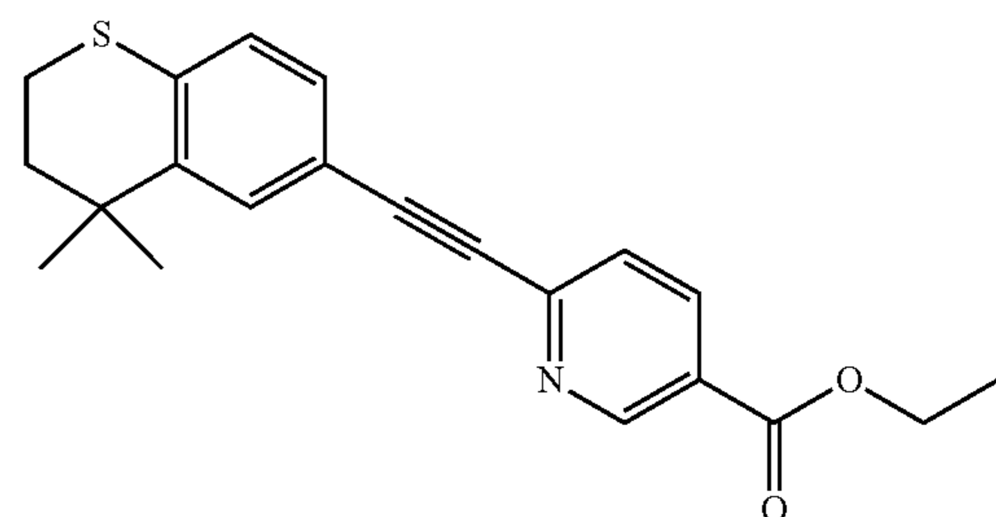
AGN 190168 (Tazarotene)
