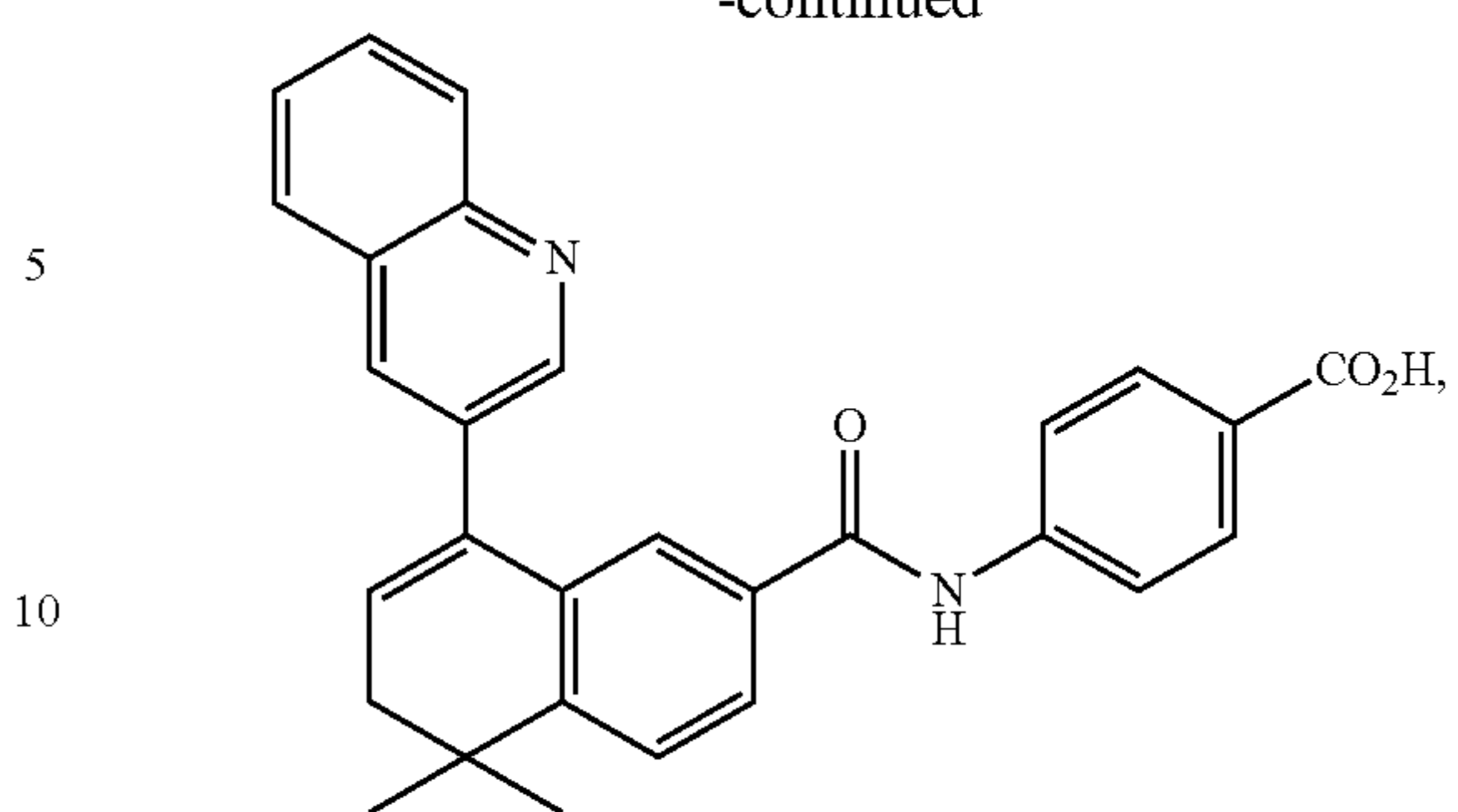
BMS614
