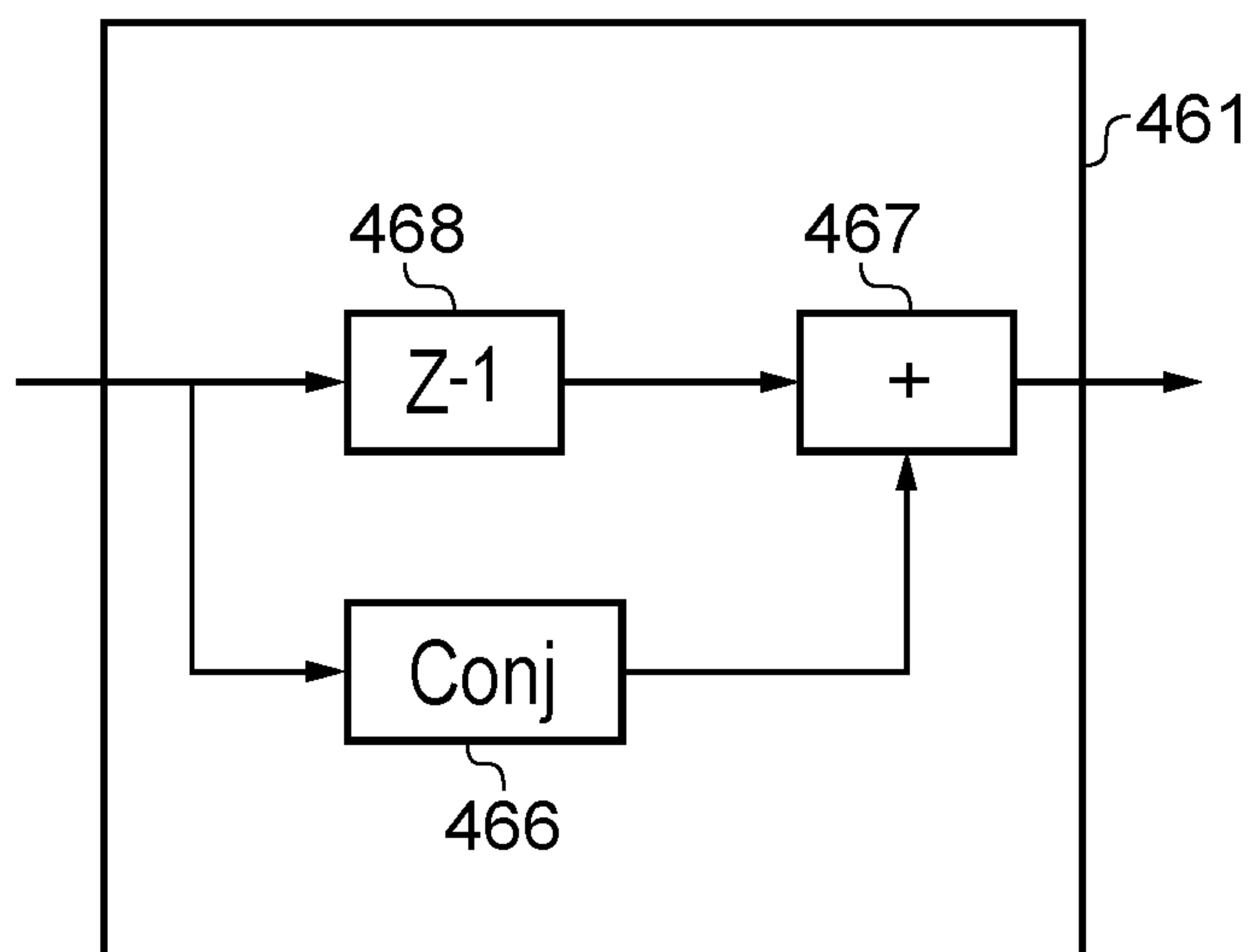
Differential Encoder
