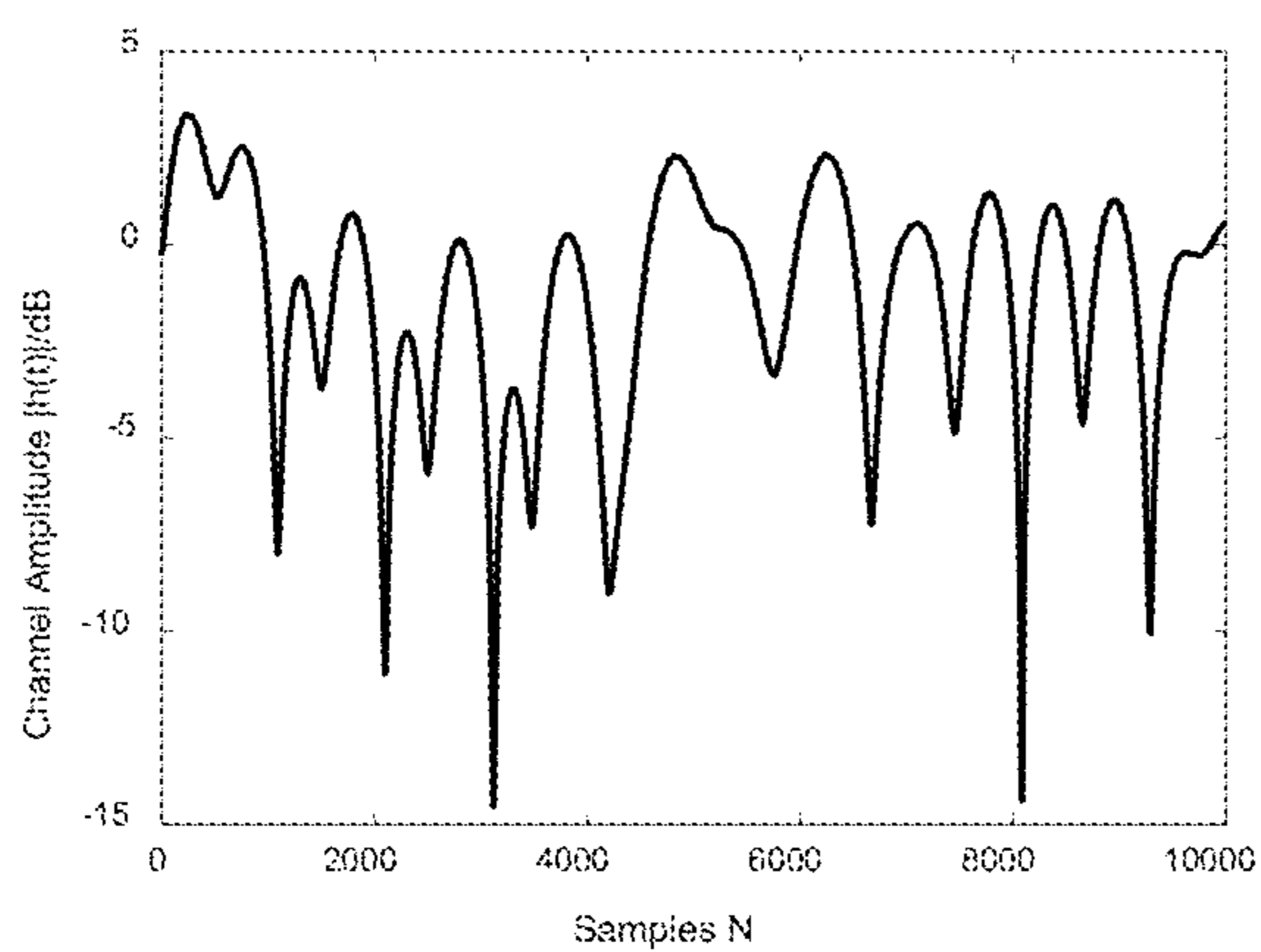
FIG. 5C (Prior Art)
