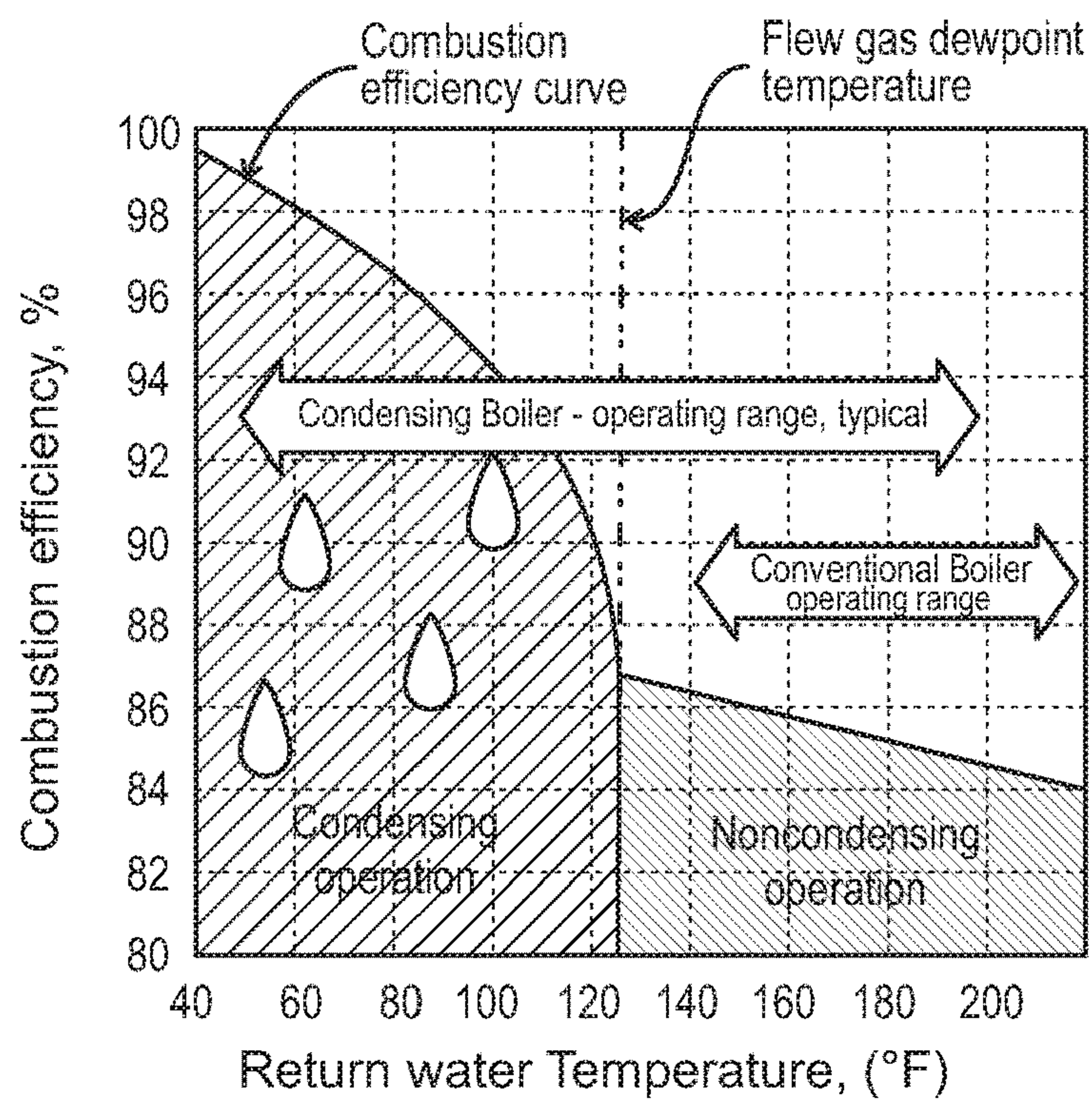
FIG. 1 (PRIOR ART)
